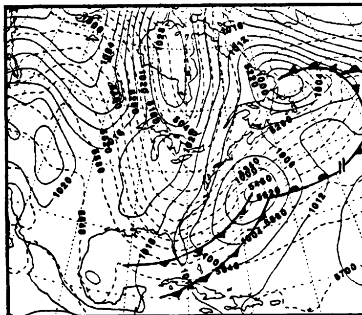
Figure 3.11 Sea-level pressure analysis (solid) mb and 1000-500 mb thickness (dashed) m valid 1200 GMT 25 February 1986.
