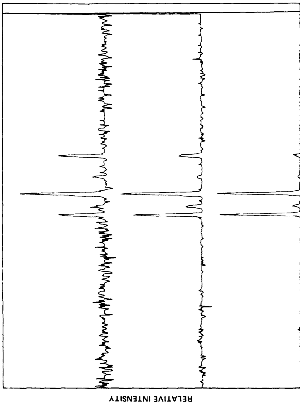
Figure 6. Time resolved (single-shot) CARS spectra of the H_2 Q branch taken at nominal 6-sec intervals after ignition and shown sequentially from bottom to top
