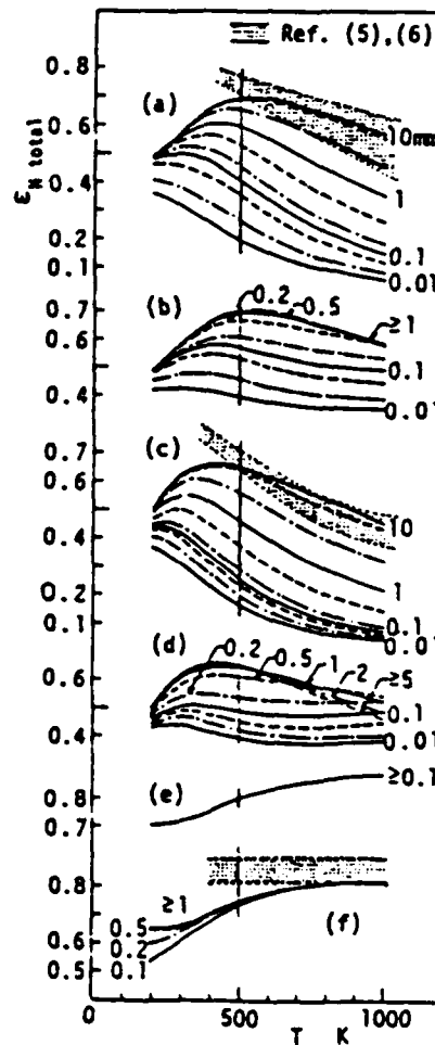
Figure 2-10 Total emittances of ceramic layers: a. Aluminum, b. Aluminum-Hastelloy I, c. Zirconia, d. Zirconia-Hastelloy I, e. Silicon nitride, f. Silicon carbide (Calc.) [92]
