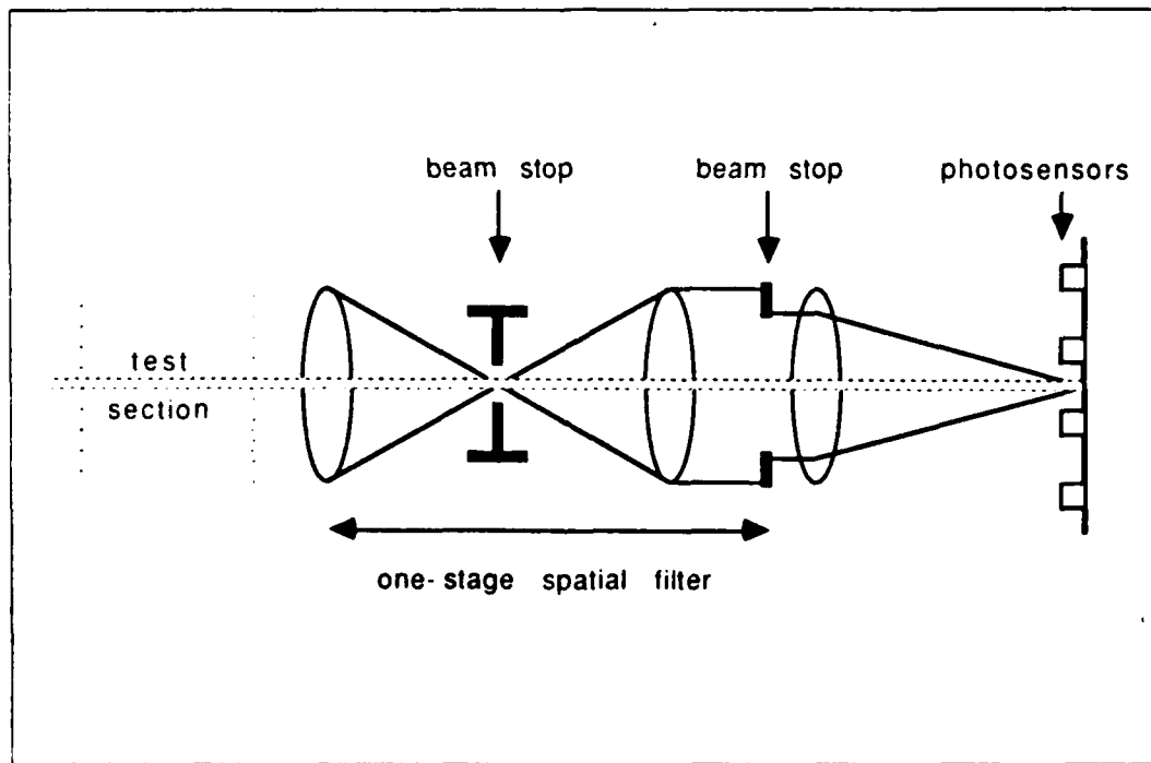
Figure 2.2 Spatial filter.
