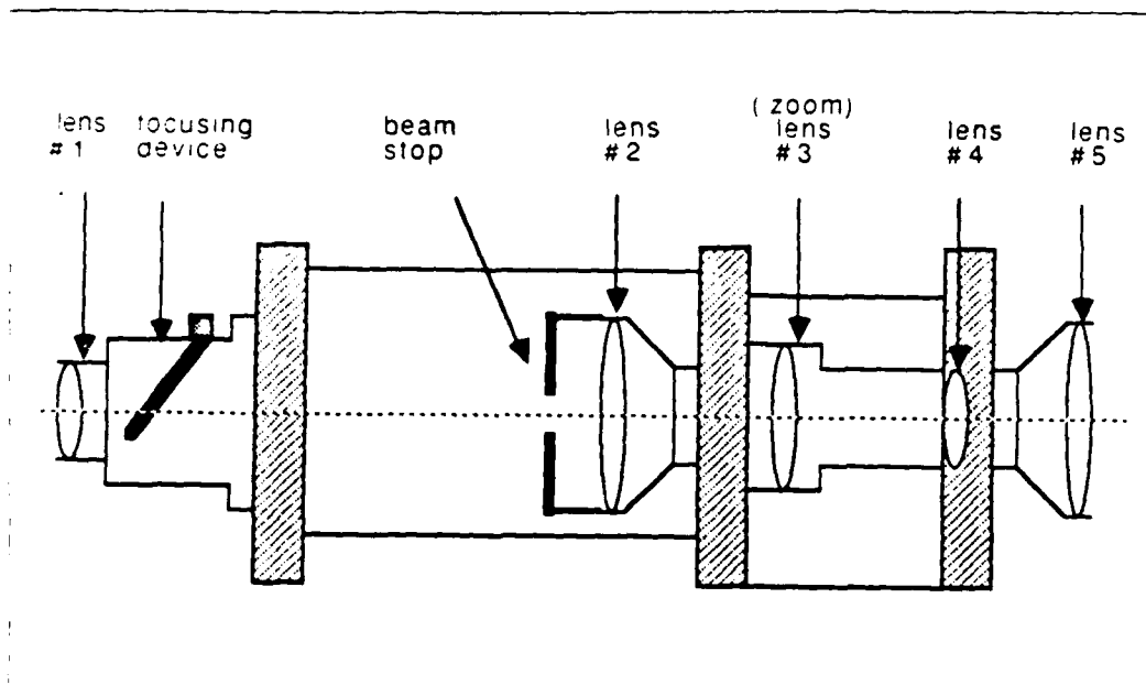
Figure 3.2 Lens' configuration.
