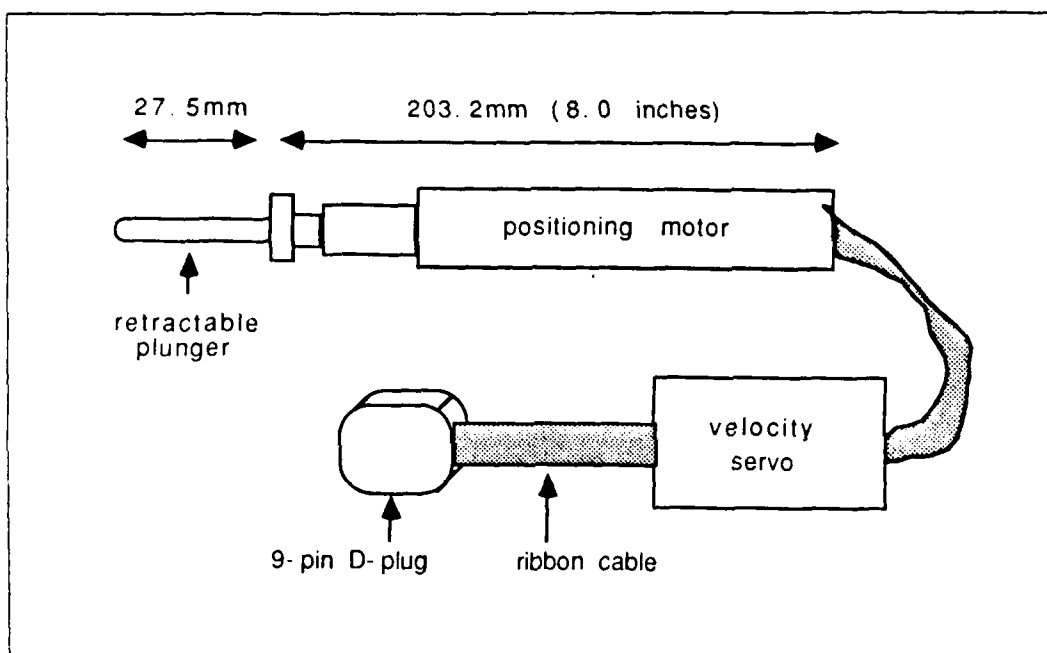
Figure F.1 Positioning motor with velocity servo control box.
