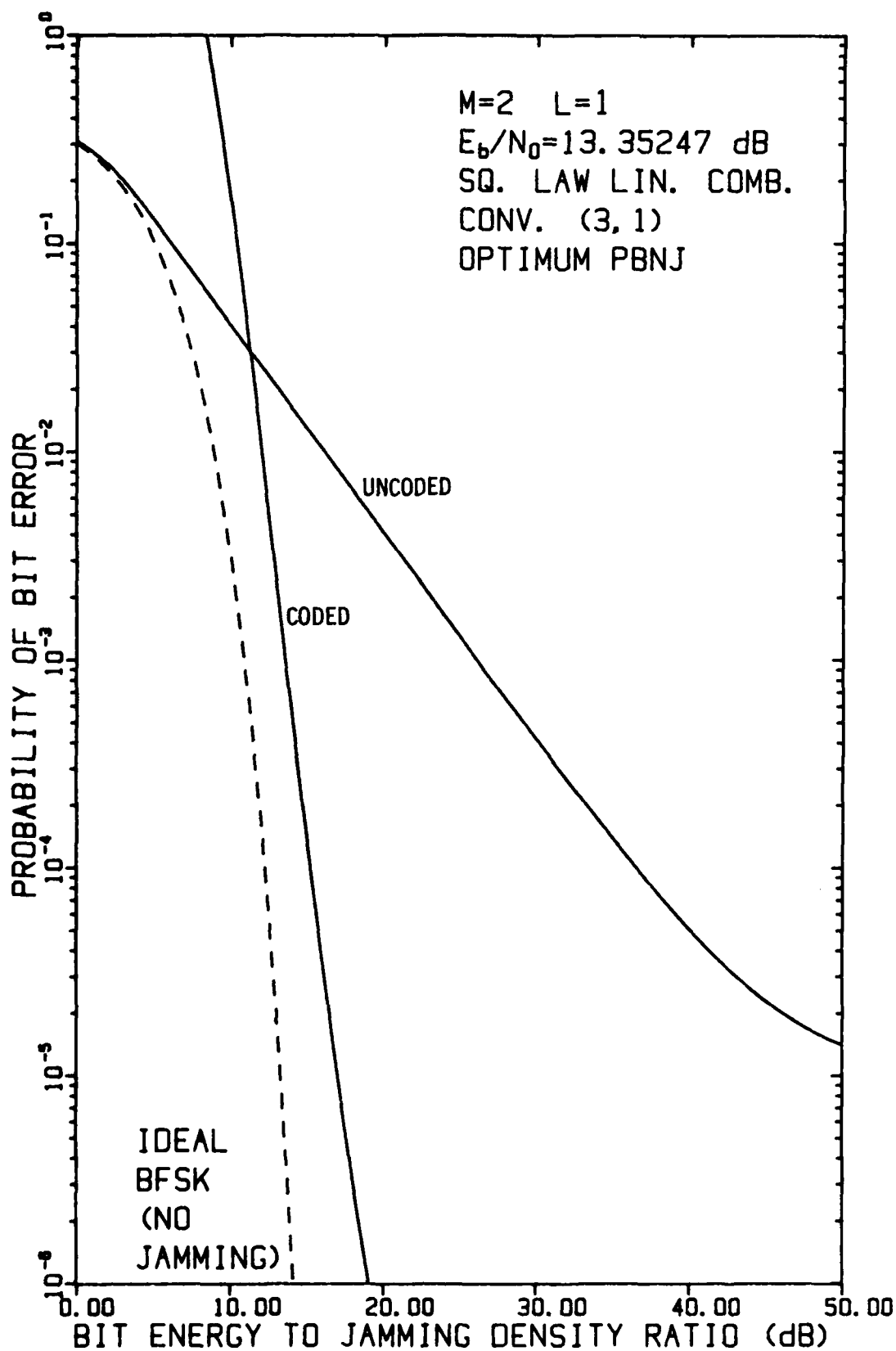
FIGURE 4-53 PERFORMANCE OF FH/BFSK WITH CONVOLUTIONAL RATE-1/3 CODE AND L=1 HOP/DIGIT AS A FUNCTION OF E_b/N_J WHEN E_b/N_0 = 13.35247 dB, USING A LINEAR COMBINING DEMODULATOR, IN OPTIMUM PARTIAL-BAND NOISE JAMMING
