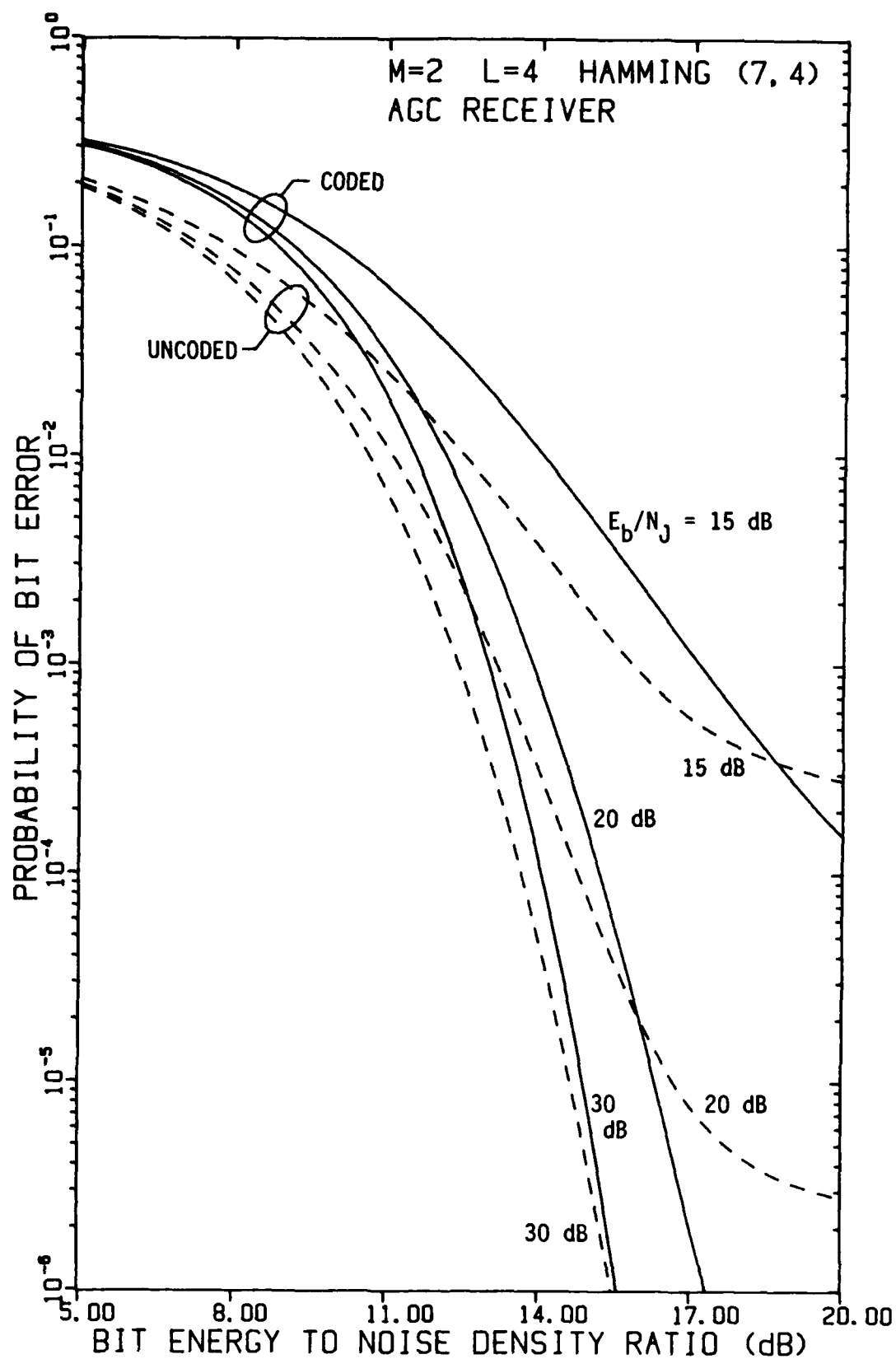
FIGURE 4-73 PERFORMANCE OF FH/BFSK WITH HAMMING (7,4) CODE AND L=4 HOPS/DIGIT AS A FUNCTION OF E_b/N_0 WITH E_b/N_J AS A PARAMETER, USING AN AGC DEMODULATOR, IN OPTIMUM PARTIAL-BAND NOISE JAMMING
