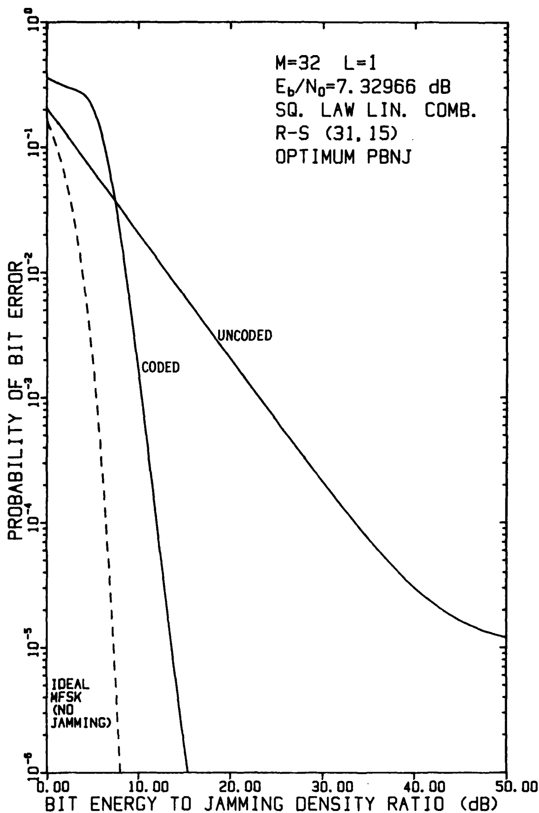
FIGURE 4-68 PERFORMANCE OF FH/MFSK WITH REED-SOLOMON (31,15) CODE AND L=1 HOP/DIGIT AS A FUNCTION OF E_b/N_j WHEN E_b/N_0 = 7.32966 dB, USING A LINEAR COMBINING DEMODULATOR, IN OPTIMUM PARTIAL-BAND NOISE JAMMING
