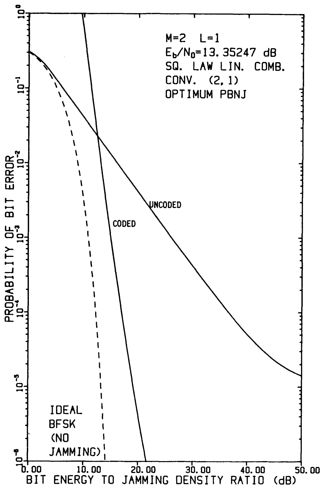
FIGURE 4-49 PERFORMANCE OF FH/BFSK WITH CONVOLUTIONAL RATE-1/2 CODE AND L=1 HOP/DIGIT AS A FUNCTION OF E_b/N_j WHEN E_b/N_0 = 13.35247 dB, USING A LINEAR COMBINING DEMODULATOR, IN OPTIMUM PARTIAL-BAND NOISE JAMMING
