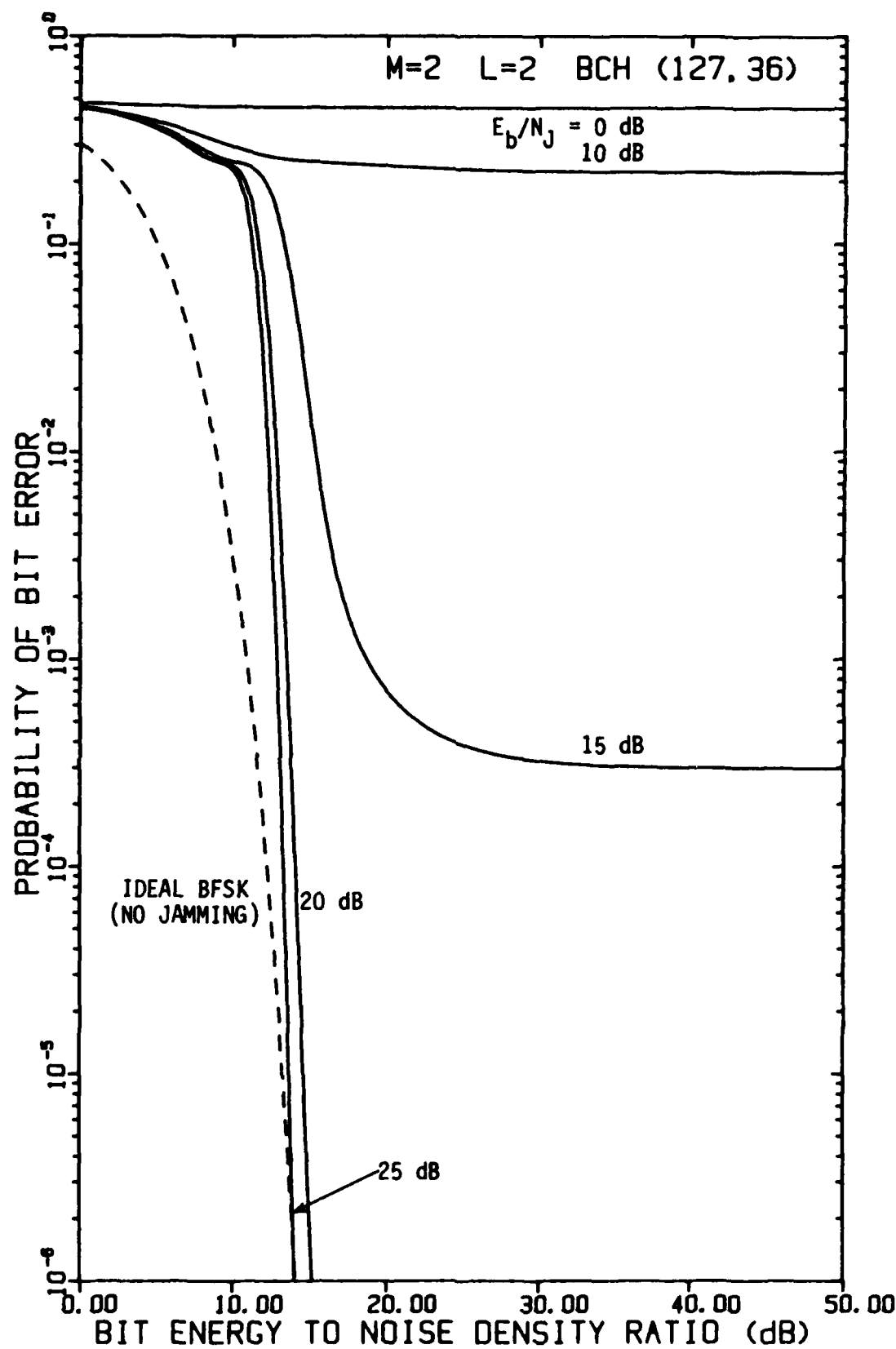
FIGURE 4-38 PERFORMANCE OF FH/BFSK WITH BCH (127,36) CODE AND L=2 HOPS/DIGIT AS A FUNCTION OF E_b/N_0 WITH E_b/N_J AS A PARAMETER, USING A LINEAR COMBINING DEMODULATOR, IN OPTIMUM PARTIAL-BAND NOISE JAMMING
