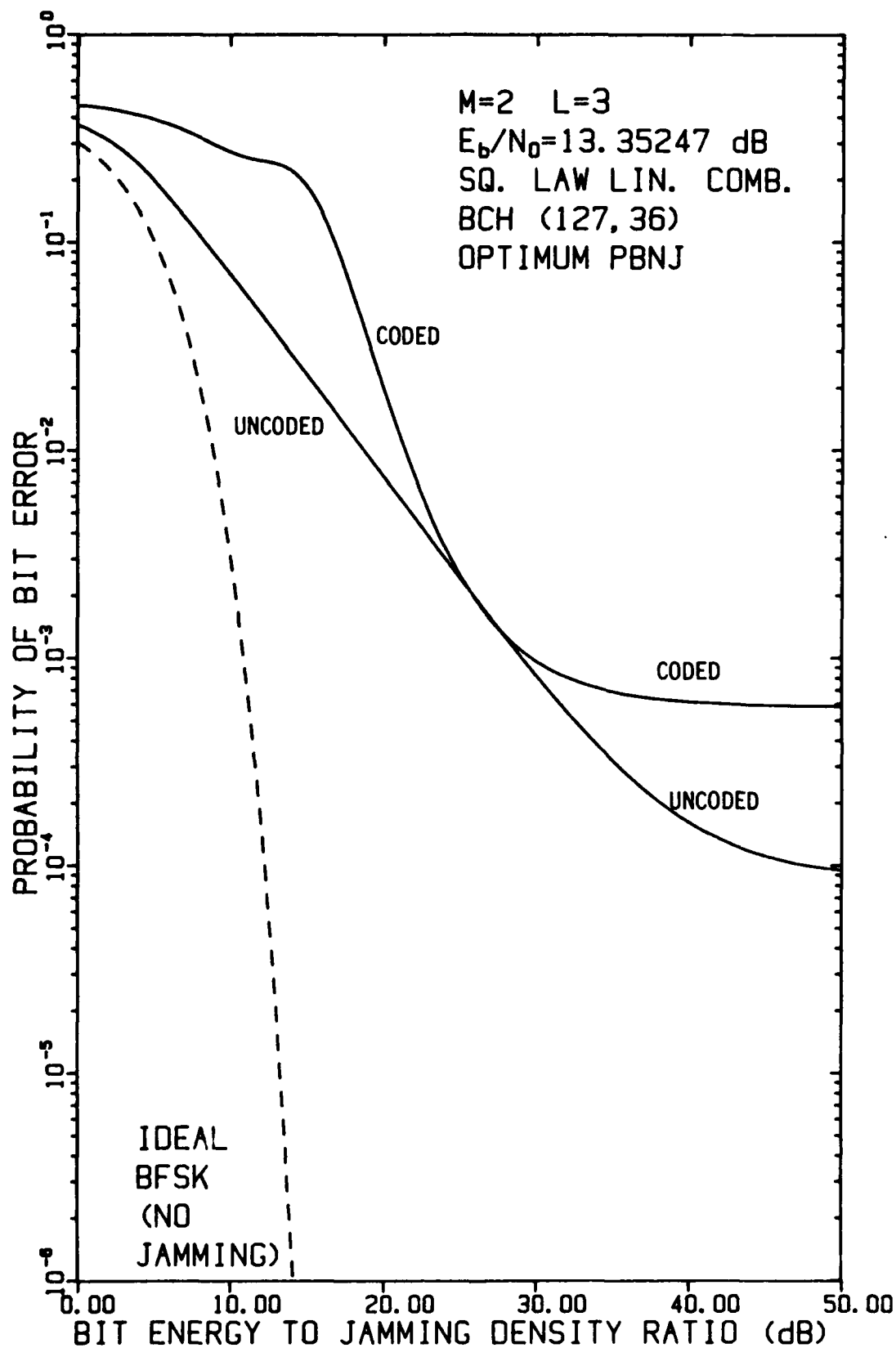
FIGURE 4-43 PERFORMANCE OF FH/BFSK WITH BCH (127,36) CODE AND L=3 HOPS/DIGIT AS A FUNCTION OF E_b/N_j WHEN E_b/N_0 = 13.35247 dB, USING A LINEAR COMBINING DEMODULATOR, IN OPTIMUM PARTIAL-BAND NOISE JAMMING
