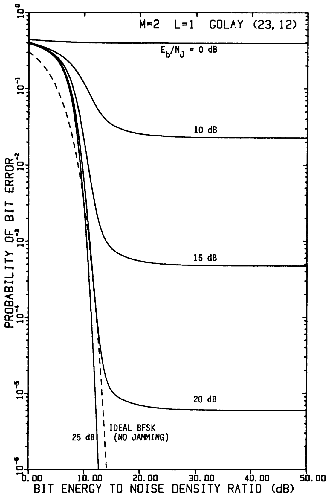
FIGURE 4-13 PERFORMANCE OF FH/BFSK WITH GOLAY (23,12) CODE AND L=1 HOP/DIGIT AS A FUNCTION OF E_b/N_0 WITH E_b/N_j AS A PARAMETER, USING A LINEAR COMBINING DEMODULATOR, IN OPTIMUM PARTIAL-BAND NOISE JAMMING
