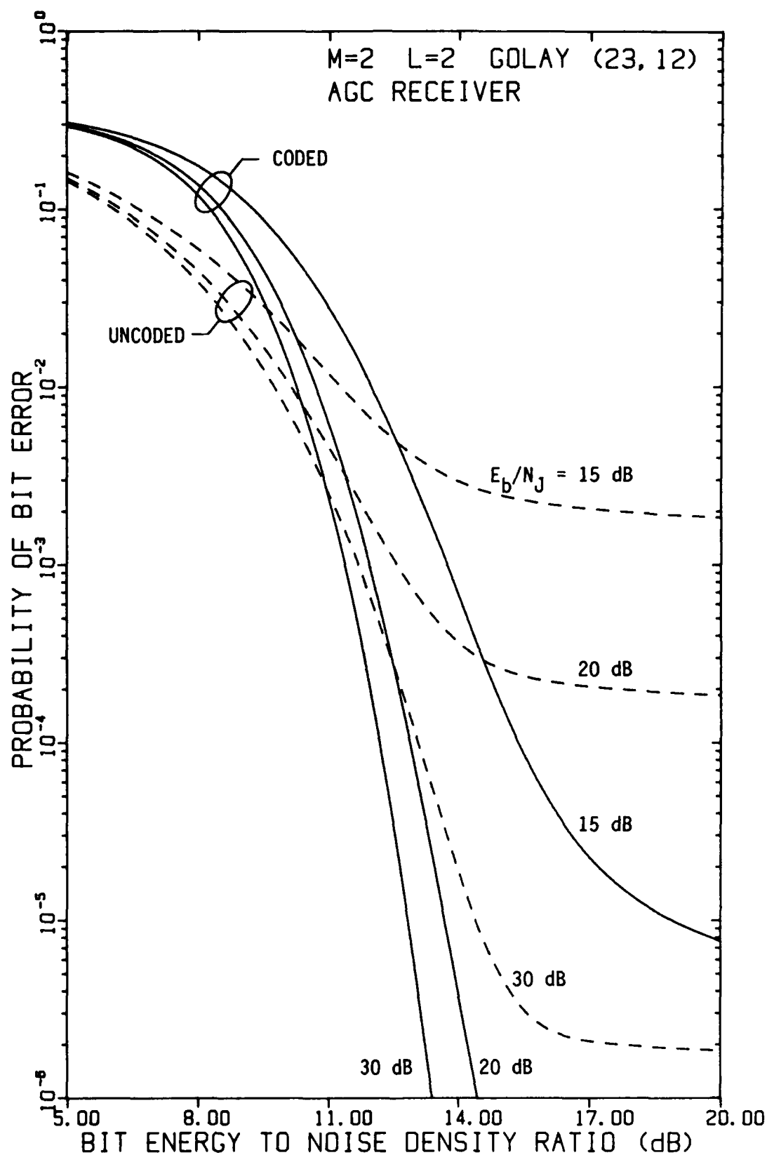
FIGURE 4-75 PERFORMANCE OF FH/BFSK WITH GOLAY (23,12) CODE AND L=2 HOPS/DIGIT AS A FUNCTION OF E_b/N_0 WITH E_b/N_j AS A PARAMETER, USING AN AGC DEMODULATOR, IN OPTIMUM PARTIAL-BAND NOISE JAMMING
