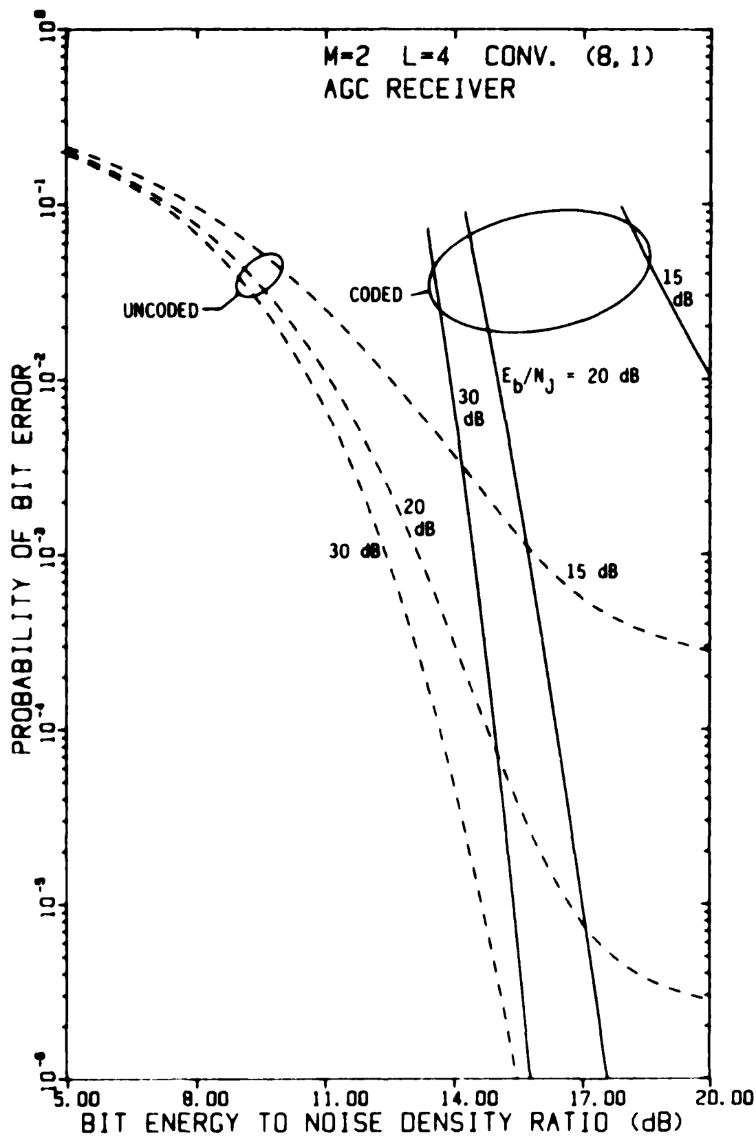
FIGURE 4-109 PERFORMANCE OF FH/BFSK WITH CONVOLUTIONAL RATE-1/8 CODE AND L=4 HOPS/DIGIT AS A FUNCTION OF E_b/N_0 WITH E_b/N_J AS A PARAMETER, USING AN AGC DEMODULATOR, IN OPTIMUM PARTIAL-BAND NOISE JAMMING
