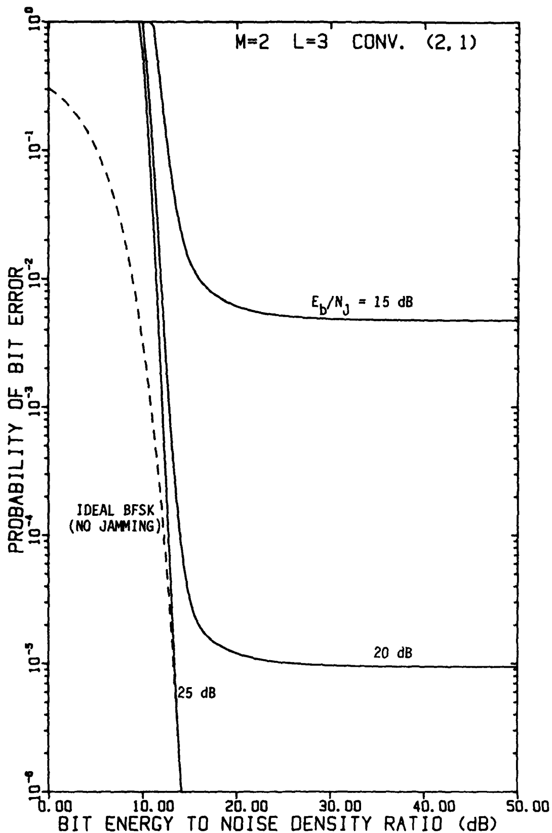
FIGURE 4-47 PERFORMANCE OF FH/BFSK WITH CONVOLUTIONAL RATE-1/2 CODE AND L=3 HOPS/DIGIT AS A FUNCTION OF E_b/N_0 WITH E_b/N_j AS A PARAMETER, USING A LINEAR COMBINING DEMODULATOR, IN OPTIMUM PARTIAL-BAND NOISE JAMMING
