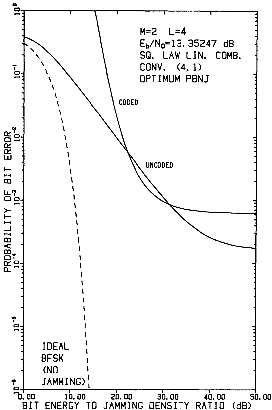
FIGURE 4-60 PERFORMANCE OF FH/BFSK WITH CONVOLUTIONAL RATE-1/4 CODE AND L=4 HOPS/DIGIT AS A FUNCTION OF E_b/N_j WHEN E_b/N_0 = 13.35247 dB, USING A LINEAR COMBINING DEMODULATOR, IN OPTIMUM PARTIAL-BAND NOISE JAMMING
