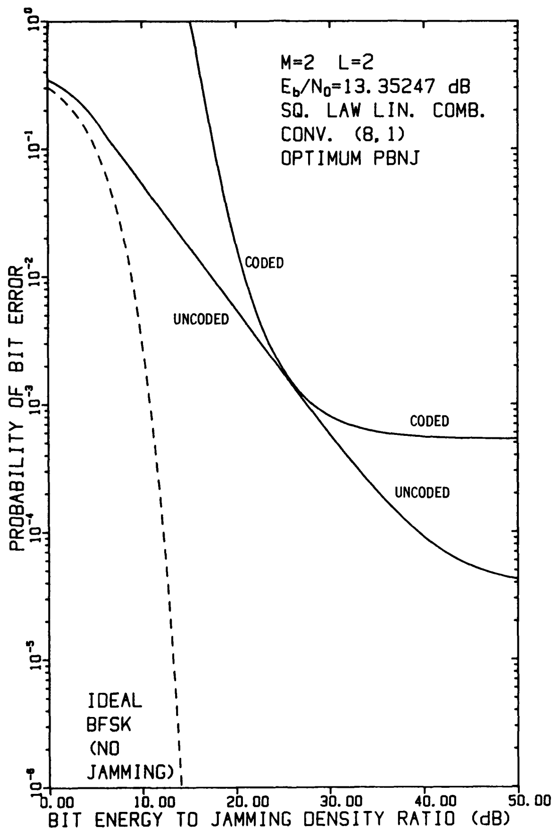
FIGURE 4-62 PERFORMANCE OF FH/BFSK WITH CONVOLUTIONAL RATE-1/8 CODE AND L=2 HOPS/DIGIT AS A FUNCTION OF E_b/N_J WHEN E_b/N_0 = 13.35247 dB, USING A LINEAR COMBINING DEMODULATOR, IN OPTIMUM PARTIAL-BAND NOISE JAMMING
