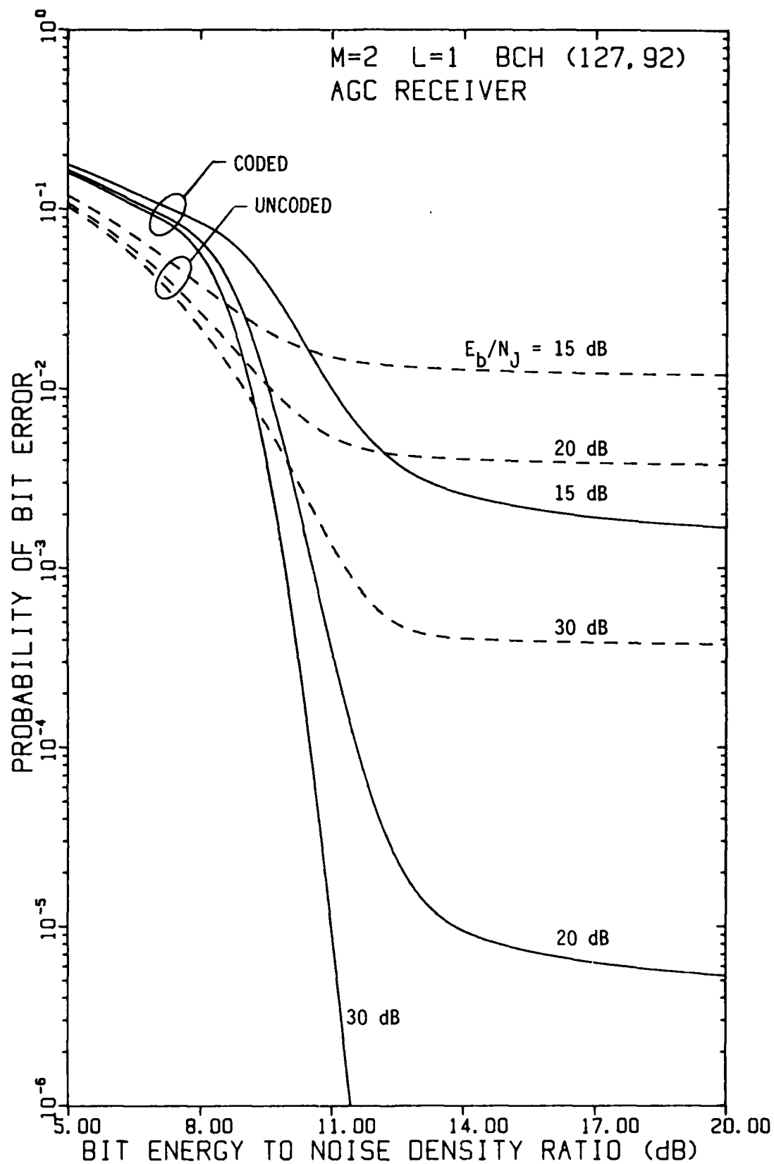
FIGURE 4-78 PERFORMANCE OF FH/BFSK WITH BCH (127,92) CODE AND L=1 HOP/DIGIT AS A FUNCTION OF E_b/N_0 WITH E_b/N_j AS A PARAMETER, USING AN AGC DEMODULATOR, IN OPTIMUM PARTIAL-BAND NOISE JAMMING
