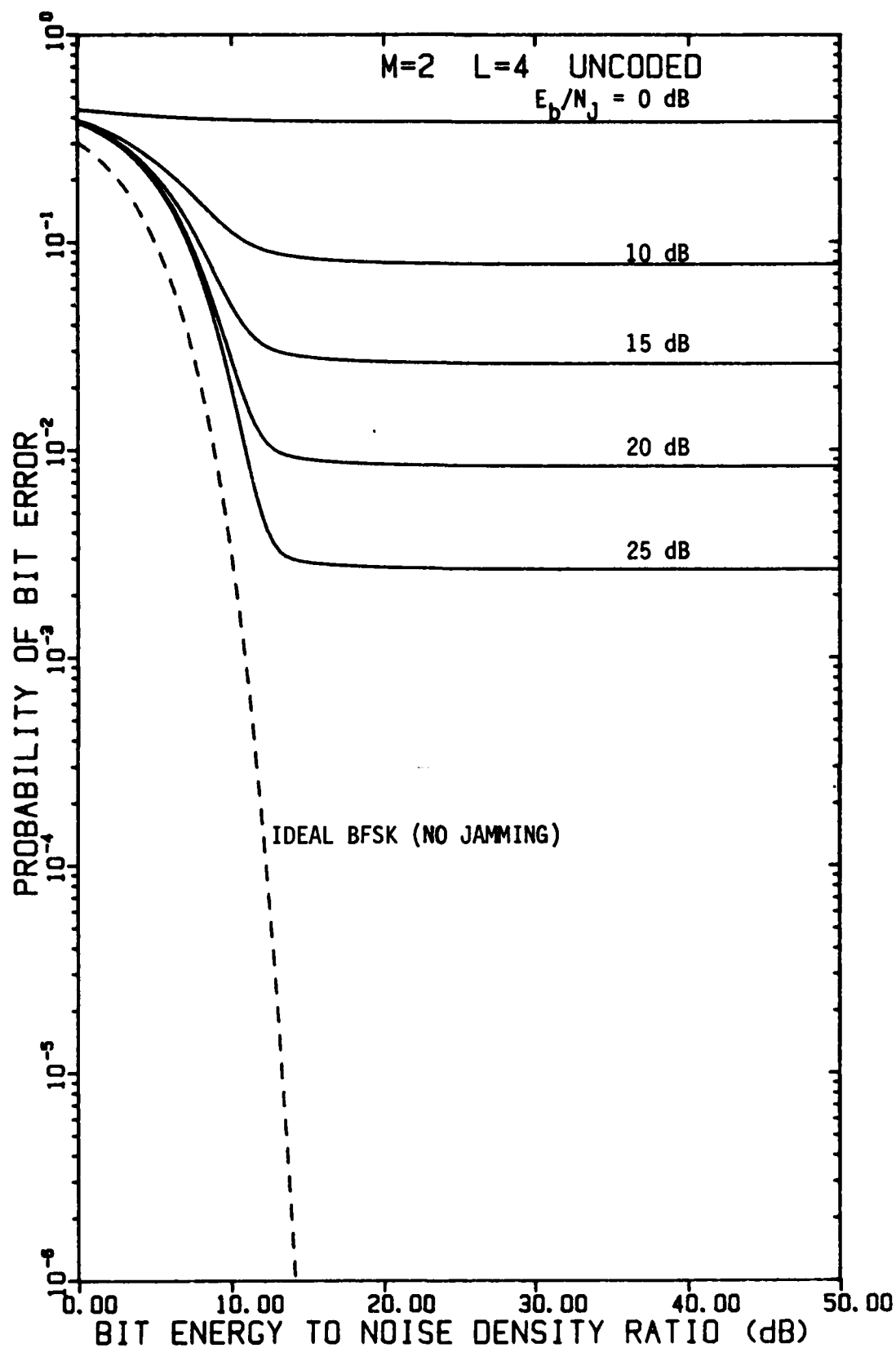
FIGURE 4-4 PERFORMANCE OF UNCODED BFSK WITH L=4 HOPS/BIT AS A FUNCTION OF E_b/N_0 WITH E_b/N_j AS A PARAMETER, USING A LINEAR COMBINING DEMODULATOR, IN OPTIMUM PARTIAL-BAND NOISE JAMMING
