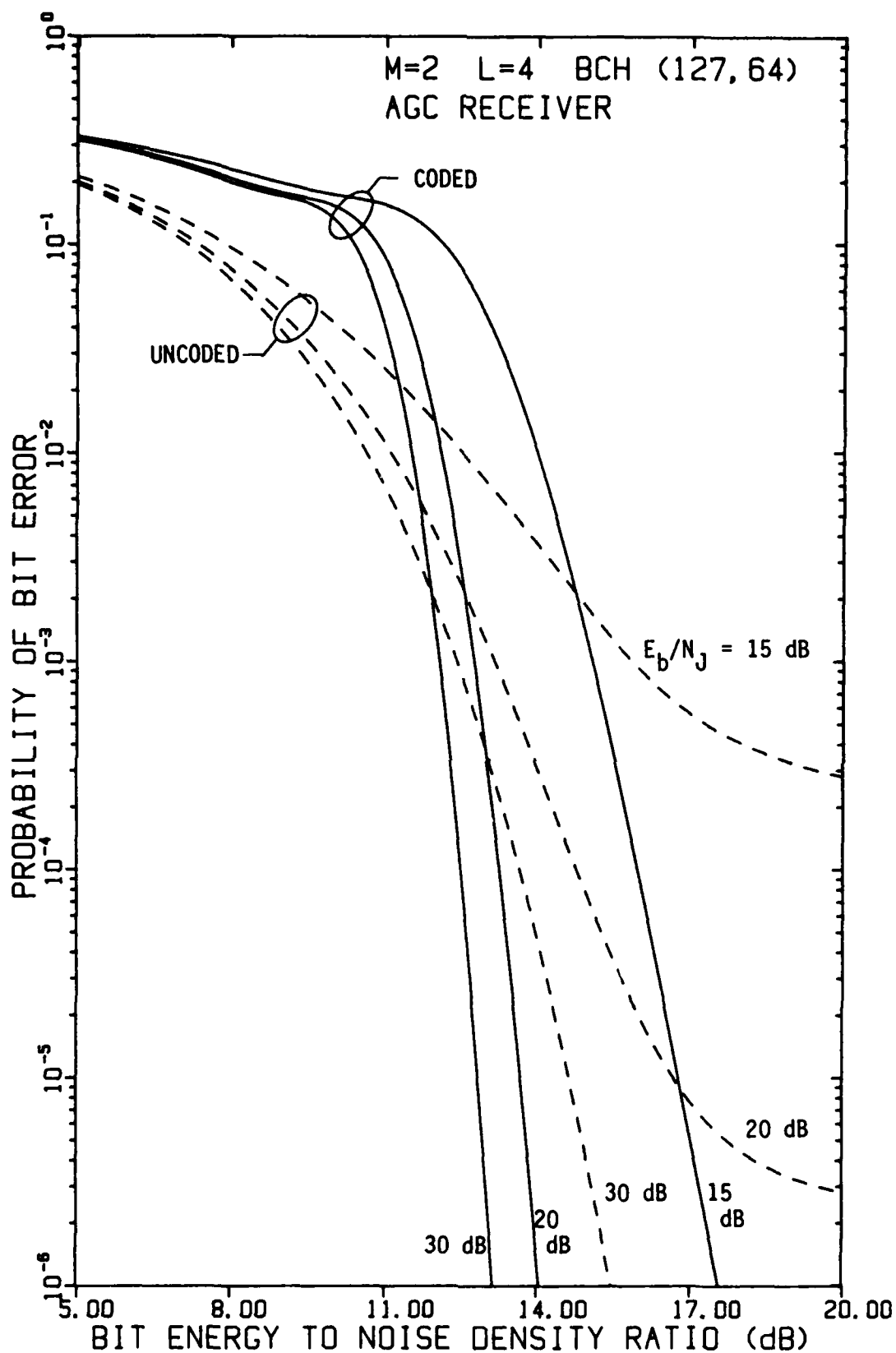
FIGURE 4-85 PERFORMANCE OF FH/BFSK WITH BCH (127,64) CODE AND L=4 HOPS/DIGIT AS A FUNCTION OF E_b/N_0 WITH E_b/N_j AS A PARAMETER, USING AN AGC DEMODULATOR, IN OPTIMUM PARTIAL-BAND NOISE JAMMING
