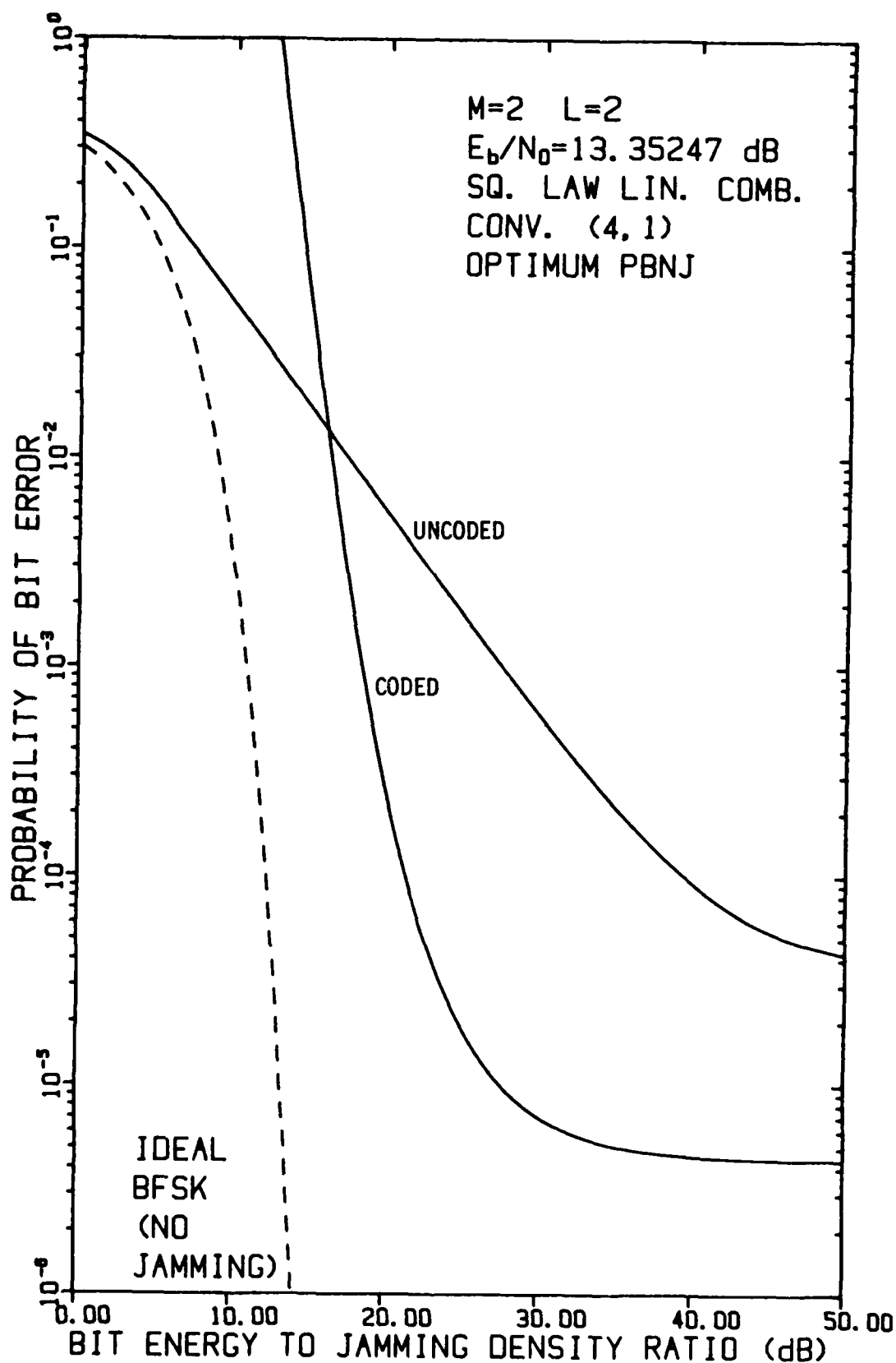
FIGURE 4-58 PERFORMANCE OF FH/BFSK WITH CONVOLUTIONAL RATE-1/4 CODE AND L=2 HOPS/DIGIT AS A FUNCTION OF E_b/N_j WHEN E_b/N_0 = 13.35247 dB, USING A LINEAR COMBINING DEMODULATOR, IN OPTIMUM PARTIAL-BAND NOISE JAMMING
