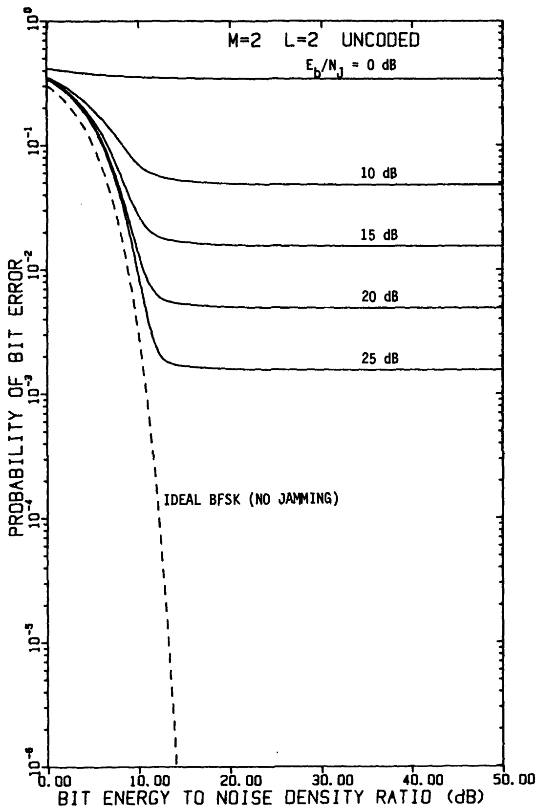
FIGURE 4-2 PERFORMANCE OF UNCODED BFSK WITH L=2 HOPS/BIT AS A FUNCTION OF E_b/N_0 WITH E_b/N_J AS A PARAMETER, USING A LINEAR COMBINING DEMODULATOR, IN OPTIMUM PARTIAL-BAND NOISE JAMMING
