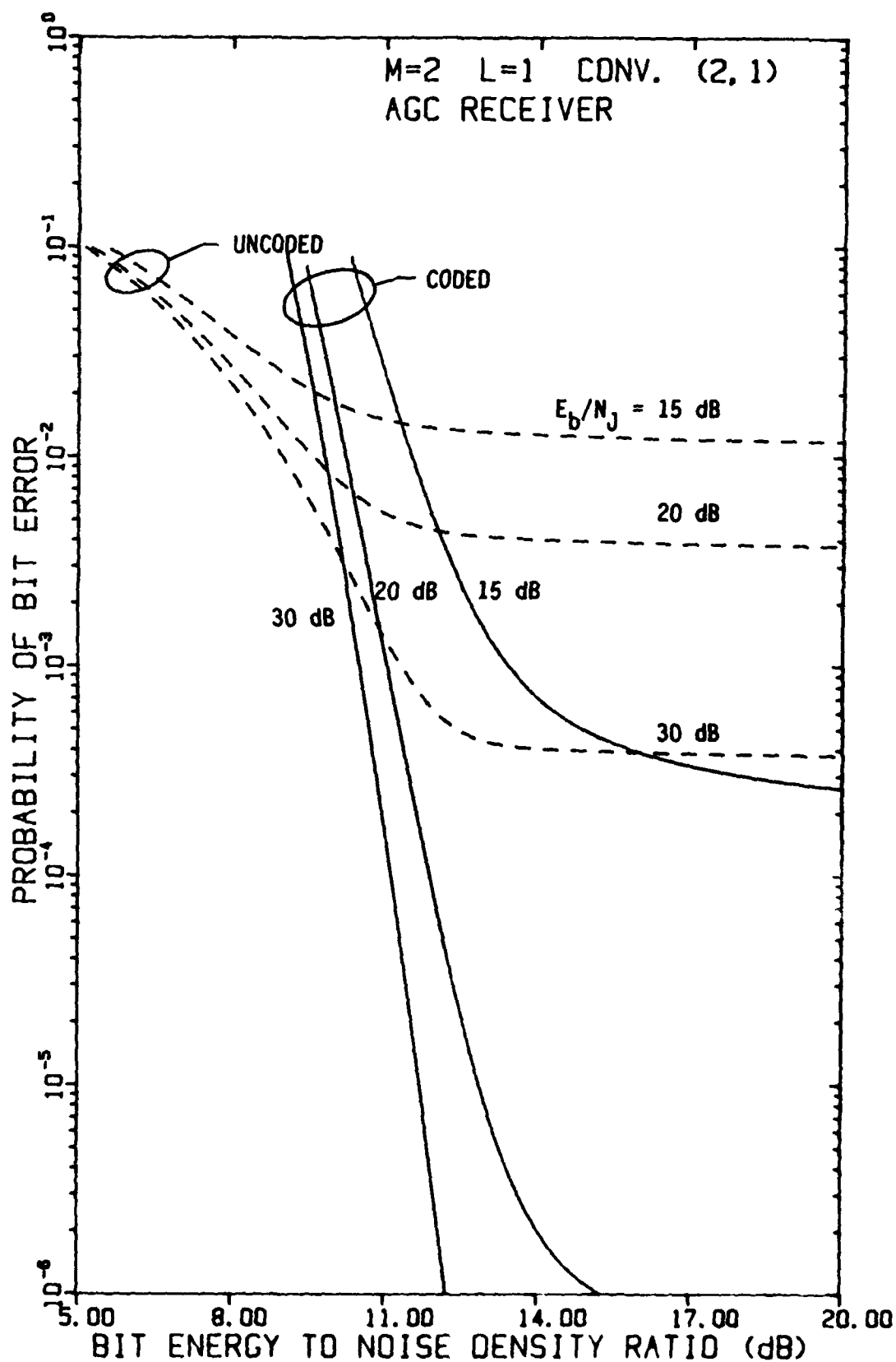
FIGURE 4-94 PERFORMANCE OF FH/BFSK WITH CONVOLUTIONAL RATE-1/2 CODE AND L=1 HOP/DIGIT AS A FUNCTION OF E_b/N_0 WITH E_b/N_j AS A PARAMETER, USING AN AGC DEMODULATOR, IN OPTIMUM PARTIAL-BAND NOISE JAMMING
