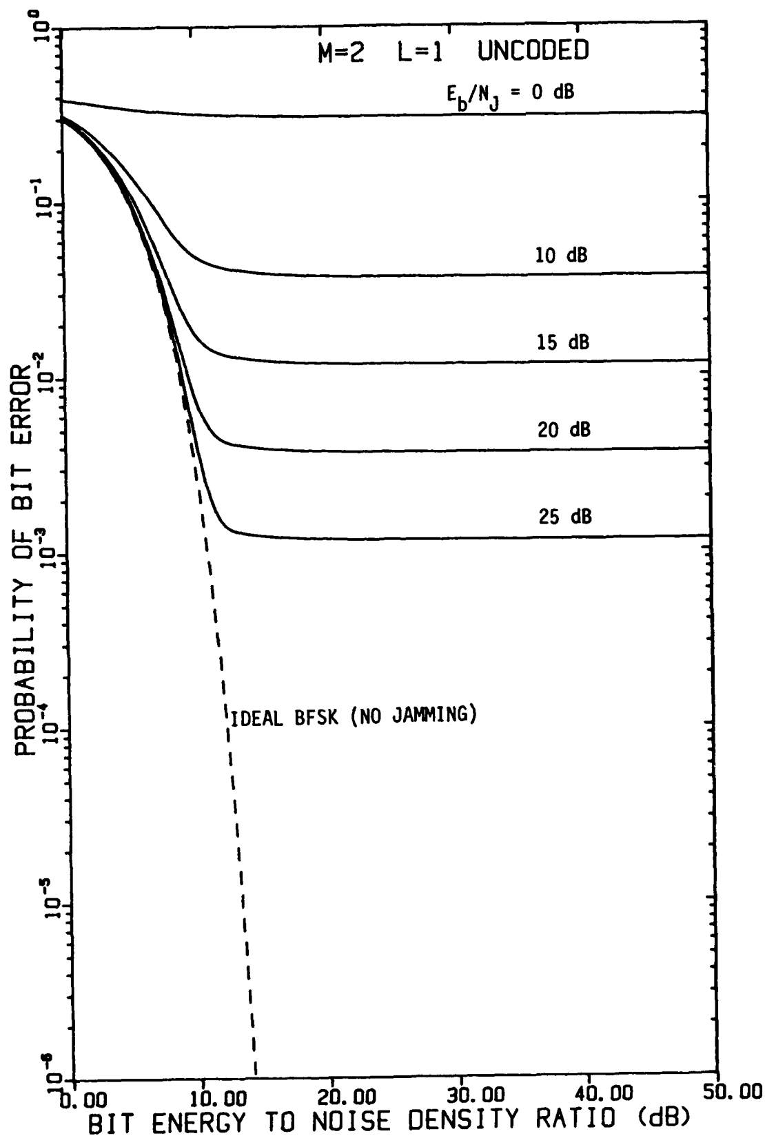
FIGURE 4-1 PERFORMANCE OF UNCODED BFSK WITH L=1 HOP/BIT AS A FUNCTION OF E_b/N_0 WITH E_b/N_j AS A PARAMETER, USING A LINEAR COMBINING DEMODULATOR, IN OPTIMUM PARTIAL-BAND NOISE JAMMING
