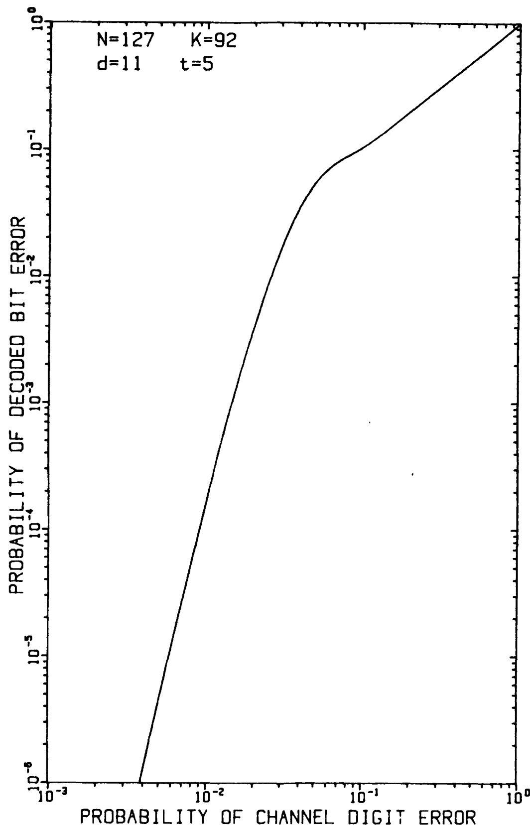
FIGURE 3-3 DECODER PERFORMANCE FOR BCH (127,92) CODE
