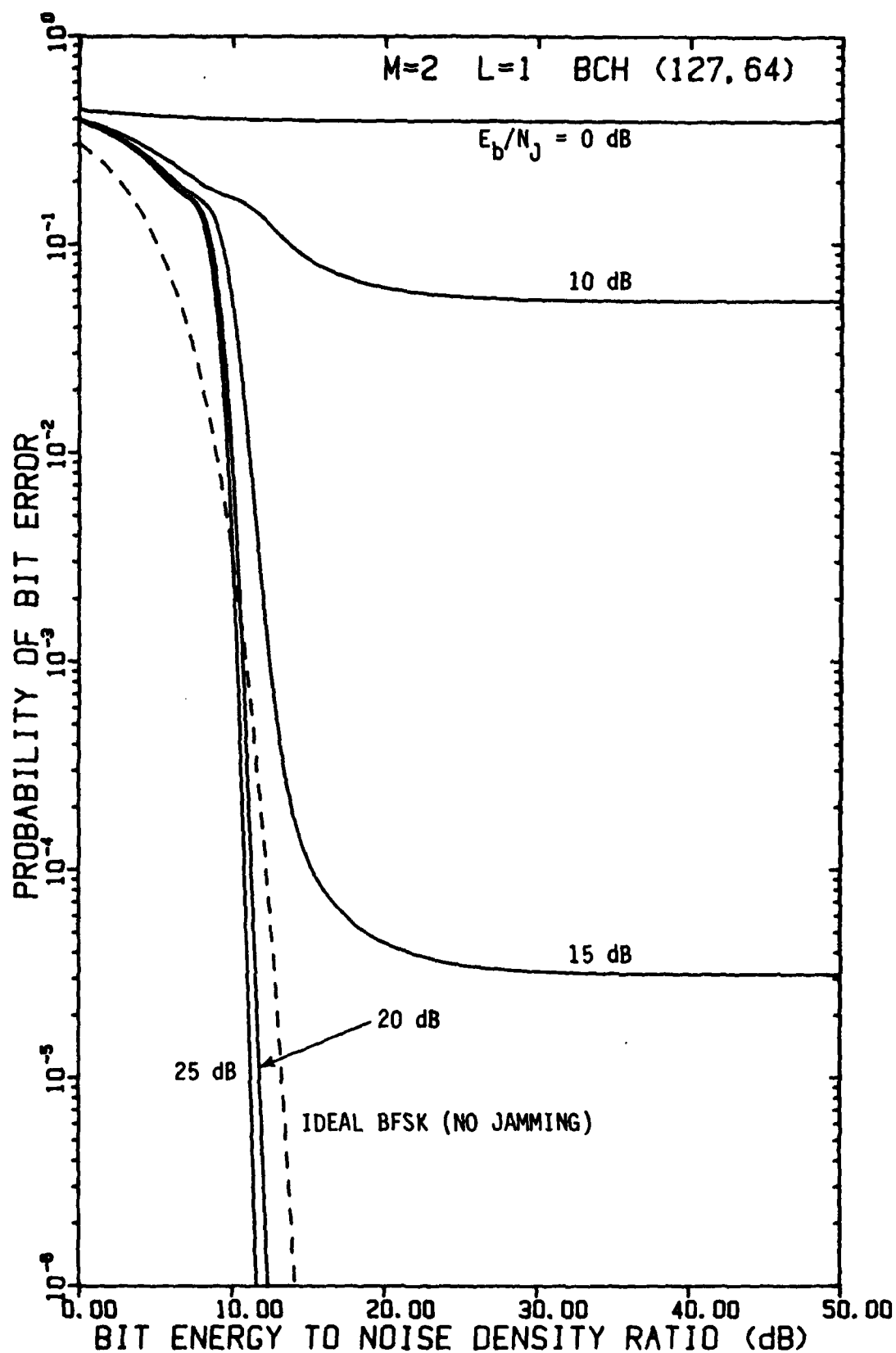
FIGURE 4-29 PERFORMANCE OF FH/BFSK WITH BCH (127,64) CODE AND L=1 HOP/DIGIT AS A FUNCTION OF E_b/N_0 WITH E_b/N_j AS A PARAMETER, USING A LINEAR COMBINING DEMODULATOR, IN OPTIMUM PARTIAL-BAND NOISE JAMMING
