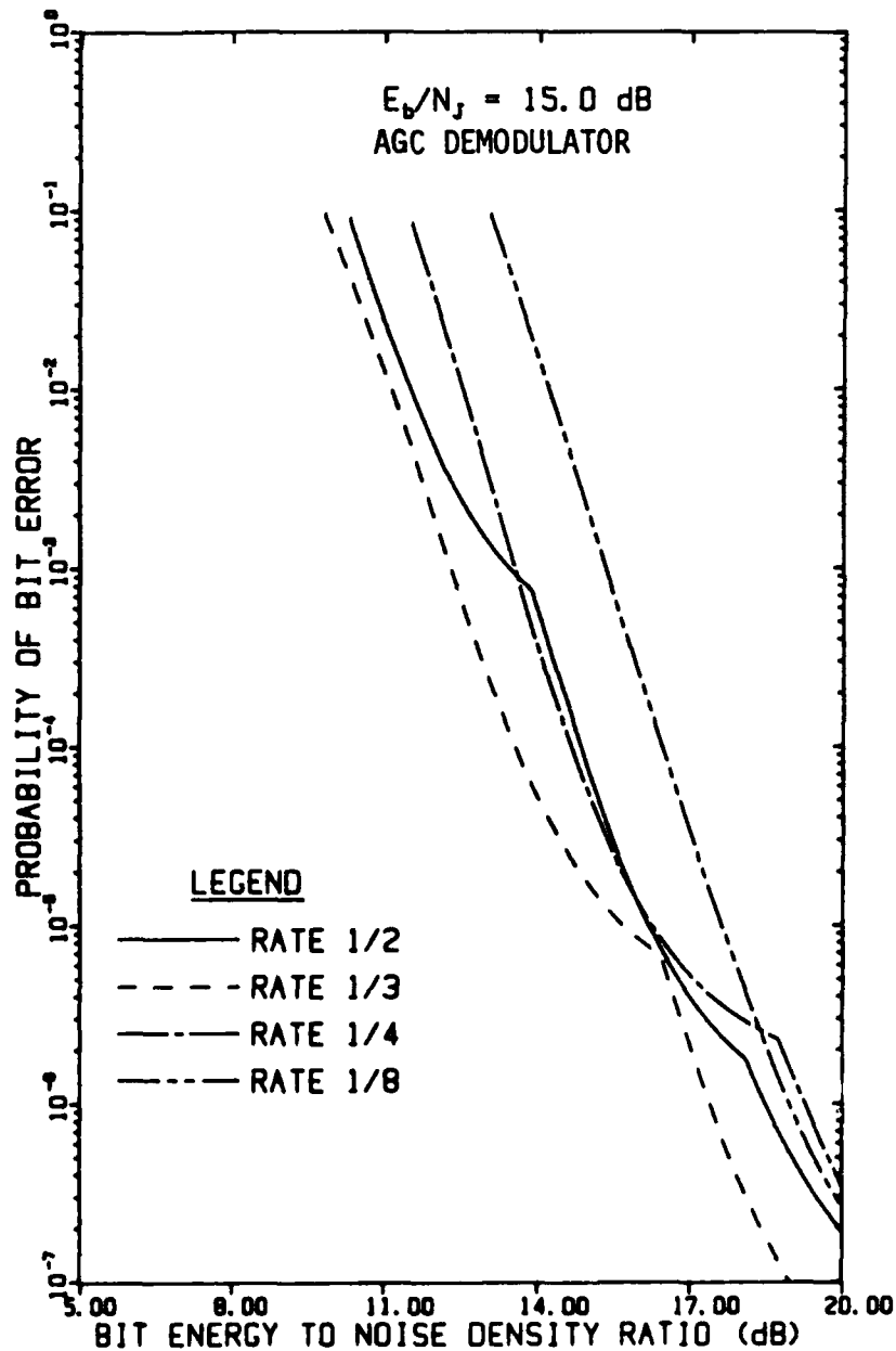
FIGURE 4-110 PERFORMANCE OF CONSTRAINT-LENGTH-7 CONVOLUTIONAL CODES USING OPTIMUM DIVERSITY IN WORST-CASE PARTIAL-BAND NOISE JAMMING AS A FUNCTION OF E_b/N_0 WHEN E_b/N_J = 15 \text{ dB}
