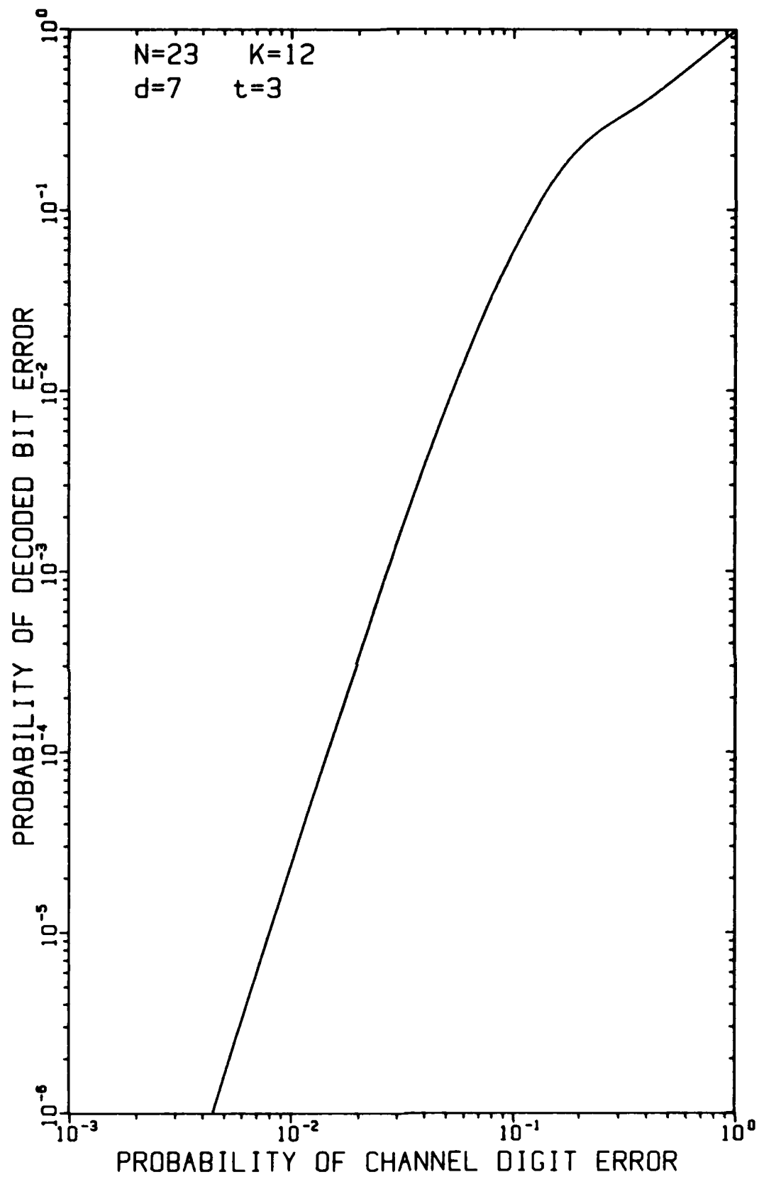
FIGURE 3-2 DECODER PERFORMANCE FOR GOLAY (23,12) CODE
