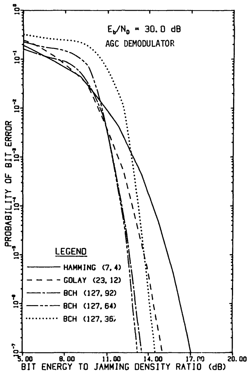
FIGURE 4-92 PERFORMANCE OF BLOCK CODES USING FH/BFSK WITH OPTIMUM DIVERSITY IN WORST-CASE PARTIAL-BAND NOISE JAMMING AS A FUNCTION OF E_b/N_J WHEN E_b/N_0 = 30 \text{ dB}
