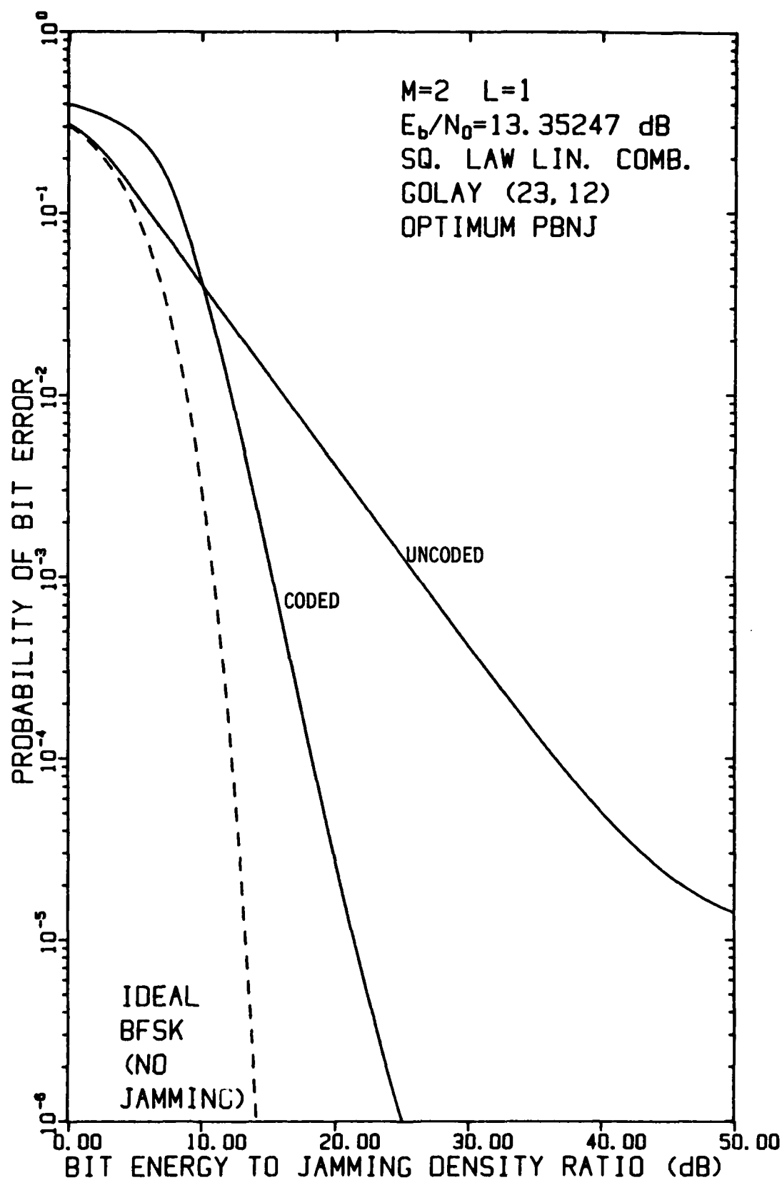
FIGURE 4-17 PERFORMANCE OF FH/BFSK WITH GOLAY (23,12) CODE AND L=1 HOP/DIGIT AS A FUNCTION OF E_b/N_j WHEN E_b/N_0 = 13.35247 dB, USING A LINEAR COMBINING DEMODULATOR, IN OPTIMUM PARTIAL-BAND NOISE JAMMING
