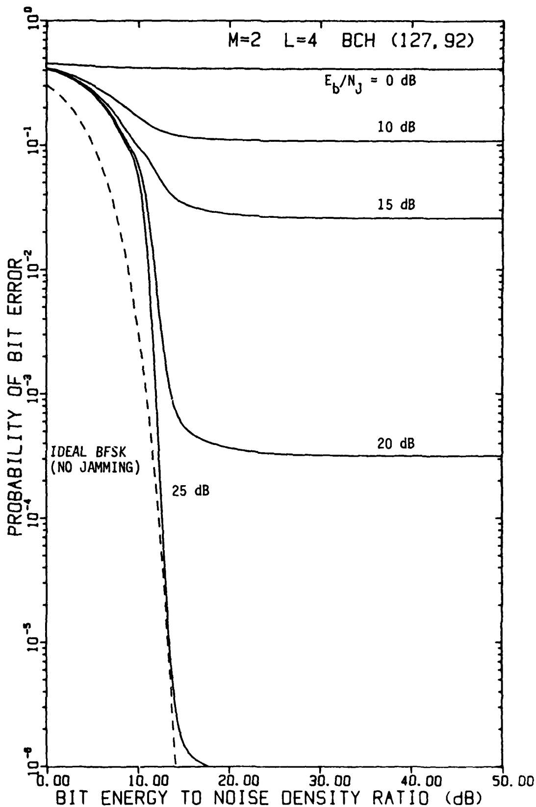
FIGURE 4-24 PERFORMANCE OF FH/BFSK WITH BCH (127,92) CODE AND L=4 HOPS/DIGIT AS A FUNCTION OF E_b/N_0 WITH E_b/N_j AS A PARAMETER, USING A LINEAR COMBINING DEMODULATOR, IN OPTIMUM PARTIAL-BAND NOISE JAMMING
