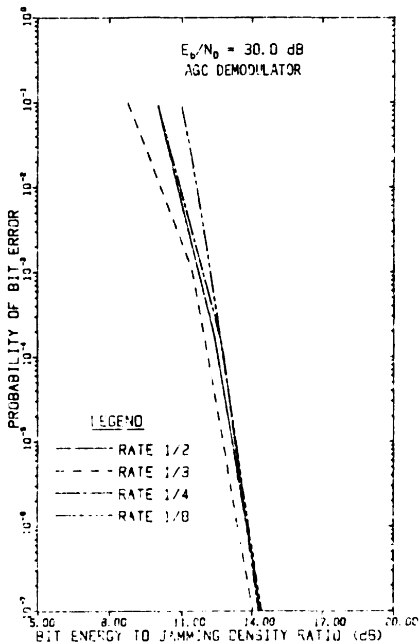
FIGURE 4-112 PERFORMANCE OF CONSTRAINT-LENGTH-7 CONVOLUTIONAL CODES USING FH/BFSK WITH OPTIMUM DIVERSITY IN WORST-CASE PARTIAL-BAND NOISE JAMMING AS A FUNCTION OF E_b/N_0 WHEN E_b/N_0 = 30 \text{ dB}
