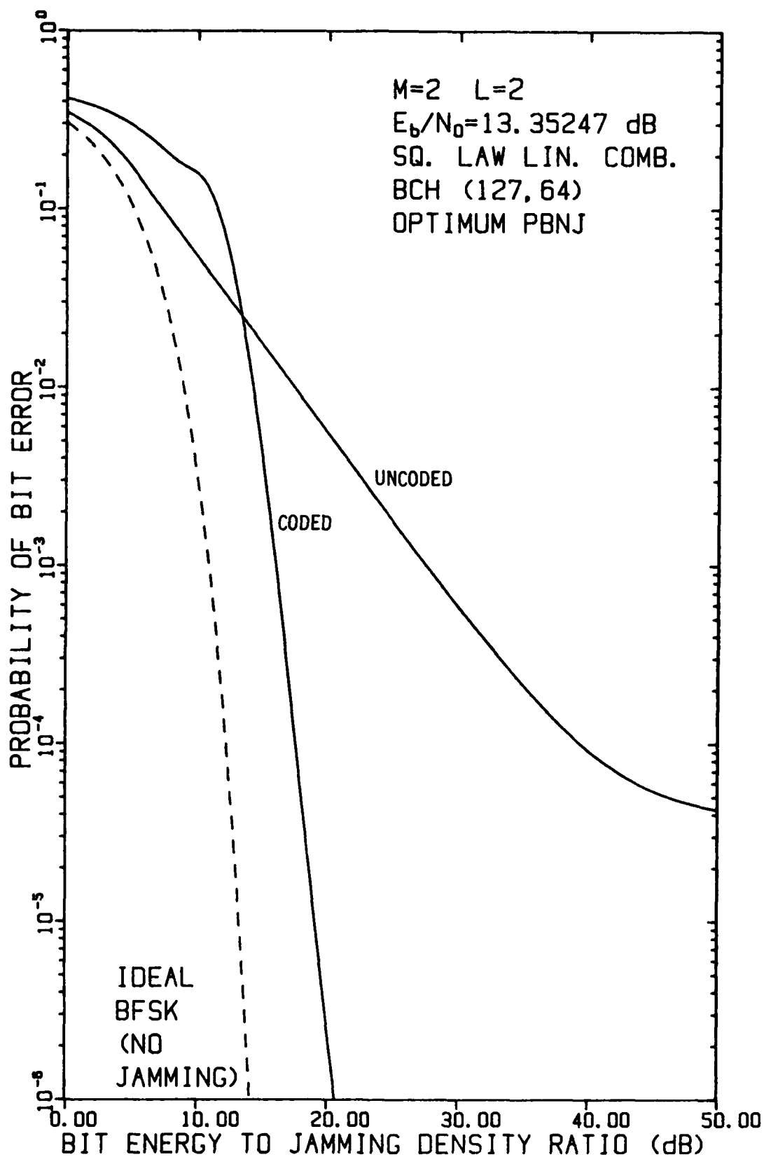
FIGURE 4-34 PERFORMANCE OF FH/BFSK WITH BCH (127,64) CODE AND L=2 HOPS/DIGIT AS A FUNCTION OF E_b/N_j WHEN E_b/N_0 = 13.35247 dB, USING A LINEAR COMBINING DEMODULATOR, IN OPTIMUM PARTIAL-BAND NOISE JAMMING
