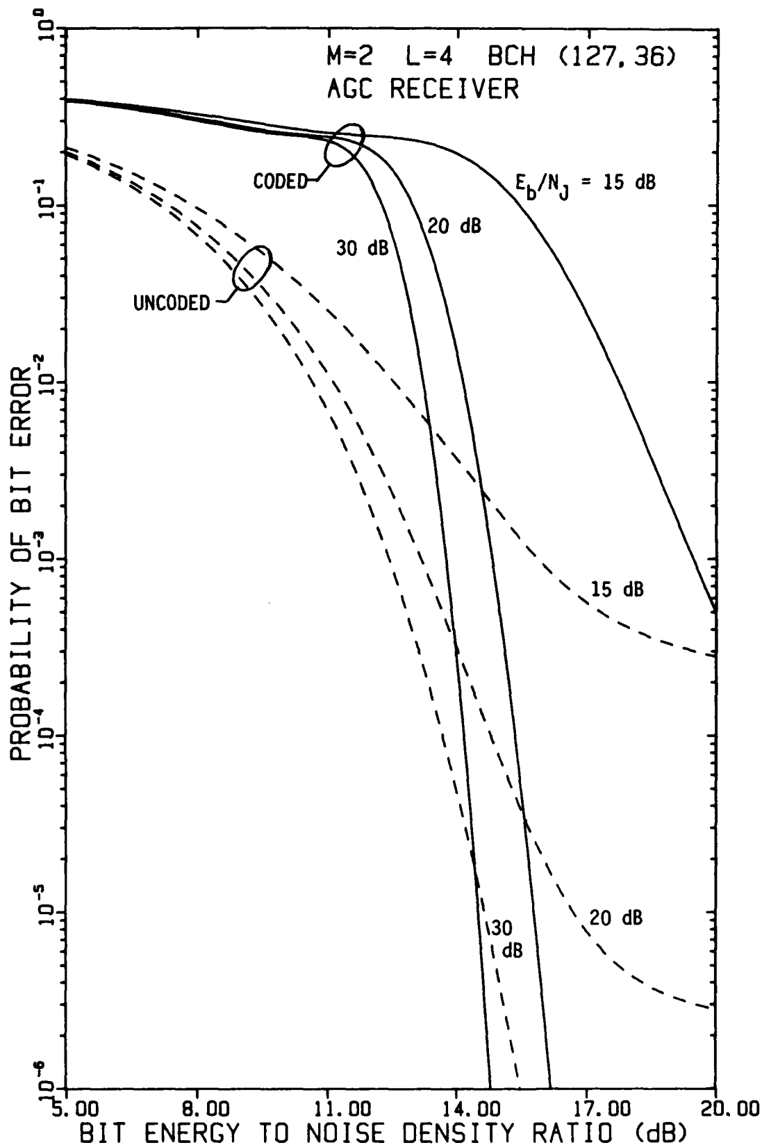
FIGURE 4-89 PERFORMANCE OF FH/BFSK WITH BCH (127,36) CODE AND L=4 HOPS/DIGIT AS A FUNCTION OF E_b/N_0 WITH E_b/N_J AS A PARAMETER, USING AN AGC DEMODULATOR, IN OPTIMUM PARTIAL-BAND NOISE JAMMING
