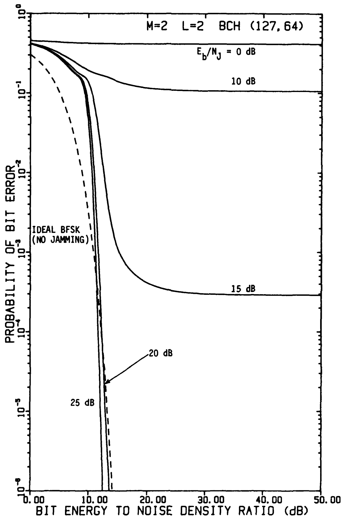
FIGURE 4-30 PERFORMANCE OF FH/BFSK WITH BCH (127,64) CODE AND L=2 HOPS/DIGIT AS A FUNCTION OF E_b/N_0 WITH E_b/N_J AS A PARAMETER, USING A LINEAR COMBINING DEMODULATOR, IN OPTIMUM PARTIAL-BAND NOISE JAMMING
