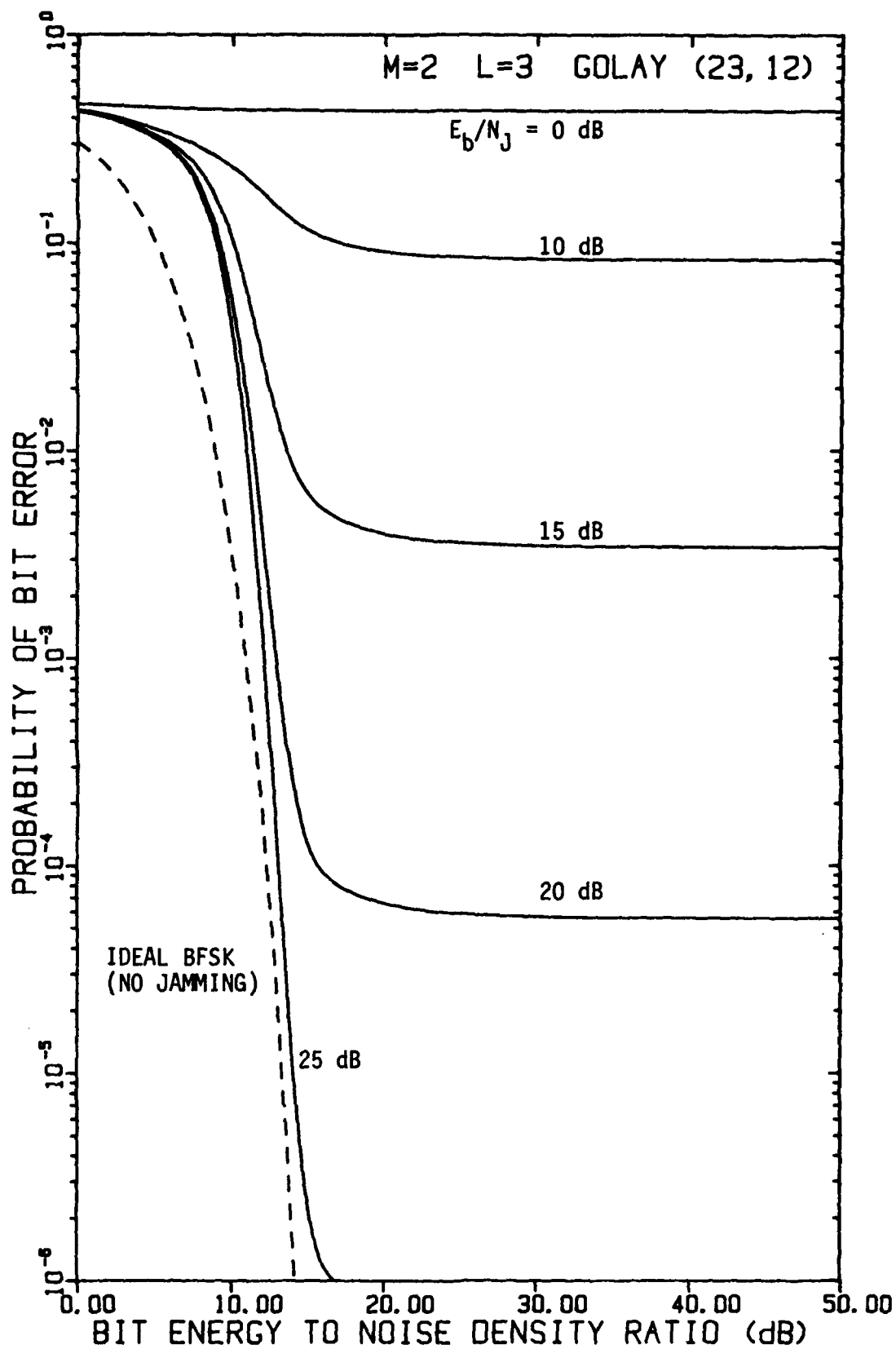
FIGURE 4-15 PERFORMANCE OF FH/BFSK WITH GOLAY (23,12) CODE AND L=3 HOPS/DIGIT AS A FUNCTION OF E_b/N_0 WITH E_b/N_j AS A PARAMETER, USING A LINEAR COMBINING DEMODULATOR, IN OPTIMUM PARTIAL-BAND NOISE JAMMING
