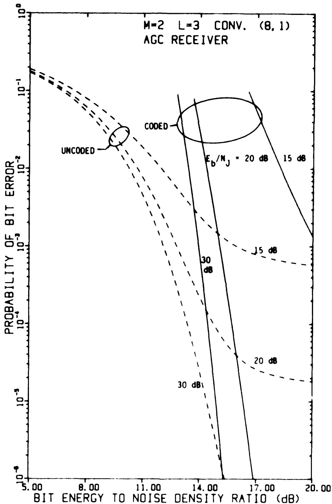
FIGURE 4-108 PERFORMANCE OF FH/BFSK WITH CONVOLUTIONAL RATE-1/8 CODE AND L=3 HOPS/DIGIT AS A FUNCTION OF E_b/N_0 WITH E_b/N_J AS A PARAMETER, USING AN AGC DEMODULATOR, IN OPTIMUM PARTIAL-BAND NOISE JAMMING
