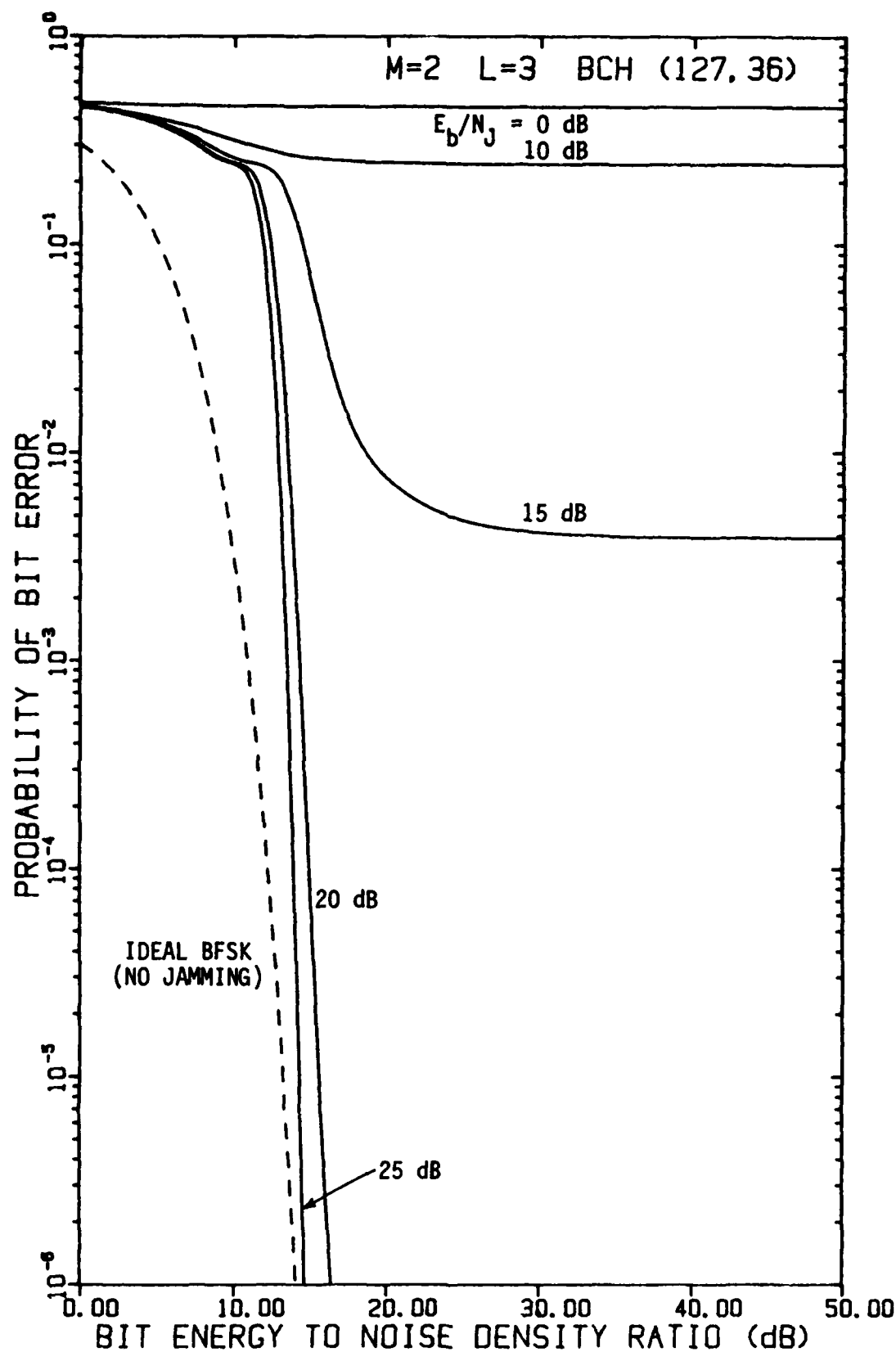
FIGURE 4-39 PERFORMANCE OF FH/BFSK WITH BCH (127,36) CODE AND L=3 HOPS/DIGIT AS A FUNCTION OF E_b/N_0 WITH E_b/N_J AS A PARAMETER, USING A LINEAR COMBINING DEMODULATOR, IN OPTIMUM PARTIAL-BAND NOISE JAMMING
