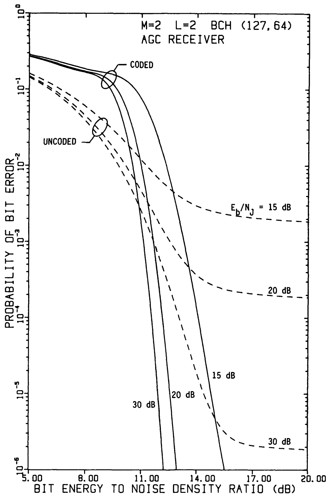
FIGURE 4-83 PERFORMANCE OF FH/BFSK WITH BCH (127,64) CODE AND L=2 HOPS/DIGIT AS A FUNCTION OF E_b/N_0 WITH E_b/N_j AS A PARAMETER, USING AN AGC DEMODULATOR, IN OPTIMUM PARTIAL-BAND NOISE JAMMING
