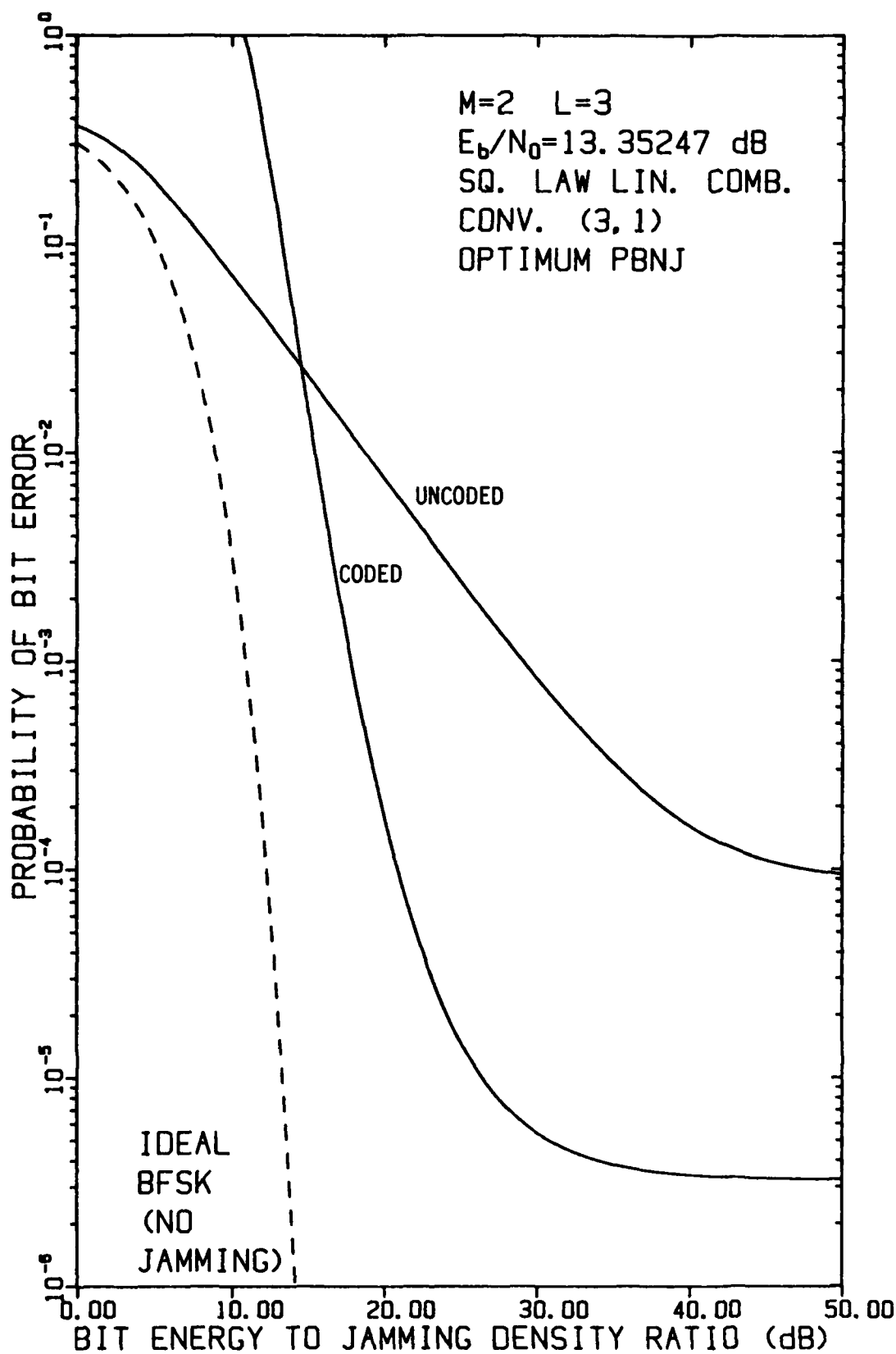
FIGURE 4-55 PERFORMANCE OF FH/BFSK WITH CONVOLUTIONAL RATE-1/3 CODE AND L=3 HOPS/DIGIT AS A FUNCTION OF E_b/N_j WHEN E_b/N_0 = 13.35247 dB, USING A LINEAR COMBINING DEMODULATOR, IN OPTIMUM PARTIAL-BAND NOISE JAMMING
