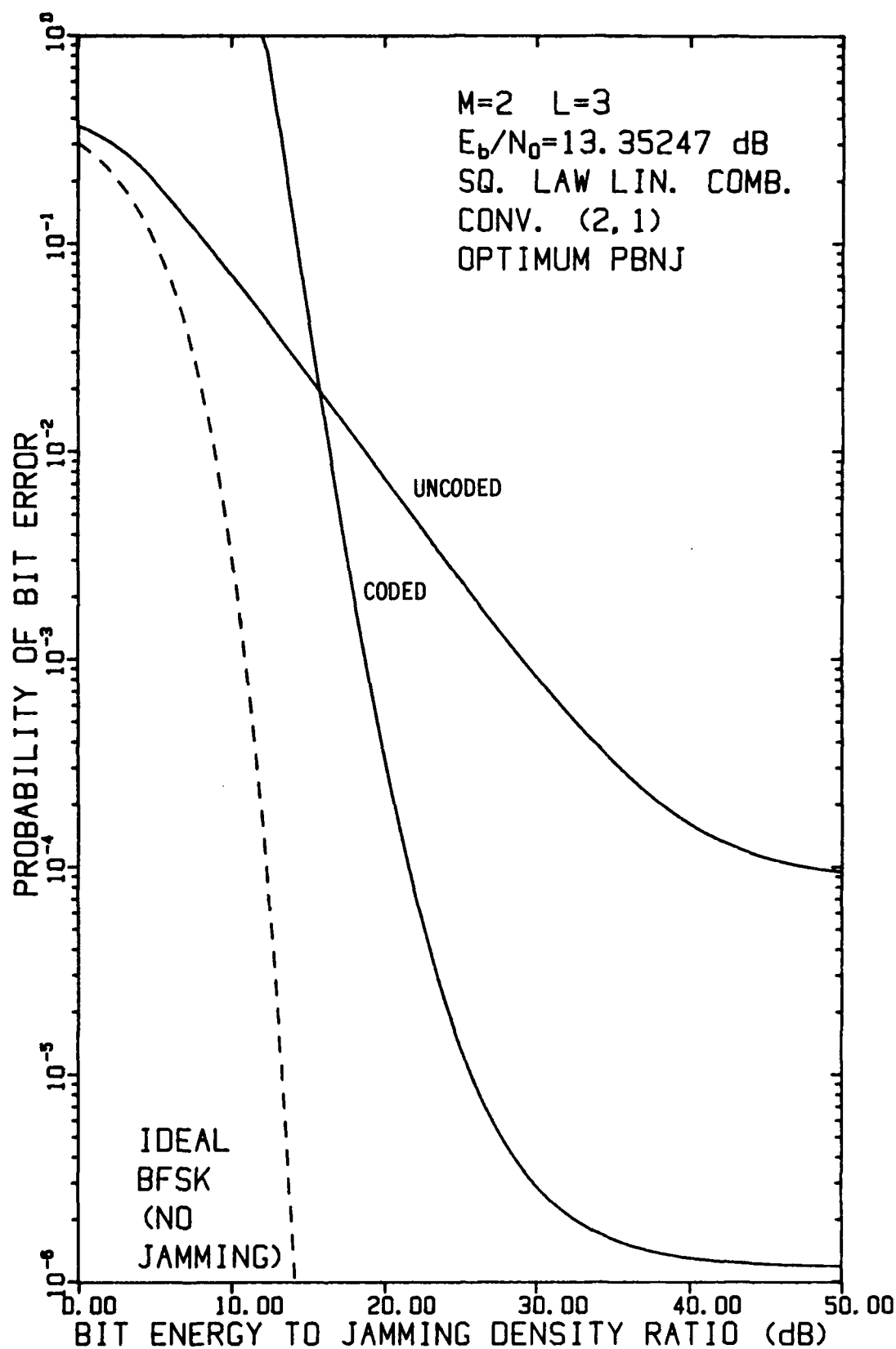
FIGURE 4-51 PERFORMANCE OF FH/BFSK WITH CONVOLUTIONAL RATE-1/2 CODE AND L=3 HOPS/DIGIT AS A FUNCTION OF E_b/N_j WHEN E_b/N_0 = 13.35247 dB, USING A LINEAR COMBINING DEMODULATOR, IN OPTIMUM PARTIAL-BAND NOISE JAMMING
