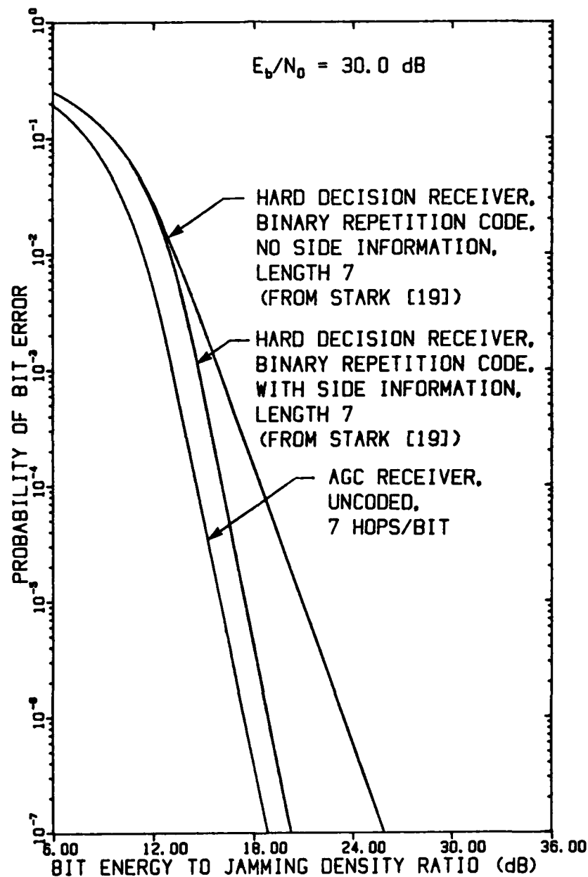
FIGURE 4-69 COMPARISON OF PERFORMANCE OF FH/BFSK AGC RECEIVER WITH L=7 DIVERSITY AND PERFORMANCE OF HARD DECISION RECEIVERS WITH LENGTH-7 BINARY REPETITION CODES
