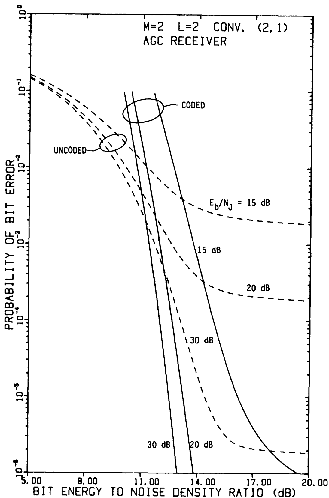
FIGURE 4-95 PERFORMANCE OF FH/BFSK WITH CONVOLUTIONAL RATE-1/2 CODE AND L=2 HOPS/DIGIT AS A FUNCTION OF E_b/N_0 WITH E_b/N_J AS A PARAMETER, USING AN AGC DEMODULATOR, IN OPTIMUM PARTIAL-BAND NOISE JAMMING
