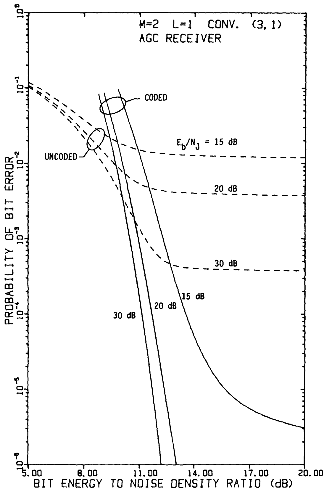
FIGURE 4-98 PERFORMANCE OF FH/BFSK WITH CONVOLUTIONAL RATE-1/3 CODE AND L=1 HOP/DIGIT AS A FUNCTION OF E_b/N_0 WITH E_b/N_j AS A PARAMETER, USING AN AGC DEMODULATOR, IN OPTIMUM PARTIAL-BAND NOISE JAMMING
