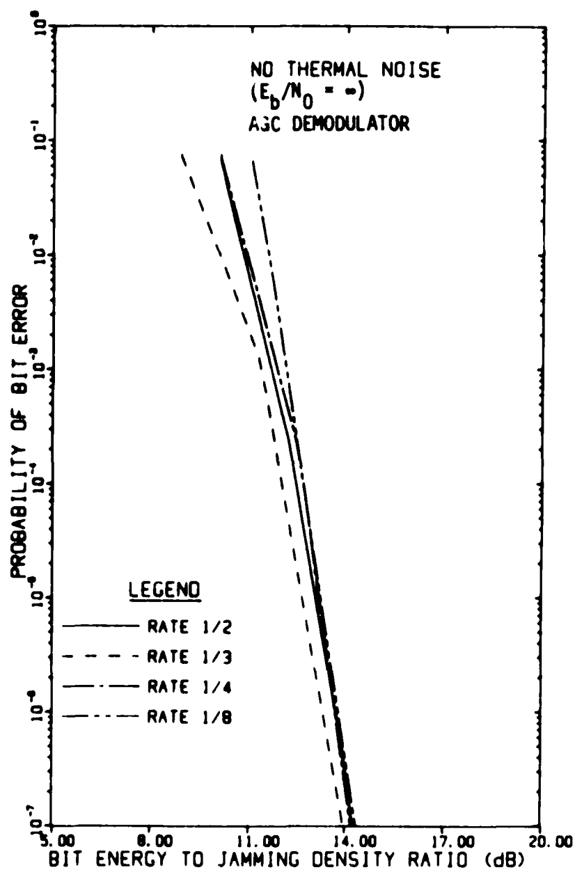
FIGURE 4-113 PERFORMANCE OF CONSTRAINT-LENGTH-7 CONVOLUTIONAL CODES USING FH/BFSK WITH OPTIMUM DIVERSITY IN WORST-CASE PARTIAL-BAND NOISE JAMMING AS A FUNCTION OF E_b/N_j WHEN E_b/N_0 = \infty
