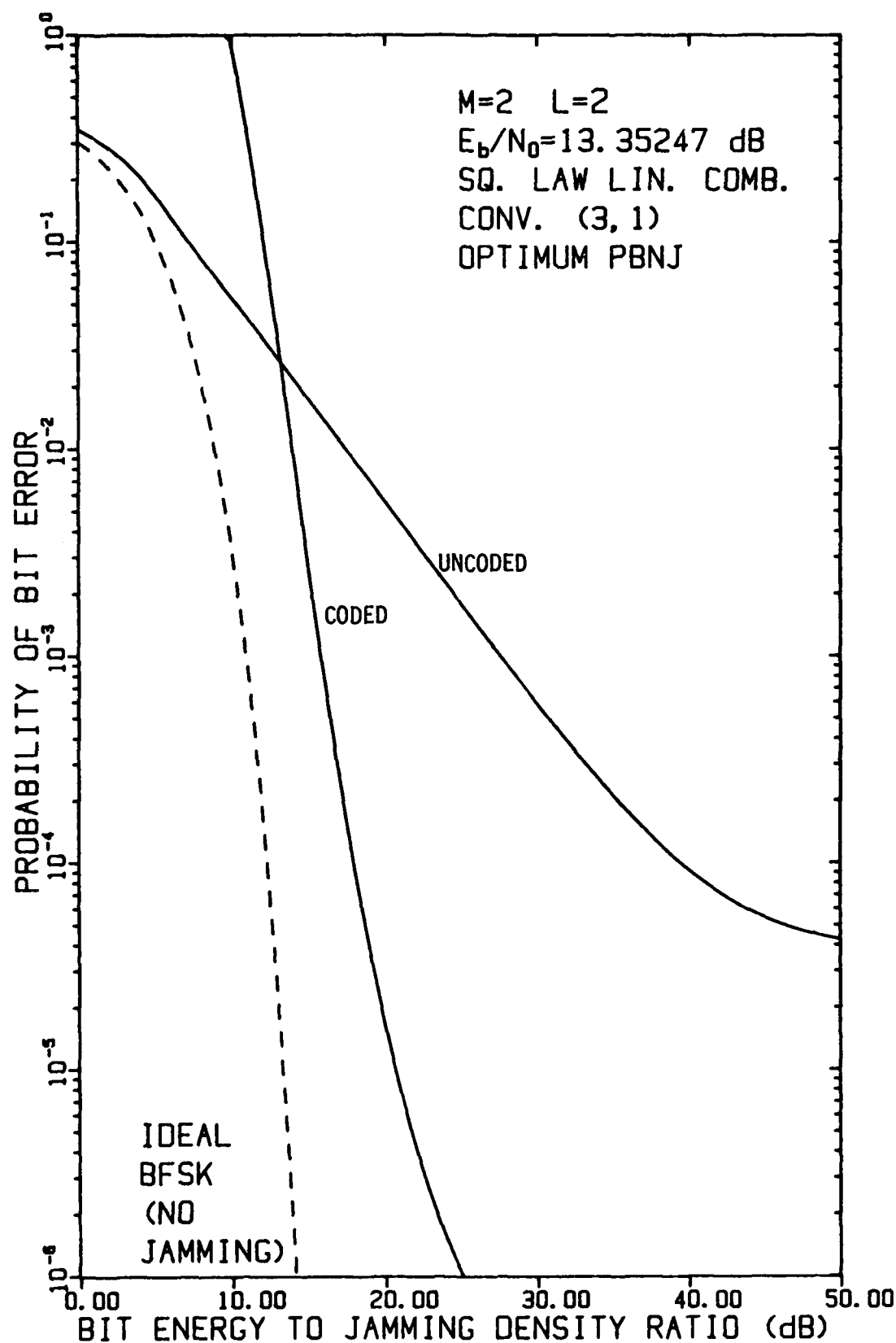
FIGURE 4-54 PERFORMANCE OF FH/BFSK WITH CONVOLUTIONAL RATE-1/3 CODE AND L=2 HOPS/DIGIT AS A FUNCTION OF E_b/N_j WHEN E_b/N_0 = 13.35247 dB, USING A LINEAR COMBINING DEMODULATOR, IN OPTIMUM PARTIAL-BAND NOISE JAMMING
