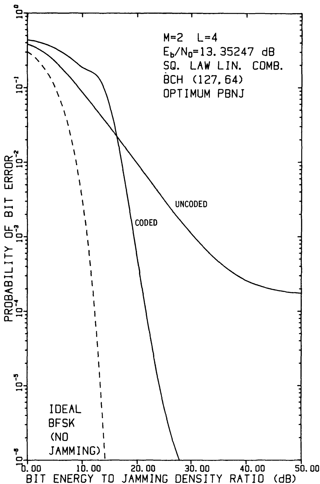
FIGURE 4-36 PERFORMANCE OF FH/BFSK WITH BCH (127,64) CODE AND L=4 HOPS/DIGIT AS A FUNCTION OF E_b/N_j WHEN E_b/N_0 = 13.35247 dB, USING A LINEAR COMBINING DEMODULATOR, IN OPTIMUM PARTIAL-BAND NOISE JAMMING
