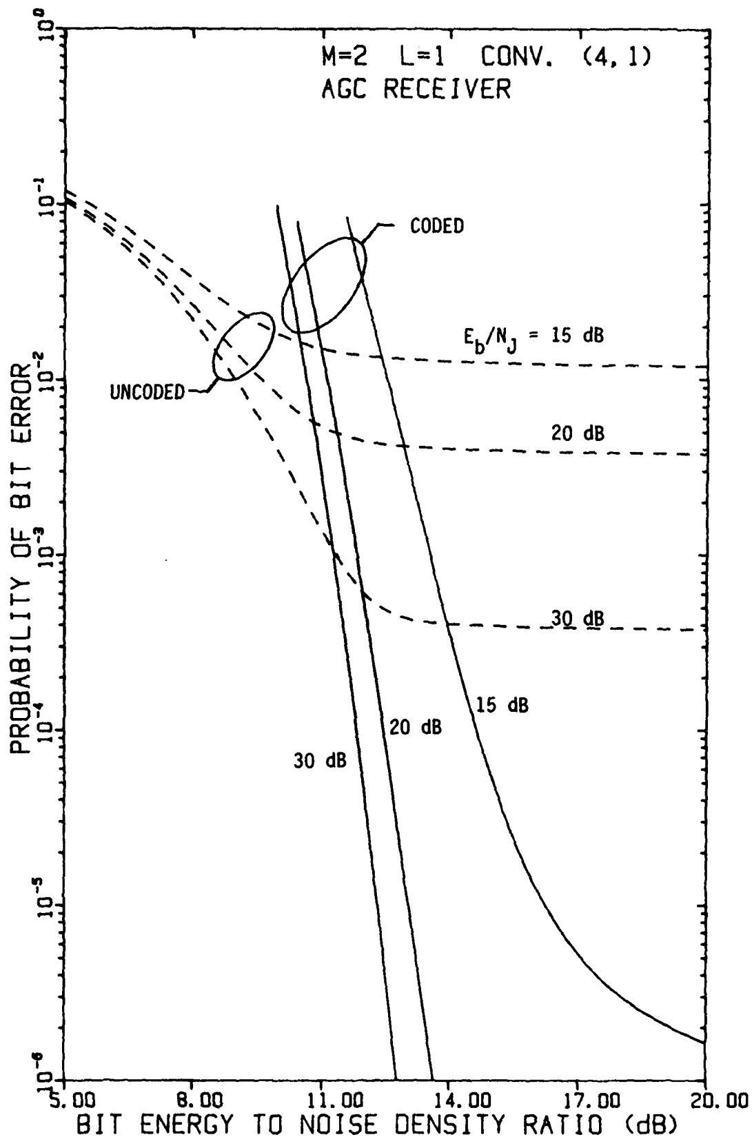
FIGURE 4-102 PERFORMANCE OF FH/BFSK WITH CONVOLUTIONAL RATE-1/4 CODE AND L=1 HOP/DIGIT AS A FUNCTION OF E_b/N_0 WITH E_b/N_J AS A PARAMETER, USING AN AGC DEMODULATOR, IN OPTIMUM PARTIAL-BAND NOISE JAMMING
