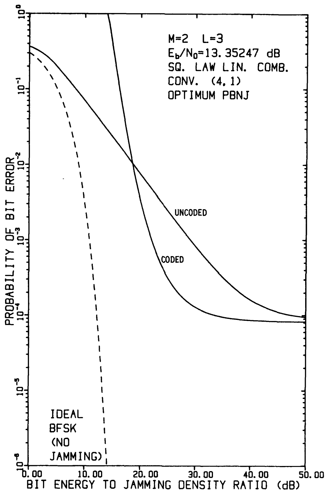
FIGURE 4-59 PERFORMANCE OF FH/BFSK WITH CONVOLUTIONAL RATE-1/4 CODE AND L=3 HOPS/DIGIT AS A FUNCTION OF E_b/N_j WITH E_b/N_0 = 13.35247 dB, USING A LINEAR COMBINING DEMODULATOR, IN OPTIMUM PARTIAL-BAND NOISE JAMMING
