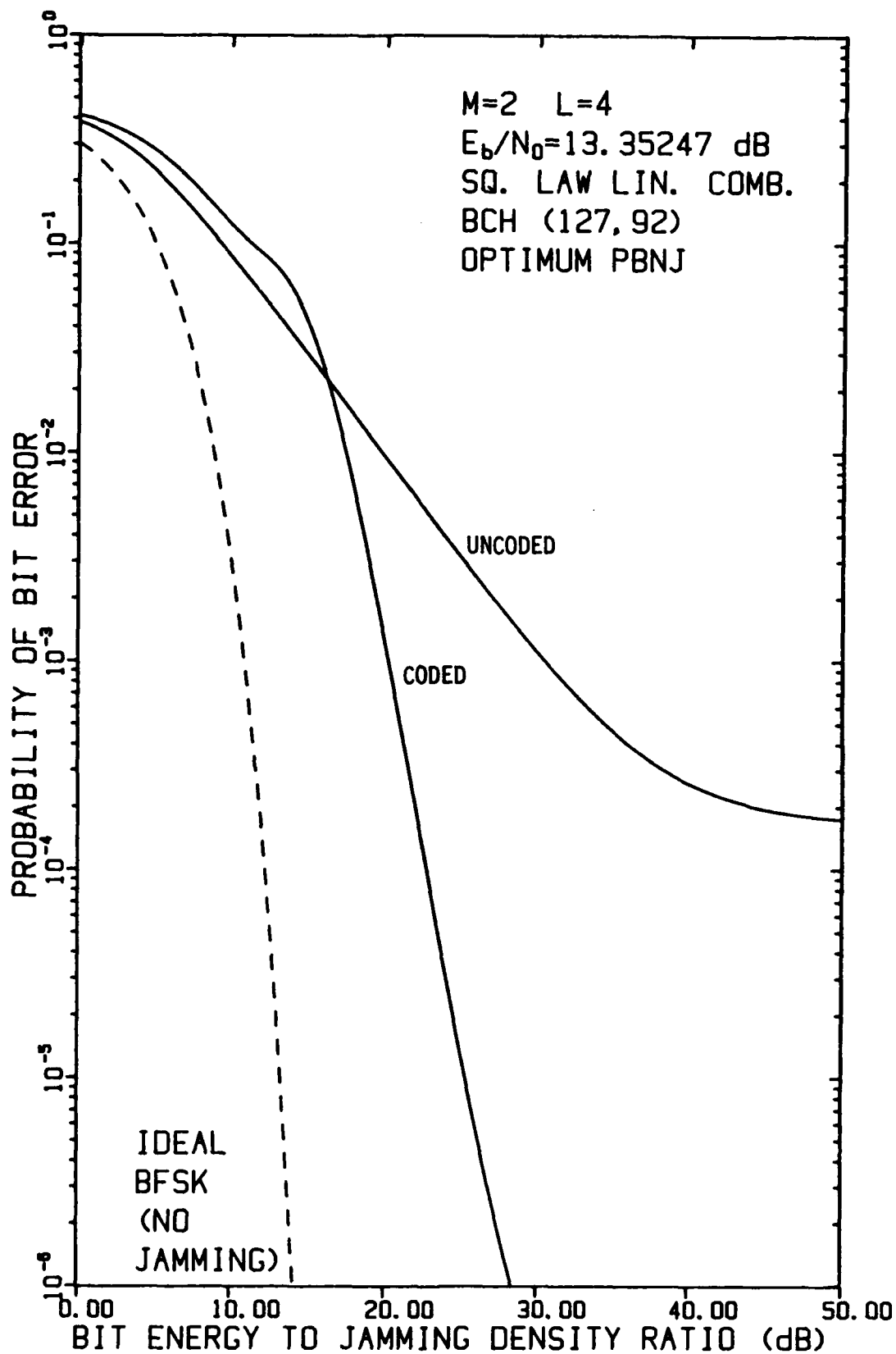
FIGURE 4-28 PERFORMANCE OF FH/BFSK WITH BCH (127,92) CODE AND L=4 HOPS/DIGIT AS A FUNCTION OF E_b/N_j WHEN E_b/N_0 = 13.35247 dB, USING A LINEAR COMBINING DEMODULATOR, IN OPTIMUM PARTIAL-BAND NOISE JAMMING
