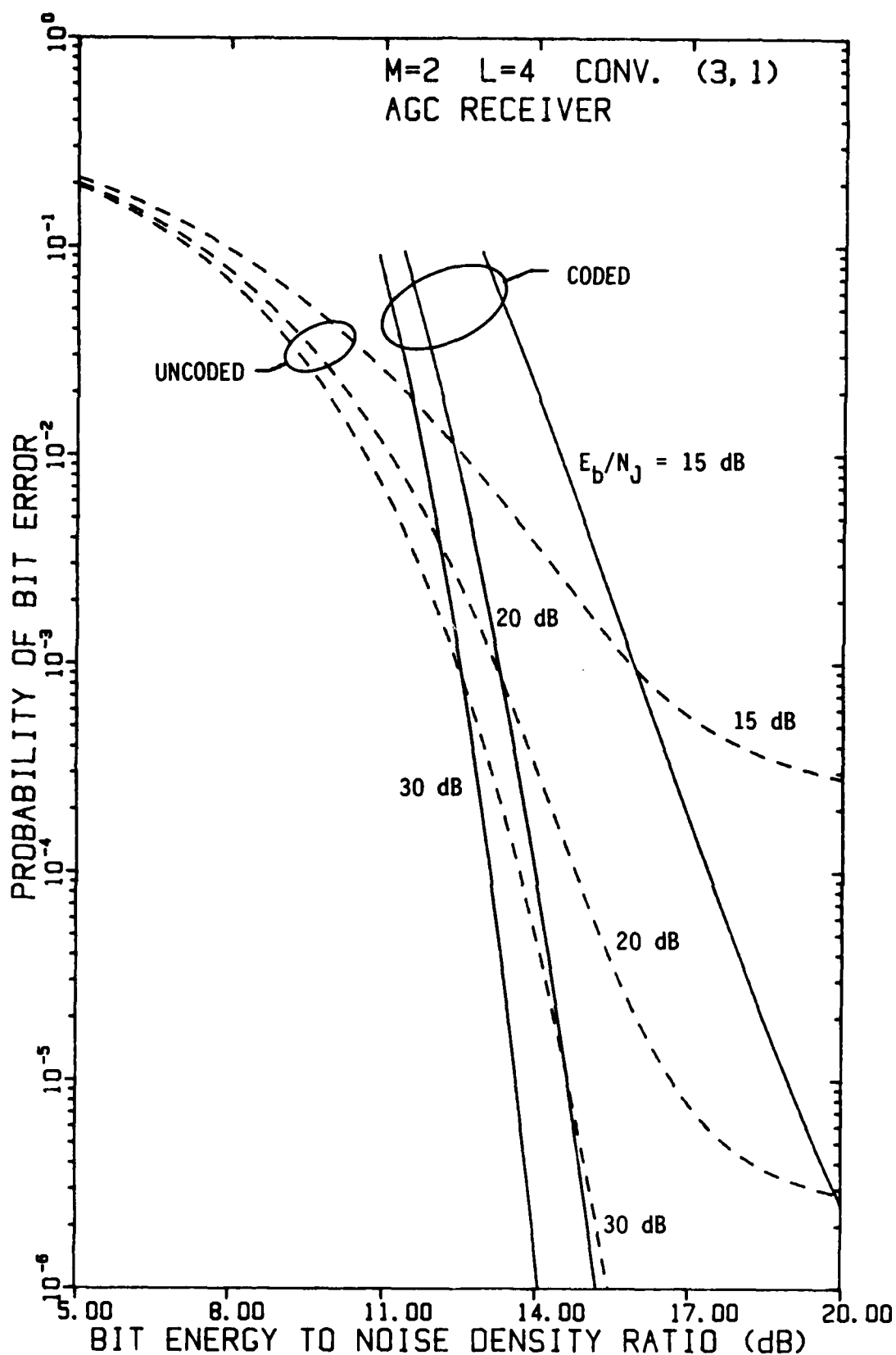
FIGURE 4-101 PERFORMANCE OF FH/BFSK WITH CONVOLUTIONAL RATE-1/3 CODE AND L=4 HOPS/DIGIT AS A FUNCTION OF E_b/N_0 WITH E_b/N_J AS A PARAMETER, USING AN AGC DEMODULATOR, IN OPTIMUM PARTIAL-BAND NOISE JAMMING
