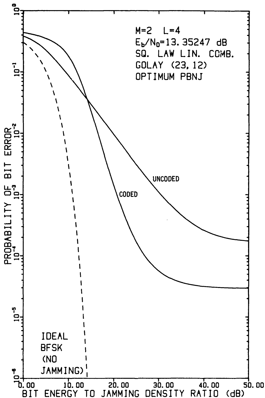
FIGURE 4-20 PERFORMANCE OF FH/BFSK WITH GOLAY (23,12) CODE AND L=4 HOPS/DIGIT AS A FUNCTION OF E_b/N_j WHEN E_b/N_0 = 13.35247 dB, USING A LINEAR COMBINING DEMODULATOR, IN OPTIMUM PARTIAL-BAND NOISE JAMMING
