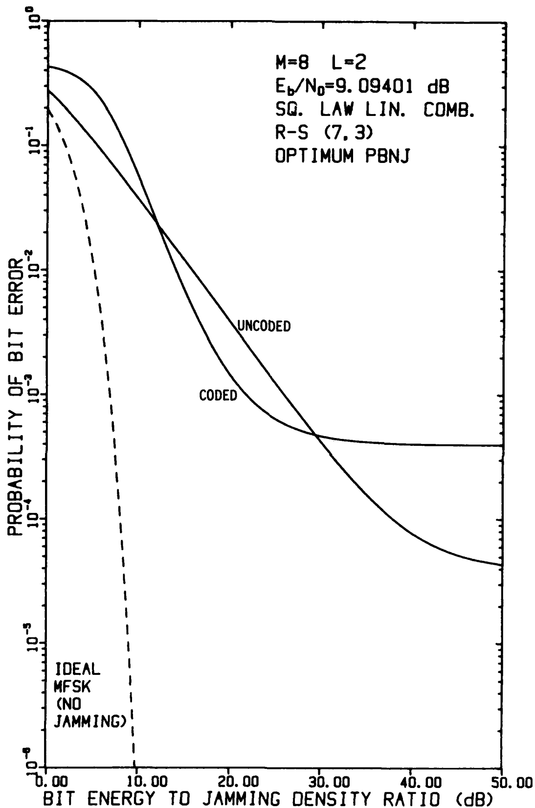
FIGURE 4-66 PERFORMANCE OF FH/MFSK WITH REED-SOLOMON (7,3) CODE AND L=2 HOPS/DIGIT AS A FUNCTION OF E_b/N_j WHEN E_b/N_0 = 9.09401 dB, USING A LINEAR COMBINING DEMODULATOR, IN OPTIMUM PARTIAL-BAND NOISE JAMMING
