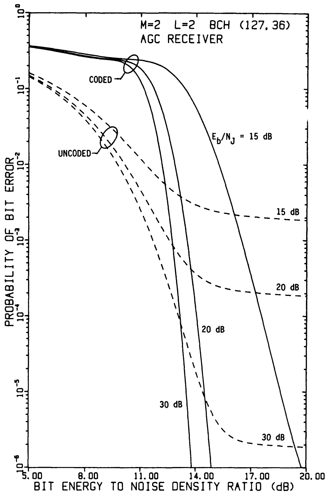
FIGURE 4-87 PERFORMANCE OF FH/BFSK WITH BCH (127,36) CODE AND L=2 HOPS/DIGIT AS A FUNCTION OF E_b/N_0 WITH E_b/N_J AS A PARAMETER, USING AN AGC DEMODULATOR, IN OPTIMUM PARTIAL-BAND NOISE JAMMING
