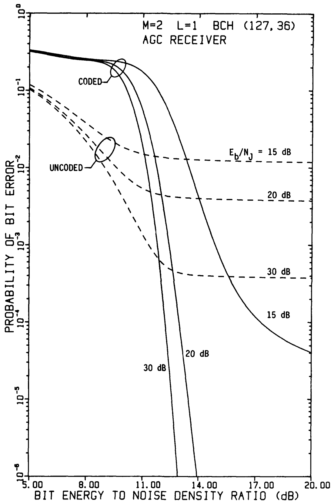
FIGURE 4-86 PERFORMANCE OF FH/BFSK WITH BCH (127,36) CODE AND L=1 HOP/DIGIT AS A FUNCTION OF E_b/N_0 WITH E_b/N_j AS A PARAMETER, USING AN AGC DEMODULATOR, IN OPTIMUM PARTIAL-BAND NOISE JAMMING
