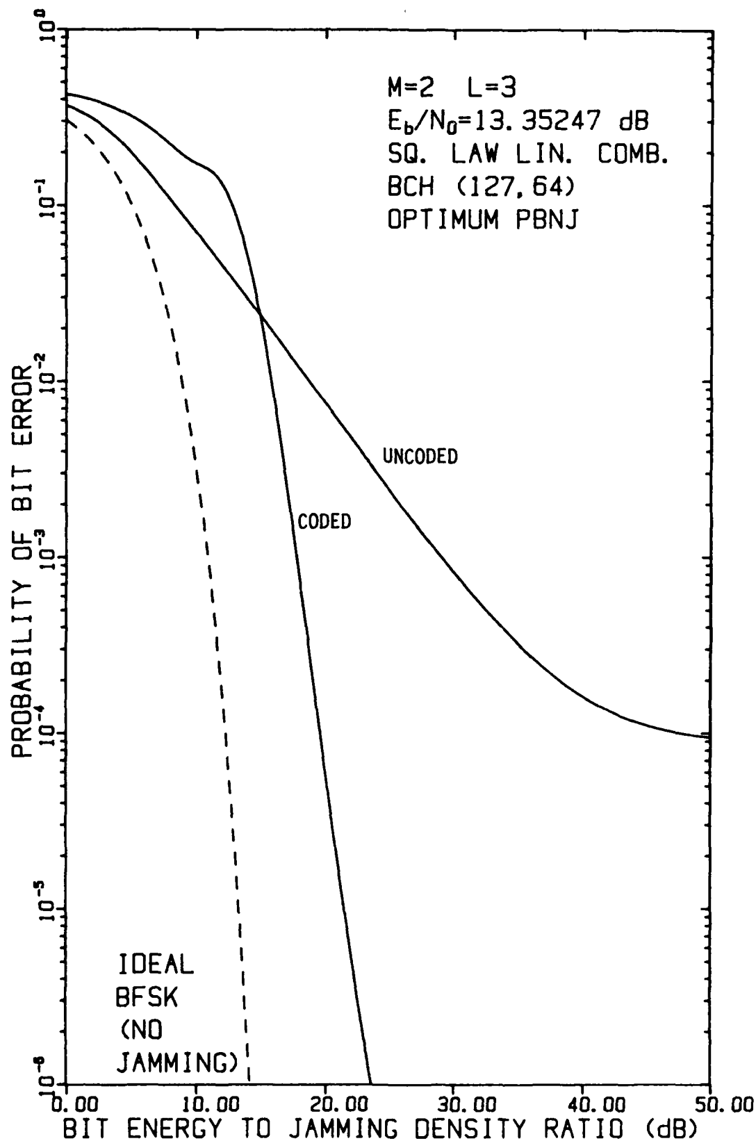
FIGURE 4-35 PERFORMANCE OF FH/BFSK WITH BCH (127,64) CODE AND L=3 HOPS/DIGIT AS A FUNCTION OF E_b/N_j WHEN E_b/N_0 = 13.35247 dB, USING A LINEAR COMBINING DEMODULATOR, IN OPTIMUM PARTIAL-BAND NOISE JAMMING
