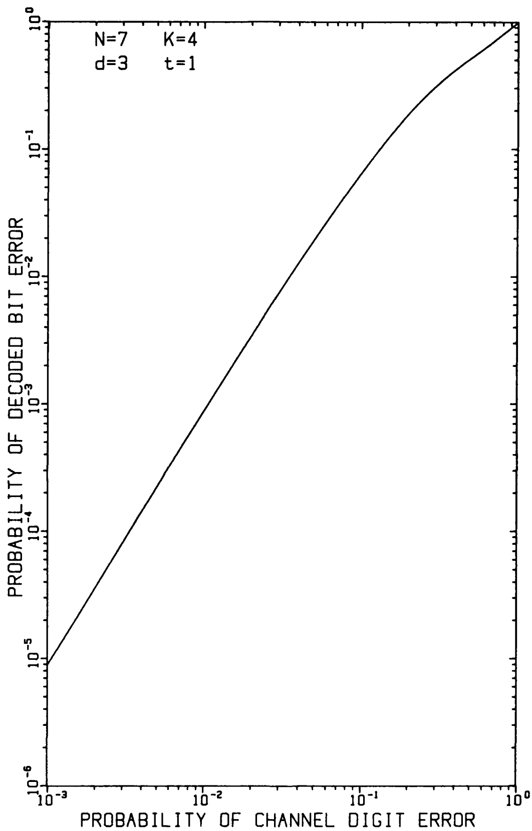
FIGURE 3-1 DECODER PERFORMANCE FOR HAMMING (7,4) CODE
