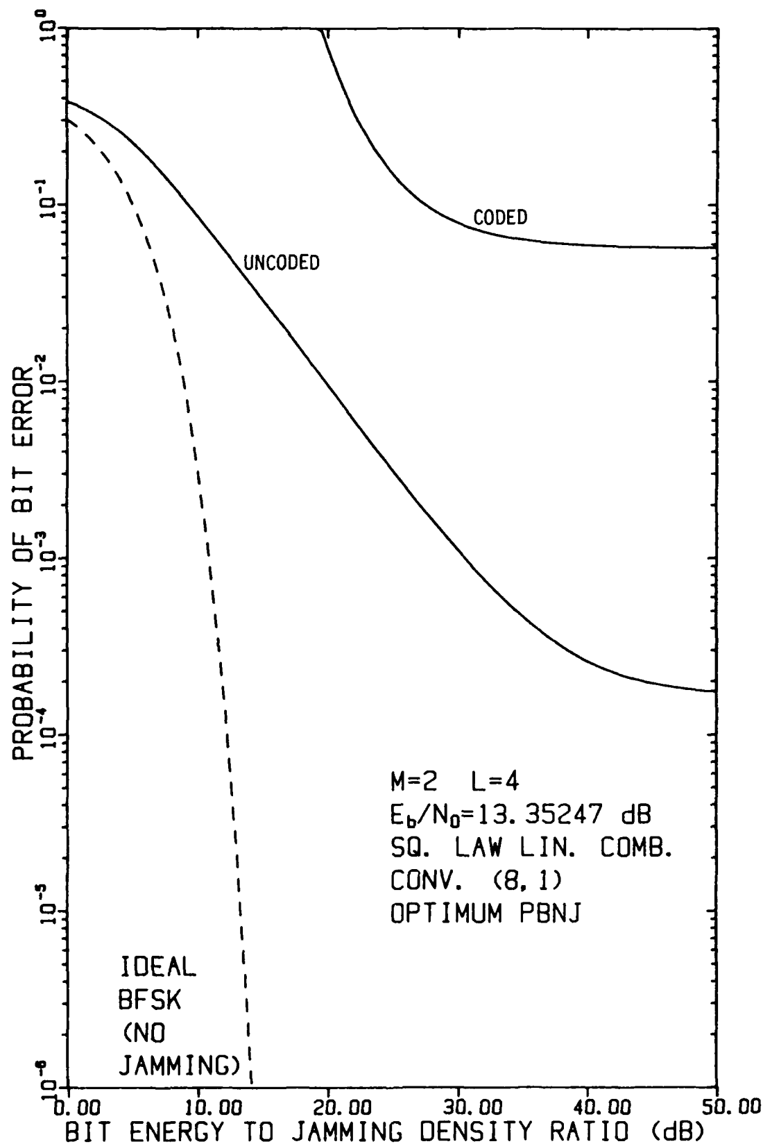
FIGURE 4-64 PERFORMANCE OF FH/BFSK WITH CONVOLUTIONAL RATE-1/8 CODE AND L=4 HOPS/DIGIT AS A FUNCTION OF E_b/N_J WHEN E_b/N_0 = 13.35247 dB, USING A LINEAR COMBINING DEMODULATOR, IN OPTIMUM PARTIAL-BAND NOISE JAMMING
