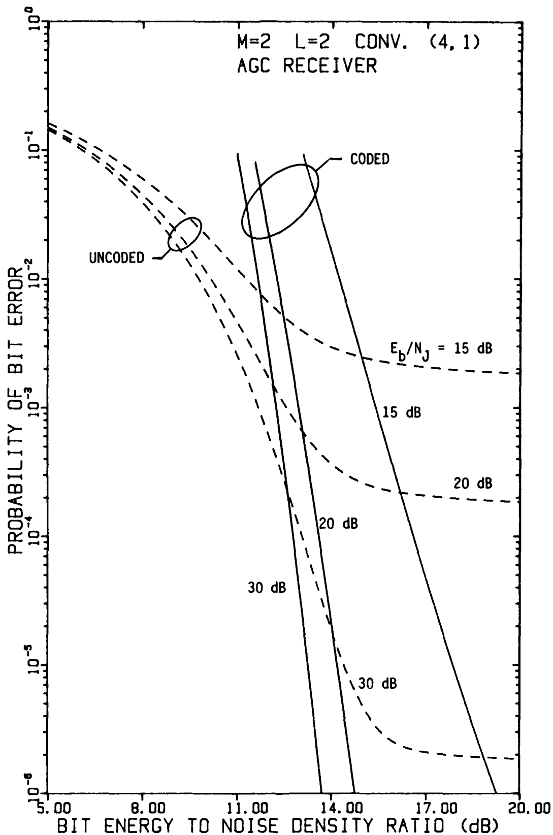
FIGURE 4-103 PERFORMANCE OF FH/BFSK WITH CONVOLUTIONAL RATE-1/4 CODE AND L=2 HOPS/DIGIT AS A FUNCTION OF E_b/N_0 WITH E_b/N_J AS A PARAMETER, USING AN AGC DEMODULATOR, IN OPTIMUM PARTIAL-BAND NOISE JAMMING
