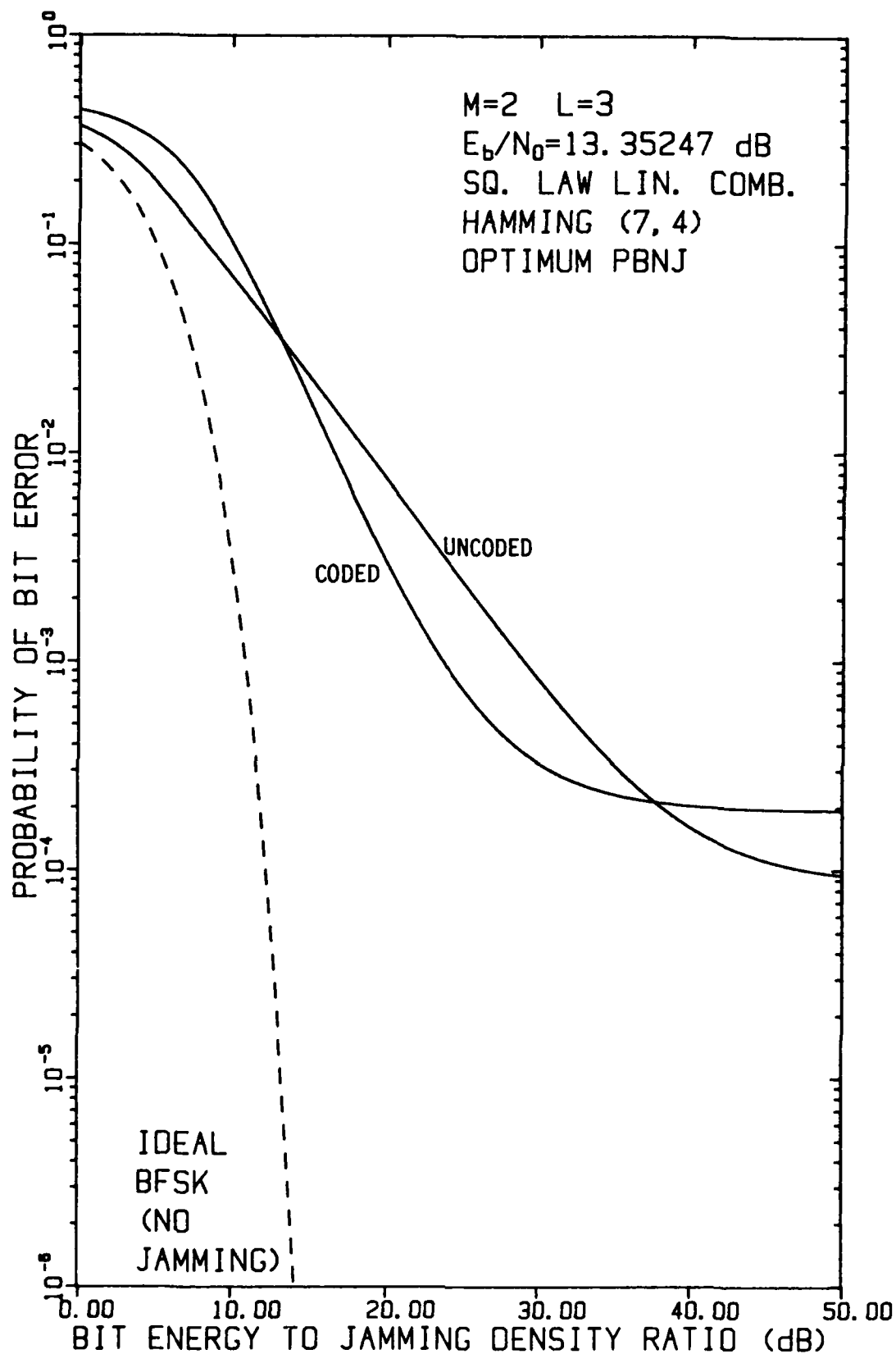
FIGURE 4-11 PERFORMANCE OF FH/BFSK WITH HAMMING (7,4) CODE AND L=3 HOPS/DIGIT AS A FUNCTION OF E_b/N_j WHEN E_b/N_0 = 13.35247 dB, USING A LINEAR COMBINING DEMODULATOR, IN OPTIMUM PARTIAL-BAND NOISE JAMMING
