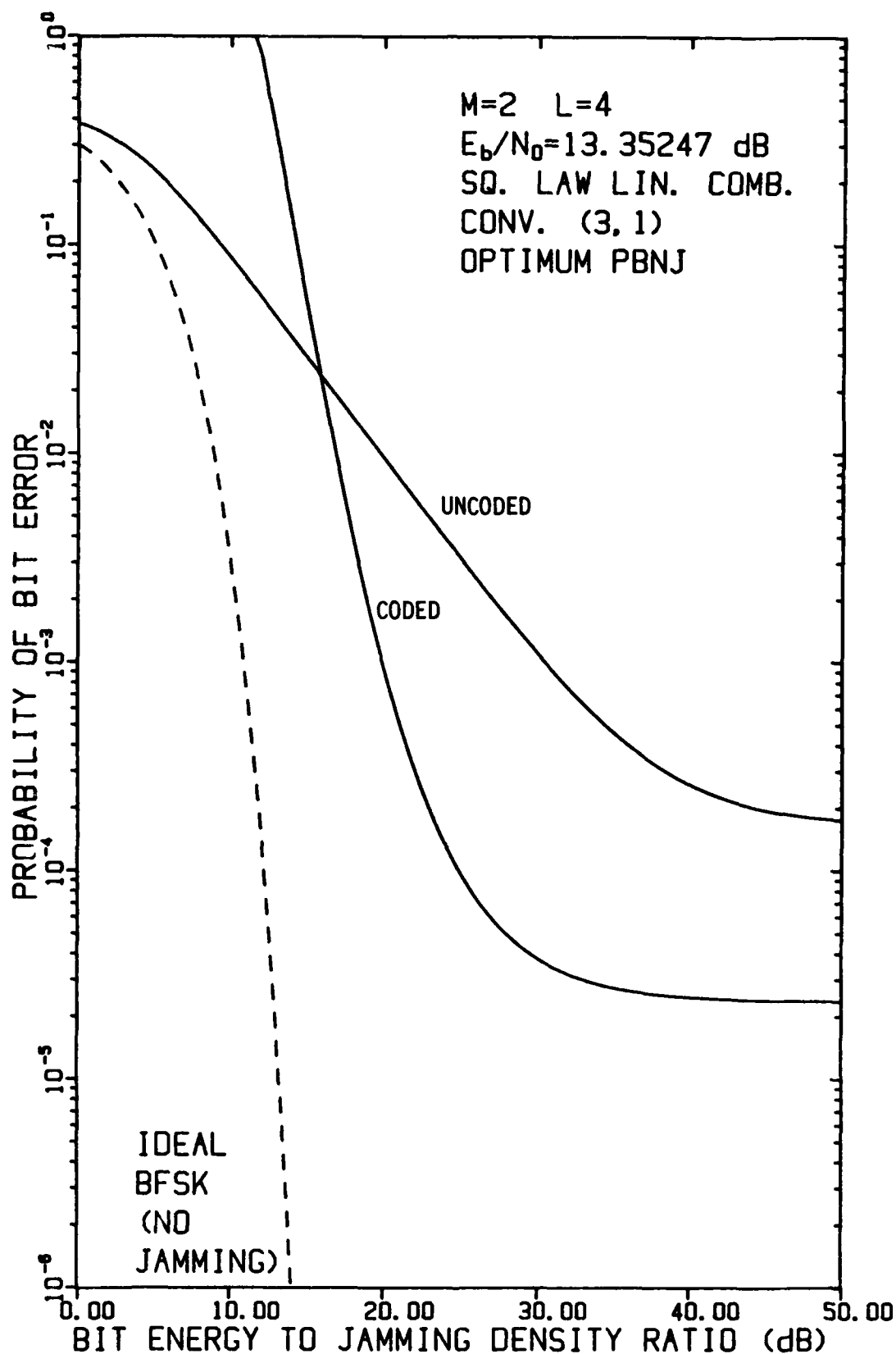
FIGURE 4-56 PERFORMANCE OF FH/BFSK WITH CONVOLUTIONAL RATE-1/3 CODE AND L=4 HOPS/DIGIT AS A FUNCTION OF E_b/N_j WHEN E_b/N_0 = 13.35247 dB, USING A LINEAR COMBINING DEMODULATOR, IN OPTIMUM PARTIAL-BAND NOISE JAMMING
