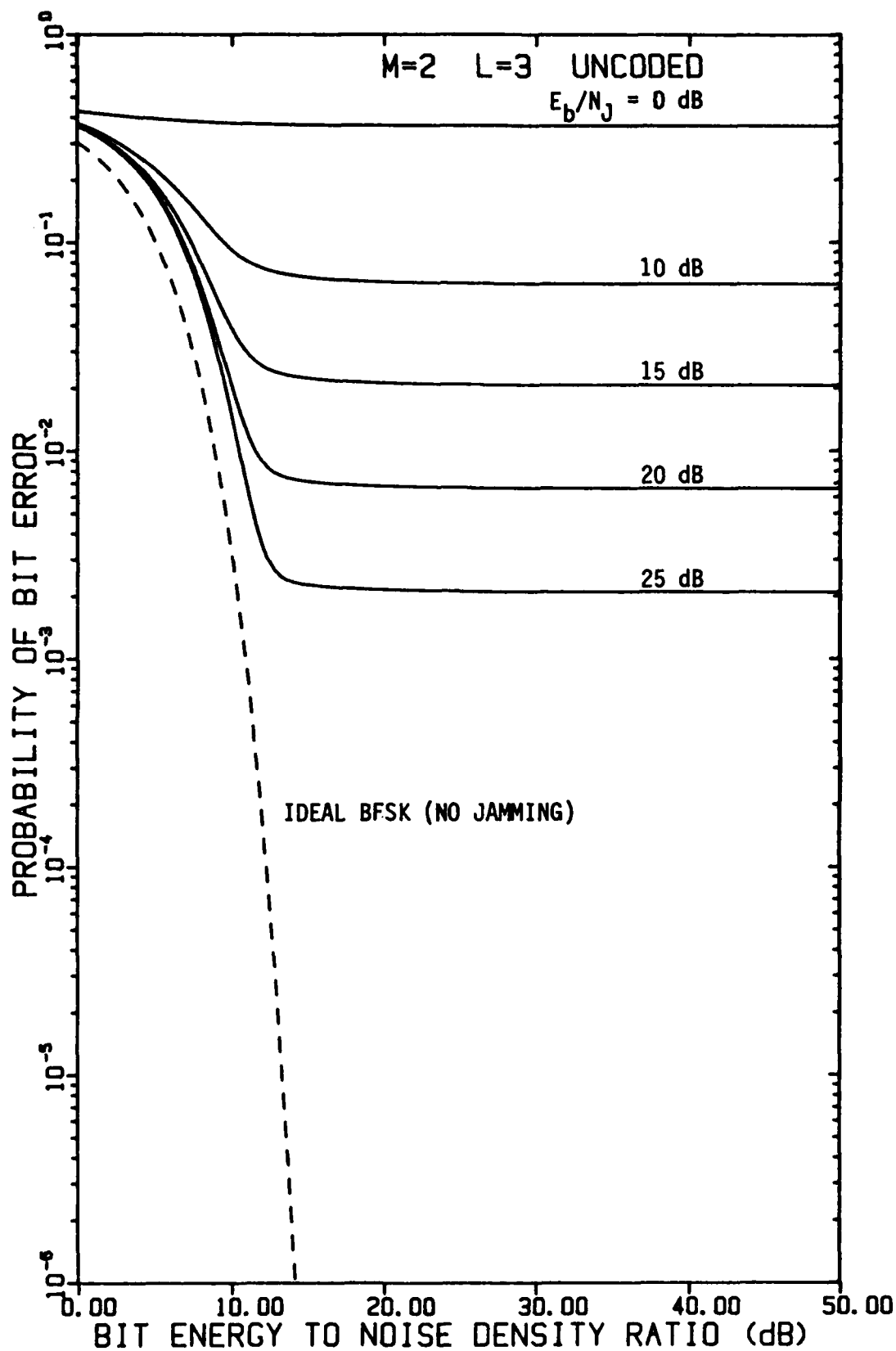
FIGURE 4-3 PERFORMANCE OF UNCODED BFSK WITH L=3 HOPS/BIT AS A FUNCTION OF E_b/N_0 WITH E_b/N_J AS A PARAMETER, USING A LINEAR COMBINING DEMODULATOR, IN OPTIMUM PARTIAL-BAND NOISE JAMMING
