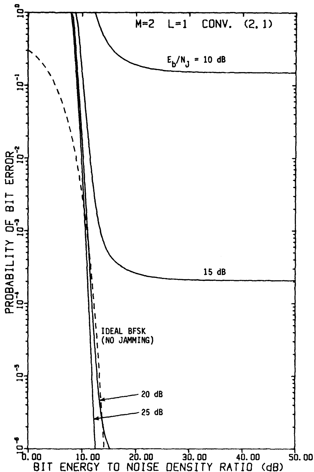
FIGURE 4-45 PERFORMANCE OF FH/BFSK WITH CONVOLUTIONAL RATE-1/2 CODE AND L=1 HOP/DIGIT AS A FUNCTION OF E_b/N_0 WITH E_b/N_J AS A PARAMETER, USING A LINEAR COMBINING DEMODULATOR, IN OPTIMUM PARTIAL-BAND NOISE JAMMING
