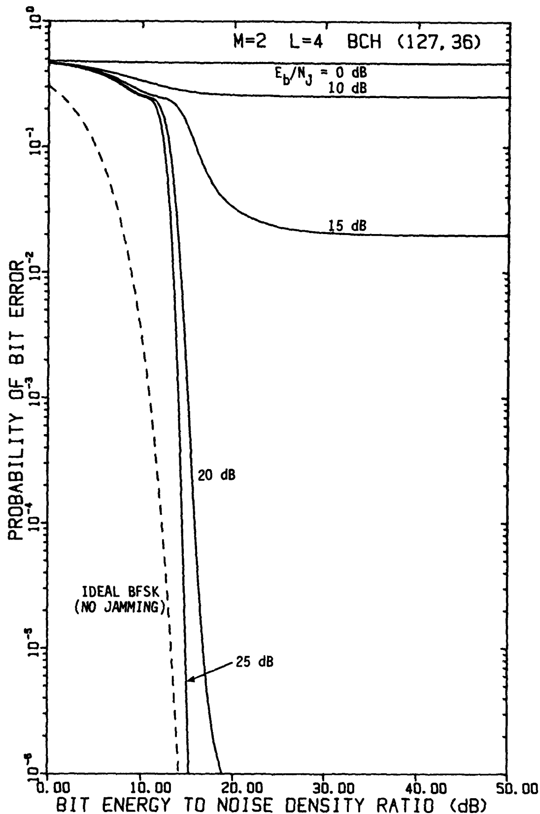
FIGURE 4-40 PERFORMANCE OF FH/BFSK WITH BCH (127,36) CODE AND L=4 HOPS/DIGIT AS A FUNCTION OF E_b/N_0 WITH E_b/N_j AS A PARAMETER, USING A LINEAR COMBINING DEMODULATOR, IN OPTIMUM PARTIAL-BAND NOISE JAMMING
