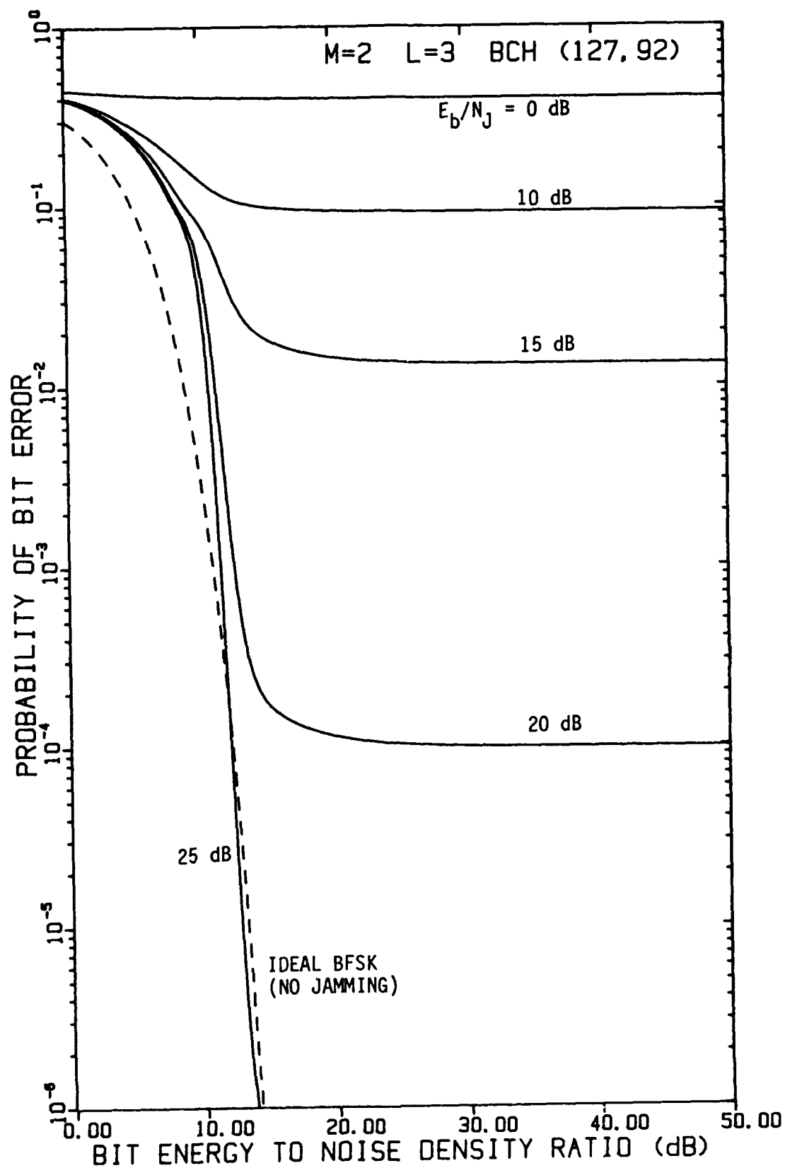
FIGURE 4-23 PERFORMANCE OF FH/BFSK WITH BCH (127,92) CODE AND L=3 HOPS/DIGIT AS A FUNCTION OF E_b/N_0 WITH E_b/N_J AS A PARAMETER, USING A LINEAR COMBINING DEMODULATOR, IN OPTIMUM PARTIAL-BAND NOISE JAMMING
