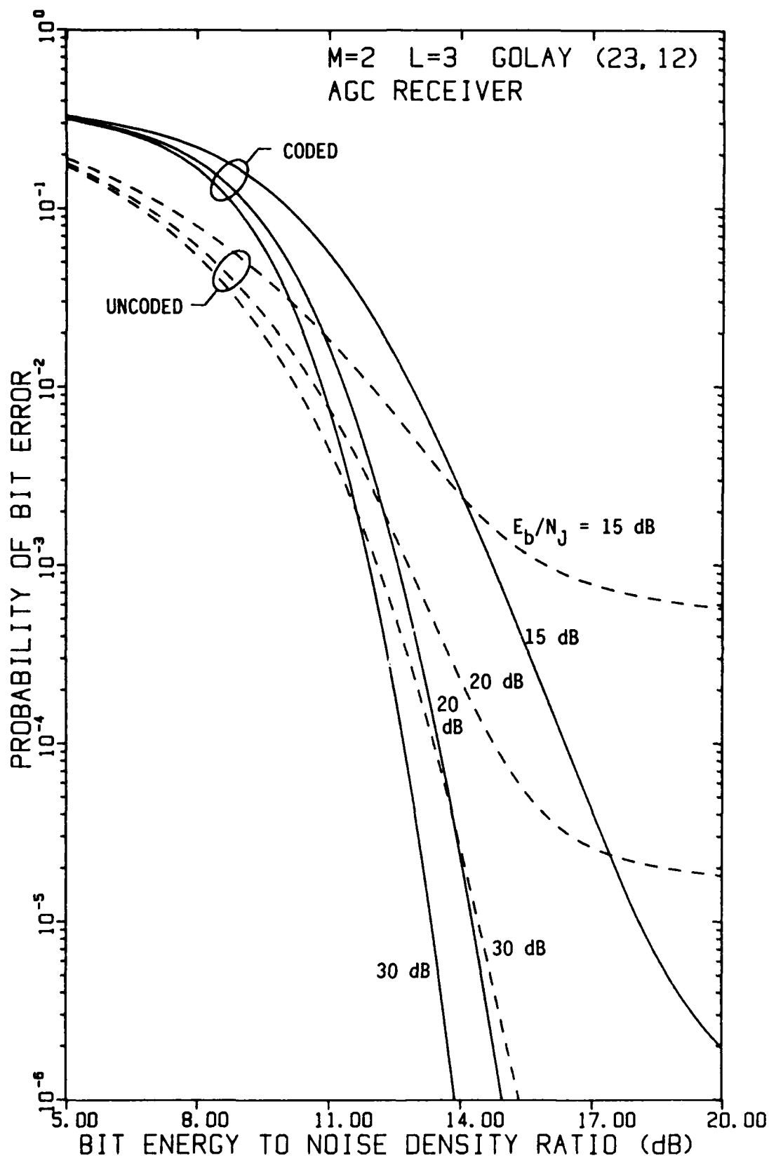
FIGURE 4-76 PERFORMANCE OF FH/BFSK WITH GOLAY (23,12) CODE AND L=3 HOPS/DIGIT AS A FUNCTION OF E_b/N_0 WITH E_b/N_j AS A PARAMETER, USING AN AGC DEMODULATOR, IN OPTIMUM PARTIAL-BAND NOISE JAMMING
