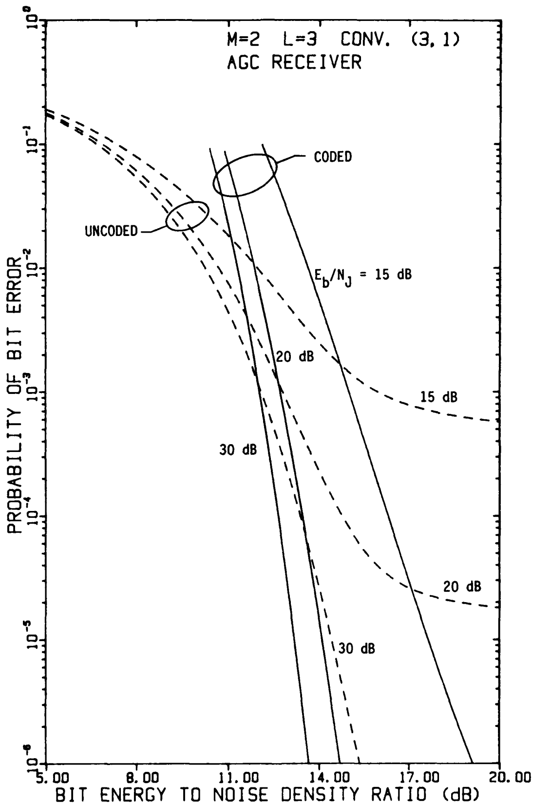
FIGURE 4-100 PERFORMANCE OF FH/BFSK WITH CONVOLUTIONAL RATE-1/3 CODE AND L=3 HOPS/DIGIT AS A FUNCTION OF E_b/N_0 WITH E_b/N_J AS A PARAMETER, USING AN AGC DEMODULATOR, IN OPTIMUM PARTIAL-BAND NOISE JAMMING
