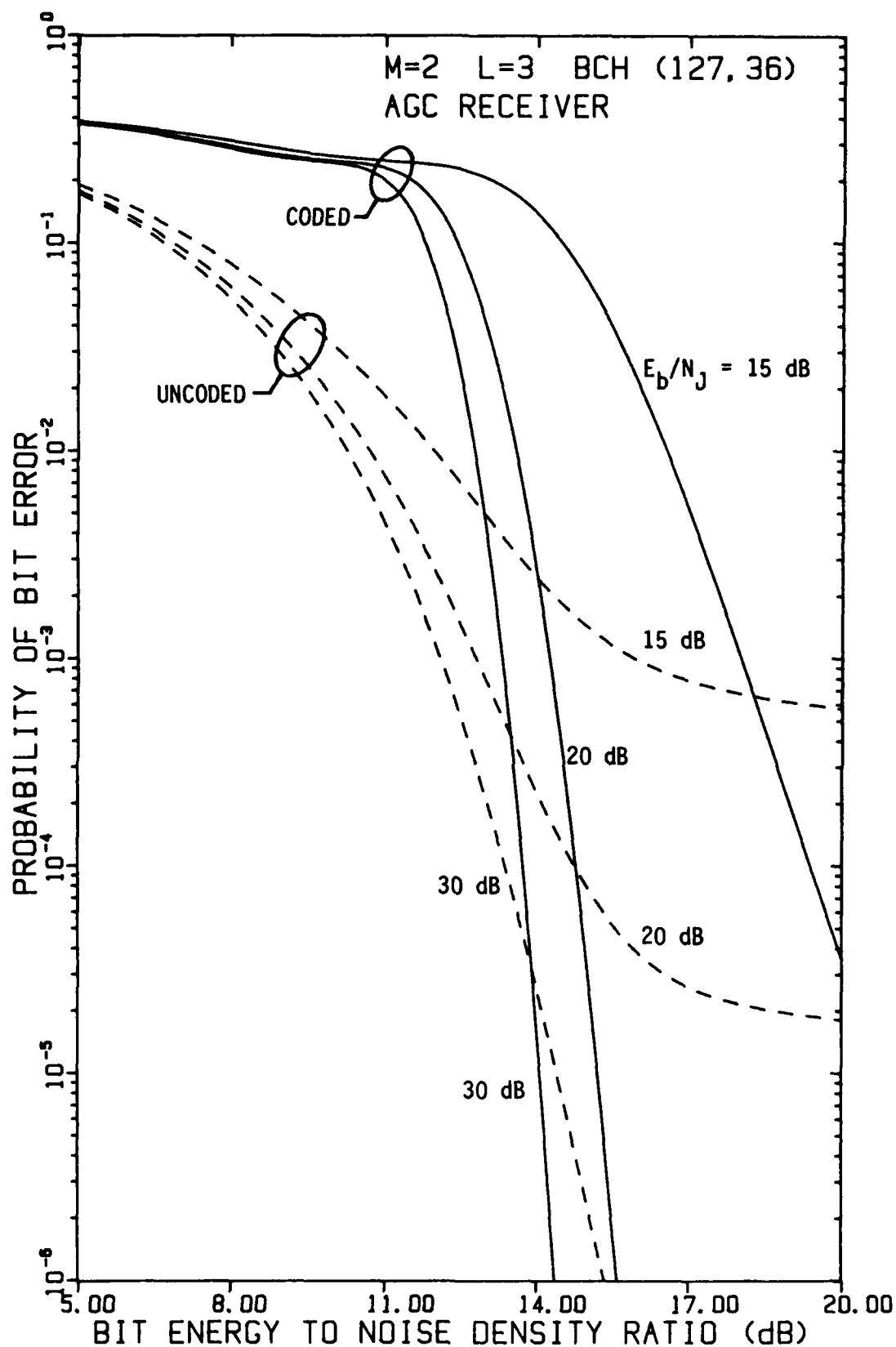
FIGURE 4-88 PERFORMANCE OF FH/BFSK WITH BCH (127,36) CODE AND L=3 HOPS/DIGIT AS A FUNCTION OF E_b/N_0 WITH E_b/N_J AS A PARAMETER, USING AN AGC DEMODULATOR, IN OPTIMUM PARTIAL-BAND NOISE JAMMING
