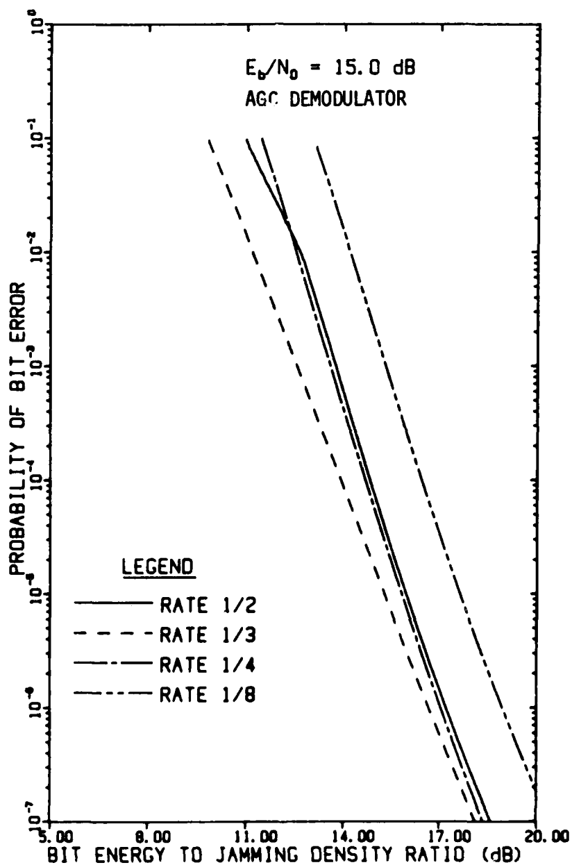
FIGURE 4-111 PERFORMANCE OF CONSTRAINT-LENGTH-7 CONVOLUTIONAL CODES USING FH/BFSK WITH OPTIMUM DIVERSITY IN WORST-CASE PARTIAL-BAND NOISE JAMMING AS A FUNCTION OF E_b/N_j WHEN E_b/N_0 = 15 \text{ dB}
