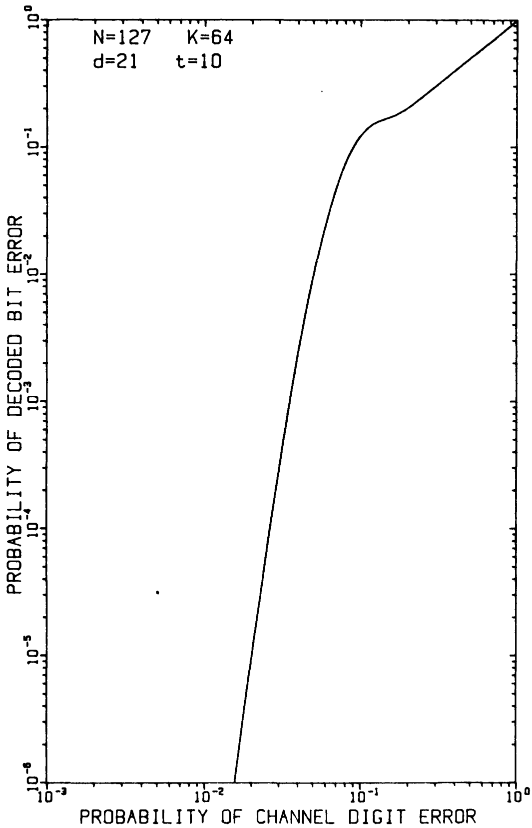
FIGURE 3-4 DECODER PERFORMANCE FOR BCH (127,64) CODE
