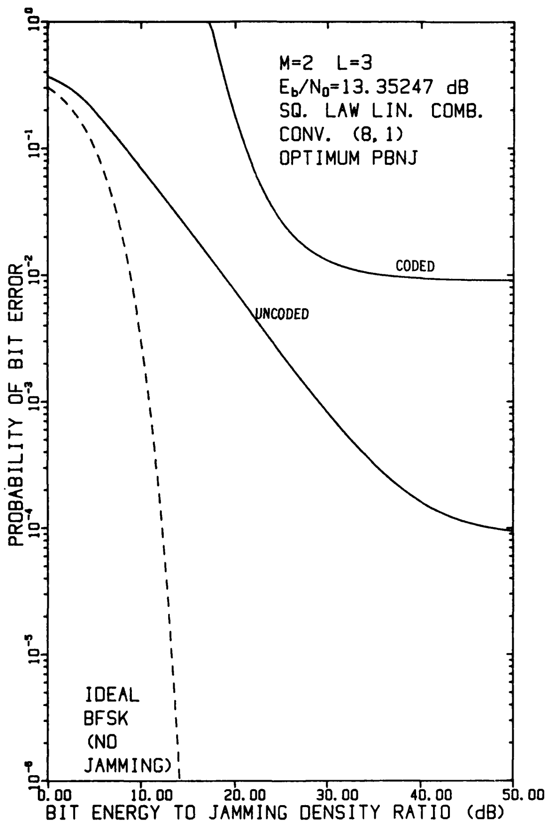
FIGURE 4-63 PERFORMANCE OF FH/BFSK WITH CONVOLUTIONAL RATE-1/8 CODE AND L=3 HOPS/DIGIT AS A FUNCTION OF E_b/N_j WHEN E_b/N_0 = 13.35247 dB, USING A LINEAR COMBINING DEMODULATOR, IN OPTIMUM PARTIAL-BAND NOISE JAMMING
