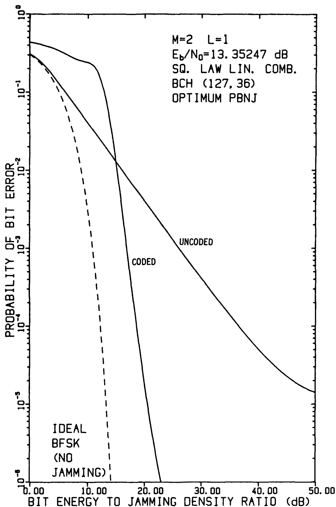
FIGURE 4-41 PERFORMANCE OF FH/BFSK WITH BCH (127,36) CODE AND L=1 HOP/DIGIT AS A FUNCTION OF E_b/N_j WHEN E_b/N_0 = 13.35247 dB, USING A LINEAR COMBINING DEMODULATOR, IN OPTIMUM PARTIAL-BAND NOISE JAMMING
