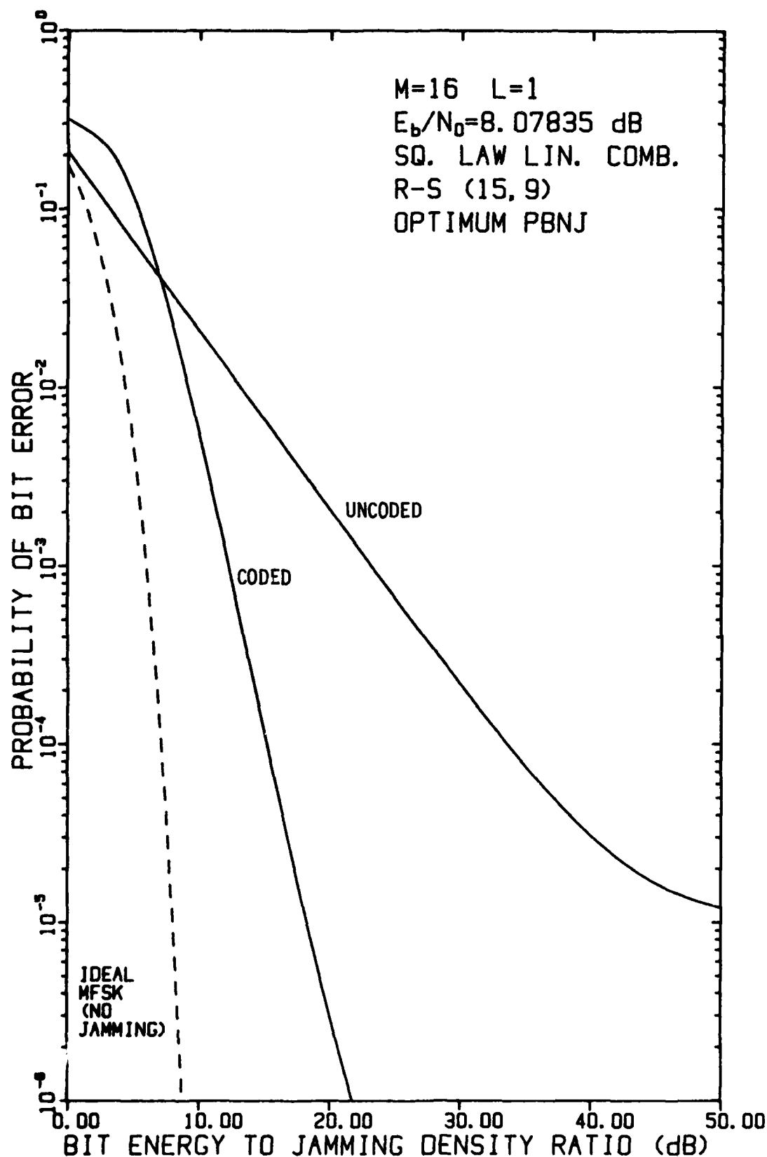
FIGURE 4-67 PERFORMANCE OF FH/MFSK WITH REED-SOLOMON (15,9) CODE AND L=1 HOP/DIGIT AS A FUNCTION OF E_b/N_j WHEN E_b/N_0 = 8.07835 dB, USING A LINEAR COMBINING DEMODULATOR, IN OPTIMUM PARTIAL-BAND NOISE JAMMING
