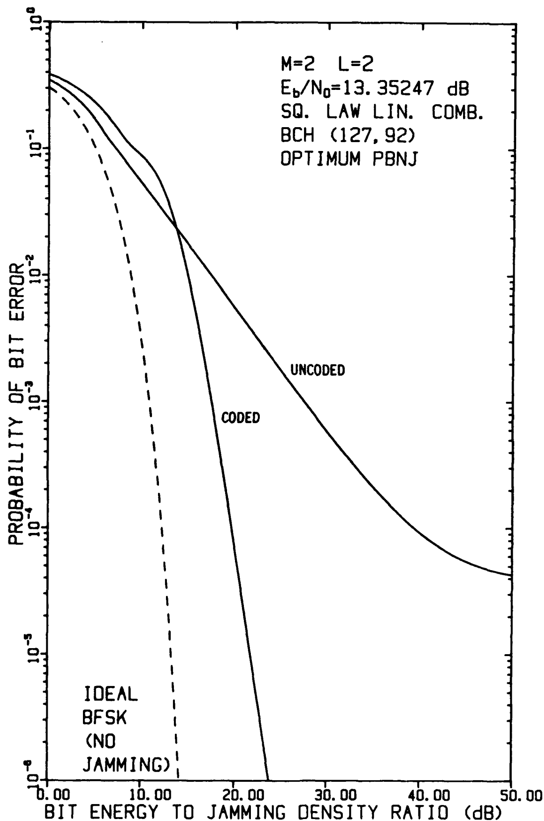
FIGURE 4-26 PERFORMANCE OF FH/BFSK WITH BCH (127,92) CODE AND L=2 HOPS/DIGIT AS A FUNCTION OF E_b/N_j WHEN E_b/N_0 = 13.35247 dB, USING A LINEAR COMBINING DEMODULATOR, IN OPTIMUM PARTIAL-BAND NOISE JAMMING
