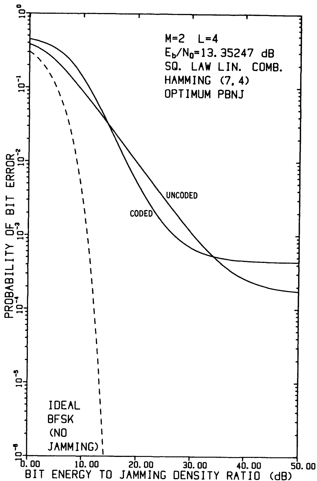
FIGURE 4-12 PERFORMANCE OF FH/BFSK WITH HAMMING (7,4) CODE AND L=4 HOPS/DIGIT AS A FUNCTION OF E_b/N_J WHEN E_b/N_0 = 13.35247 dB, USING A LINEAR COMBINING DEMODULATOR, IN OPTIMUM PARTIAL-BAND NOISE JAMMING
