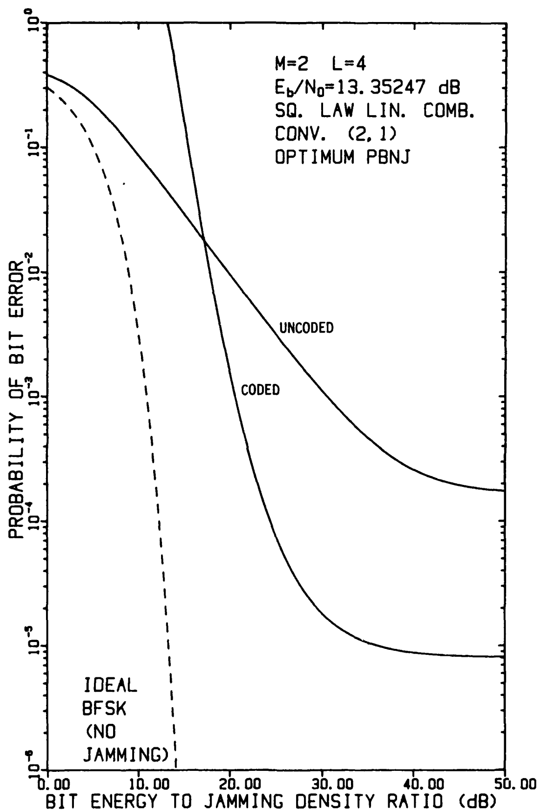
FIGURE 4-52 PERFORMANCE OF FH/BFSK WITH CONVOLUTIONAL RATE-1/2 CODE AND L=4 HOPS/DIGIT AS A FUNCTION OF E_b/N_j WHEN E_b/N_0 = 13.35247 dB, USING A LINEAR COMBINING DEMODULATOR, IN OPTIMUM PARTIAL-BAND NOISE JAMMING
