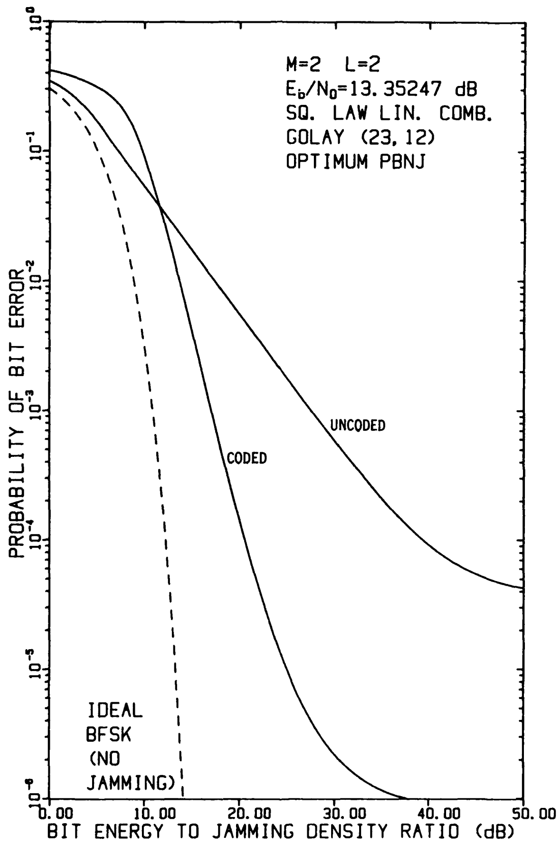
FIGURE 4-18 PERFORMANCE OF FH/BFSK WITH GOLAY (23,12) CODE AND L=2 HOPS/DIGIT AS A FUNCTION OF E_b/N_J WHEN E_b/N_0 = 13.35247 dB, USING A LINEAR COMBINING DEMODULATOR, IN OPTIMUM PARTIAL-BAND NOISE JAMMING
