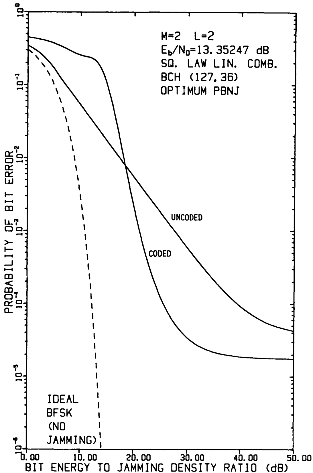
FIGURE 4-42 PERFORMANCE OF FH/BFSK WITH BCH (127,36) CODE AND L=2 HOPS/DIGIT AS A FUNCTION OF E_b/N_j WHEN E_b/N_0 = 13.35247 dB, USING A LINEAR COMBINING DEMODULATOR, IN OPTIMUM PARTIAL-BAND NOISE JAMMING
