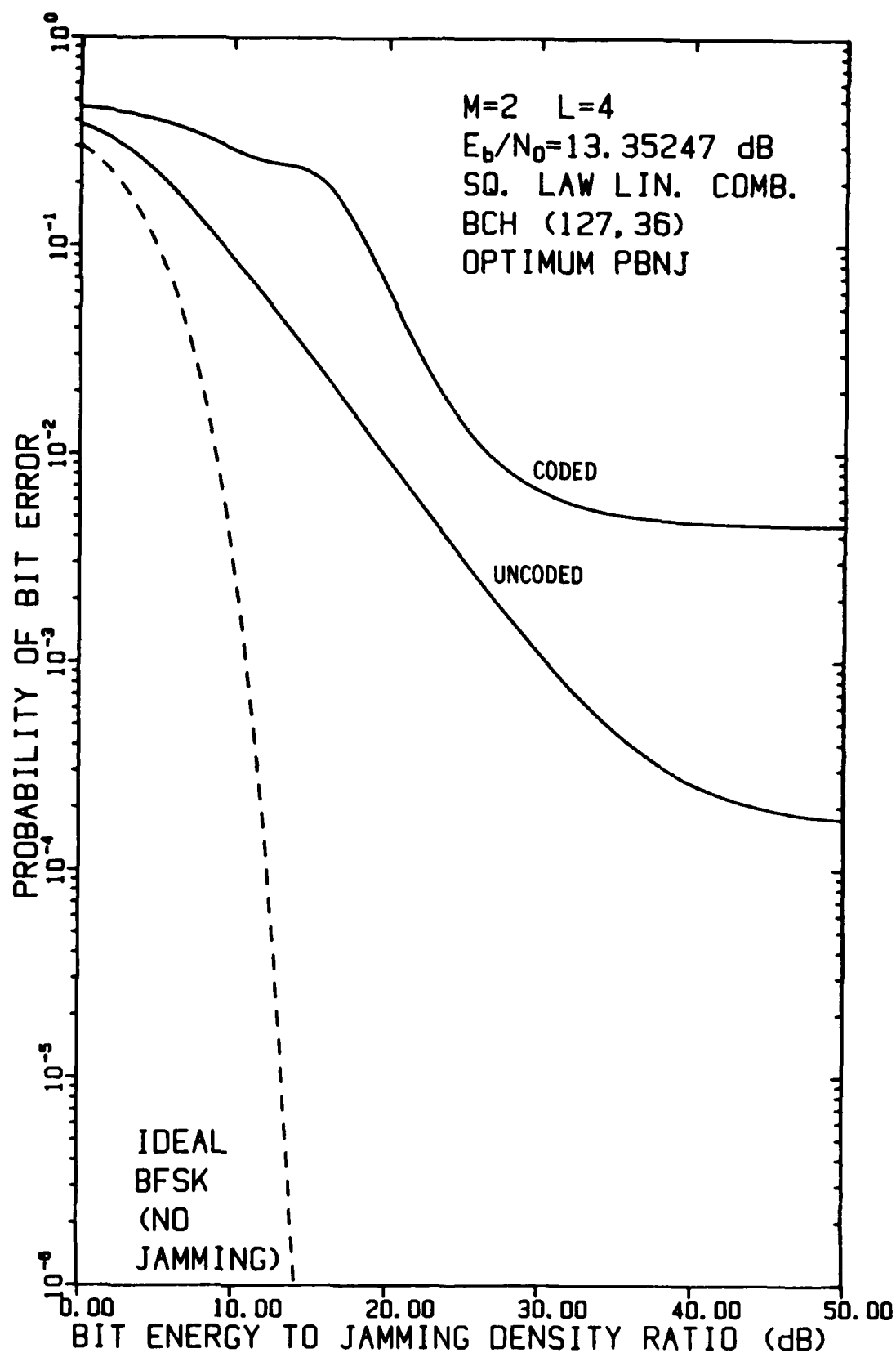
FIGURE 4-44 PERFORMANCE OF FH/BFSK WITH BCH (127,36) CODE AND L=4 HOPS/DIGIT AS A FUNCTION OF E_b/N_j WHEN E_b/N_0 = 13.35247 dB, USING A LINEAR COMBINING DEMODULATOR, IN OPTIMUM PARTIAL-BAND NOISE JAMMING
