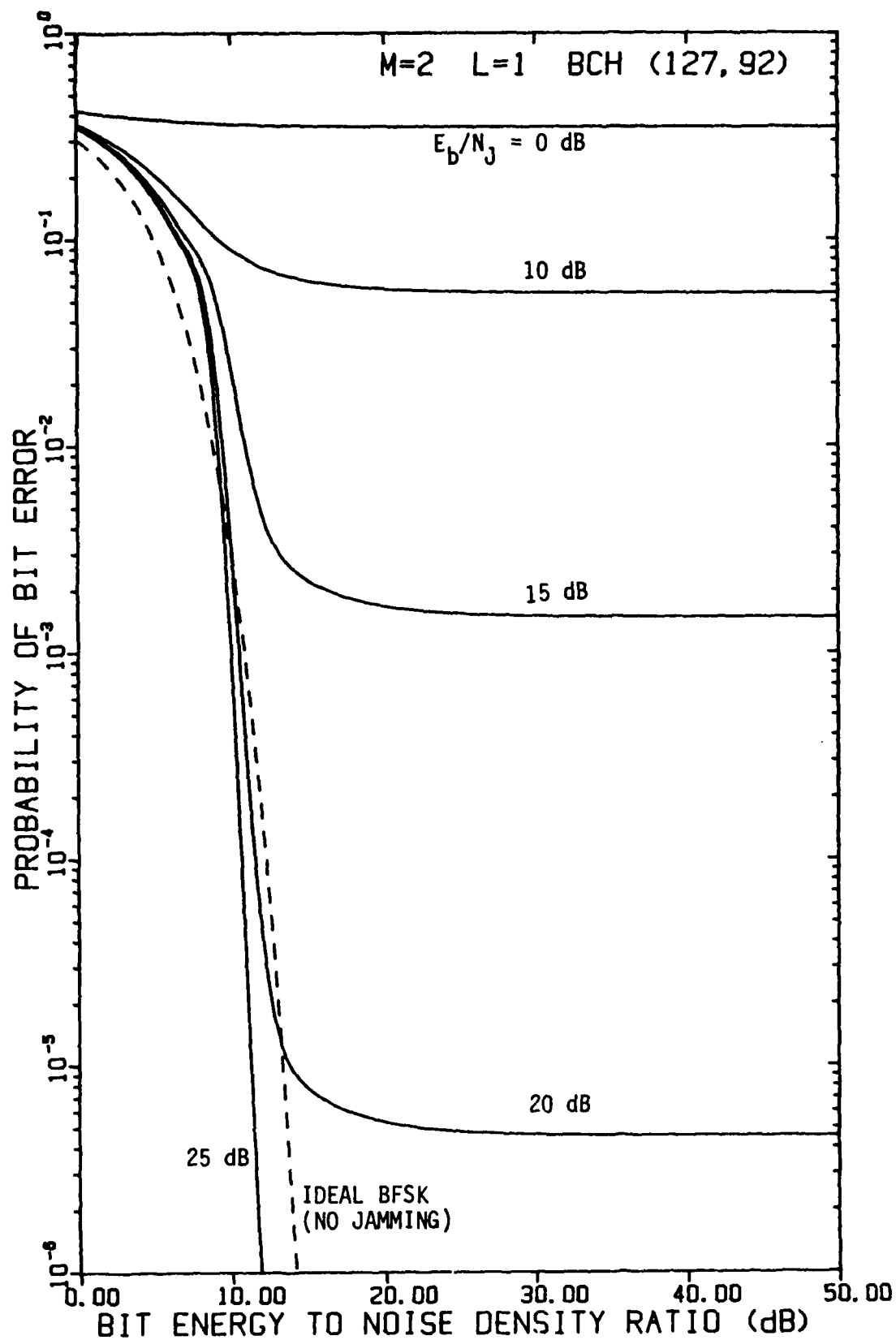
FIGURE 4-21 PERFORMANCE OF FH/BFSK WITH BCH (127,92) CODE AND L=1 HOP/DIGIT AS A FUNCTION OF E_b/N_0 WITH E_b/N_j AS A PARAMETER, USING A LINEAR COMBINING DEMODULATOR, IN OPTIMUM PARTIAL-BAND NOISE JAMMING
