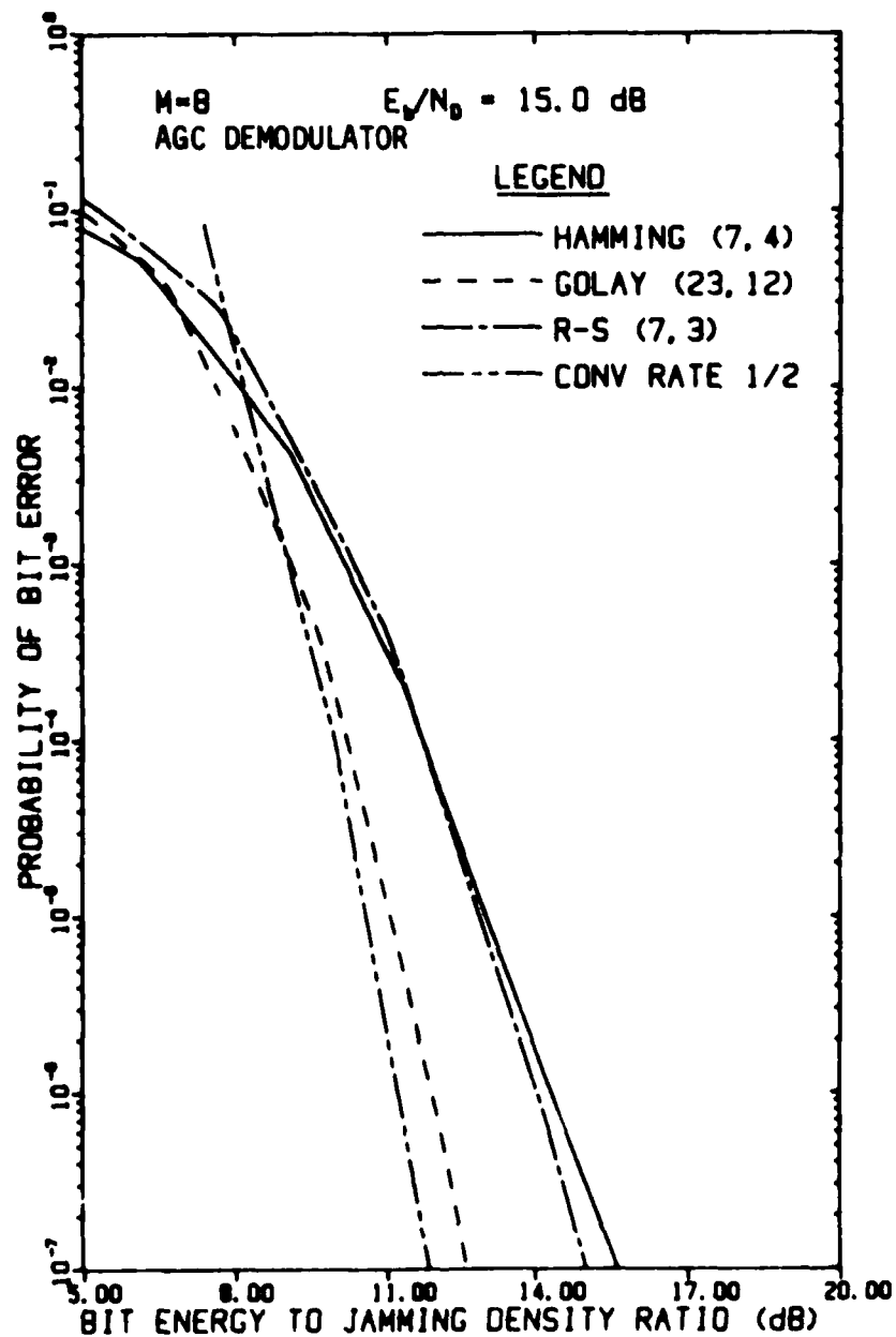
FIGURE 4-114 PERFORMANCE OF SEVERAL CODES WITH FH/8-ARY FSK USING OPTIMUM DIVERSITY IN WORST-CASE PARTIAL-BAND NOISE JAMMING AS A FUNCTION OF E_b/N_J WHEN E_b/N_0 = 15 \text{ dB} (R-S DENOTES REED-SOLOMON)
