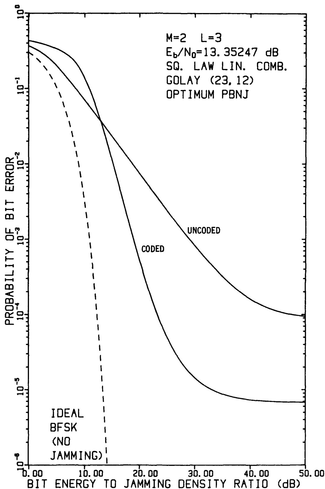
FIGURE 4-19 PERFORMANCE OF FH/BFSK WITH GOLAY (23,12) CODE AND L=3 HOPS/DIGIT AS A FUNCTION OF E_b/N_j WHEN E_b/N_0 = 13.35247 dB, USING A LINEAR COMBINING DEMODULATOR, IN OPTIMUM PARTIAL-BAND NOISE JAMMING
