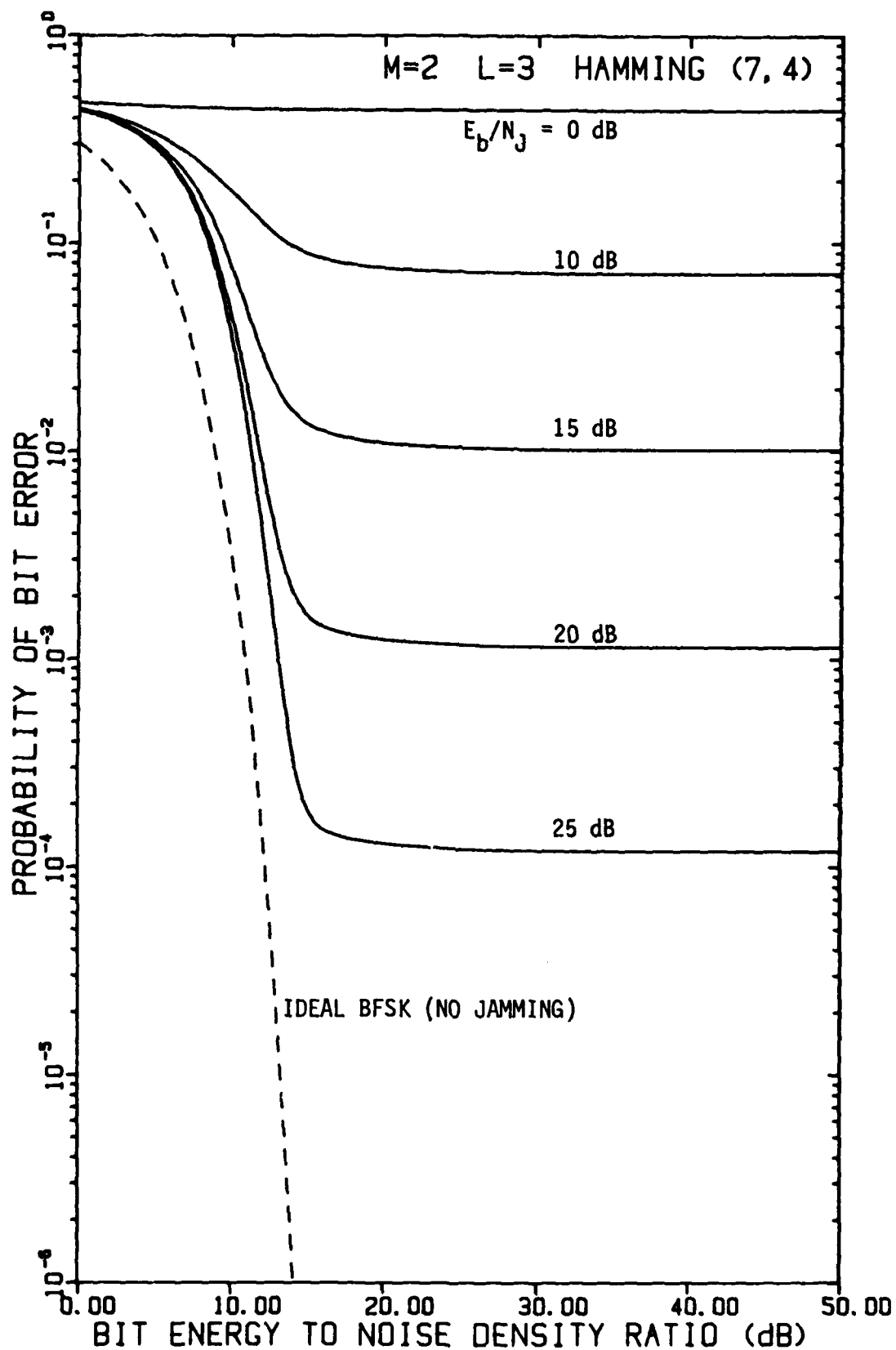
FIGURE 4-7 PERFORMANCE OF FH/BFSK WITH HAMMING (7,4) CODE AND L=3 HOPS/DIGIT AS A FUNCTION OF E_b/N_0 WITH E_b/N_j AS A PARAMETER, USING A LINEAR COMBINING DEMODULATOR, IN OPTIMUM PARTIAL-BAND NOISE JAMMING
