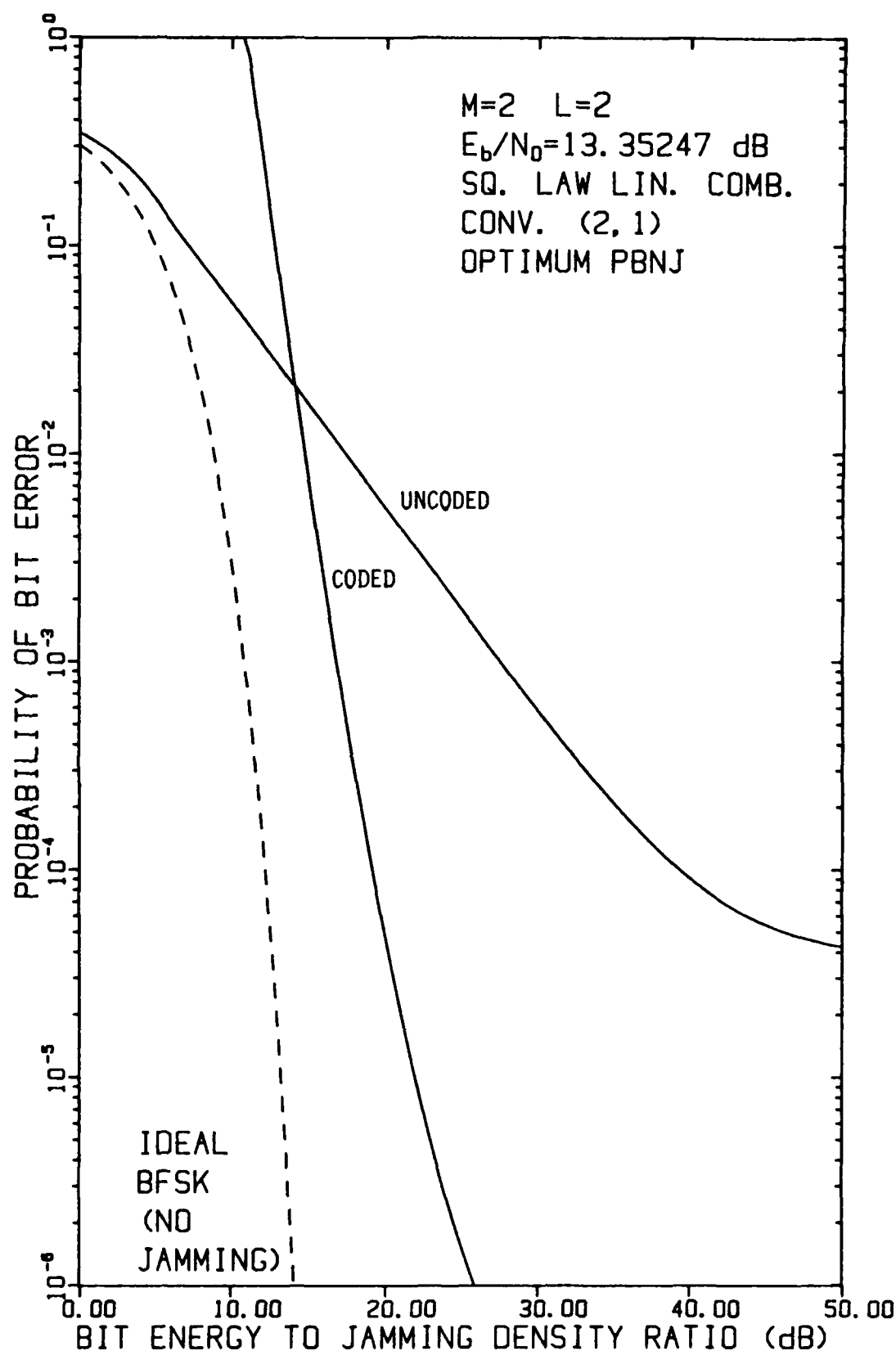
FIGURE 4-50 PERFORMANCE OF FH/BFSK WITH CONVOLUTIONAL RATE-1/2 CODE AND L=2 HOPS/DIGIT AS A FUNCTION OF E_b/N_j WHEN E_b/N_0 = 13.35247 dB, USING A LINEAR COMBINING DEMODULATOR, IN OPTIMUM PARTIAL-BAND NOISE JAMMING
