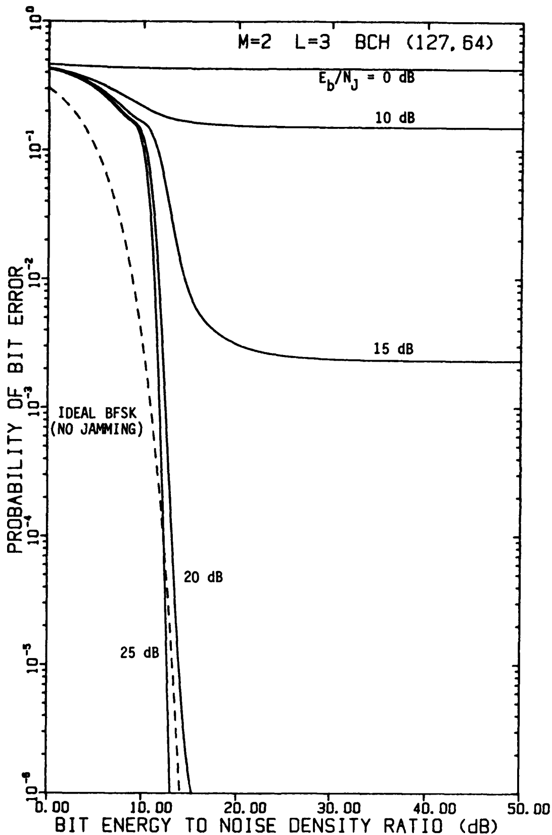
FIGURE 4-31 PERFORMANCE OF FH/BFSK WITH BCH (127,64) CODE AND L=3 HOPS/DIGIT AS A FUNCTION OF E_b/N_0 WITH E_b/N_J AS A PARAMETER, USING A LINEAR COMBINING DEMODULATOR, IN OPTIMUM PARTIAL-BAND NOISE JAMMING
