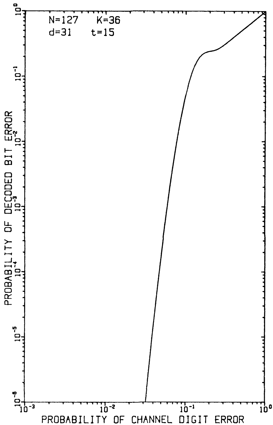
FIGURE 3-5 DECODER PERFORMANCE FOR BCH (127,36) CODE
