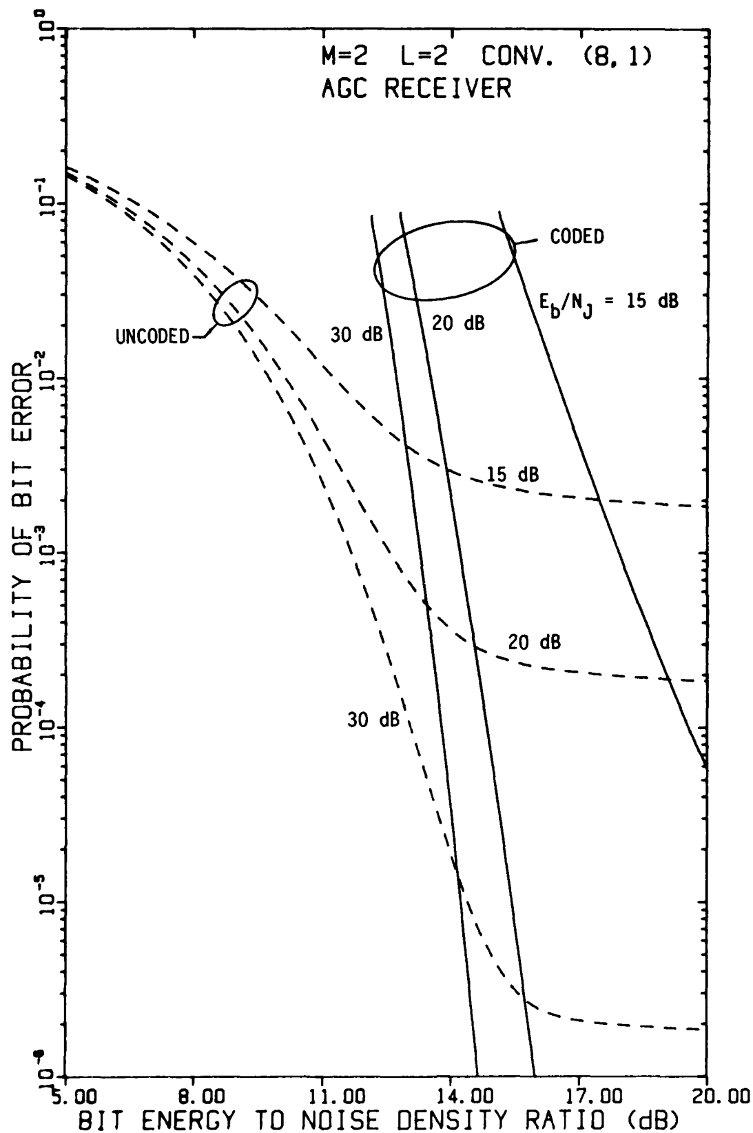
FIGURE 4-107 PERFORMANCE OF FH/BFSK WITH CONVOLUTIONAL RATE-1/8 CODE AND L=2 HOPS/DIGIT AS A FUNCTION OF E_b/N_0 WITH E_b/N_J AS A PARAMETER, USING AN AGC DEMODULATOR, IN OPTIMUM PARTIAL-BAND NOISE JAMMING
