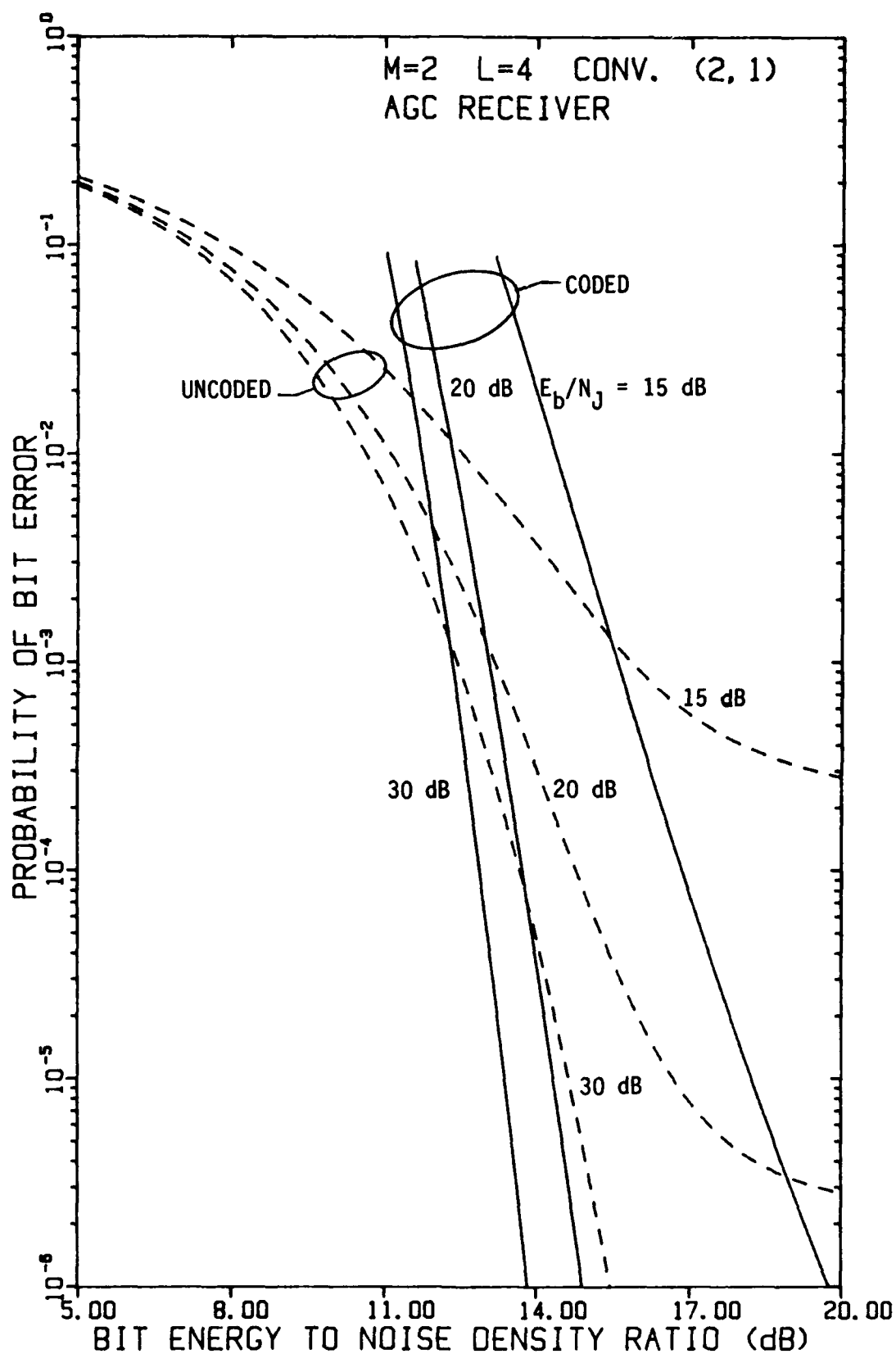
FIGURE 4-97 PERFORMANCE OF FH/BFSK WITH CONVOLUTIONAL RATE-1/2 CODE AND L=4 HOPS/DIGIT AS A FUNCTION OF E_b/N_0 WITH E_b/N_J AS A PARAMETER, USING AN AGC DEMODULATOR, IN OPTIMUM PARTIAL-BAND NOISE JAMMING
