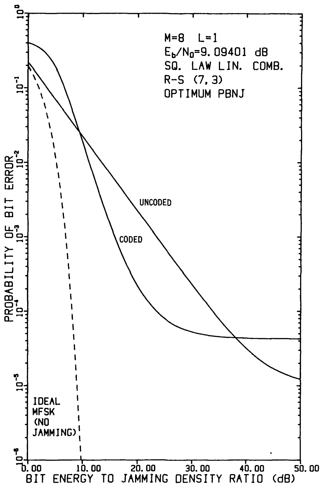
FIGURE 4-65 PERFORMANCE OF FH/MFSK WITH REED-SOLOMON (7,3) CODE AND L=1 HOP/DIGIT AS A FUNCTION OF E_b/N_j WHEN E_b/N_0 = 9.09401 dB, USING A LINEAR COMBINING DEMODULATOR, IN OPTIMUM PARTIAL-BAND NOISE JAMMING
