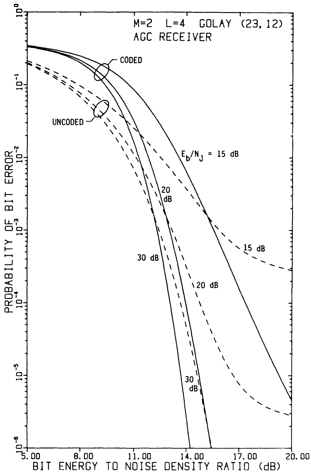
FIGURE 4-77 PERFORMANCE OF FH/BFSK WITH GOLAY (23,12) CODE AND L=4 HOPS/DIGIT AS A FUNCTION OF E_b/N_0 WITH E_b/N_J AS A PARAMETER, USING AN AGC DEMODULATOR, IN OPTIMUM PARTIAL-BAND NOISE JAMMING
