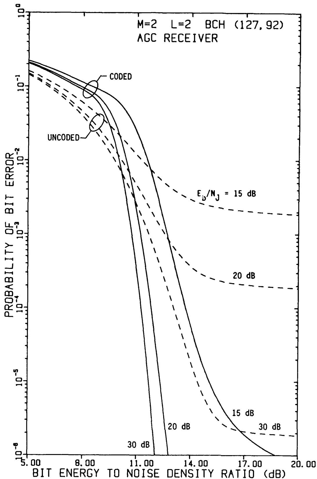
FIGURE 4-79 PERFORMANCE OF FH/BFSK WITH BCH (127,92) CODE AND L=2 HOPS/DIGIT AS A FUNCTION OF E_b/N_0 WITH E_b/N_J AS A PARAMETER, USING AN AGC DEMODULATOR, IN OPTIMUM PARTIAL-BAND NOISE JAMMING
