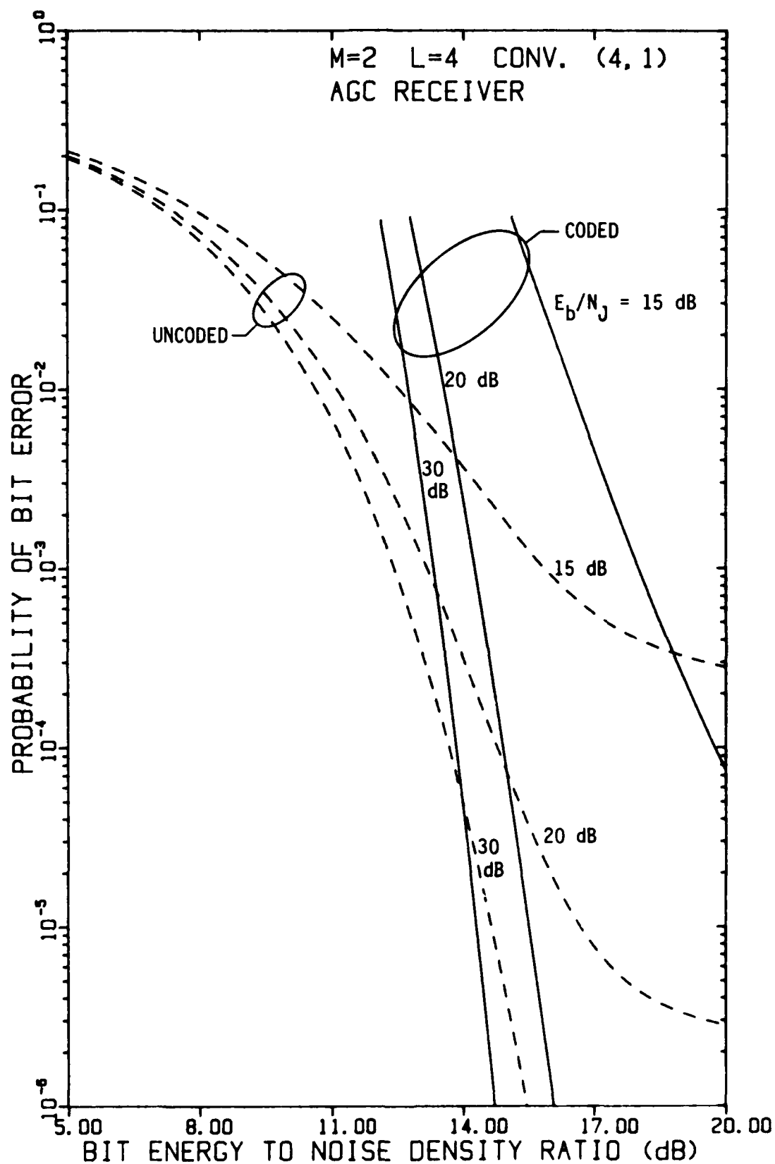
FIGURE 4-105 PERFORMANCE OF FH/BFSK WITH CONVOLUTIONAL RATE-1/4 CODE AND L=4 HOPS/DIGIT AS A FUNCTION OF E_b/N_0 WITH E_b/N_j AS A PARAMETER, USING AN AGC DEMODULATOR, IN OPTIMUM PARTIAL-BAND NOISE JAMMING
