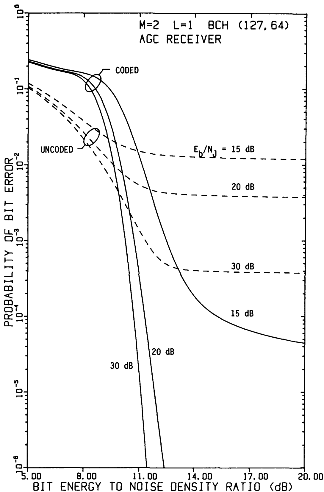
FIGURE 4-82 PERFORMANCE OF FH/BFSK WITH BCH (127,64) CODE AND L=1 HOP/DIGIT AS A FUNCTION OF E_b/N_0 WITH E_b/N_j AS A PARAMETER, USING AN AGC DEMODULATOR, IN OPTIMUM PARTIAL-BAND NOISE JAMMING
