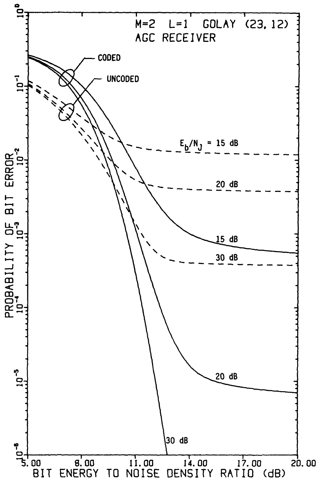
FIGURE 4-74 PERFORMANCE OF FH/BFSK WITH GOLAY (23,12) CODE AND L=1 HOP/DIGIT AS A FUNCTION OF E_b/N_0 WITH E_b/N_j AS A PARAMETER, USING AN AGC DEMODULATOR, IN OPTIMUM PARTIAL-BAND NOISE JAMMING
