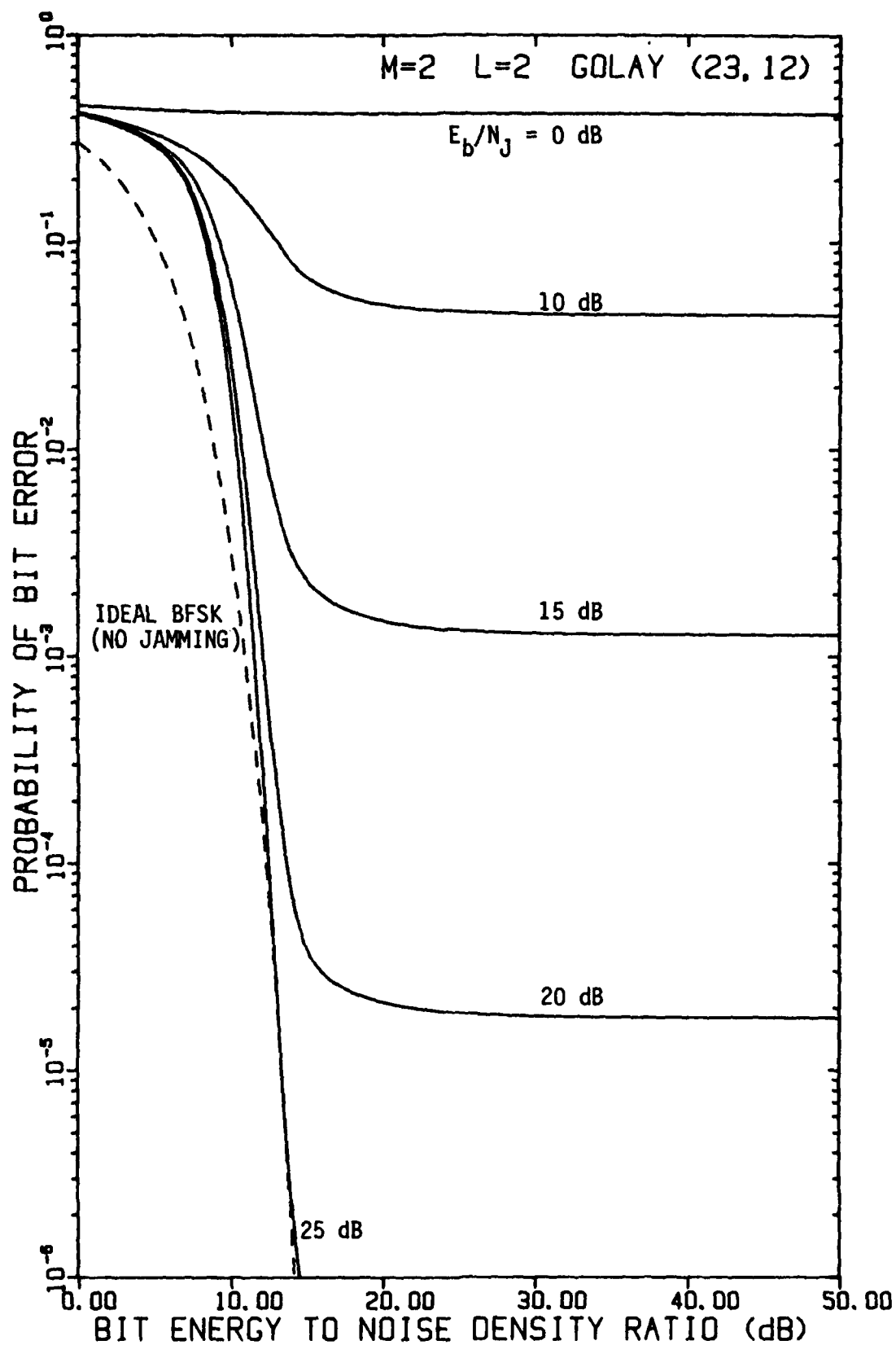
FIGURE 4-14 PERFORMANCE OF FH/BFSK WITH GOLAY (23,12) CODE AND L=2 HOPS/DIGIT AS A FUNCTION OF E_b/N_0 WITH E_b/N_J AS A PARAMETER, USING A LINEAR COMBINING DEMODULATOR, IN OPTIMUM PARTIAL-BAND NOISE JAMMING
