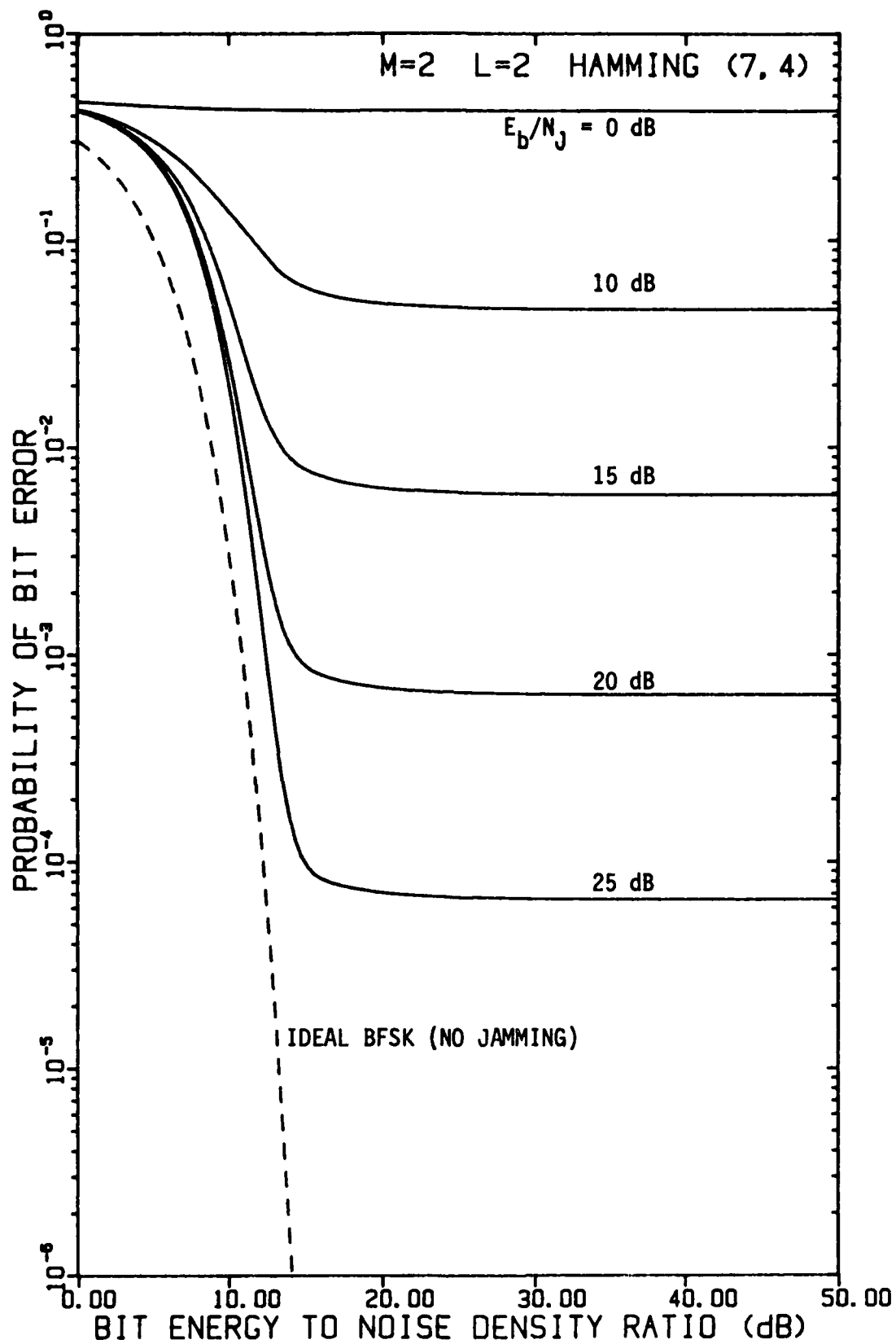
FIGURE 4-6 PERFORMANCE OF FH/BFSK WITH HAMMING (7,4) CODE AND L=2 HOPS/DIGIT AS A FUNCTION OF E_b/N_0 WITH E_b/N_j AS A PARAMETER, USING A LINEAR COMBINING DEMODULATOR, IN OPTIMUM PARTIAL-BAND NOISE JAMMING
