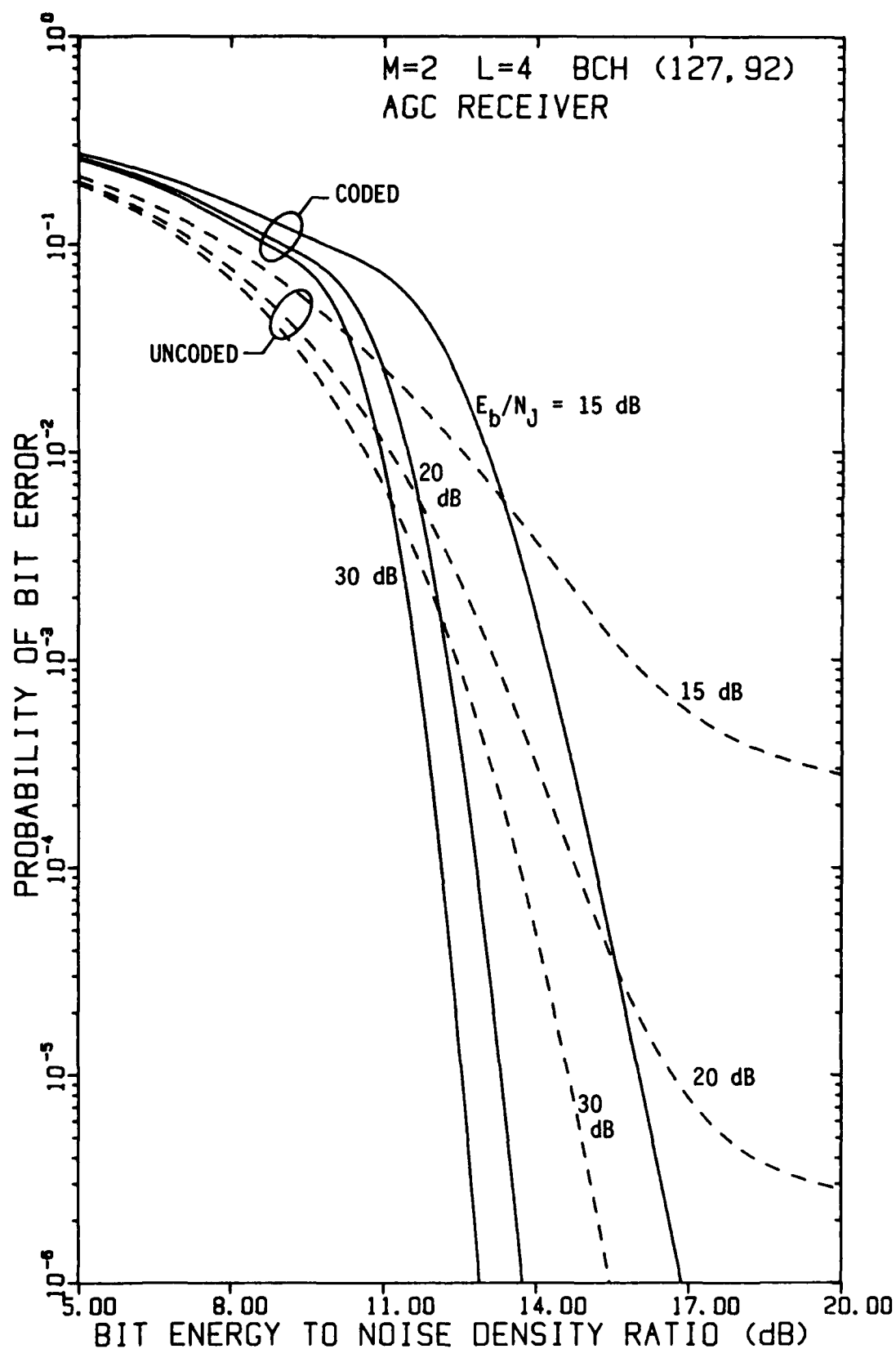
FIGURE 4-81 PERFORMANCE OF FH/BFSK WITH BCH (127,92) CODE AND L=4 HOPS/DIGIT AS A FUNCTION OF E_b/N_0 WITH E_b/N_J AS A PARAMETER, USING AN AGC DEMODULATOR, IN OPTIMUM PARTIAL-BAND NOISE JAMMING
