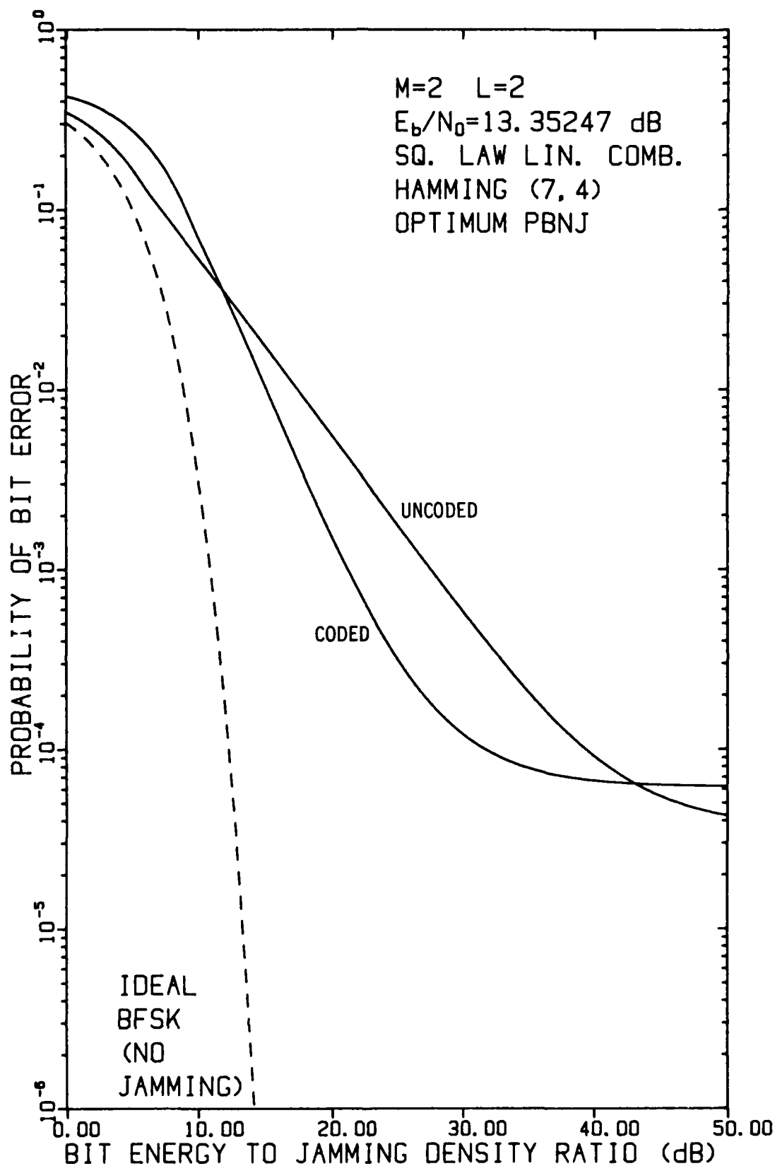
FIGURE 4-10 PERFORMANCE OF FH/BFSK WITH HAMMING (7,4) CODE AND L=2 HOPS/DIGIT AS A FUNCTION OF E_b/N_j WHEN E_b/N_0 = 13.35247 dB, USING A LINEAR COMBINING DEMODULATOR, IN OPTIMUM PARTIAL-BAND NOISE JAMMING
