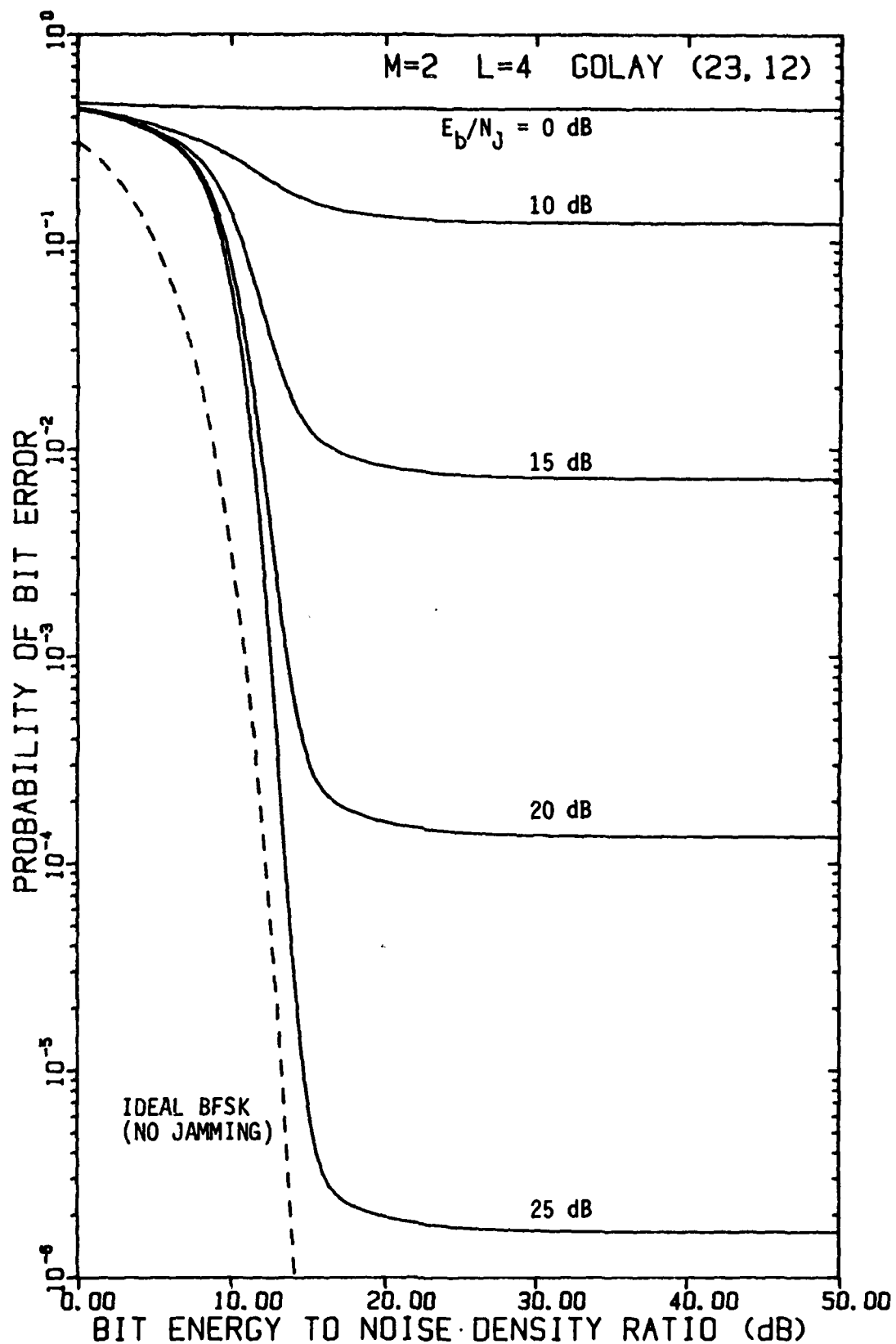
FIGURE 4-16 PERFORMANCE OF FH/BFSK WITH GOLAY (23,12) CODE AND L=4 HOPS/DIGIT AS A FUNCTION OF E_b/N_0 WITH E_b/N_j AS A PARAMETER, USING A LINEAR COMBINING DEMODULATOR, IN OPTIMUM PARTIAL-BAND NOISE JAMMING
