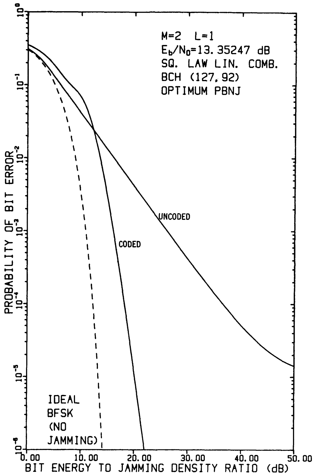
FIGURE 4-25 PERFORMANCE OF FH/BFSK WITH BCH (127,92) CODE AND L=1 HOP/DIGIT AS A FUNCTION OF E_b/N_j WHEN E_b/N_0 = 13.35247 dB, USING A LINEAR COMBINING DEMODULATOR, IN OPTIMUM PARTIAL-BAND NOISE JAMMING
