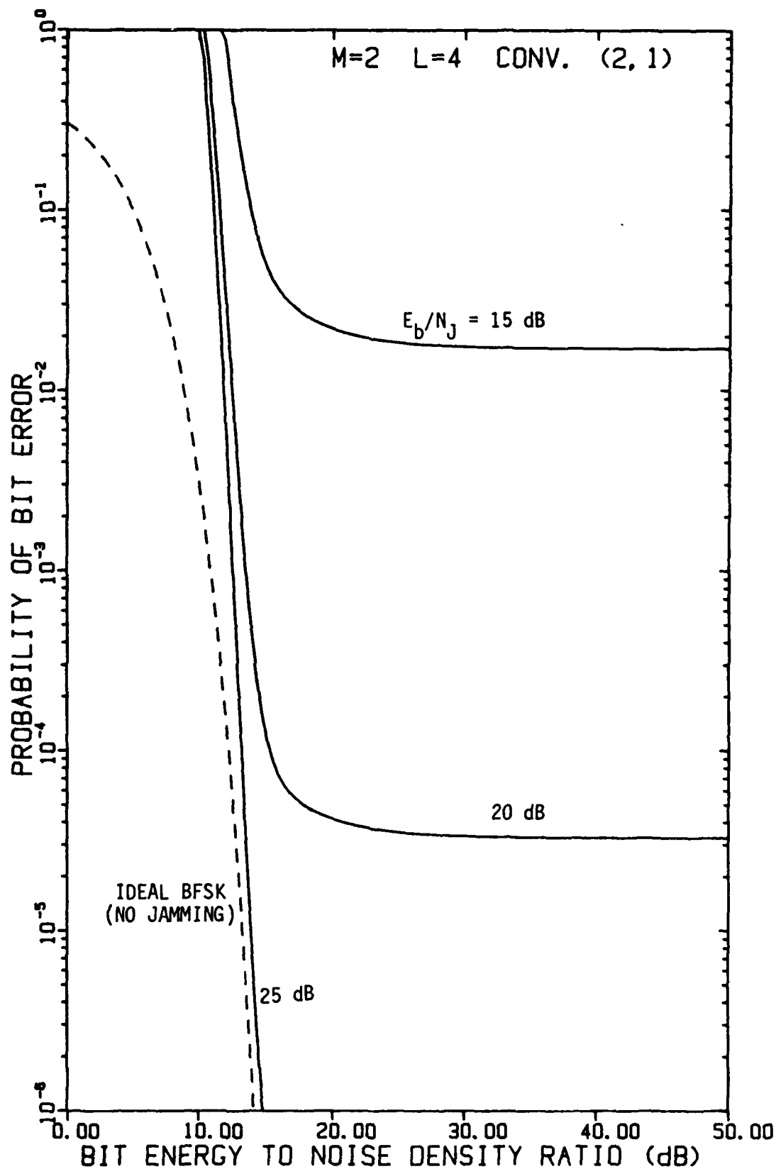
FIGURE 4-48 PERFORMANCE OF FH/BFSK WITH CONVOLUTIONAL RATE-1/2 CODE AND L=4 HOPS/DIGIT AS A FUNCTION OF E_b/N_0 WITH E_b/N_J AS A PARAMETER, USING A LINEAR COMBINING DEMODULATOR, IN OPTIMUM PARTIAL-BAND NOISE JAMMING
