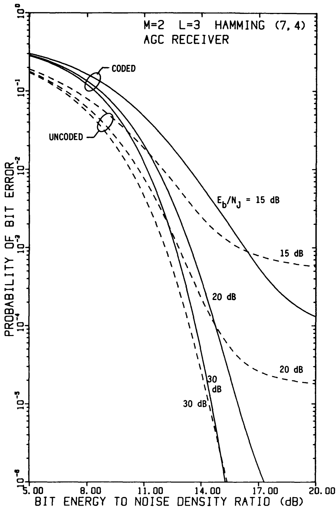
FIGURE 4-72 PERFORMANCE OF FH/BFSK WITH HAMMING (7,4) CODE AND L=3 HOPS/DIGIT AS A FUNCTION OF E_b/N_0 WITH E_b/N_j AS A PARAMETER, USING AN AGC DEMODULATOR, IN OPTIMUM PARTIAL-BAND NOISE JAMMING
