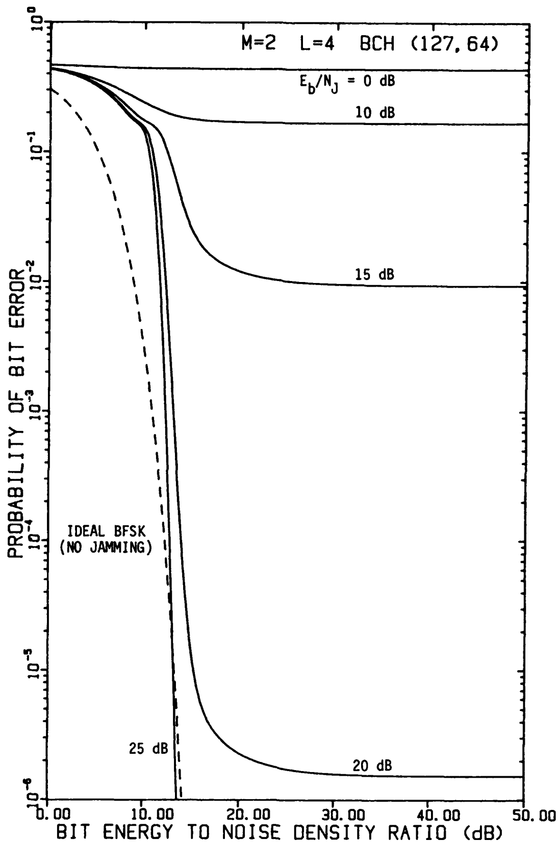
FIGURE 4-32 PERFORMANCE OF FH/BFSK WITH BCH (127,64) CODE AND L=4 HOPS/DIGIT AS A FUNCTION OF E_b/N_0 WITH E_b/N_J AS A PARAMETER, USING A LINEAR COMBINING DEMODULATOR, IN OPTIMUM PARTIAL-BAND NOISE JAMMING
