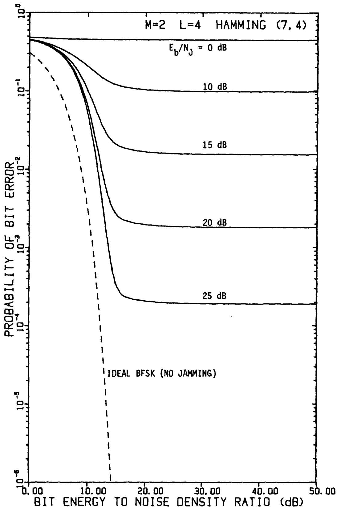
FIGURE 4-8 PERFORMANCE OF FH/BFSK WITH HAMMING (7,4) CODE AND L=4 HOPS/DIGIT AS A FUNCTION OF E_b/N_0 WITH E_b/N_J AS A PARAMETER, USING A LINEAR COMBINING DEMODULATOR, IN OPTIMUM PARTIAL-BAND NOISE JAMMING
