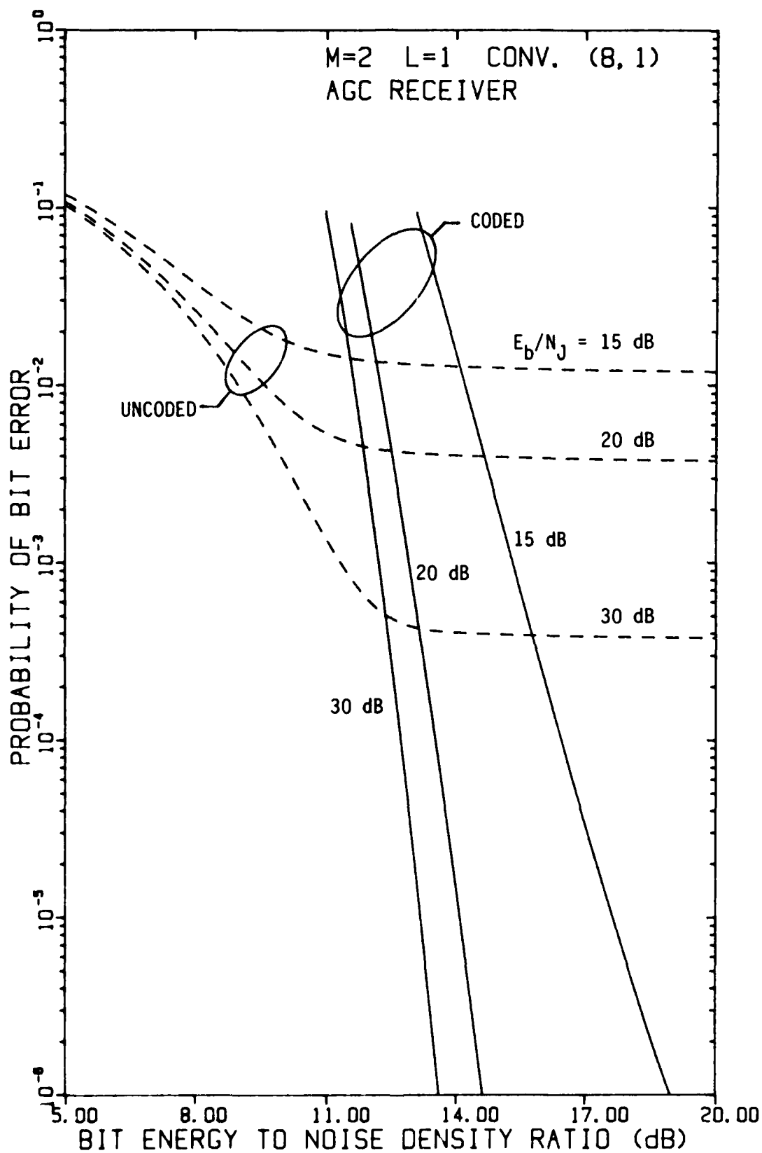
FIGURE 4-106 PERFORMANCE OF FH/BFSK WITH CONVOLUTIONAL RATE-1/8 CODE AND L=1 HOP/DIGIT AS A FUNCTION OF E_b/N_0 WITH E_b/N_J AS A PARAMETER, USING AN AGC DEMODULATOR, IN OPTIMUM PARTIAL-BAND NOISE JAMMING
