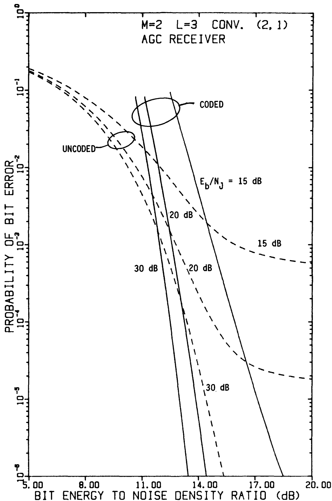
FIGURE 4-96 PERFORMANCE OF FH/BFSK WITH CONVOLUTIONAL RATE-1/2 CODE AND L=3 HOPS/DIGIT AS A FUNCTION OF E_b/N_0 WITH E_b/N_j AS A PARAMETER, USING AN AGC DEMODULATOR, IN OPTIMUM PARTIAL-BAND NOISE JAMMING
