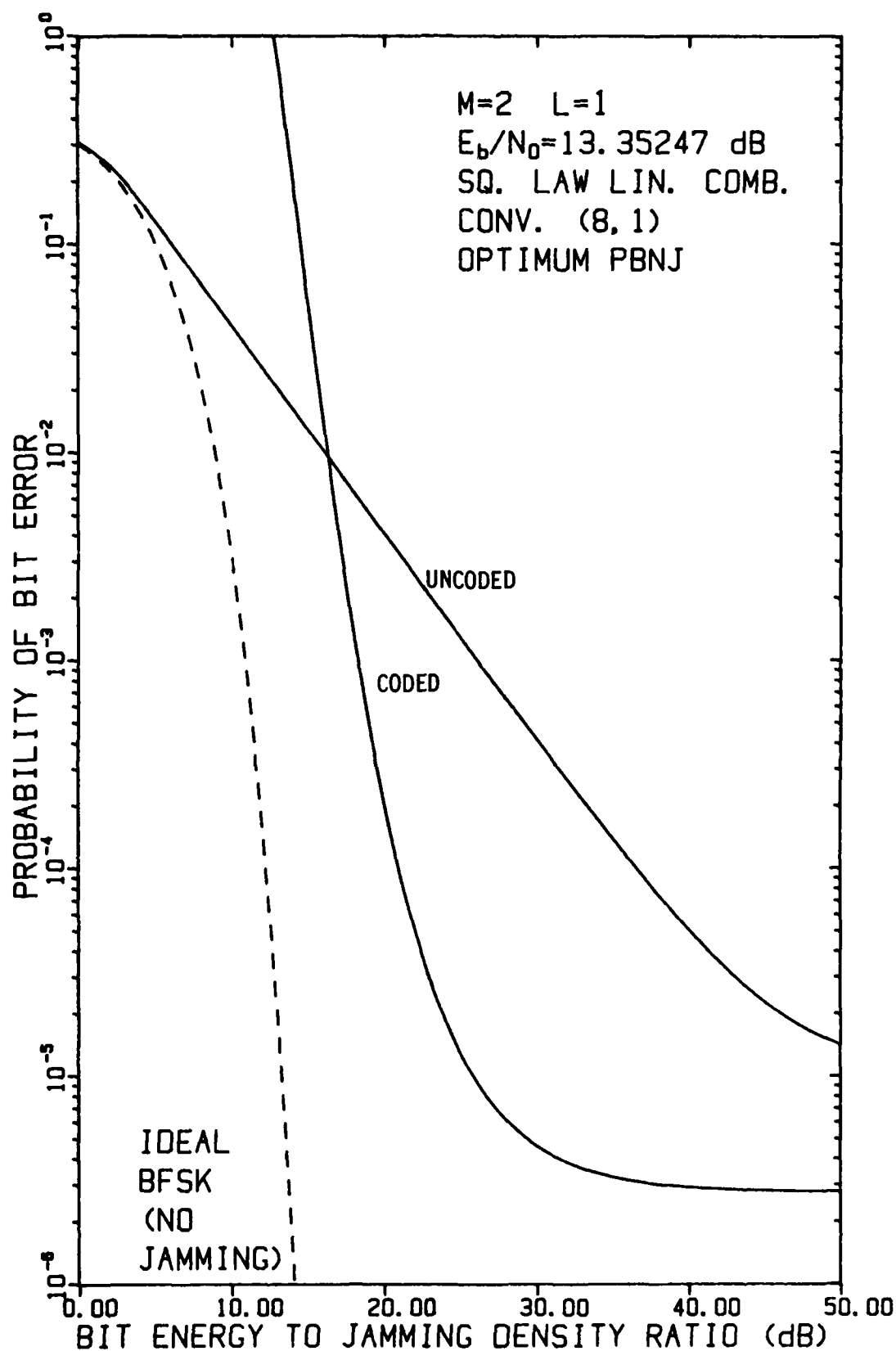
FIGURE 4-61 PERFORMANCE OF FH/BFSK WITH CONVOLUTIONAL RATE-1/8 CODE AND L=1 HOP/DIGIT AS A FUNCTION OF E_b/N_J WHEN E_b/N_0 = 13.35247 dB, USING A LINEAR COMBINING DEMODULATOR, IN OPTIMUM PARTIAL-BAND NOISE JAMMING
