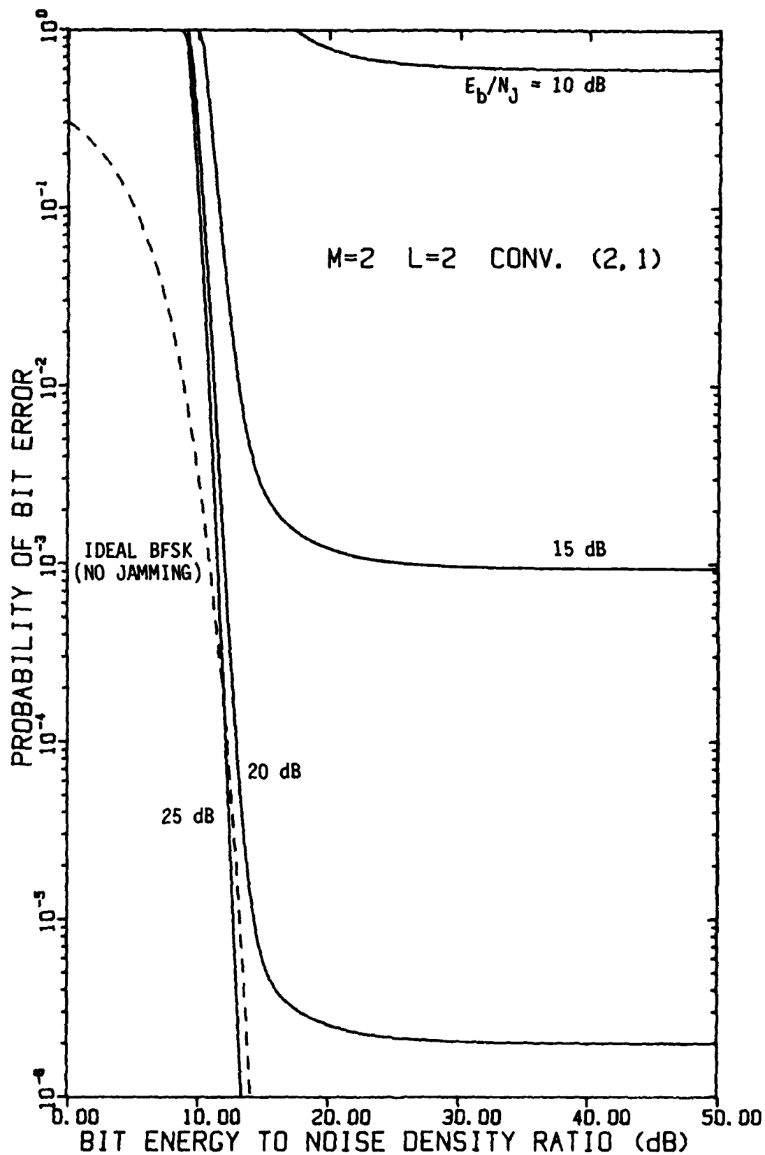
FIGURE 4-46 PERFORMANCE OF FH/BFSK WITH CONVOLUTIONAL RATE-1/2 CODE AND L=2 HOPS/DIGIT AS A FUNCTION OF E_b/N_0 WITH E_b/N_J AS A PARAMETER, USING A LINEAR COMBINING DEMODULATOR, IN OPTIMUM PARTIAL-BAND NOISE JAMMING
