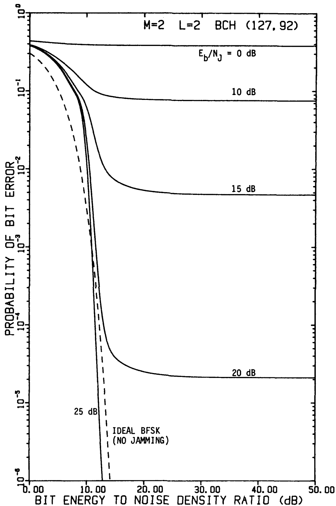
FIGURE 4-22 PERFORMANCE OF FH/BFSK WITH BCH (127,92) CODE AND L=2 HOPS/DIGIT AS A FUNCTION OF E_b/N_0 WITH E_b/N_j AS A PARAMETER, USING A LINEAR COMBINING DEMODULATOR, IN OPTIMUM PARTIAL-BAND NOISE JAMMING
