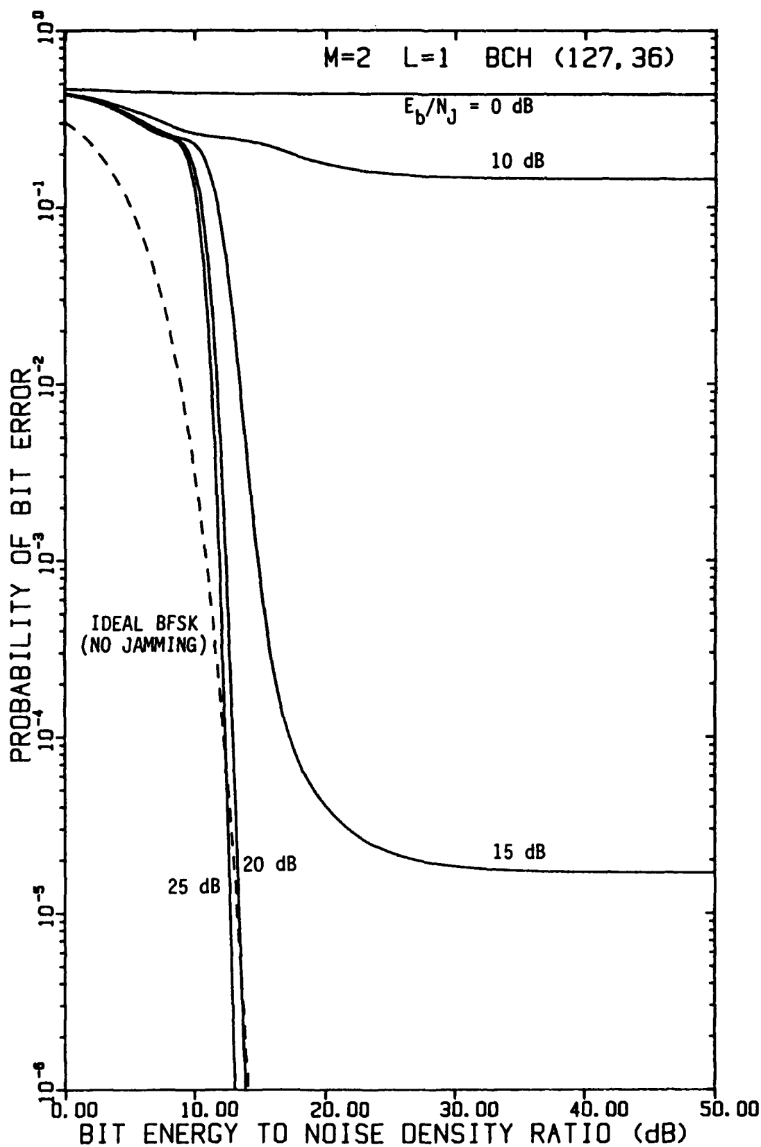
FIGURE 4-37 PERFORMANCE OF FH/BFSK WITH BCH (127,36) CODE AND L=1 HOP/DIGIT AS A FUNCTION OF E_b/N_0 WITH E_b/N_J AS A PARAMETER, USING A LINEAR COMBINING DEMODULATOR, IN OPTIMUM PARTIAL-BAND NOISE JAMMING
