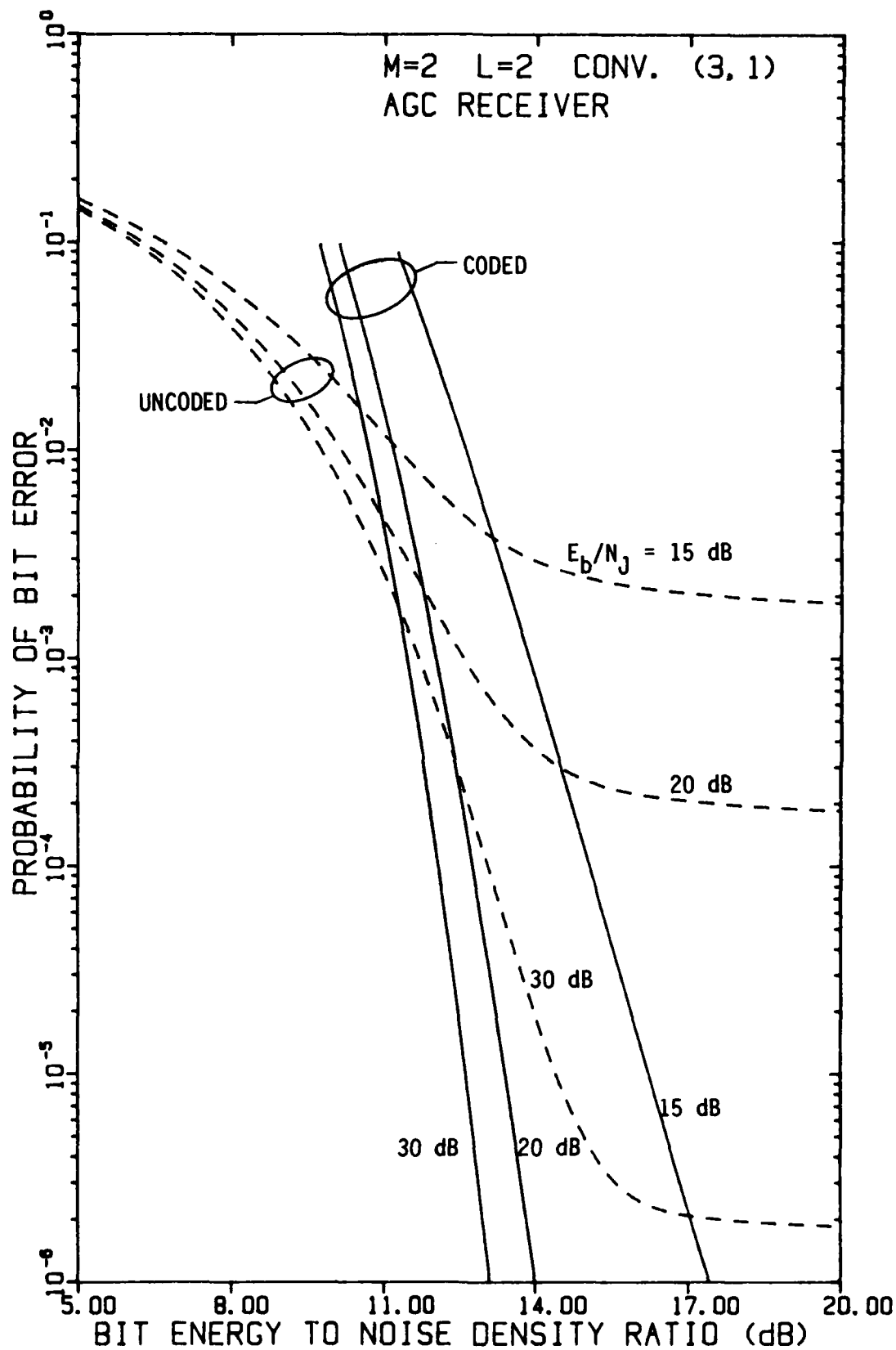
FIGURE 4-99 PERFORMANCE OF FH/BFSK WITH CONVOLUTIONAL RATE-1/3 CODE AND L=2 HOPS/DIGIT AS A FUNCTION OF E_b/N_0 WITH E_b/N_J AS A PARAMETER, USING AN AGC DEMODULATOR, IN OPTIMUM PARTIAL-BAND NOISE JAMMING
