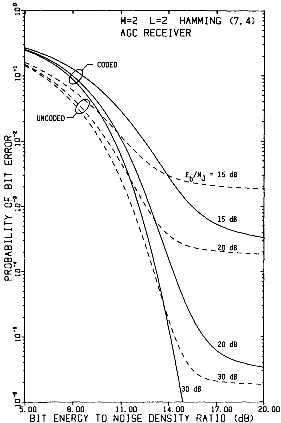
FIGURE 4-71 PERFORMANCE OF FH/BFSK WITH HAMMING (7,4) CODE AND L=2 HOPS/DIGIT AS A FUNCTION OF E_b/N_0 WITH E_b/N_J AS A PARAMETER, USING AN AGC DEMODULATOR, IN OPTIMUM PARTIAL-BAND NOISE JAMMING
