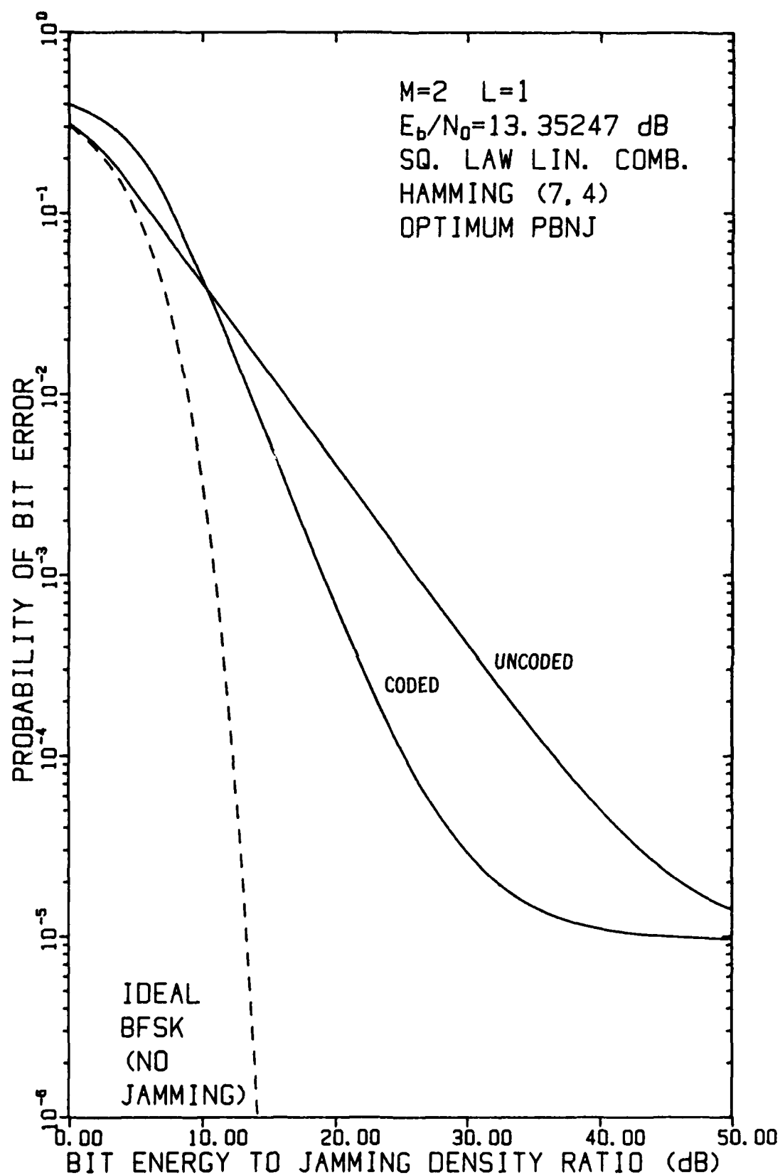
FIGURE 4-9 PERFORMANCE OF FH/BFSK WITH HAMMING (7,4) CODE AND L=1 HOP/DIGIT AS A FUNCTION OF E_b/N_j WHEN E_b/N_0 = 13.35247 dB, USING A LINEAR COMBINING DEMODULATOR, IN OPTIMUM PARTIAL-BAND NOISE JAMMING
