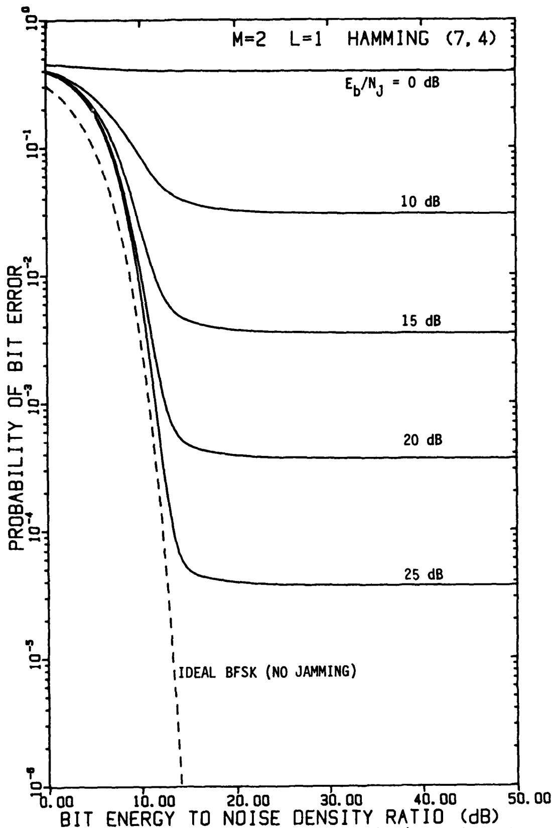
FIGURE 4-5 PERFORMANCE OF FH/BFSK WITH HAMMING (7,4) CODE AND L=1 HOPS/DIGIT AS A FUNCTION OF E_b/N_0 WITH E_b/N_j AS A PARAMETER, USING A LINEAR COMBINING DEMODULATOR, IN OPTIMUM PARTIAL-BAND NOISE JAMMING
