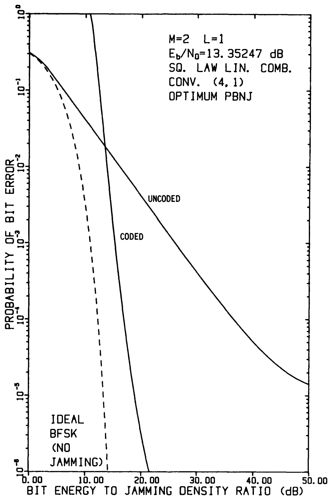
FIGURE 4-57 PERFORMANCE OF FH/BFSK WITH CONVOLUTIONAL RATE-1/4 CODE AND L=1 HOP/DIGIT AS A FUNCTION OF E_b/N_j WHEN E_b/N_0 = 13.35247 dB, USING A LINEAR COMBINING DEMODULATOR, IN OPTIMUM PARTIAL-BAND NOISE JAMMING
