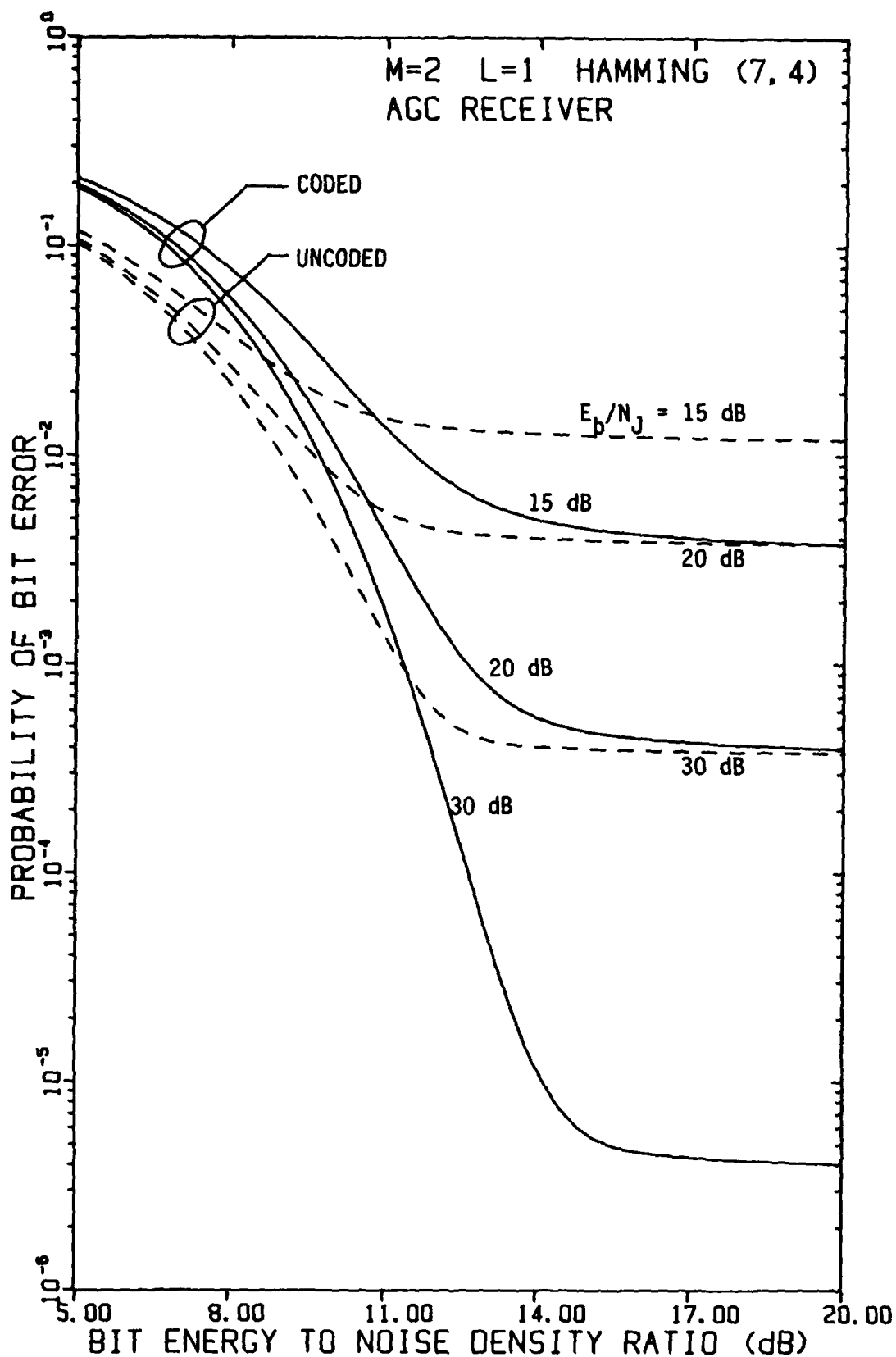
FIGURE 4-70 PERFORMANCE OF FH/BFSK WITH HAMMING (7,4) CODE AND L=1 HOP/DIGIT AS A FUNCTION OF E_b/N_0 WITH E_b/N_J AS A PARAMETER, USING AN AGC DEMODULATOR, IN OPTIMUM PARTIAL-BAND NOISE JAMMING
