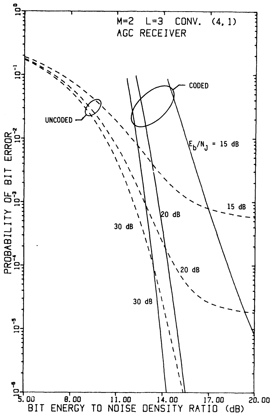
FIGURE 4-104 PERFORMANCE OF FH/BFSK WITH CONVOLUTIONAL RATE-1/4 CODE AND L=3 HOPS/DIGIT AS A FUNCTION OF E_b/N_0 WITH E_b/N_j AS A PARAMETER, USING AN AGC DEMODULATOR, IN OPTIMUM PARTIAL-BAND NOISE JAMMING
