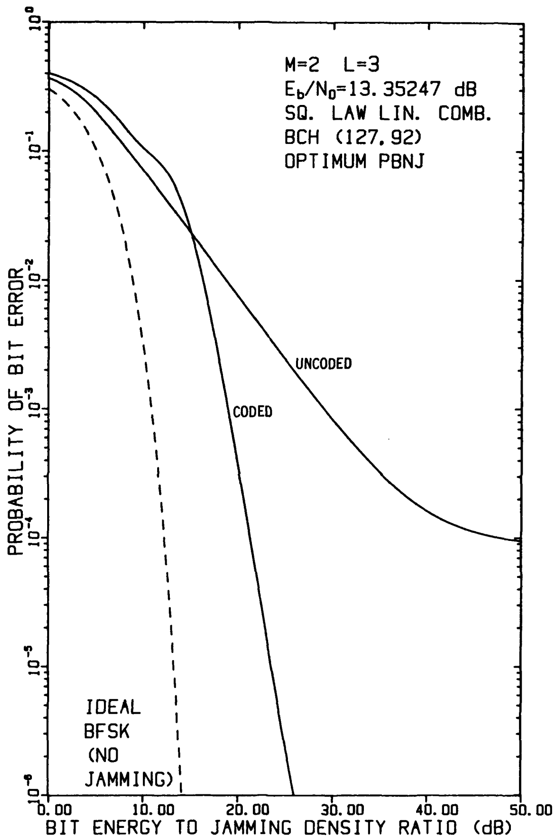
FIGURE 4-27 PERFORMANCE OF FH/BFSK WITH BCH (127,92) CODE AND L=3 HOPS/DIGIT AS A FUNCTION OF E_b/N_J WHEN E_b/N_0 = 13.35247 dB, USING A LINEAR COMBINING DEMODULATOR, IN OPTIMUM PARTIAL-BAND NOISE JAMMING
