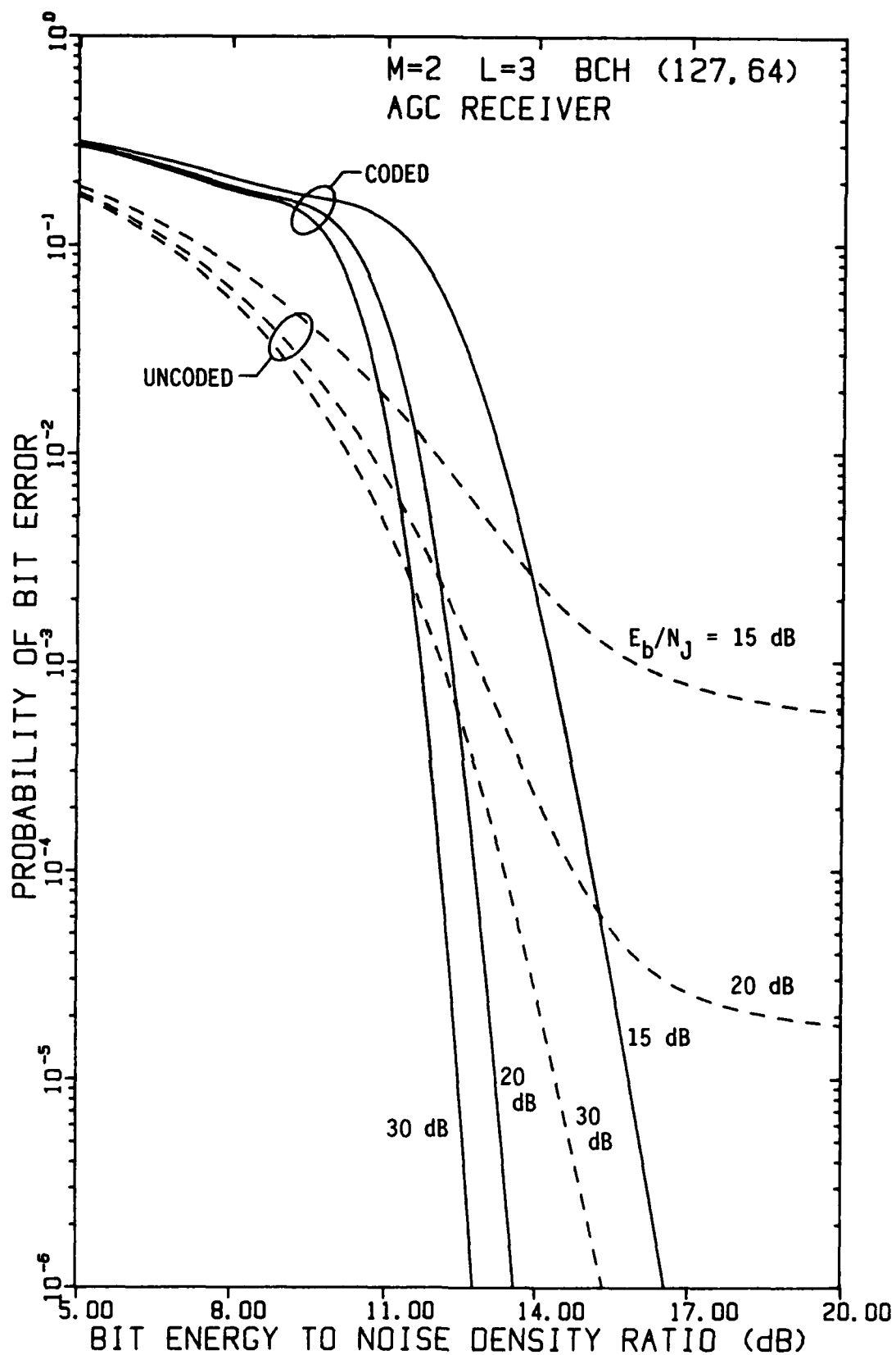
FIGURE 4-84 PERFORMANCE OF FH/BFSK WITH BCH (127,64) CODE AND L=3 HOPS/DIGIT AS A FUNCTION OF E_b/N_0 WITH E_b/N_j AS A PARAMETER, USING AN AGC DEMODULATOR, IN OPTIMUM PARTIAL-BAND NOISE JAMMING
