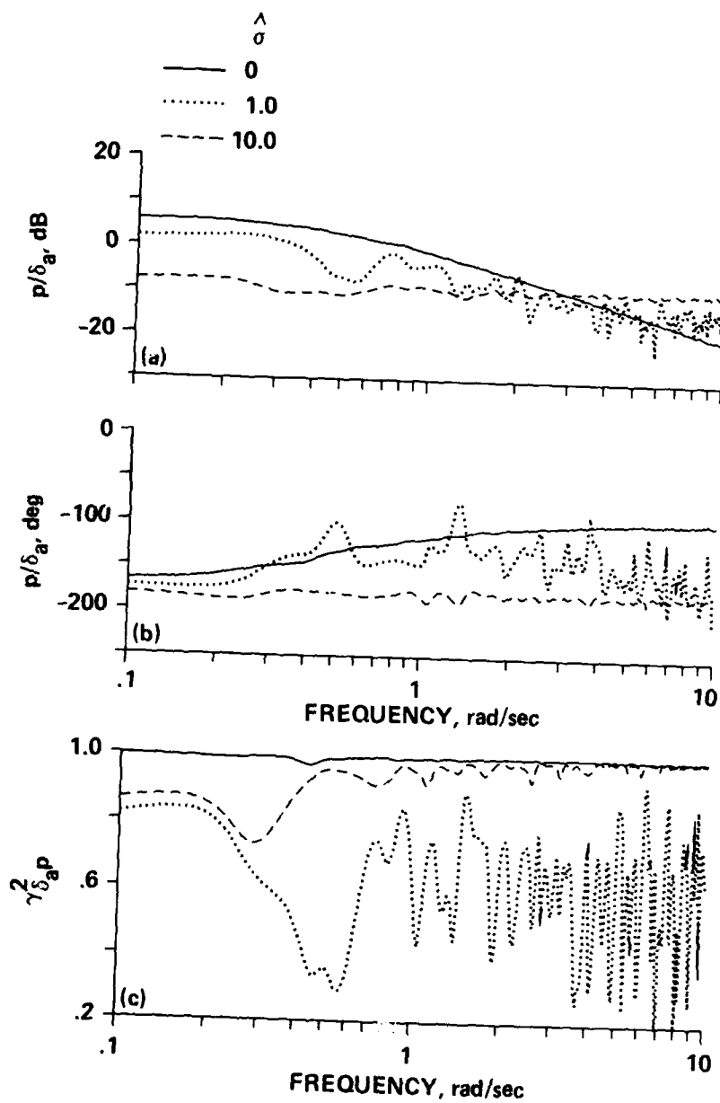
Fig. B.11. Effect of Noise-to-Signal Ratios \hat{\sigma} = 0, 1.0, 10.0 on the Identification of the Open-Loop Frequency-Response for the Nominal-System, \kappa = 3.0 . (a) Magnitude; (b) Phase; (c) Coherence.
