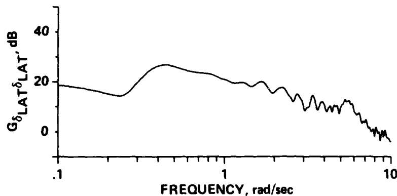
Fig. 4.2. Lateral-Stick Input Autospectrum ( G_{\delta_{LAT}}^2 ).
