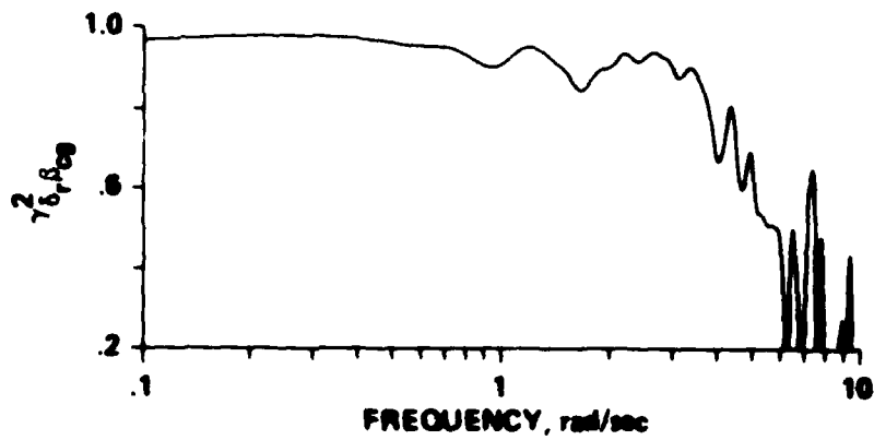
Fig. 5.5. Coherence Function ( \gamma^2_{\delta_r, \beta_{cg}} ) for Sideslip Response Identification.
