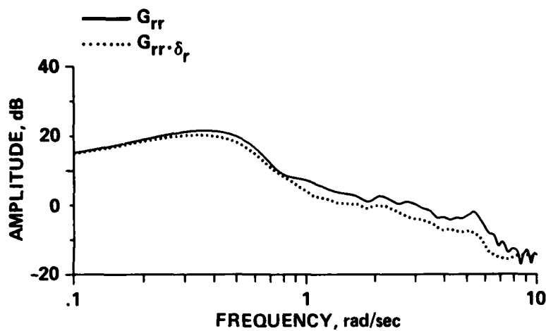
Fig. 4.18. Yaw-Rate Output Autospectrum.
