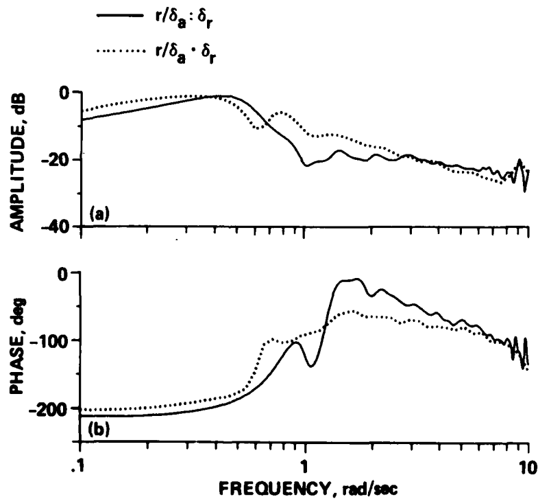
Fig. 4.19. Magnitude of Cross-Spectrum between Aileron Surface Inputs and Yaw-Rate Response.
