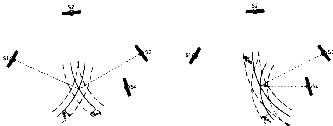
Figure 8 : Angle of intersection of the two lines of position and its influence to positioning (two examples)
