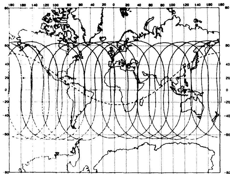
Figure 3 : SATELLITE-NO. 3, 6, 8, 9, 11, 12, 13 SUBSATELLITE TRACK OF GPS-SATELLITES DATE : 10 6 1986
