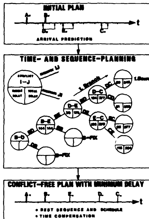
Figure 7: COMPAS-planning algorithm (Schematic)
