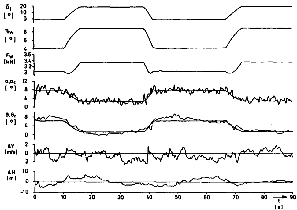
fig.7 Altitude and speed hold at flap setting
