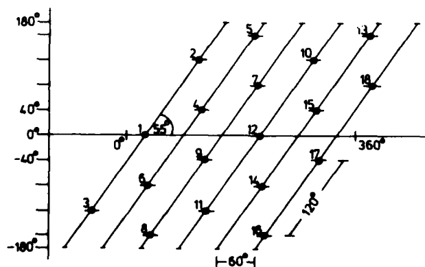
Figure 5 : Arrangement of the satellites
