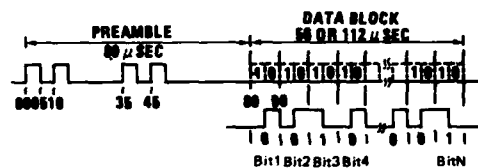
Fig 2-d MODE S REPLY
