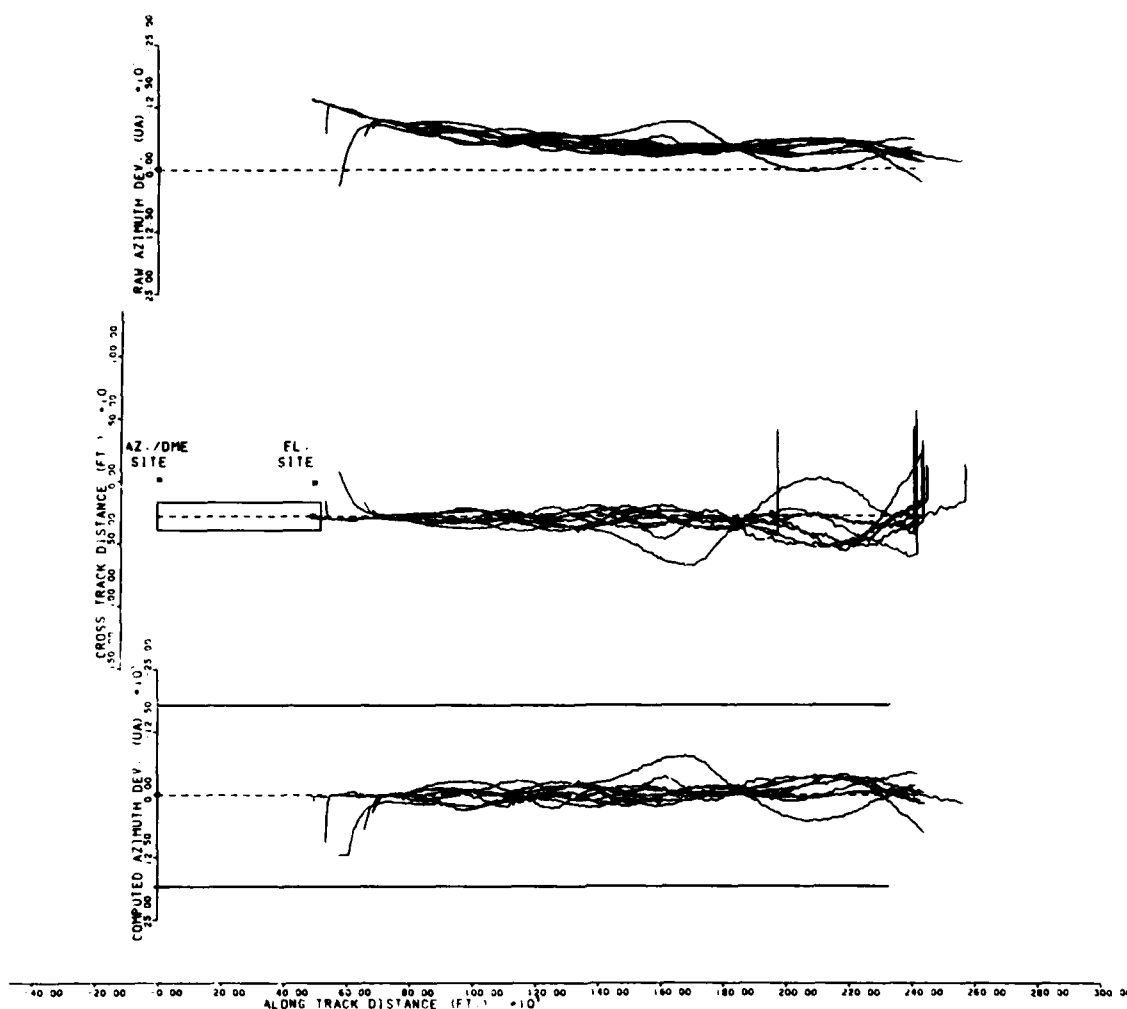
FIGURE 11. RAW AZIMUTH, COMPUTED AZIMUTH AND CROSSTRACK DEVIATIONS
