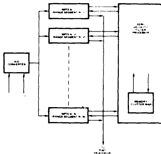
Fig 4.1 - MTD PROCESSOR ARCHITECTURE
