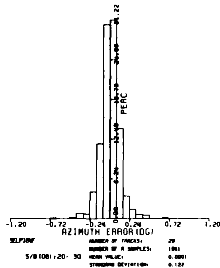
Fig 5.7 - AZIMUTH ERROR HISTOGRAM
