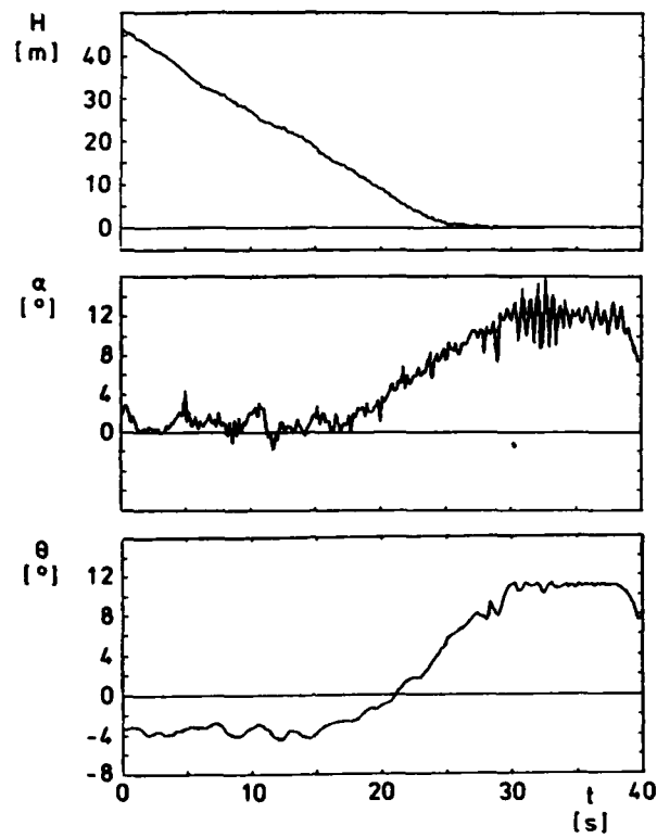
fig.9 Automatic landing (flap position \delta_e = 52^\circ )
