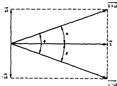
Fig 6b PHASE RECEIVER PRINCIPLE
