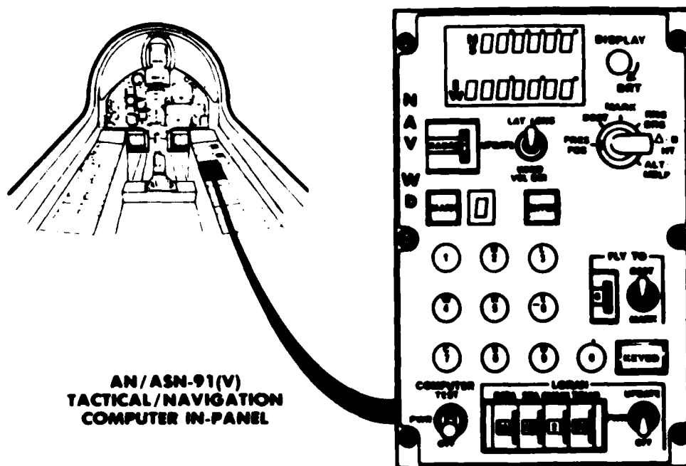
FIGURE 3. A-7E PILOTS CONTROL AND DISPLAY
