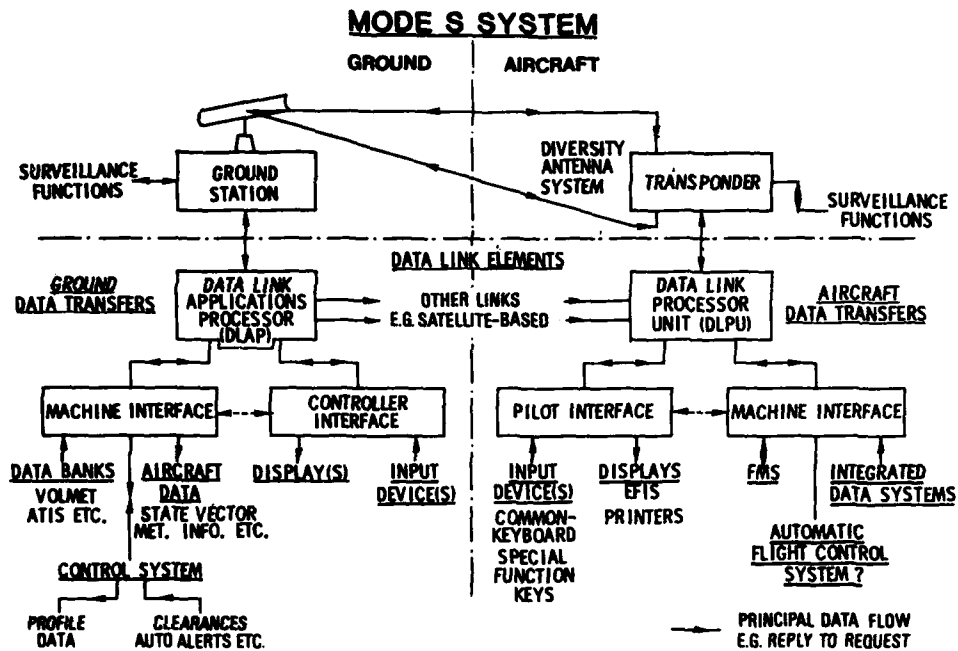
FIG. 3 - SSR MODE S - FUNCTIONAL ELEMENTS AND DATA INTERFACES
