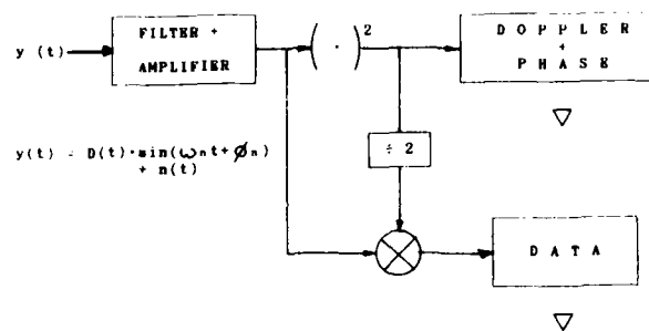
Figure 15 : Squaring Loop
