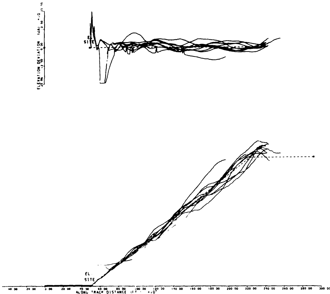
FIGURE 12. VERTICAL POSITION AND ELEVATION DEVIATIONS
