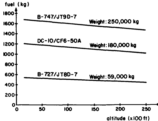
Fig.6 - FUEL PENALTY RESULTING FROM A 10-MIN HOLDING.
