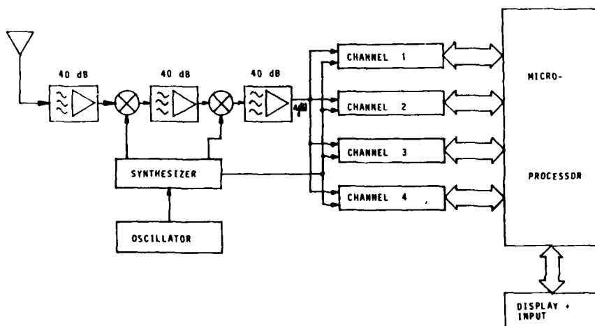
Figure 13 : Receiver Block-Diagram
