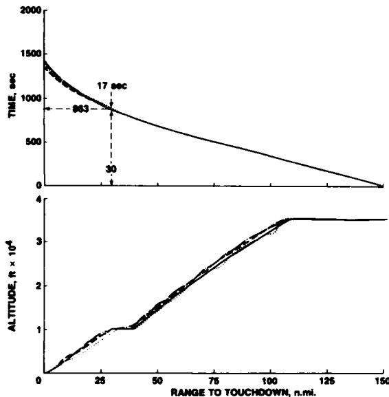
Fig. 7. Fast descents: 0.84/350.
