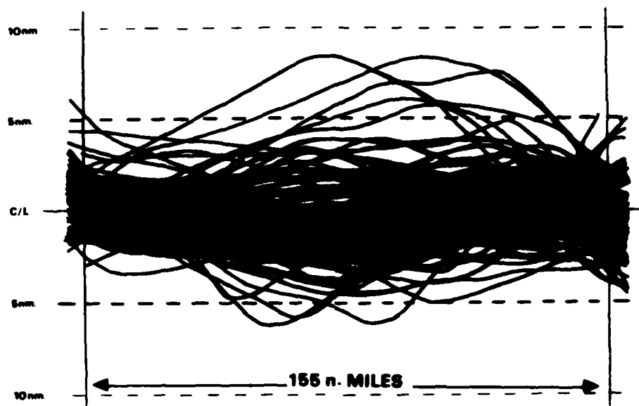
FIG 2. OBSERVED ON AIRWAY PERFORMANCE USING VOR.
