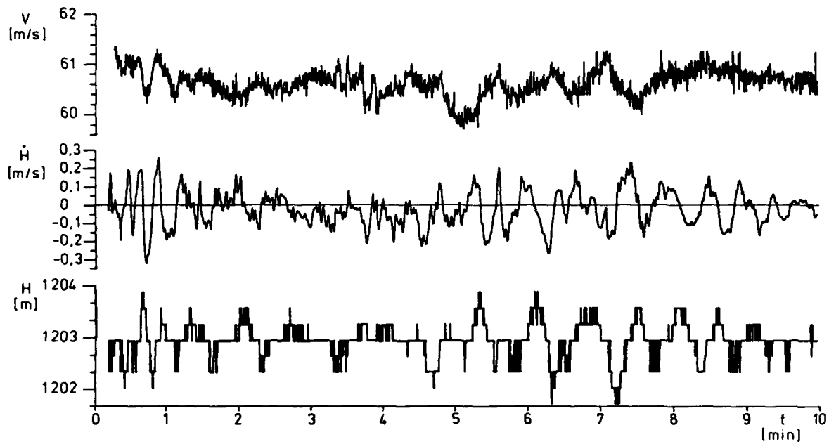
fig.5 Altitude and speed hold (calm air)
