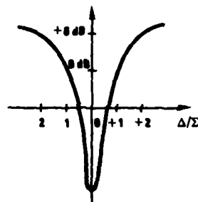
Fig 6a AMPLITUDE RECEIVER CURVE
