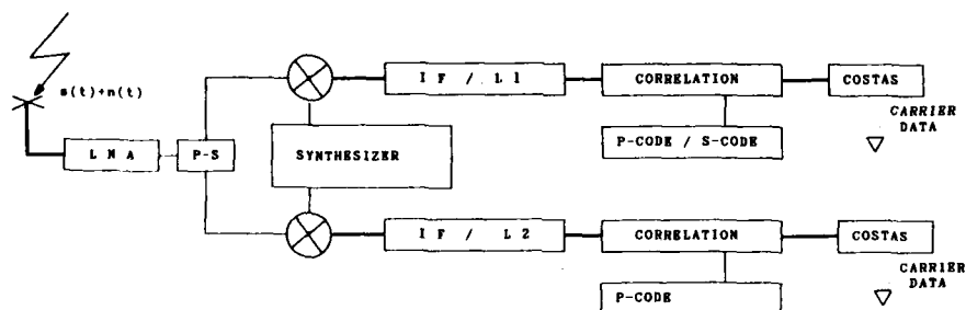
Figure 12: Satellite Signals with Block-Diagram
