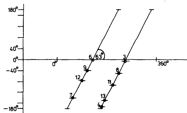
Figure 1 : Present satellite orbit configuration
