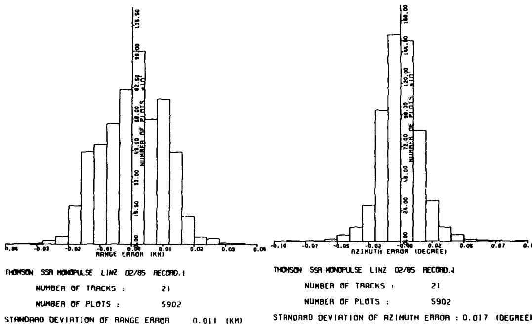
Fig 18 - HISTOGRAM OF RANGE ERROR AND AZIMUTH ERROR
