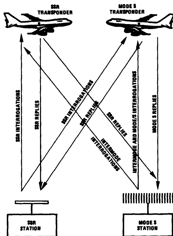
Fig 1 COMPATIBILITY BETWEEN SSR AND MODES
