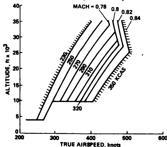
Fig. 4. Speed profiles for time control.
