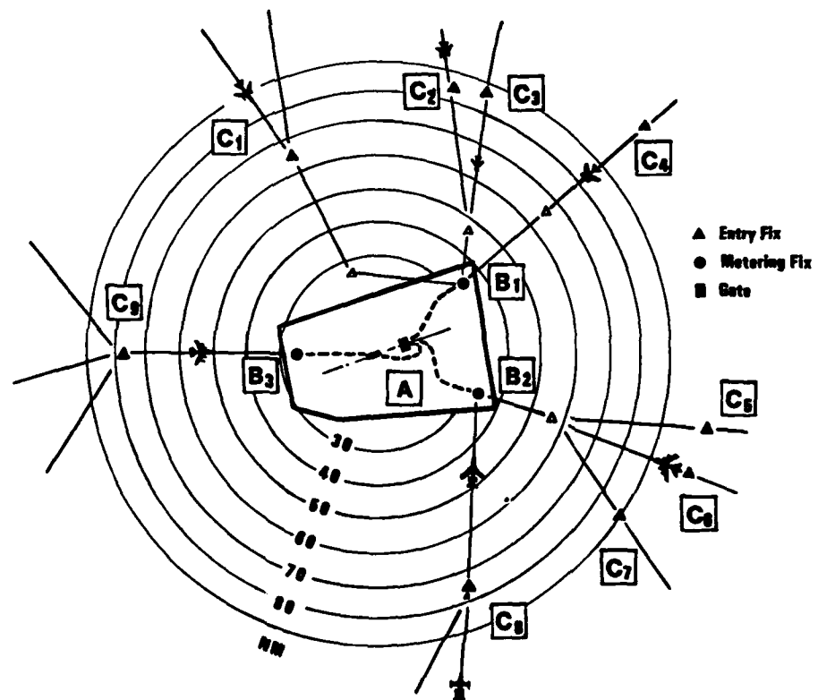
Figure 2: Structure of the Frankfurt Approach Area
