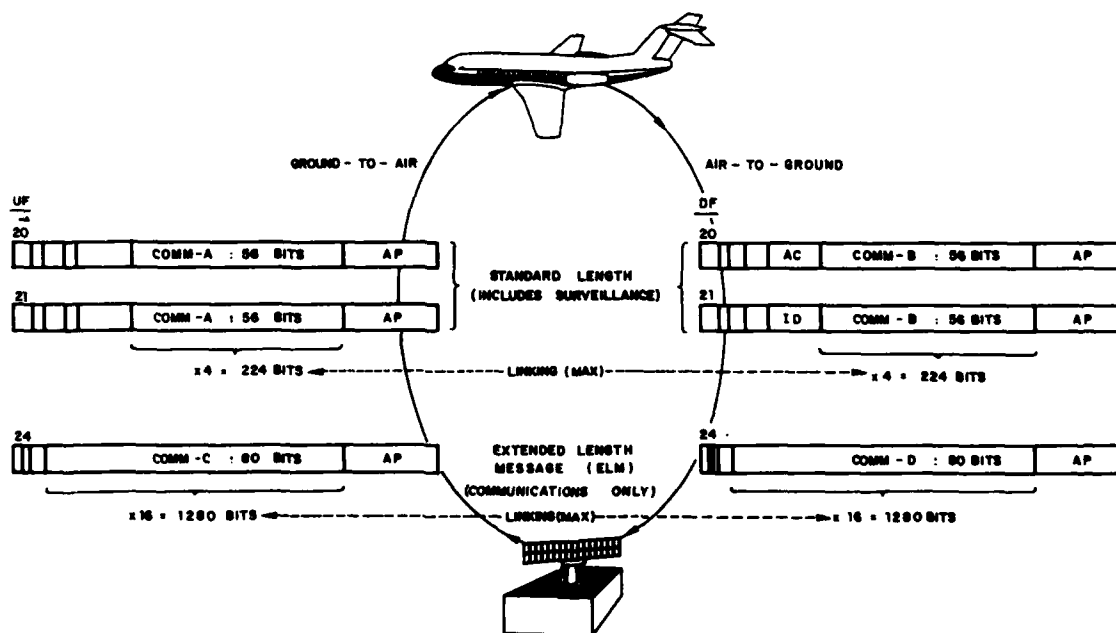
FIG. 2 - SSR MODE S - MESSAGE FORMATS AND DATA LINK FIELDS
