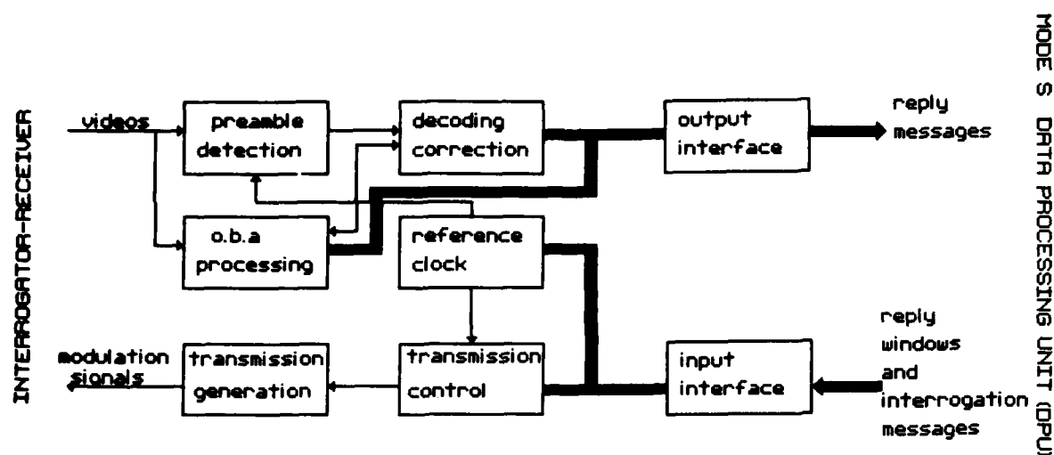
FIG.20 MODE S PROCESSING INTERFACE
