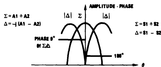
SUM AND DIFFERENCE PATTERNS - 3C
