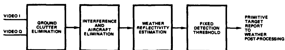
Fig 3.4 - BLOCK DIAGRAM OF WEATHER SIGNAL PROCESSING
