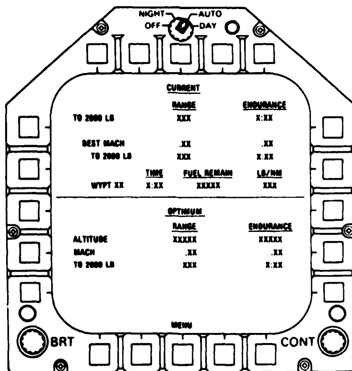
FIGURE 2. F/A-18 FPAS DIGITAL DISPLAY INDICATOR (DDI)
