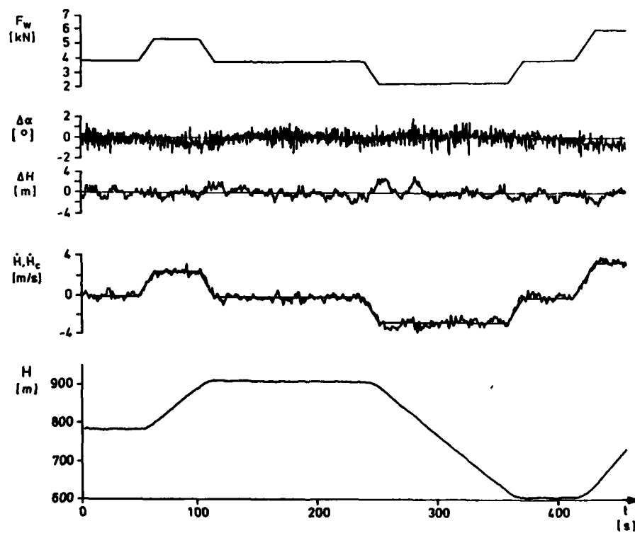
fig.8 Altitude acquire (strong turbulence)
