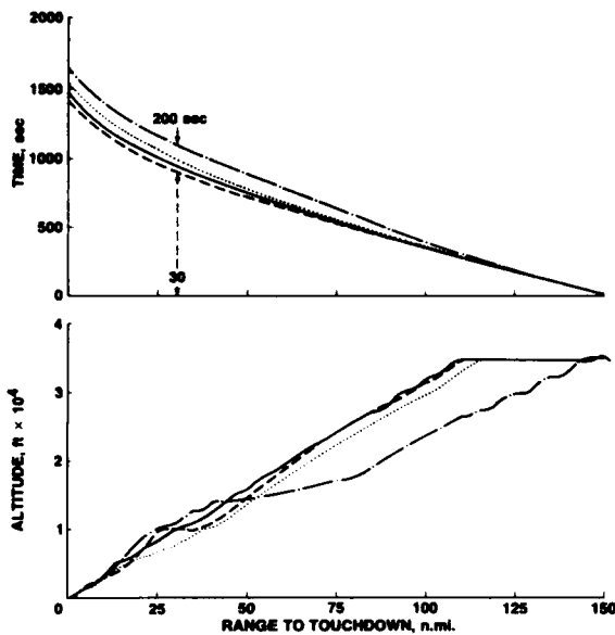
Fig. 5. Baseline descents.
