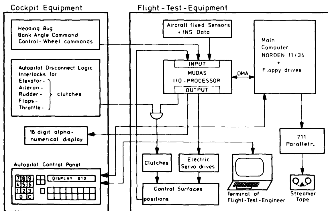
fig.4 Equipment of the D0-28 research aircraft
