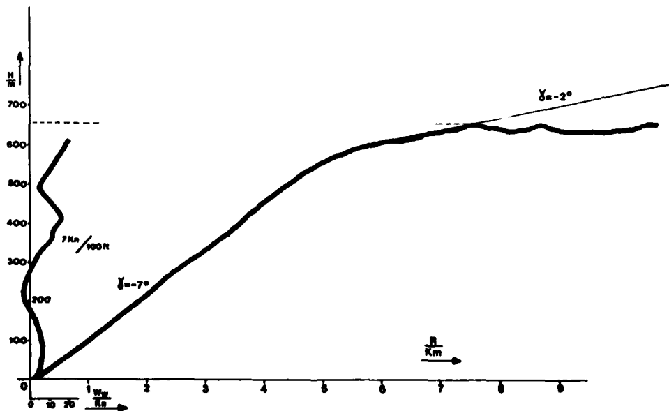
fig.10 Curved MLS approach (passing a moderate windshear)
