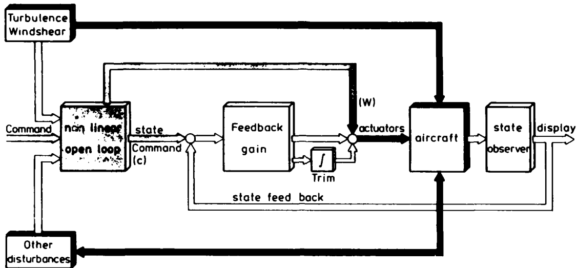
fig.1 Block diagramm of the control loops
