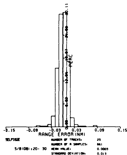
Fig 5.6 - RANGE ERROR HISTOGRAM
