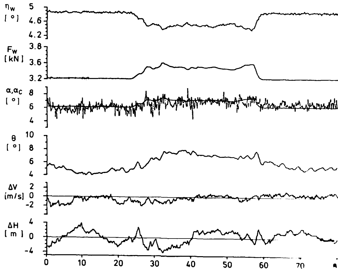
fig.6 Altitude and speed hold in turn flight (moderate)
