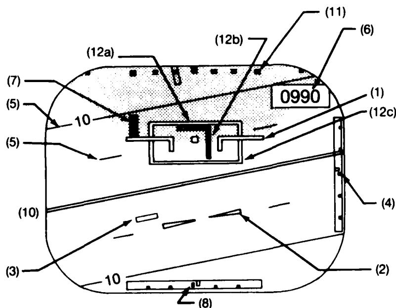
Fig. 8 EADI landing symbology
