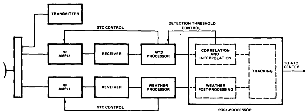
Fig 2.1 - BLOCK DIAGRAM OF ATC AND WEATHER CHANNELS
