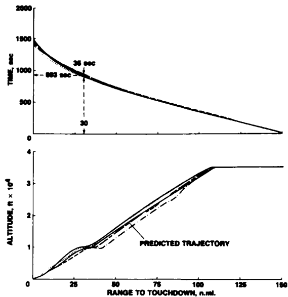
Fig. 6. Nominal descents: 0.8/320.
