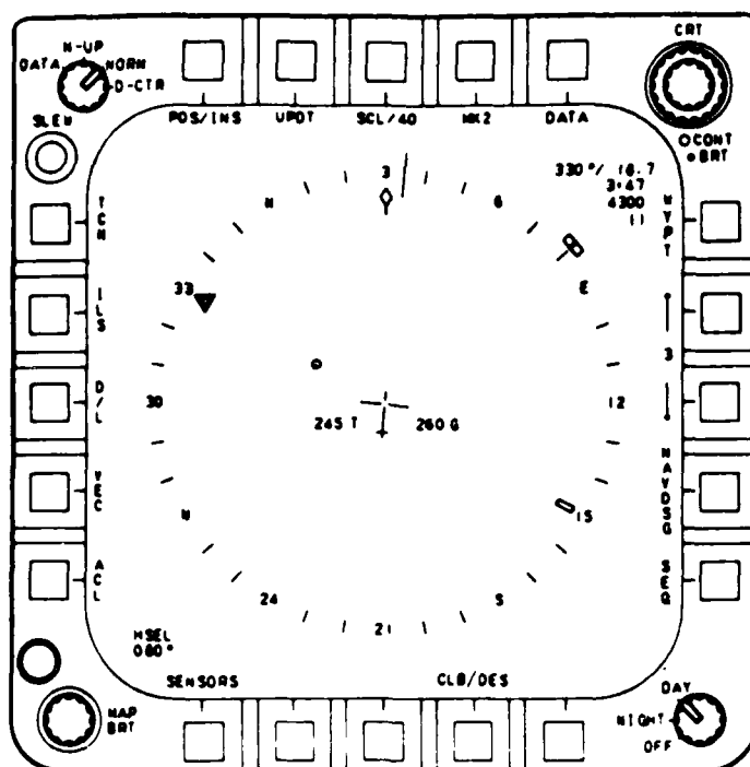
FIGURE 1. F/A-18 HORIZONTAL SITUATION DISPLAY (HSD)
