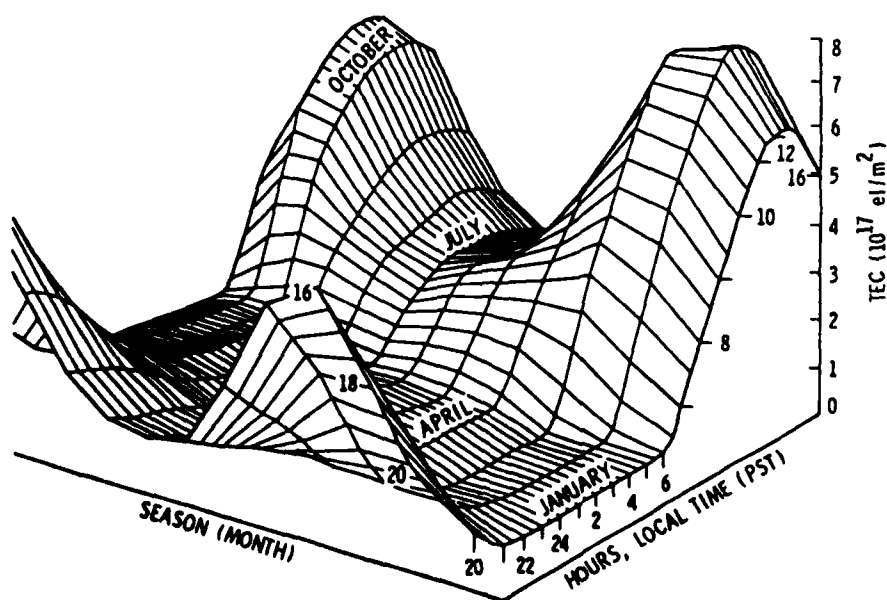
Figure 11 : 1979 Monthly Average of Total Electron Columnar Content Profile for Goldstone, Ca.
