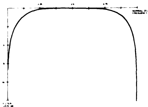
Fig 3.5 - EXAMPLE OF GROUND CLUTTER FILTER
