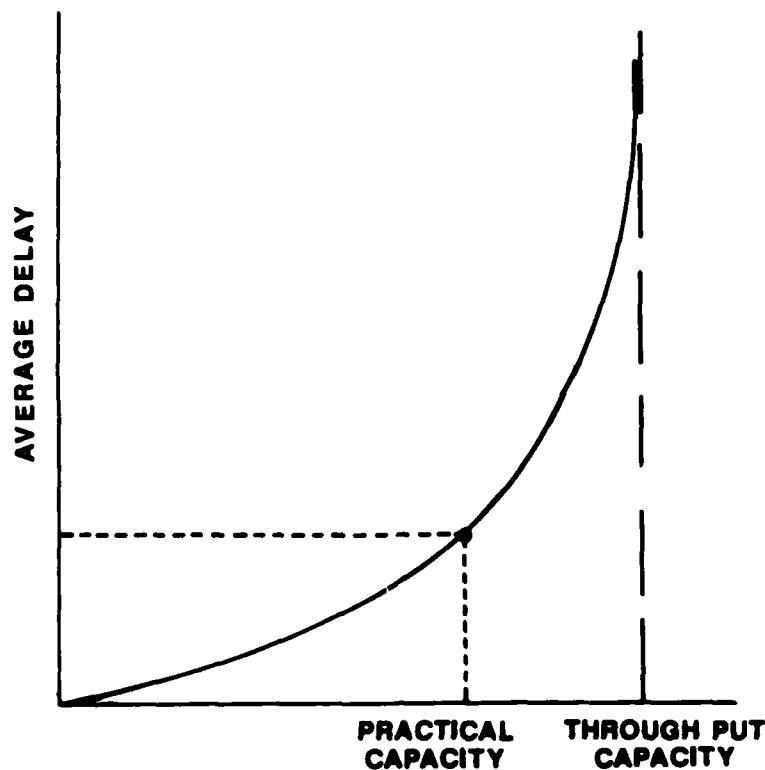
Figure 1. - Relationship between Capacity and Delay.
