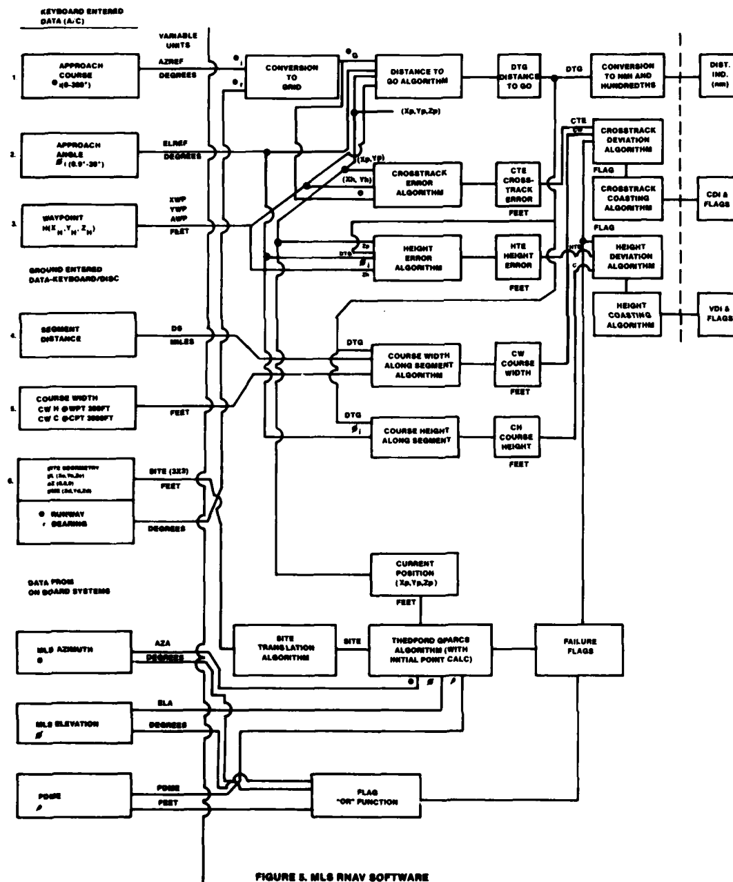
FIGURE 5. MLS RNAV SOFTWARE
