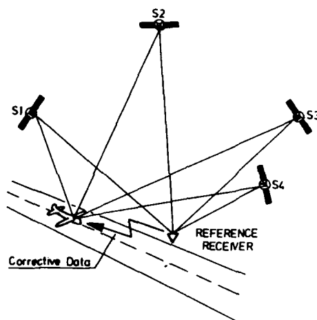
Figure 10 : Differential GPS-Measurement
