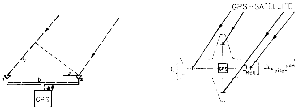
Figure 18 : Interferometric Principle for attitude control
