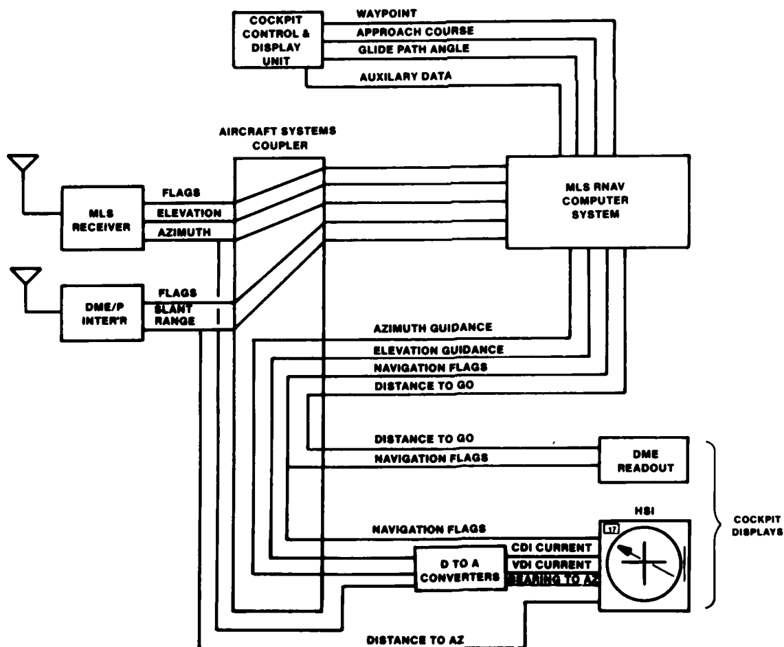
FIGURE 4. MLS RNAV SYSTEM BLOCK DIAGRAM
