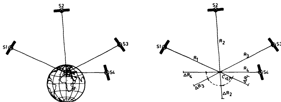
Figure 6 : Pseudo-ranging concept
