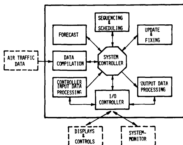
Figure 5: COMPAS data-processing functions
