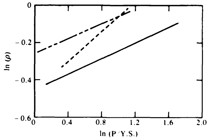
Figure 12. Variation of \ln (density) with \ln (pressure/yield stress) for (————) aluminum, (-----) Al-3Li-1Cu-1Mg-0.2, and (— · — · —) Al-8Fe-7Ce alloy powders.
