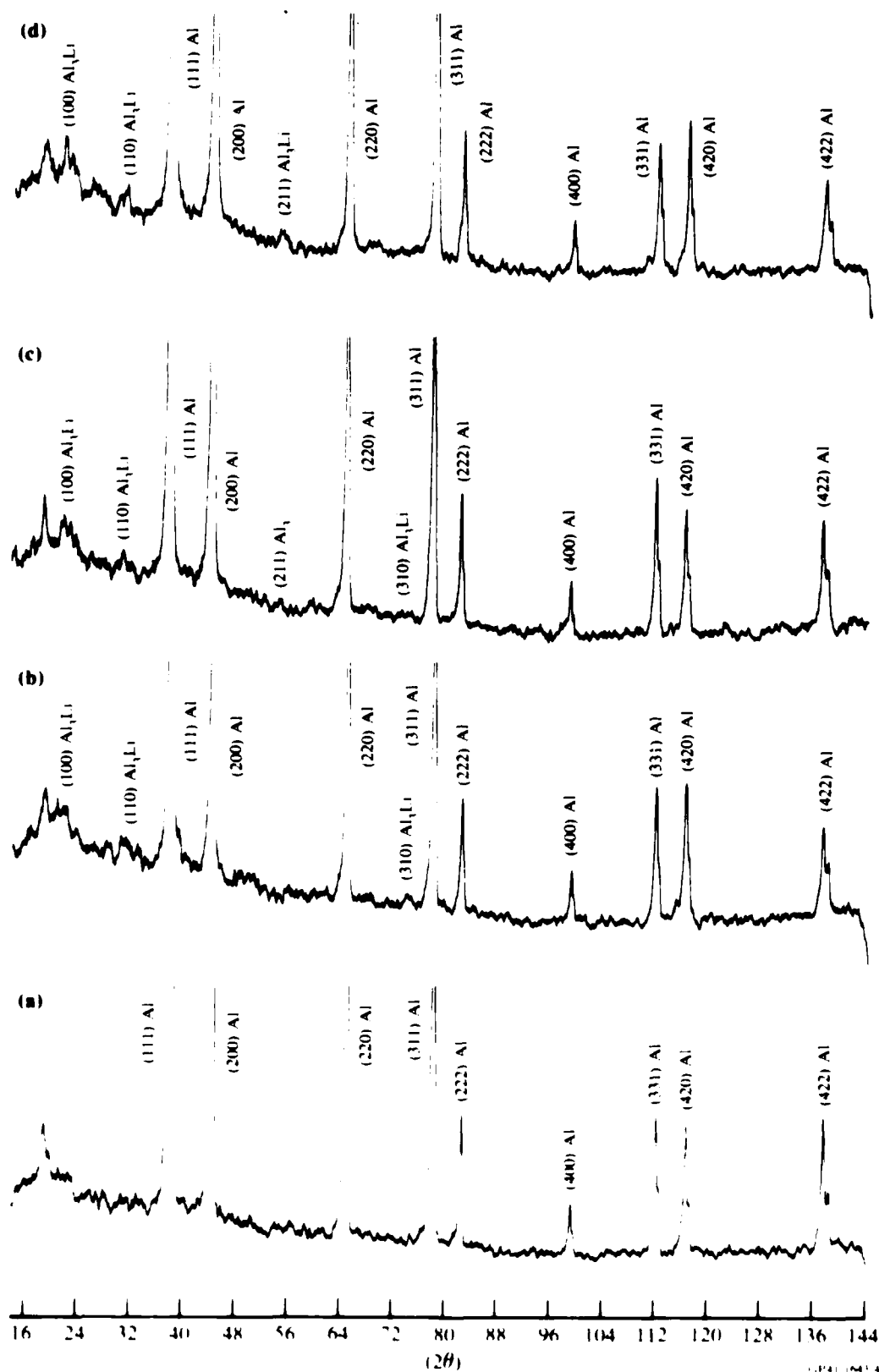
Figure 4. X-ray diffraction peaks of (a) aluminum, (b, c, and d) Al-31.1-1Cu-1Mg-0.2Zr alloy, (b) rapidly solidified, (c) annealed at 400°C for 2 h, and (d) annealed at 500°C for 2 h.
