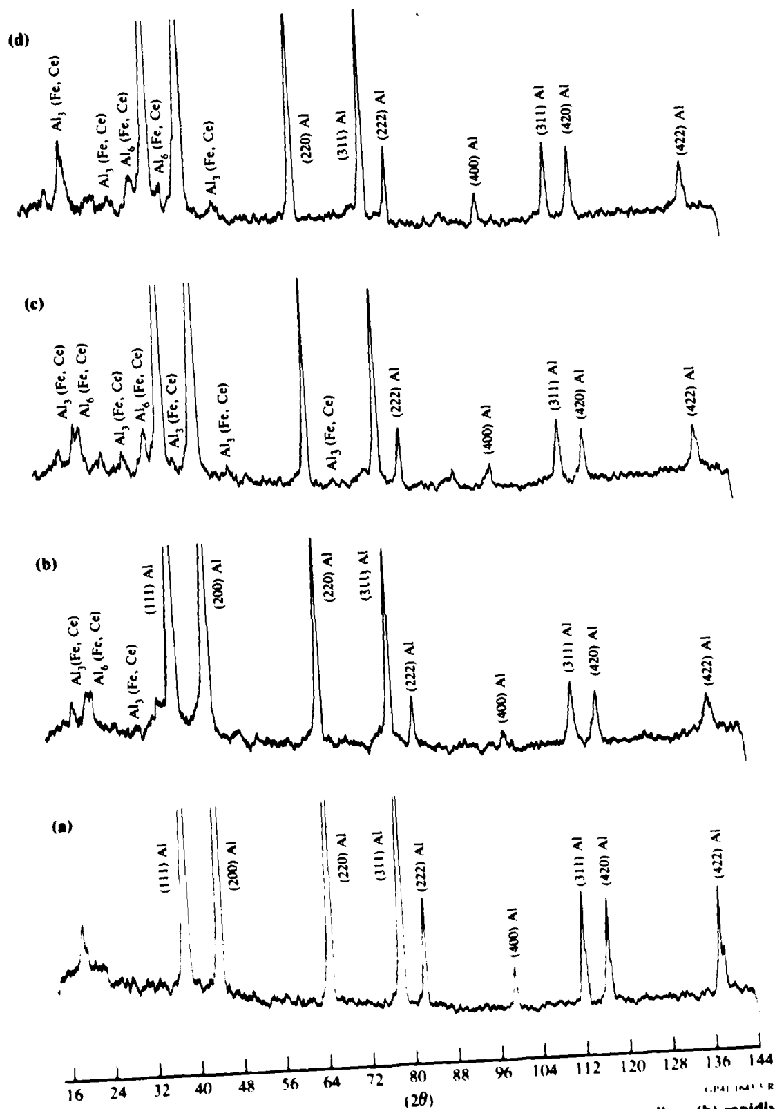
Figure 5. X-ray diffraction peaks of (a) aluminum, (b, c, and d) Al-8Fe-4Ce alloy, (b) rapidly solidified, (c) annealed at 400^\circ\text{C} for 2 h, and (d) annealed at 500^\circ\text{C} for 2 h.
