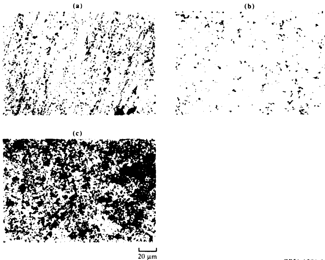
Figure 42. Optical micrographs of explosive compacts of (a) 99.9% Al, (b) Al-3Li-1Cu-1Mg-0.2Zr, and (c) Al-8.4Fe-7Ce alloys.
