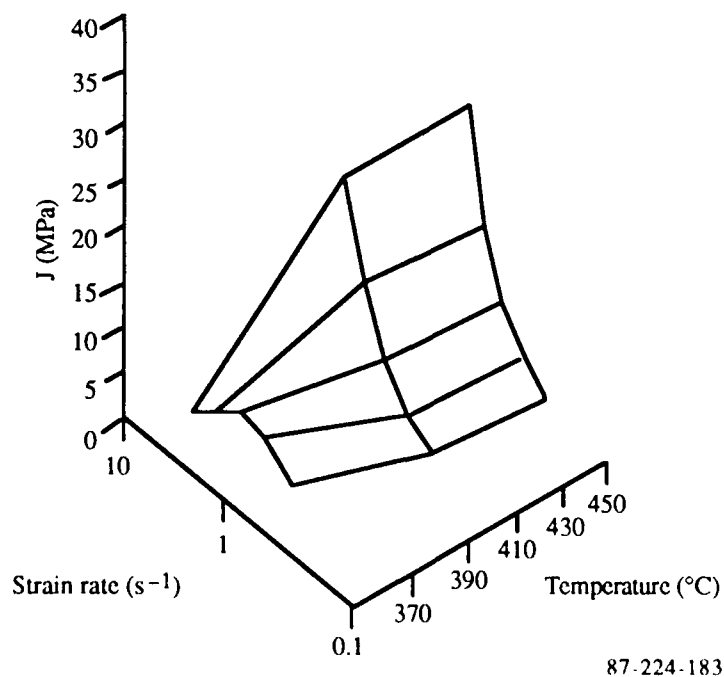
Figure 48. Effect of isothermal extrusion temperature and strain rate on co-content J of Al-3Li-1Cu-1Mg-0.2Zr.
