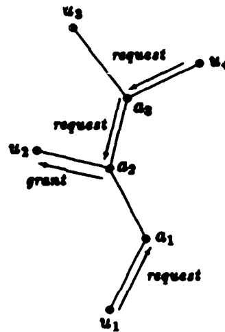
Figure 3.2: One state of the arbiter modeled by A_1 .
