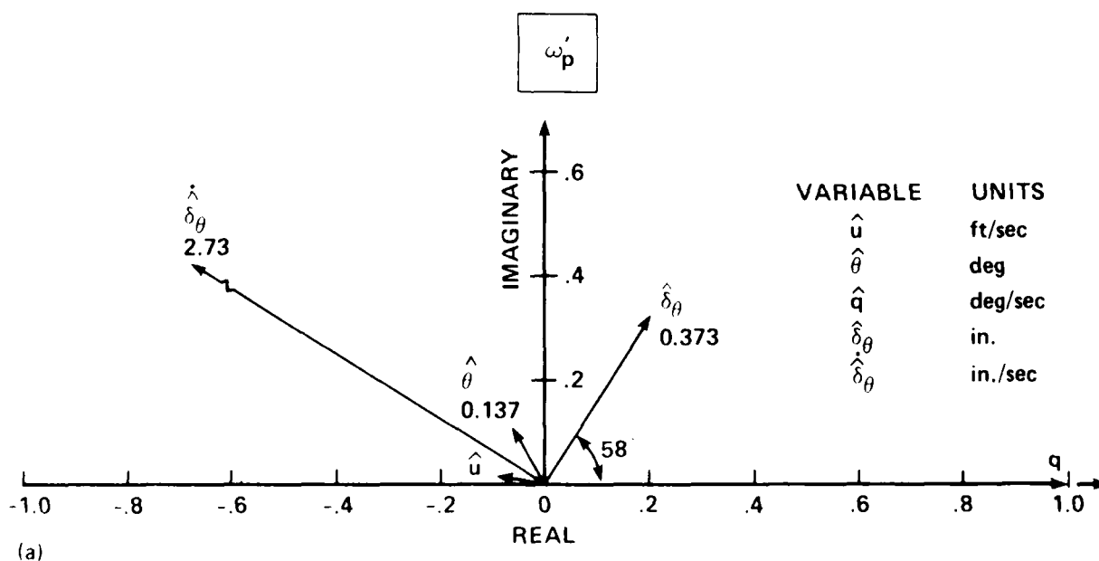
Figure 22.- Dynamics of the closed-loop complex mode ( \omega'_p ). (a) Eigenvector diagram; (b) time-vector diagram.
