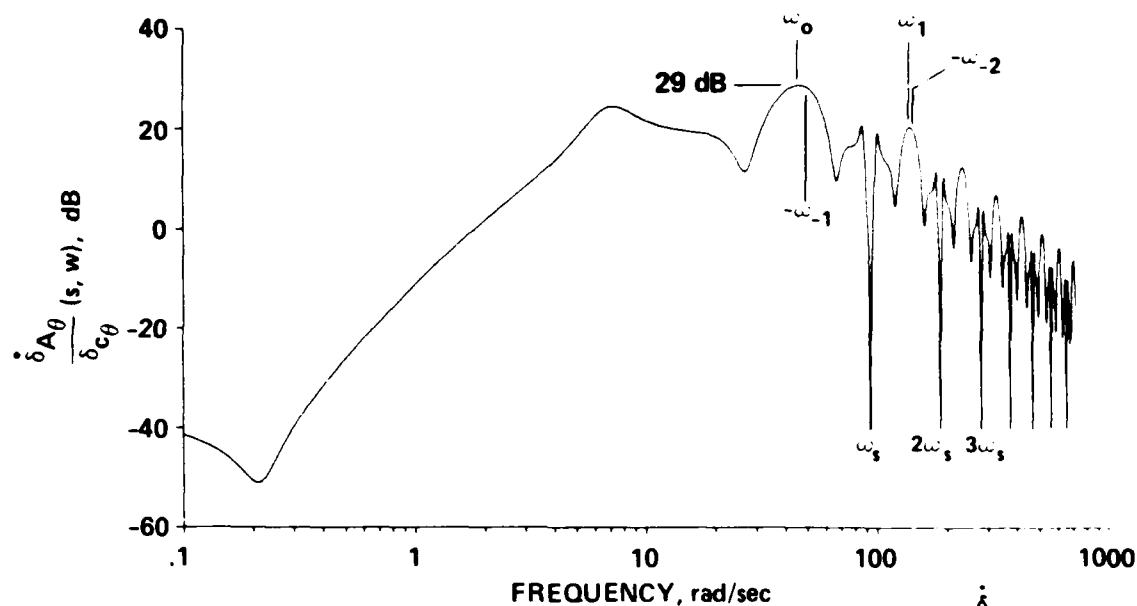
Figure 59.- Hybrid frequency response of the actuator rate \frac{\delta A_\theta(s, w)}{\delta c_\theta} (15 Hz system).
