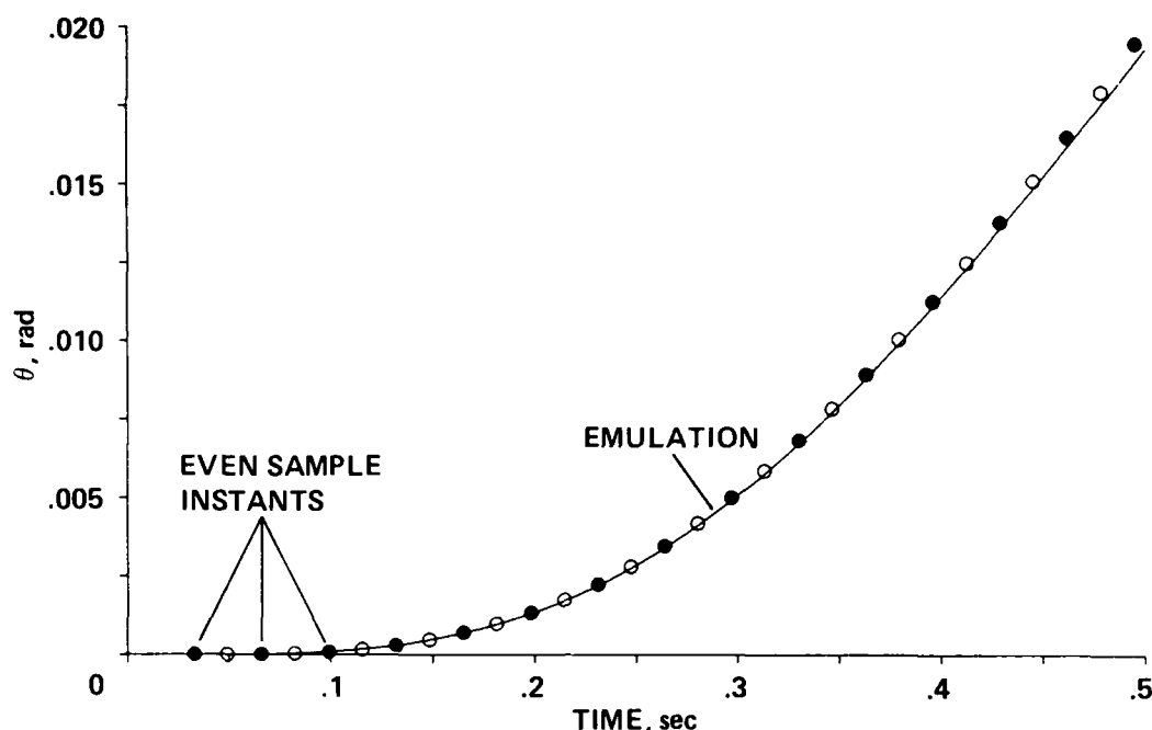
Figure 49.- Pitch attitude response ( \theta ) to a step input, \delta_{c0} = 1 ; digital and emulation analyses (30.3 Hz system).
