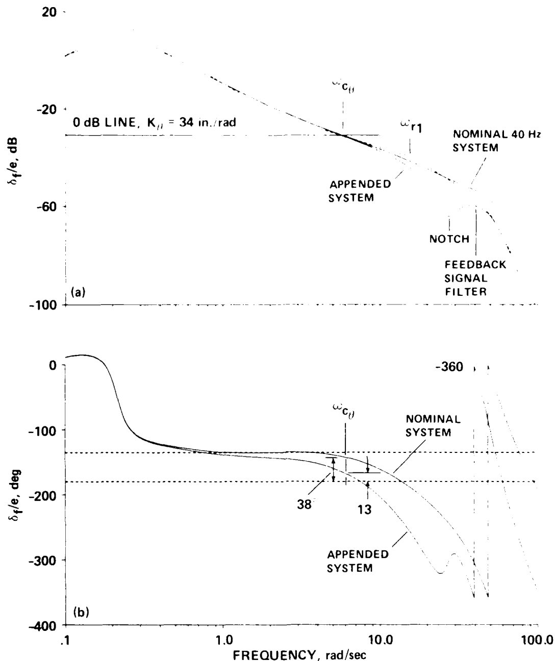
Figure 32.- Effect of appended system dynamics on the nominal design. (a) Magnitude; (b) phase.
