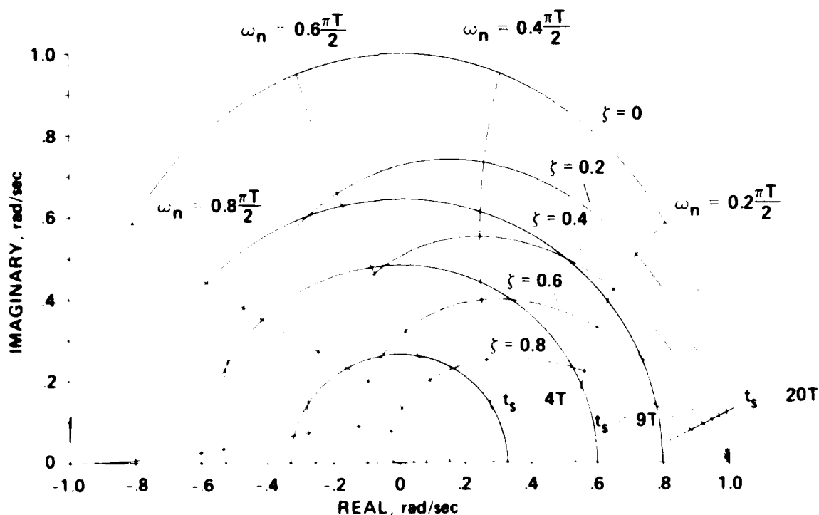
Figure 11.- Mappings of s -plane contours on the z -plane.
