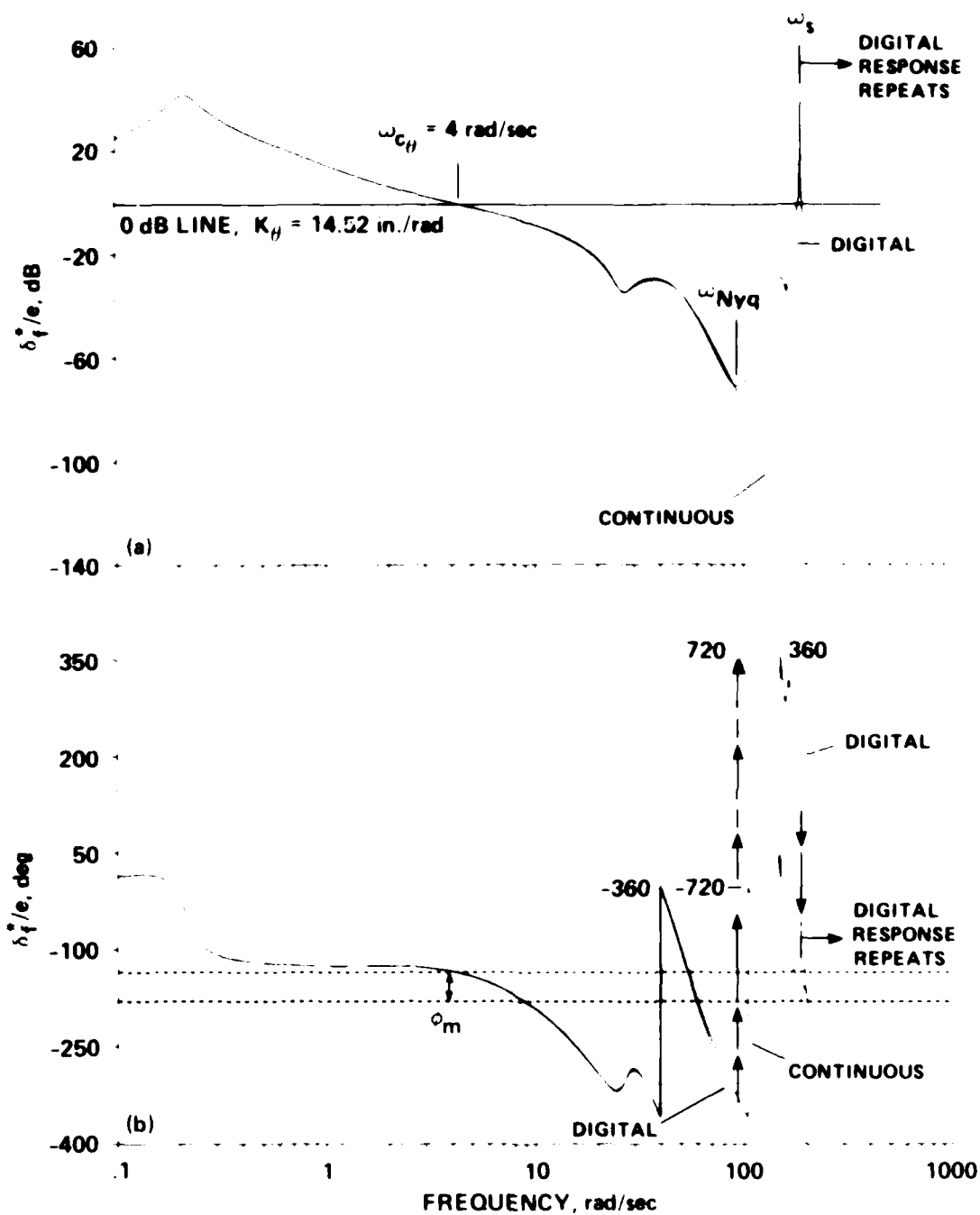
Figure 43.- Equalized open-loop frequency response of s_f/e for the 30.3 Hz digital and continuous systems. (a) Magnitude; (b) phase.
