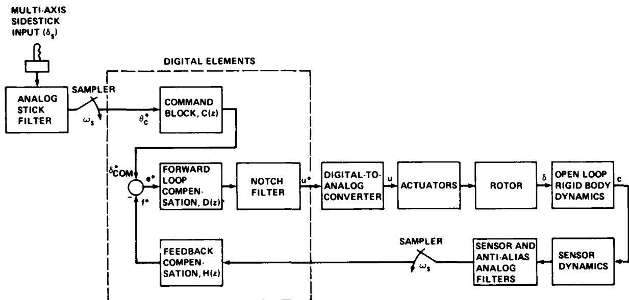
Figure 2.- Generic digital control implementation.
