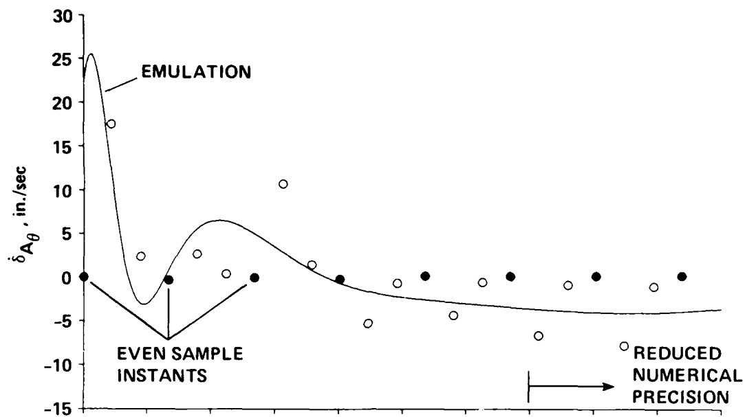
Figure 57.- ADOCS actuator rate ( \delta A_\theta ) response to a step input, \delta_{c\theta} = 1 ; digital versus emulation results (15 Hz system).
