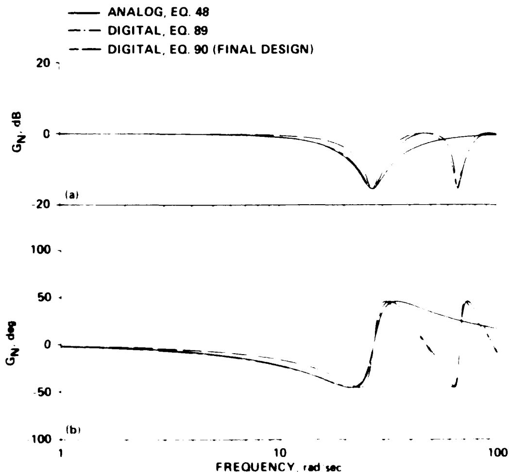
Figure 52.- Digital and analog notch filters for the 15 Hz system. (a) Magnitude; (b) phase.
