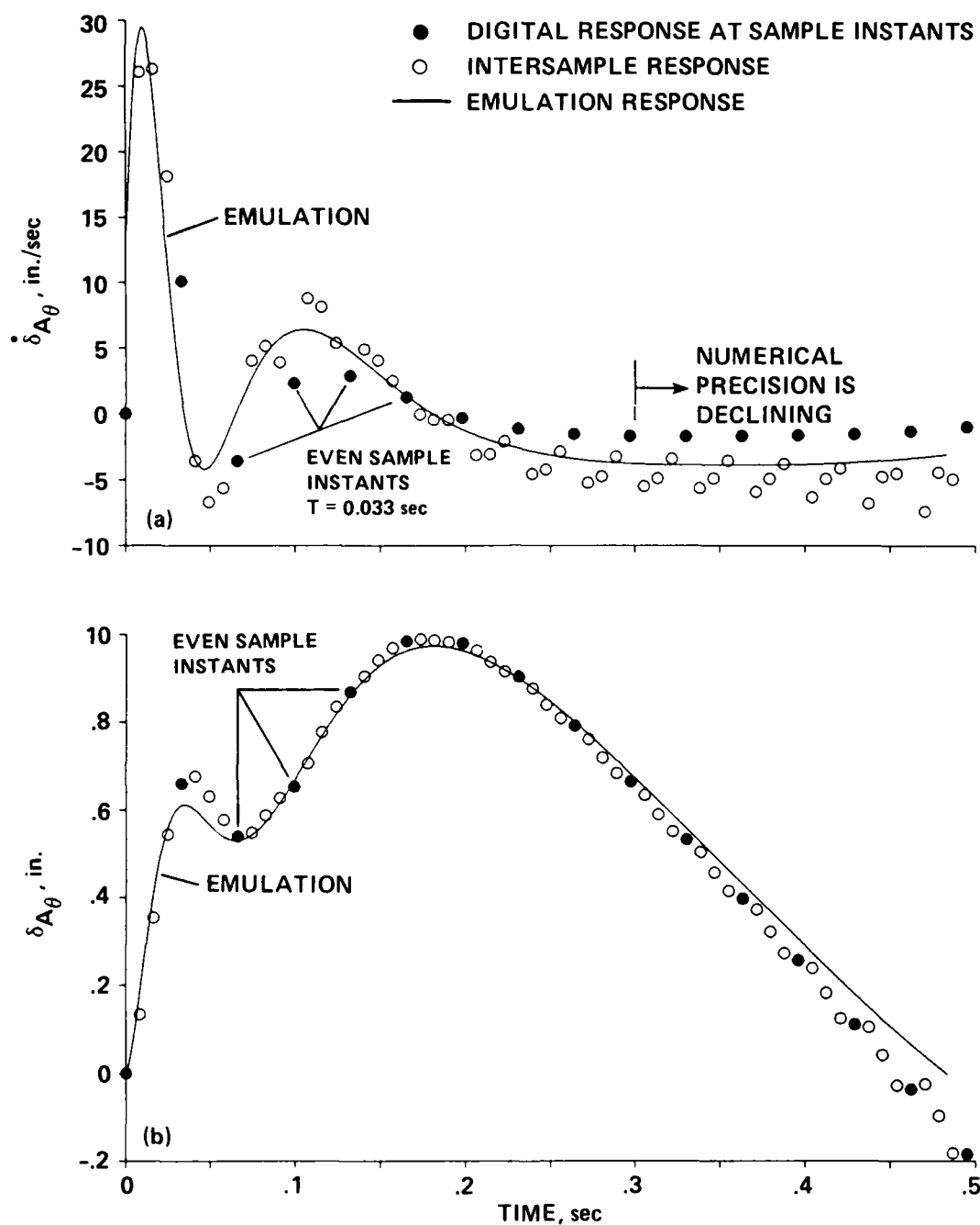
Figure 48.- Response to a step input, \delta_{c\theta} = 1 , digital and emulation analyses (30.3 Hz system). (a) ADOCS actuator rate ( \dot{\delta}_{A\theta} ); (b) ADOCS actuator deflection ( \delta_{A\theta} ).
