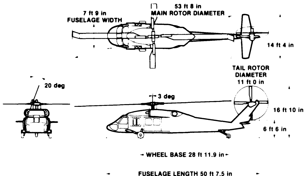
Figure 14.- UH-60A Black Hawk general arrangement.
