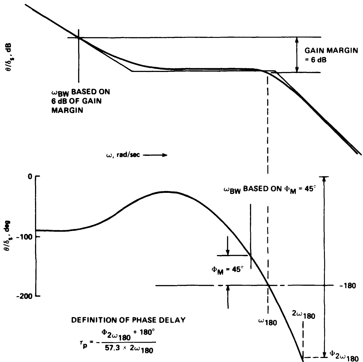
Figure 3.- Definition of pitch attitude bandwidth ( \omega_{BW} ) and phase delay ( \tau_p ); for this case the bandwidth is governed by the gain margin requirement.
