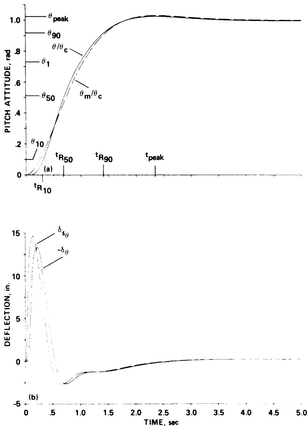
Figure 26.- Time response of the overall system ( \theta/\theta_c ) to a normalized step input ( \theta_c = 1 ) compared with the command model response. (a) Pitch attitude response ( \theta ); (b) swashplate ( \delta_{s\theta} ) and flapping angle ( \delta_\theta ) responses; (c) swashplate rate ( \dot{\delta}_s ) response; (d) swashplate rate ( \dot{\delta}_{s\theta} ) response shown on an expanded time scale.
