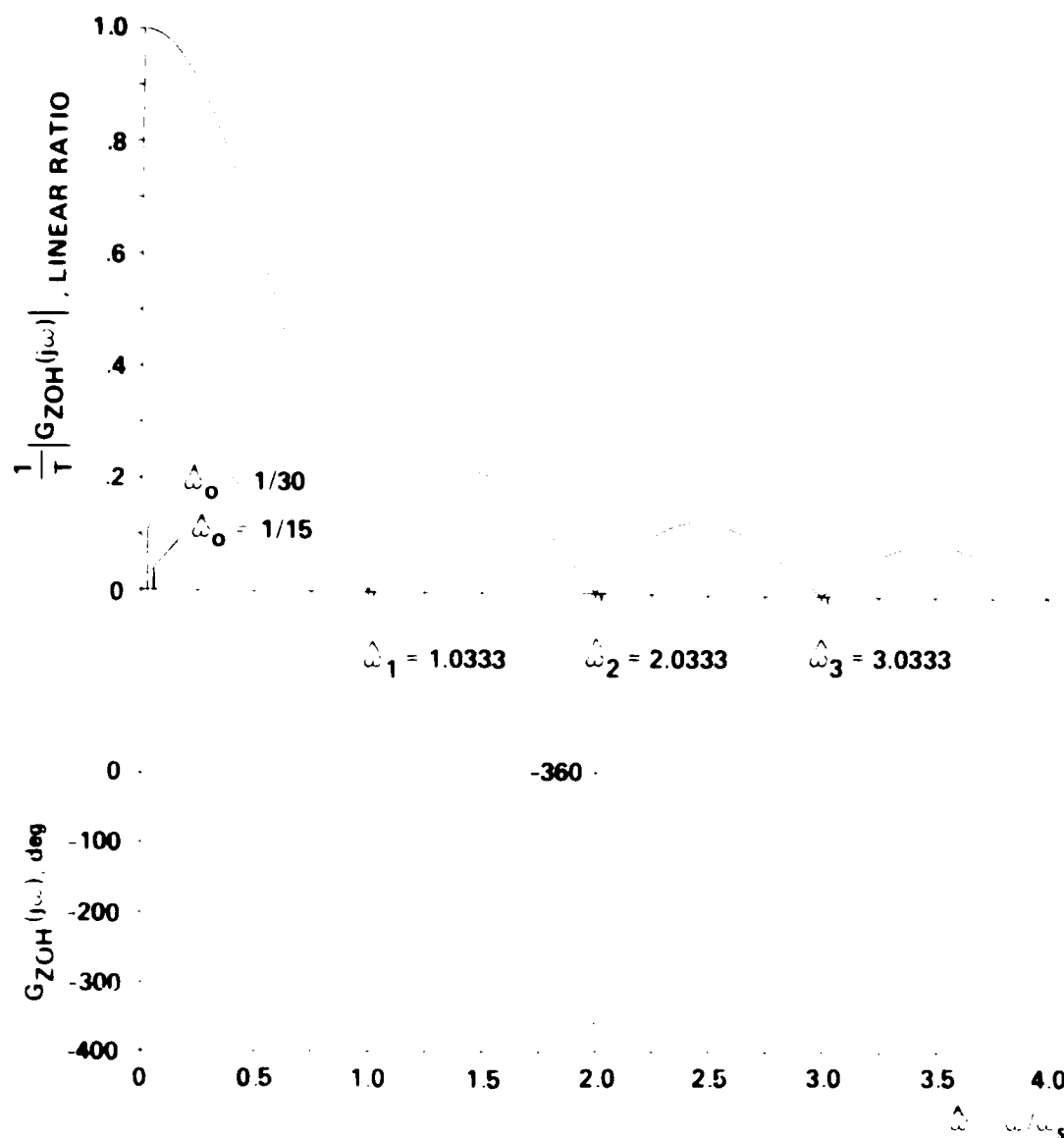
Figure 10.- Frequency response of the zero-order hold.
