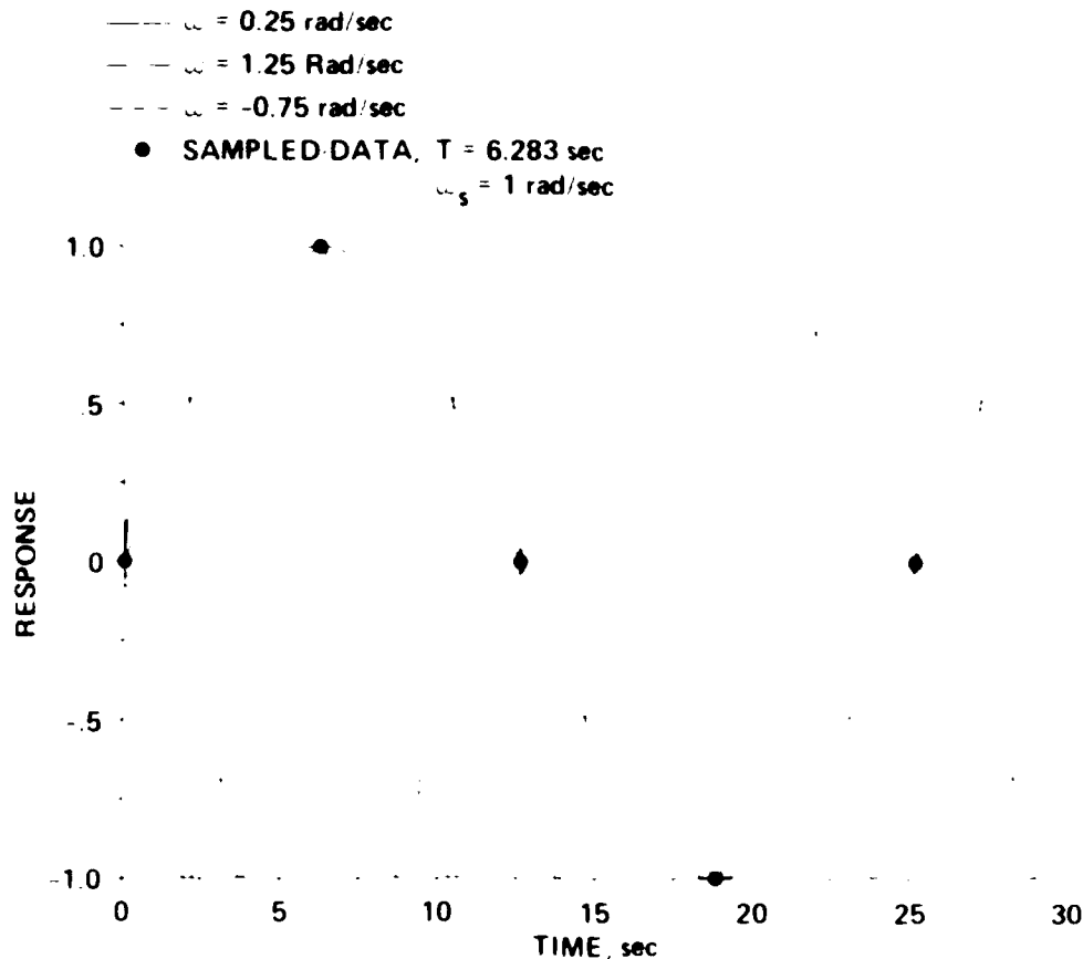
Figure 9.- Time domain illustration of aliasing.
