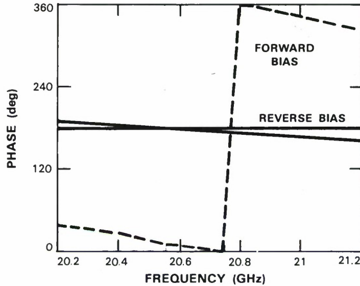
Figure 8. Typical reflection phase variation as diode bias condition changes.
