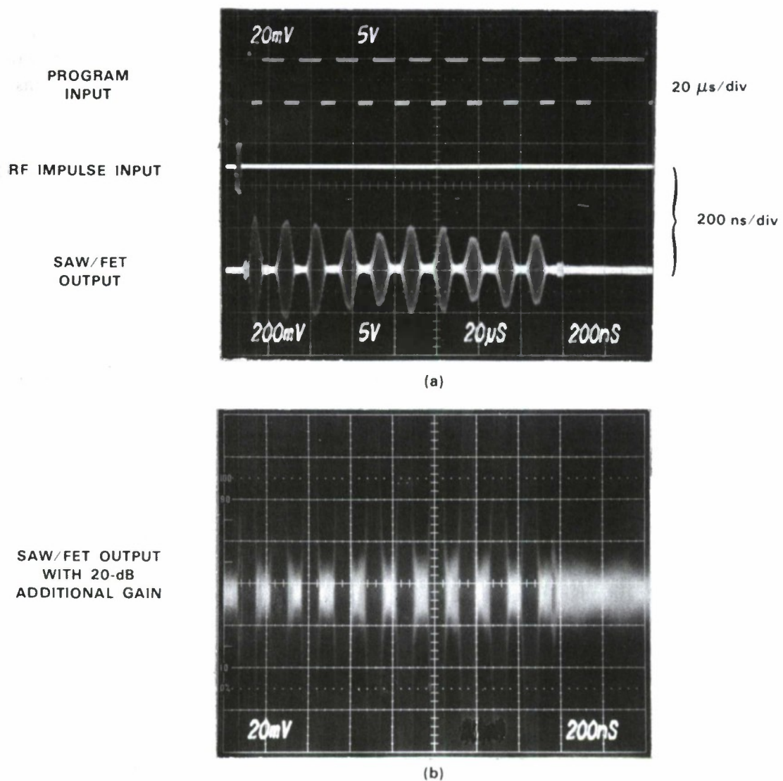
Figure 5-4. Demonstration of 30-dB programmable on/off ratio of SAW/FET. (a) Top trace: low-speed programming of the device, turning alternate groups of taps fully on and off. Middle trace: RF input, a 175-MHz-carrier impulse. Bottom trace: device output. (b) Device output with 20-dB additional gain, demonstrating the on/off ratio. Most of the signal from the 'off' finger groups is thermal noise, as evidenced by its continuation past the 1.5- \mu\text{s} impulse response duration.
