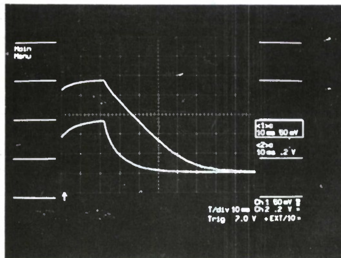
Figure 2-4. Temporal display on an oscilloscope of the 1.65- \mu\text{m} fluorescence from Er:YAG as 1.47- \mu\text{m} excitation intensity was varied.
