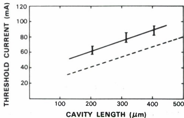
Figure 3-11. Threshold current as a function of cavity length for stripe-geometry (110) DH lasers. The dotted line represents data reported in Reference 7 for Al_{0.07}Ga_{0.93}As/Al_{0.45}Ga_{0.55}As DH lasers.
