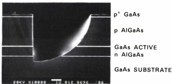
Figure 3-12. Scanning electron micrograph showing the cross section of a facet-deflector pair formed by Br:methanol etching.
