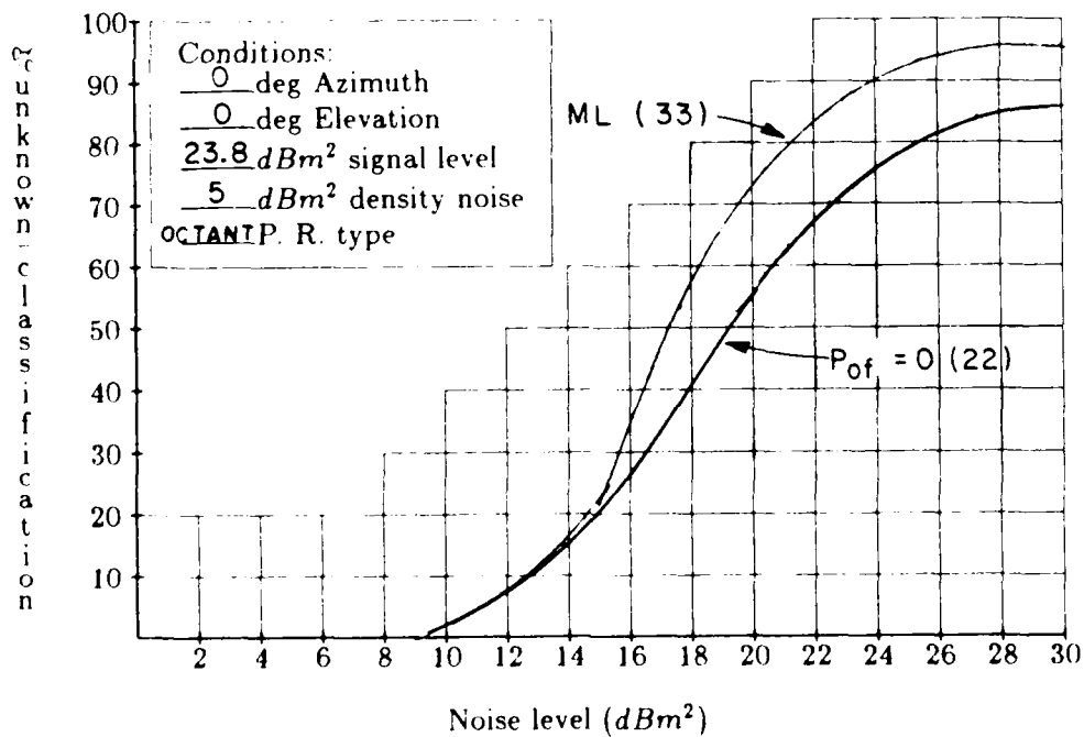
Figure 17: Percent unclassification, Octant crossing, 5 \text{ dBm}^2 likelihood function and associated automata
