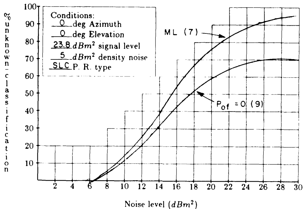
Figure 16: Percent unclassification, SLC, 5 \text{ dBm}^2 likelihood function and associated automata
