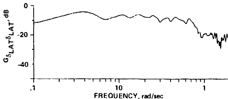
Figure 6.- Lateral stick input autospectrum in hover.
