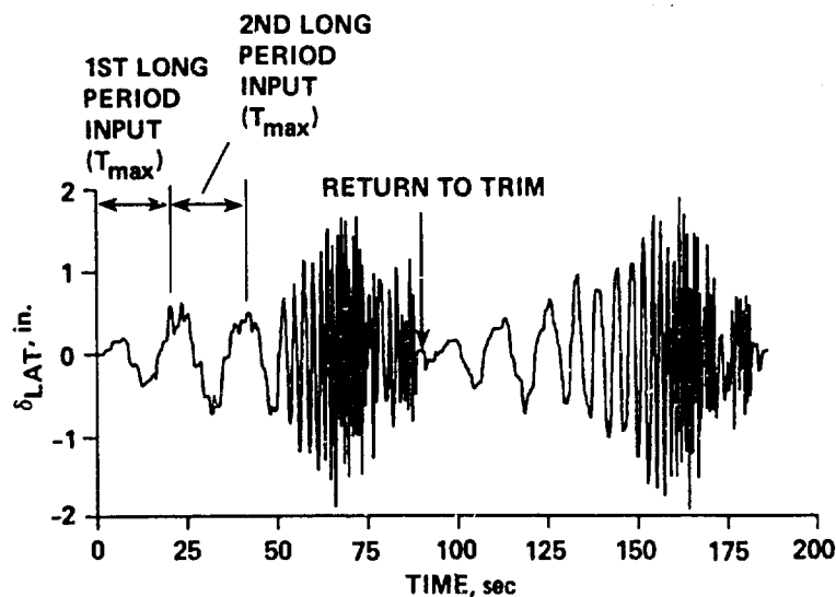
Figure 3.- Frequency sweep input.
