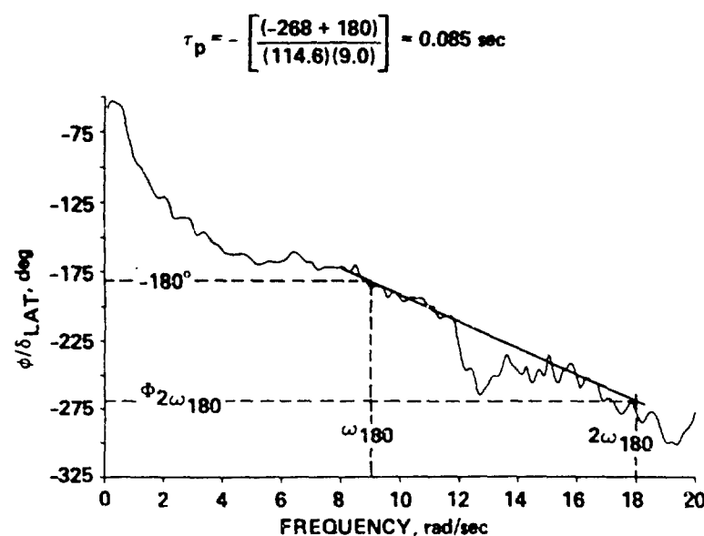
Figure 15.- Linear frequency plot of phase of roll rate response to lateral stick in hover.
