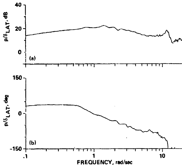
Figure 9.- Roll rate response of lateral stick in hover. (a) Magnitude; (b) phase.
