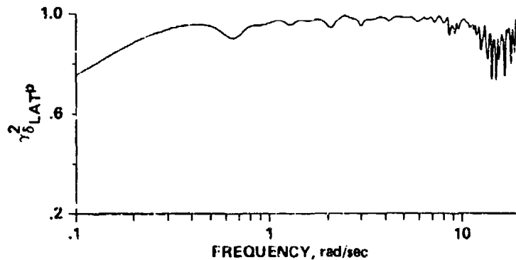
Figure 10.- Coherence function for roll rate response to lateral stick in hover.
