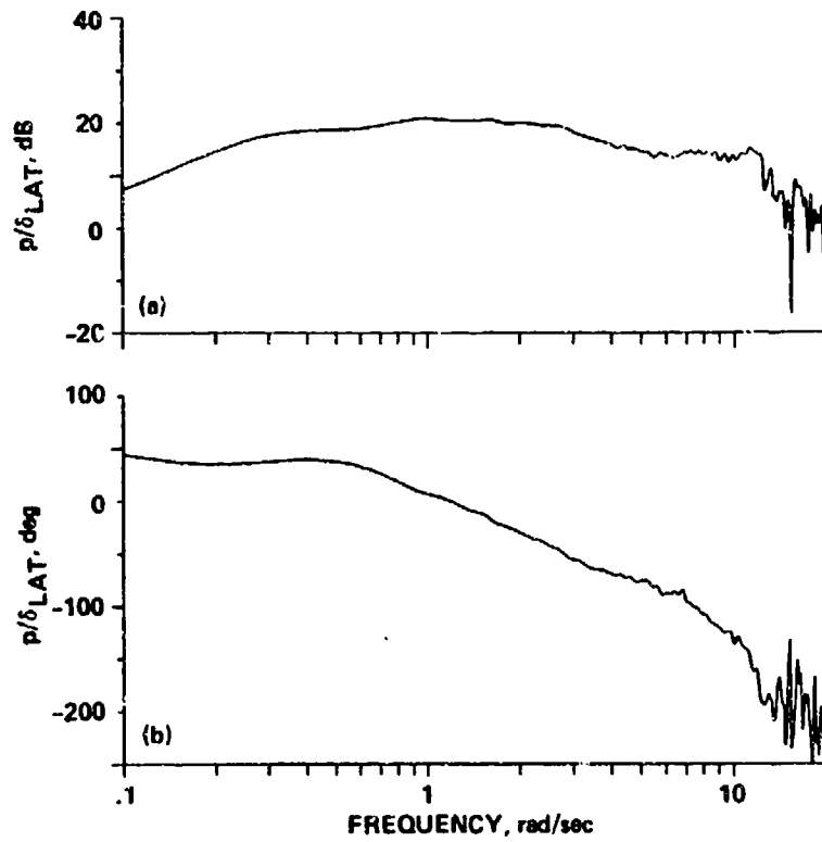
Figure B5.- Roll rate response to lateral stick. (a) Magnitude; (b) phase.
