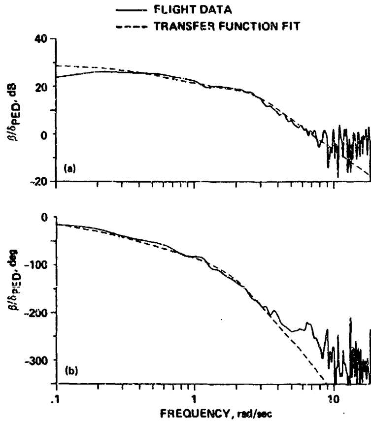
Figure B31.- Transfer function model for side slip angle response to pedals. (a) Magnitude; (b) phase.
