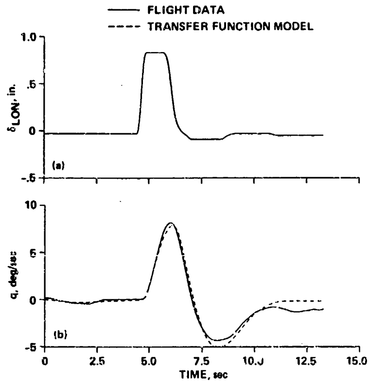
Figure P16.- Comparison of filtered aircraft response and transfer function model response to a filtered longitudinal stick step input. (a) Longitudinal stick input; (b) pitch rate.
