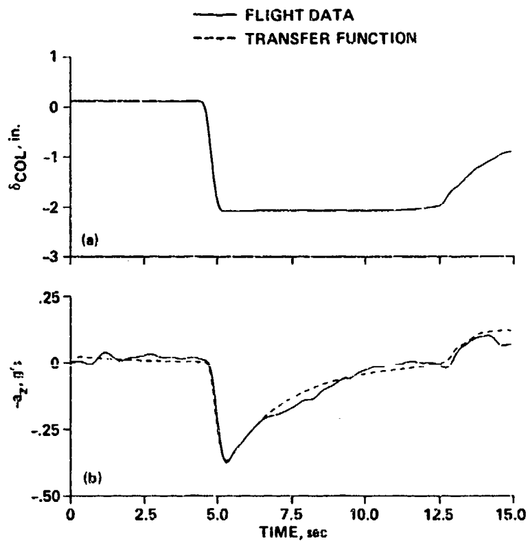
Figure B40- Comparison of filtered aircraft response and transfer function model response to a filtered collective stick step input. (a) Collective-stick input; (b) vertical acceleration.
