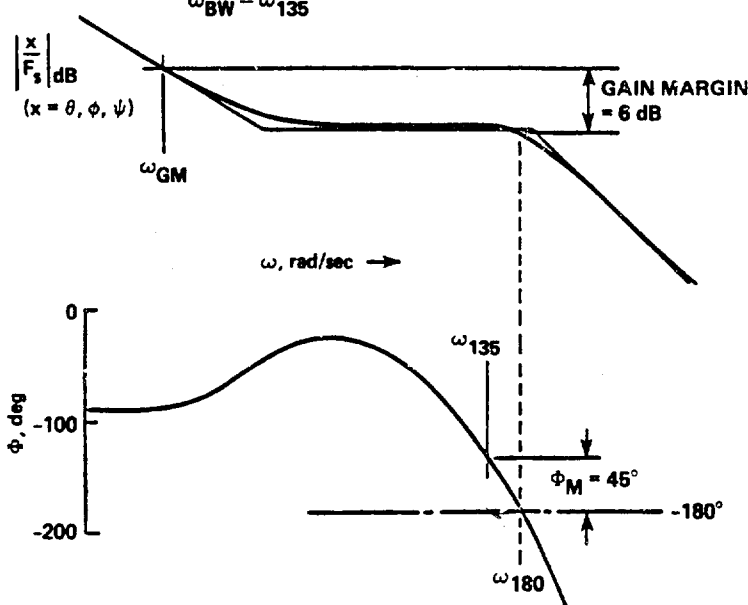
Figure 1.- Definitions of bandwidth and phase delay.
