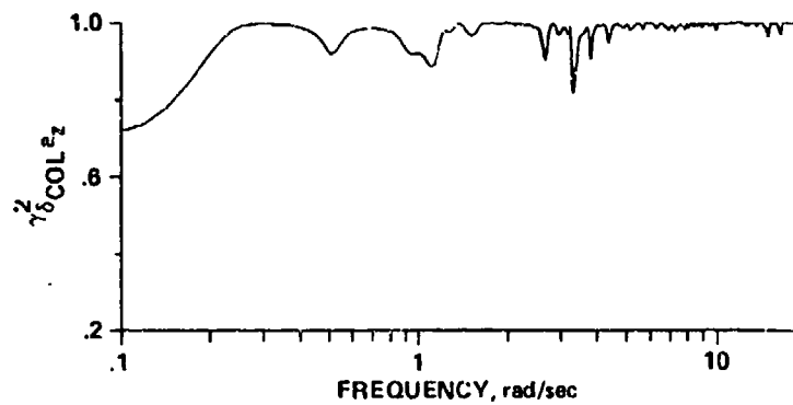
Figure B38.- Coherence function for vertical acceleration response to collective stick.
