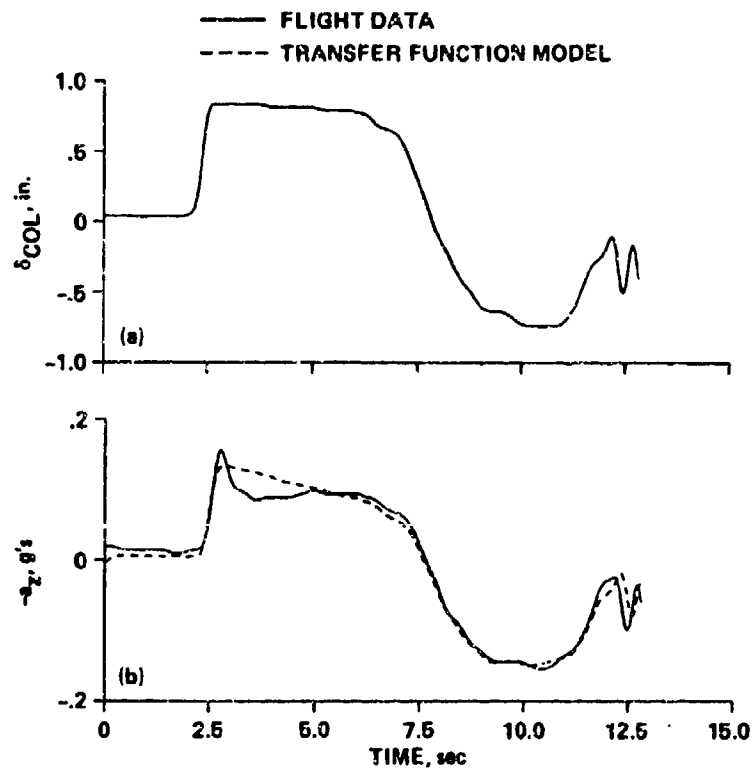
Figure A32.- Comparison of filtered aircraft response and transfer-function model response to a filtered collective stick step input. (a) Collective stick input; (b) vertical acceleration.
