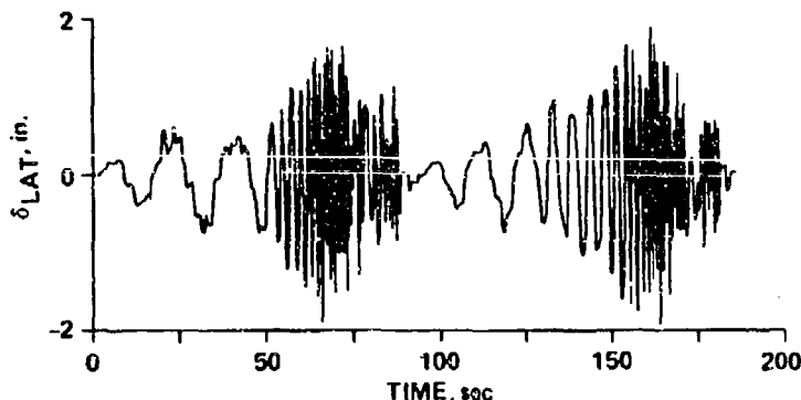
Figure 5.- Lateral stick frequency sweeps in hover.
