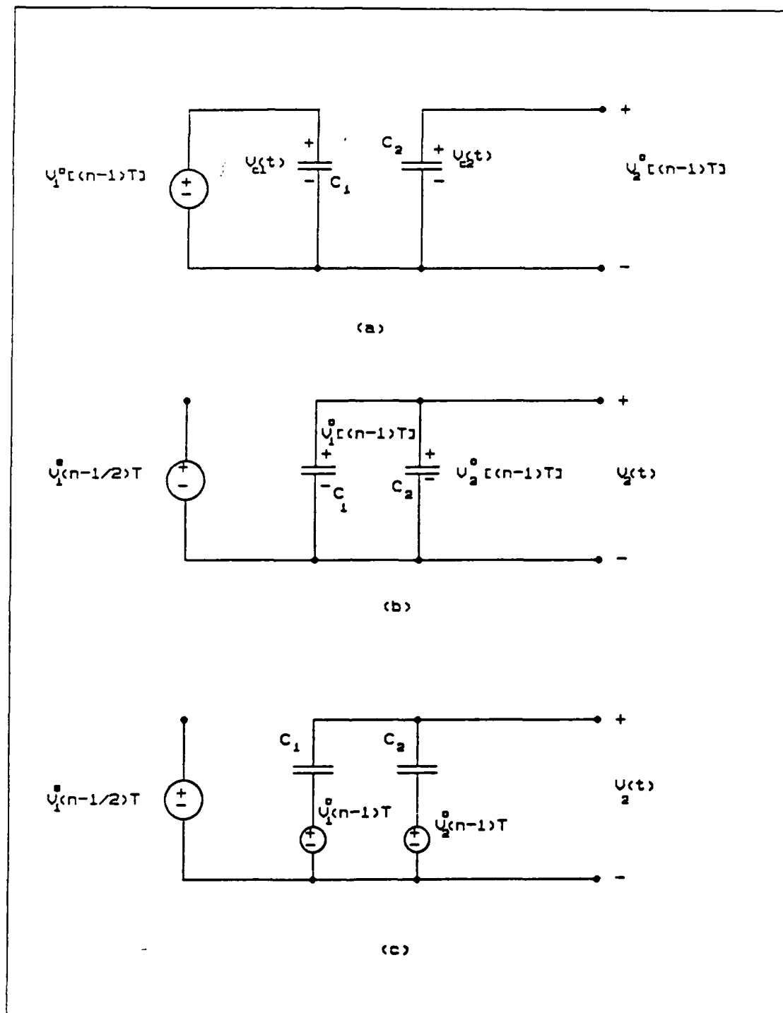
Figure 2.4 Equivalent Circuit of Figure 2.3. (a) Equivalent Odd Circuit when \Phi_1 switch is closed. (b) Equivalent even circuit when \Phi_2 switch is closed. (c) Alternative form of (b).
