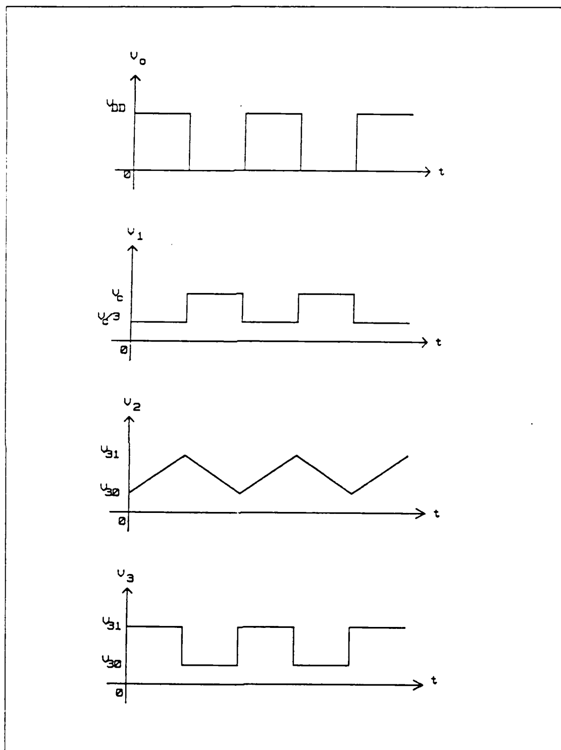
Figure 3.3 The Waveforms of the VCO.
