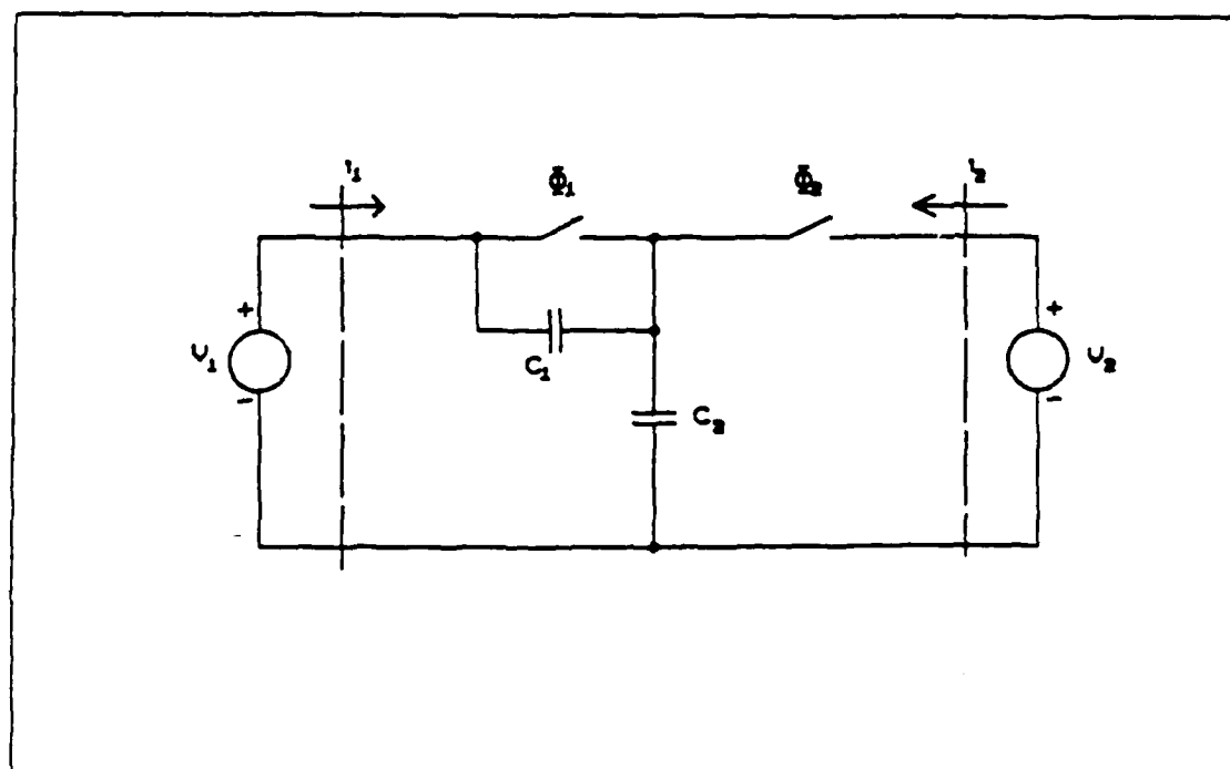
Figure 1.4 Series-Parallel Switched Capacitor Realization of a Continuous Resistance.
