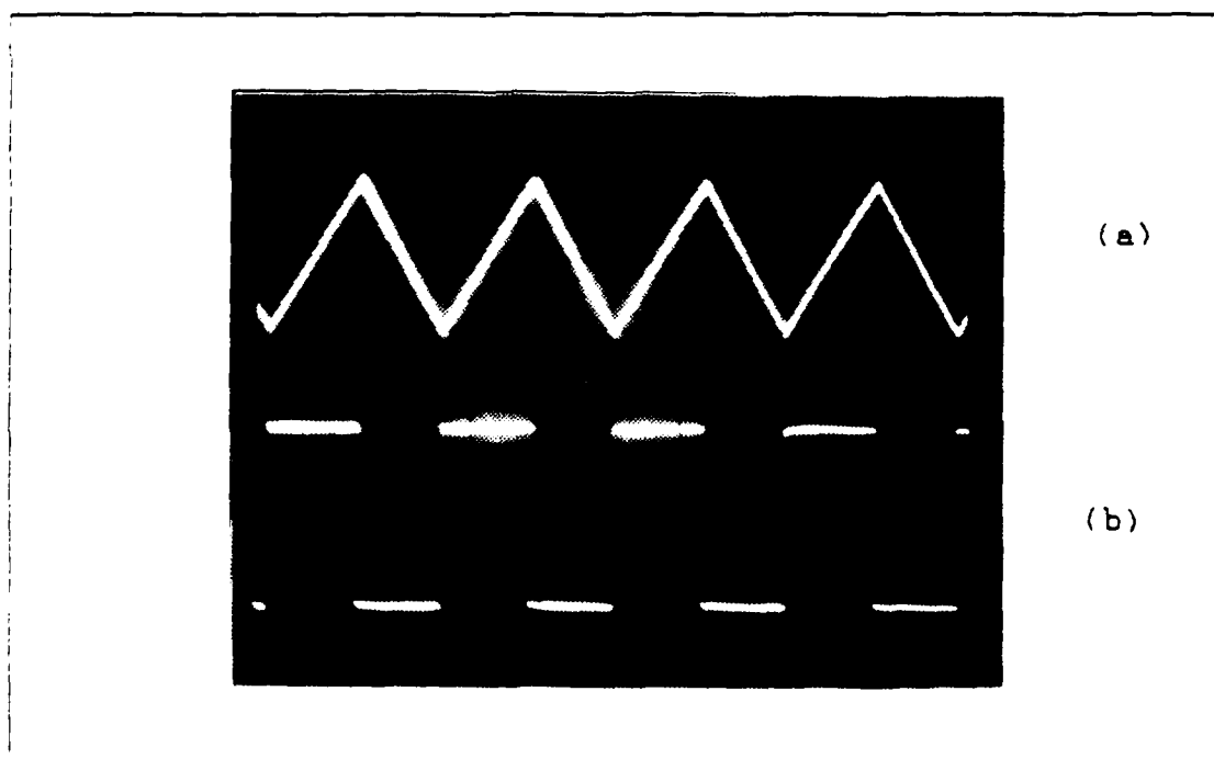
Figure 3.14 (a) The Output of the Integrator (0.5 volt div.) (b) The Output of the VCO (5 volt div, 5 \mu sec div).
