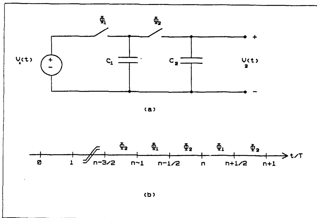
Figure 2.3 Switched Capacitor Realization of Figure 2.1. (a) Parallel Configuration. (b) Clock Phasing.
