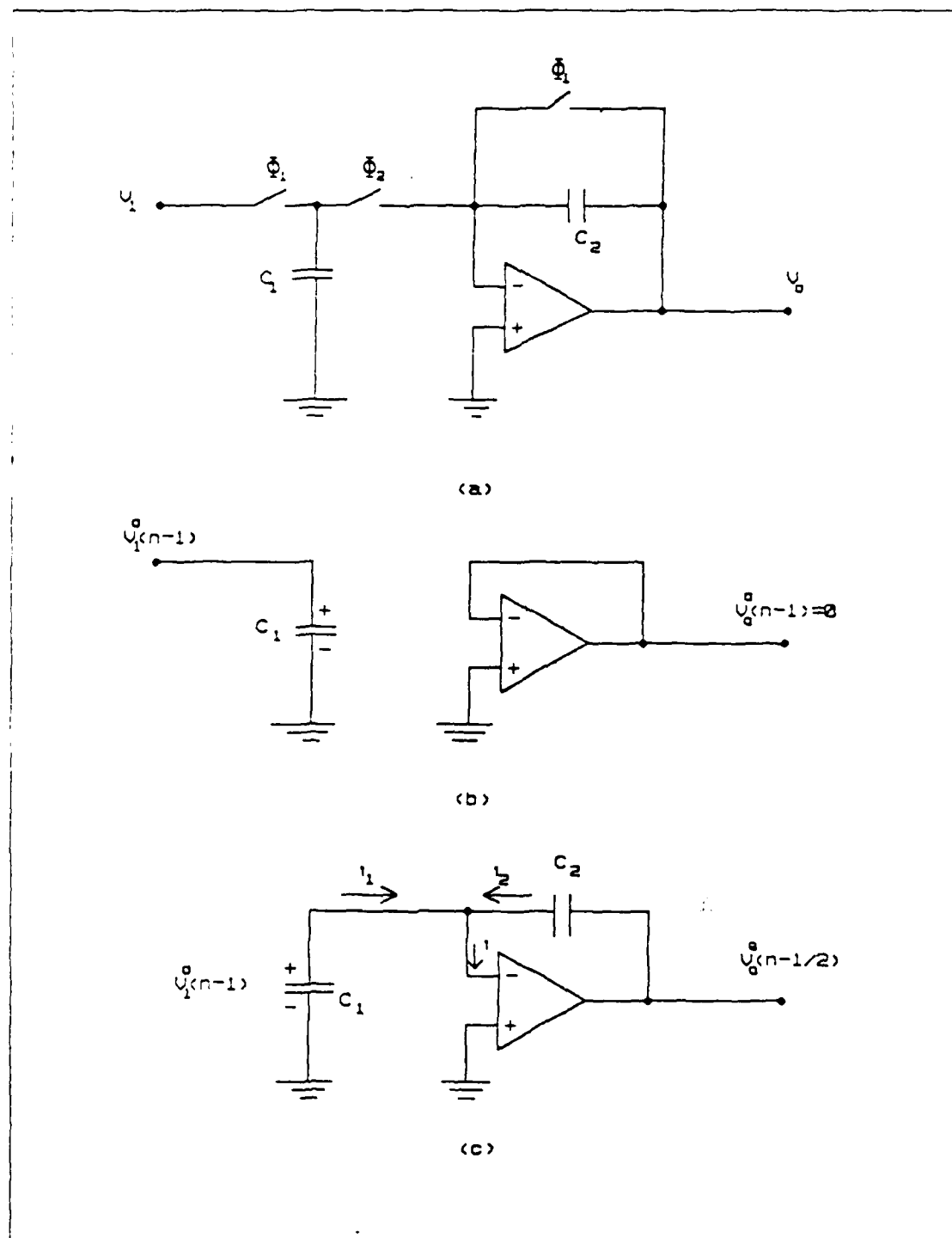
Figure 4.11. (a) A Practical Realization of Figure 3.9 (b) Equivalent Circuit of (a) when \Phi_1 is closed (c) when \Phi_2 is closed.
