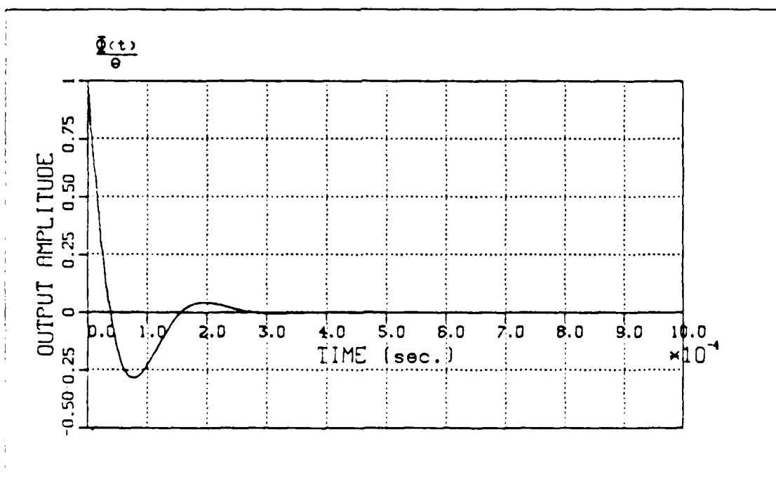
Figure 3.21 The Phase Step Response of the Error Function.
