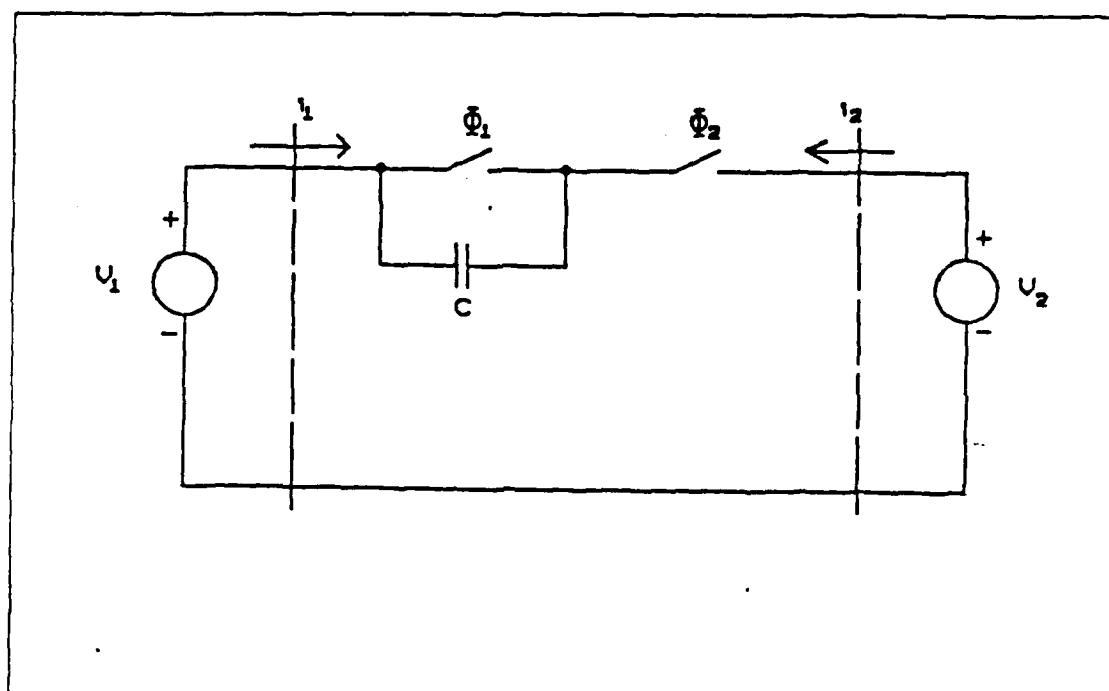
Figure 1.3 Series Switched Capacitor Realization of a Continuous Resistance.
