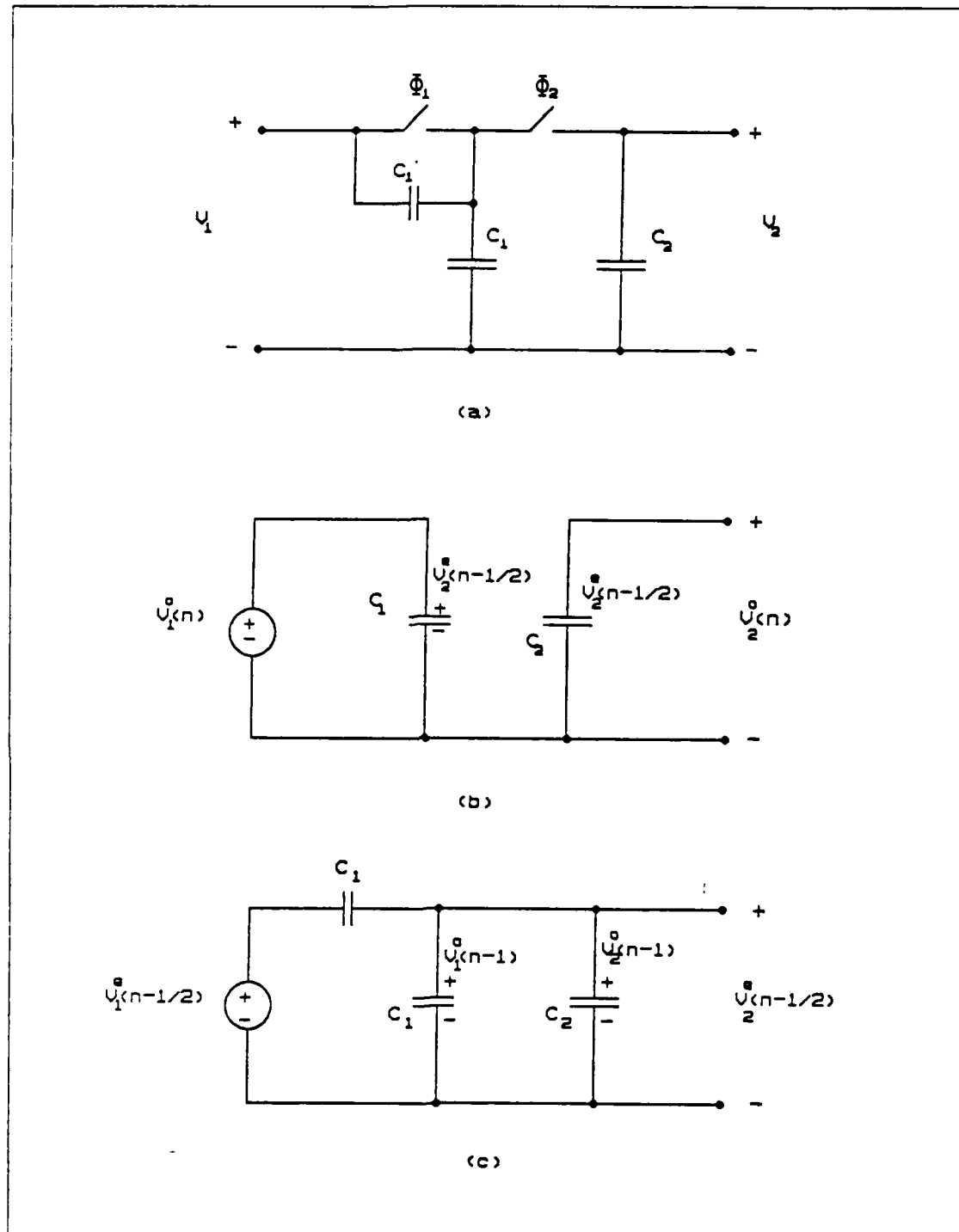
Figure 2.10 Parallel-Series SC Realization of Figure 2.1. (a) Equivalent SC Circuit. (b) Equivalent Representations of (a) when \Phi_1 is closed and (c) when \Phi_2 is closed.
