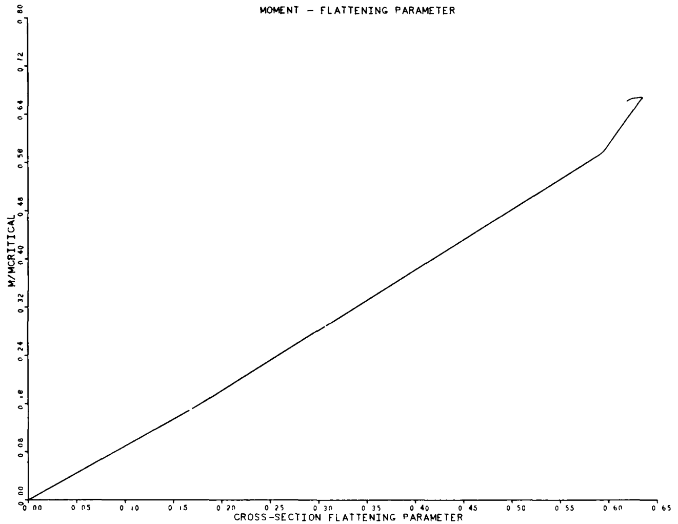
FIGURE 21. M/M_{CRITICAL} VERSUS CROSS-SECTION FLATTENING PARAMETER \Delta w/h FOR MODEL IC1
