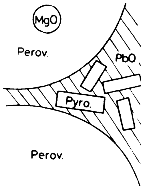
Figure 2. Schematic Illustration of Microstructure in PMN.
