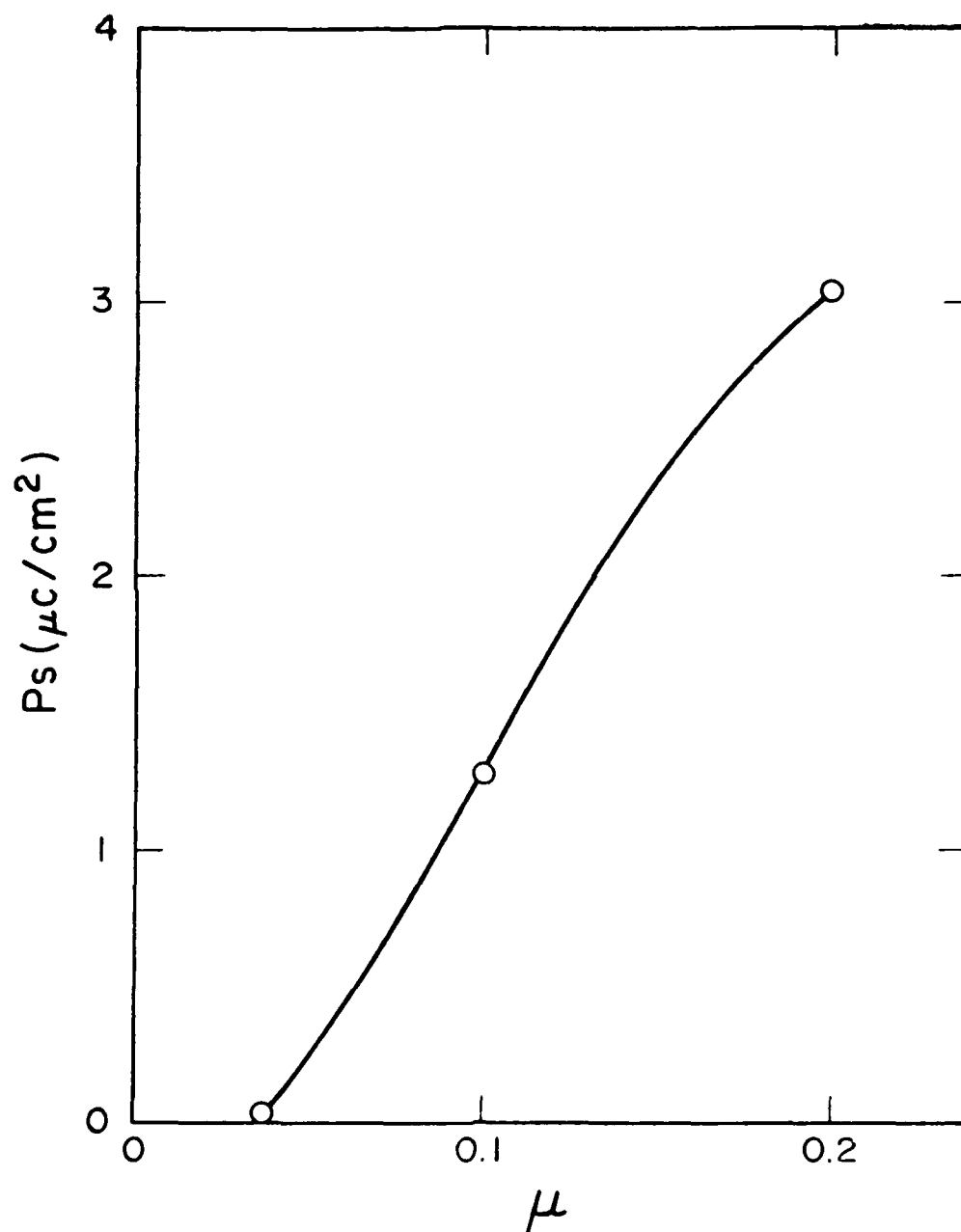
Figure 43. Variation of Spontaneous Polarization of \text{BaTiO}_3 Film at Room Temperature with Grain Size.
