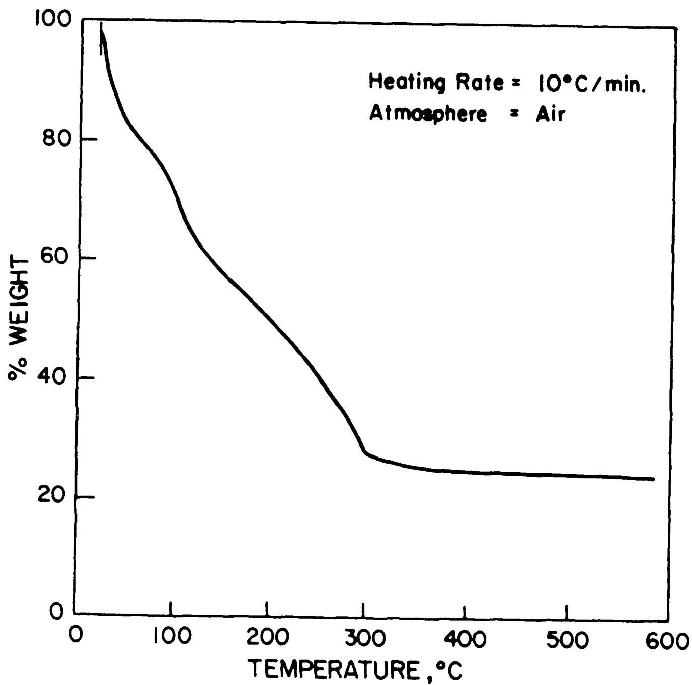
Figure 27. Thermogram of \text{Zr}(\text{OC}_4\text{H}_9)_4 Solution in xylene.
