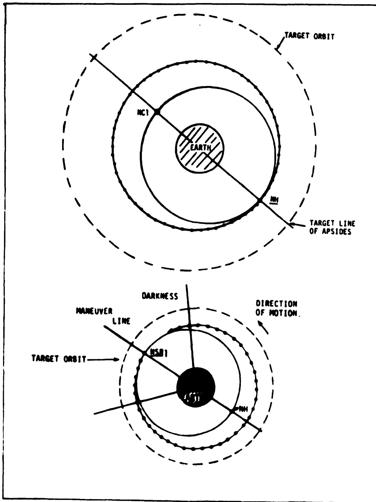
Figure 1. Coelliptic Rendezvous Sequence (Airfig 5-1 - 3-5)
