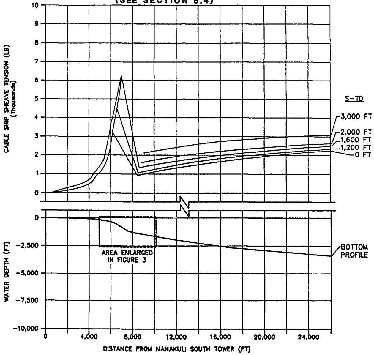
SECTION PROFILE ALONG PROPOSED CABLE ROUTE
