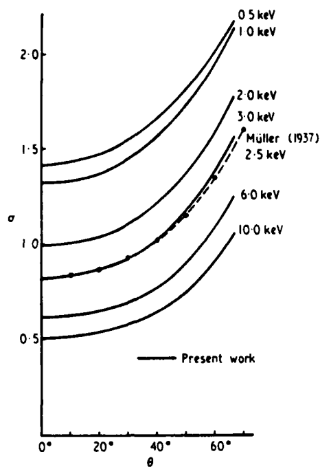
Fig. 8. Total secondary electron yield versus angle of incidence for a number of primary electron energies using a polycrystalline copper target. 8
