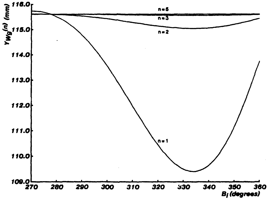
Figure 6: Y_{W_g}^{(n)}(B_1)
