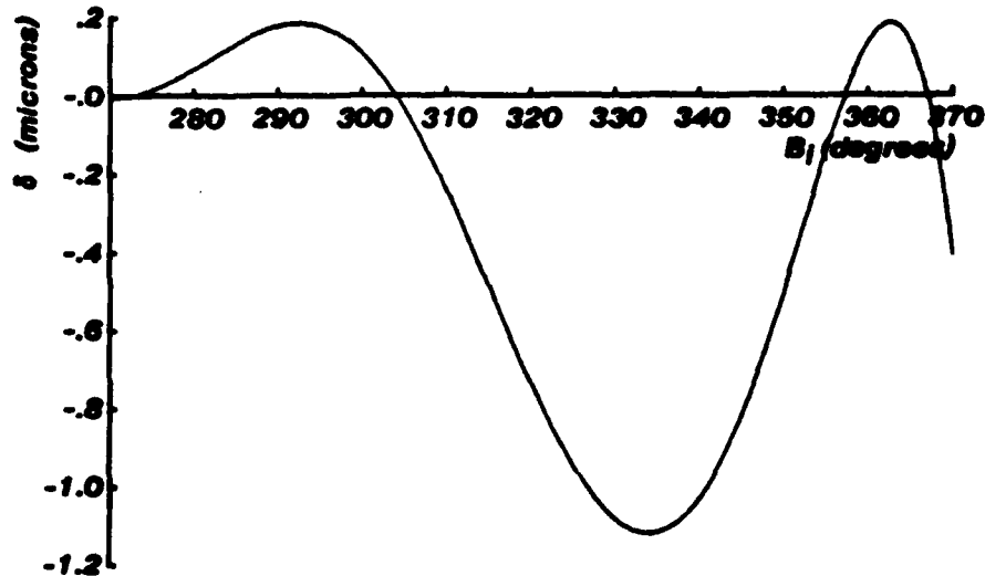
Figure 7: ERROR( B_1 )
