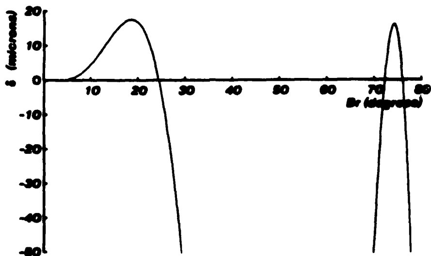
Figure 8: ERROR(B)
