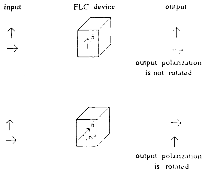
Figure 2. Smectic C phase ferroelectric liquid crystal as an addressable half-wave plate.
