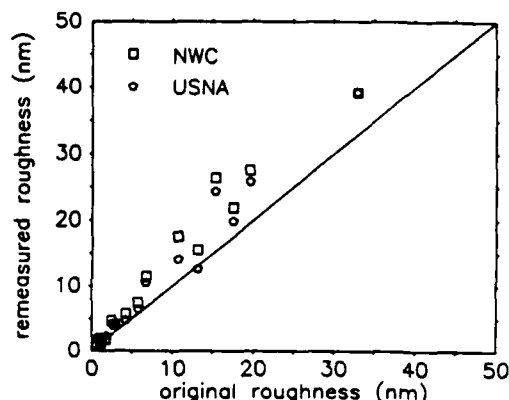
Fig. 2. Performance of the USNA TIS instrument compared with that of a state-of-the-art instrument at NWC, China Lake, using a set of 15 roughness standards. Roughnesses measured using USNA and NWC instruments are plotted versus original roughnesses measured at NWC, as discussed in the text. Diagonal line indicates equal original and remeasured values.
