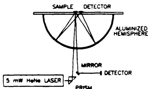
Fig. 1 Schematic diagram of the USNA TIS instrument. The detectors are connected to a relay, a digital multimeter, and a small personal computer which are not shown.
