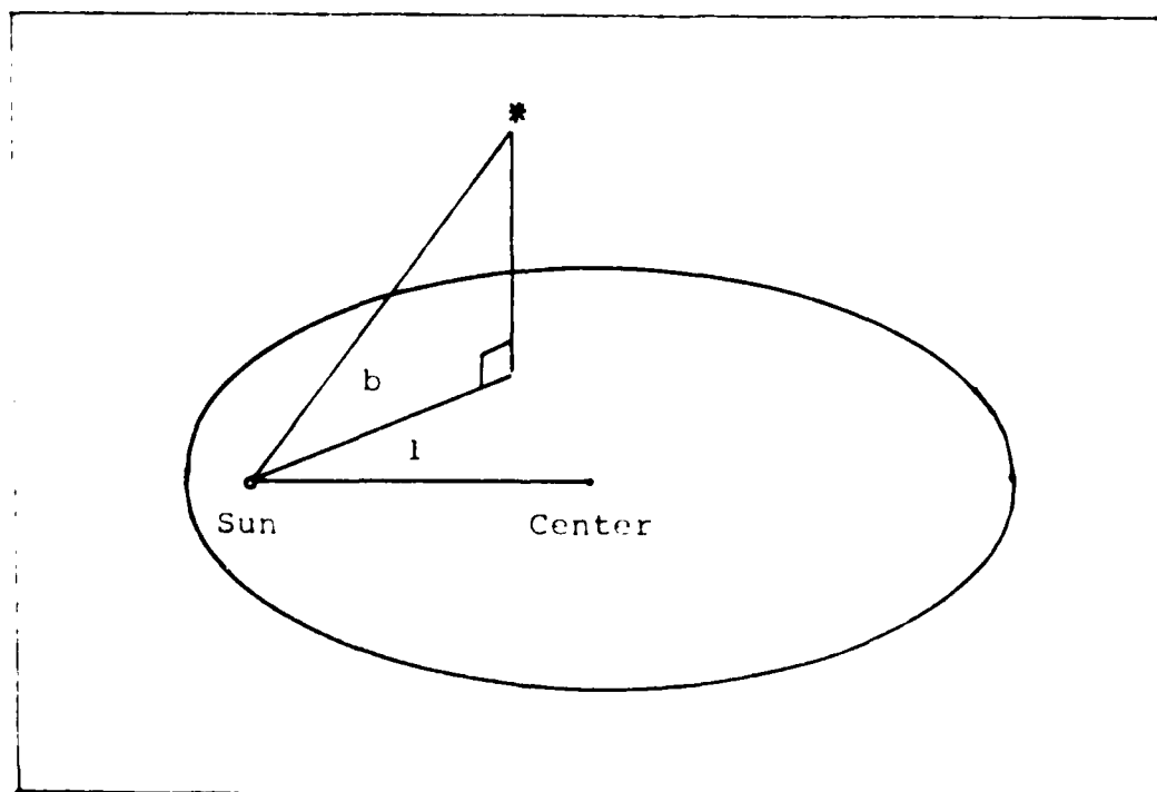
Figure A-4. Galactic Coordinates
