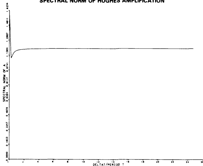
(A) OF HUGHES AMPLIFICATION MATRIX \underline{A} FOR \theta = 1.4, \xi = 0.10, \gamma = 0.10, \beta = 0.916275
