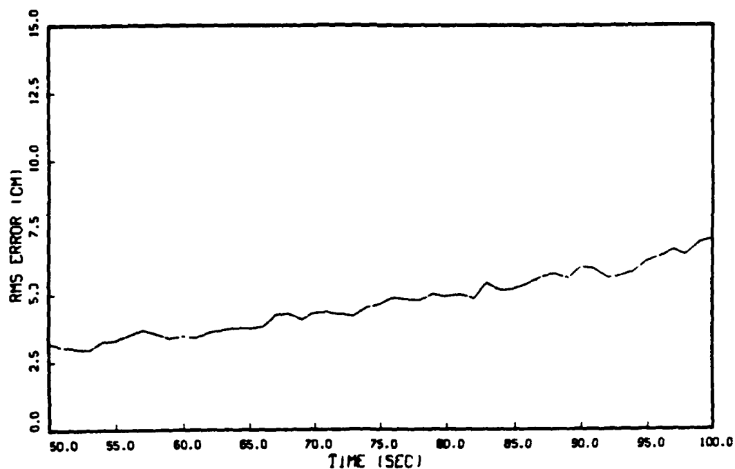
Figure 5-12. RMS Error Between the Target and Beam Position: \tau_{Bf}=20.0 (sec), \tau_{Bt}=20.4 (sec)
