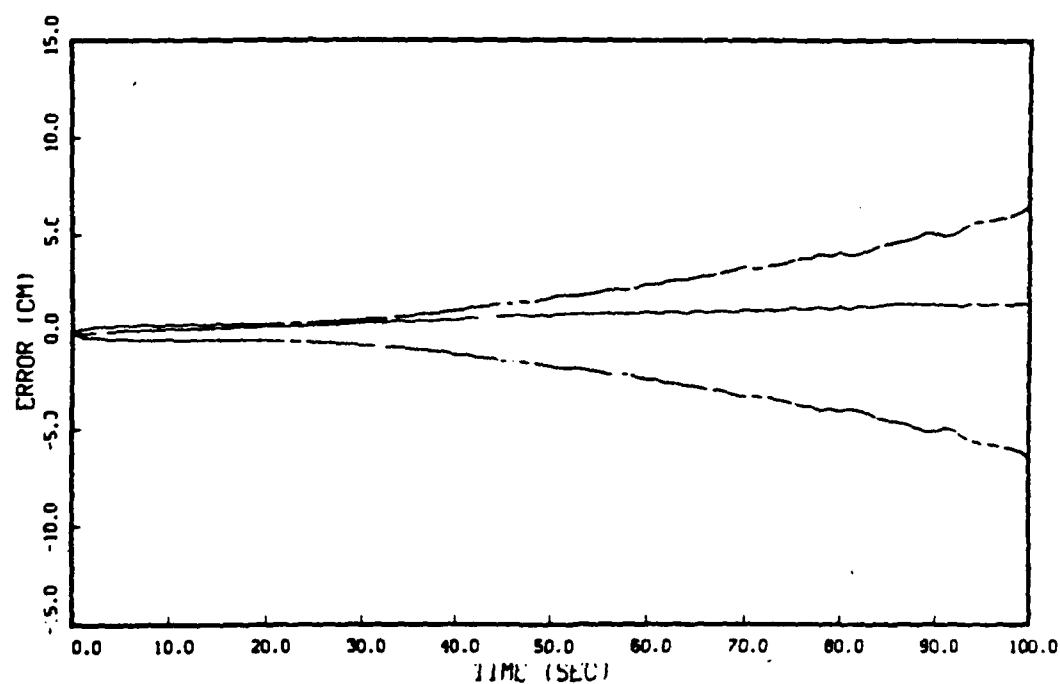
Figure 5-13. Mean and \pm Standard Deviation Envelope of the Error between the True and Filter Position States: \tau_{Bf}=20.0 (sec), \tau_{Bt}=20.4 (sec)
