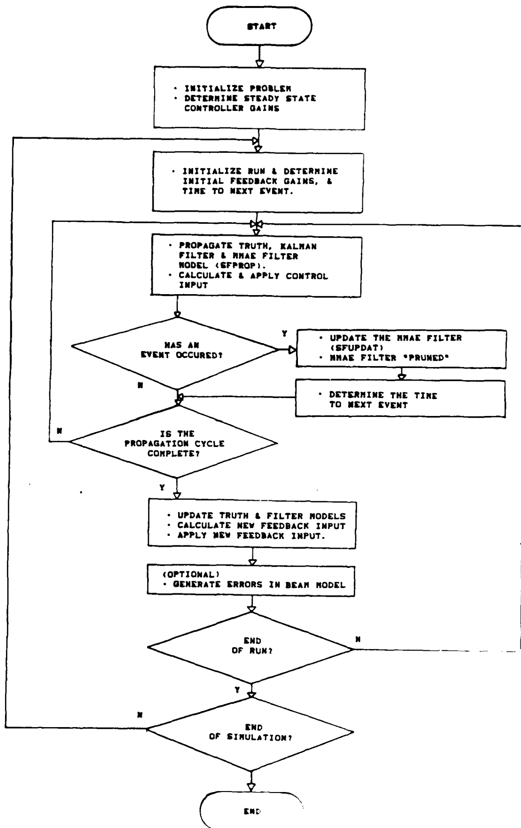
Figure 4-1. Macro Level Flow Chart of the Simulation
