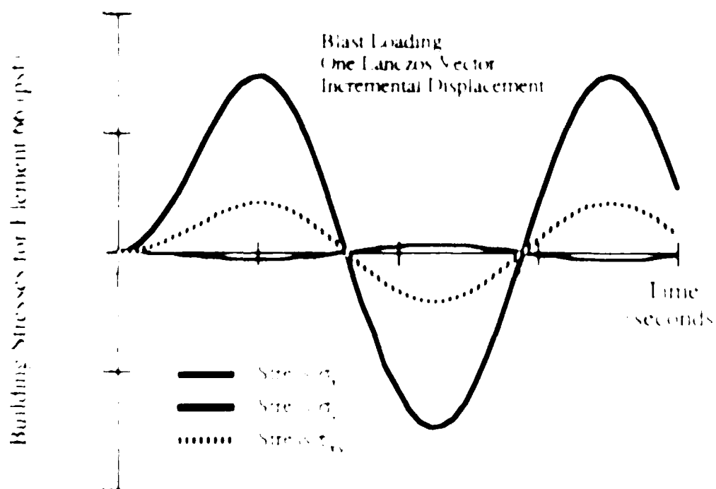
Figure 4.21. Element Stresses for Reduced Problem 1 Mode.
