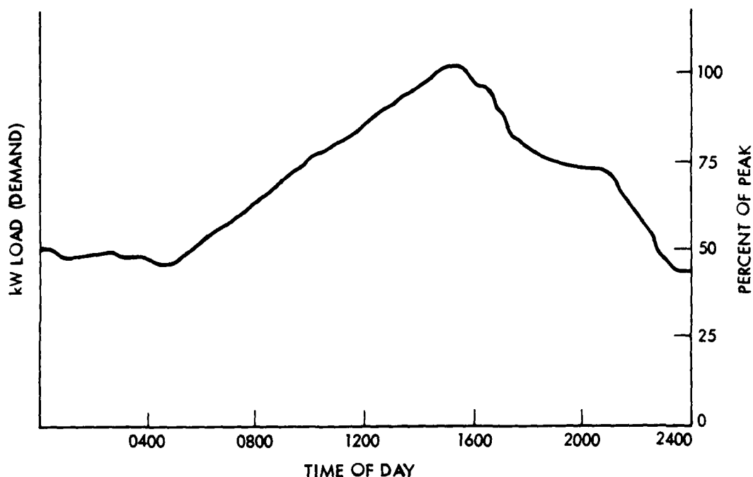
Figure 1. Typical Load Profile Curve
