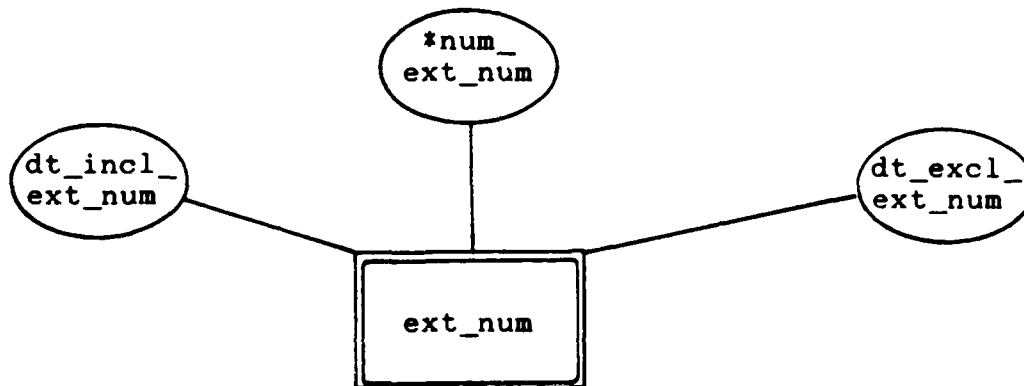
Weak entity ext_num
