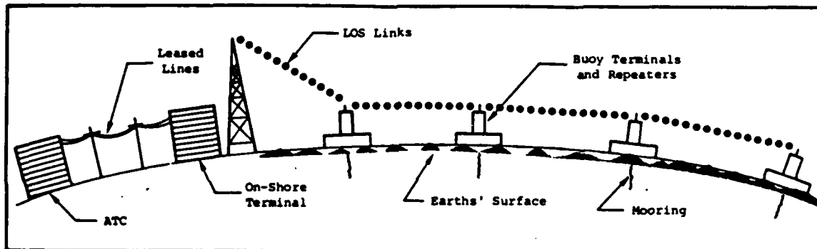
(b) Link Scheme
