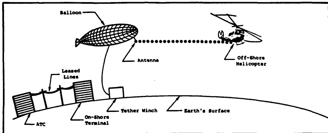
Figure 7. BALLOON SYSTEM
