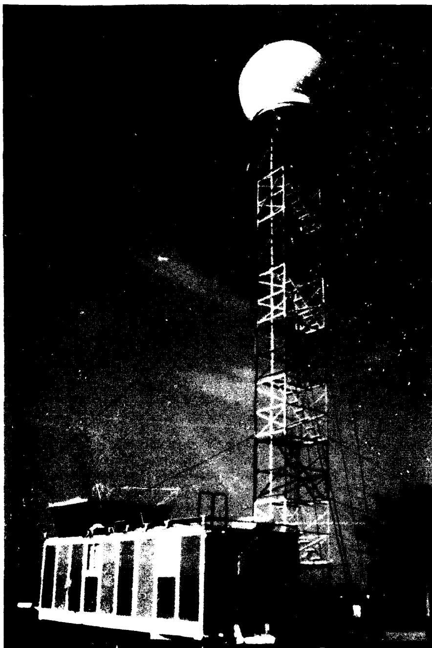
Figure 2.3 Photograph of the UND radar site at Southaven, Mississippi.
