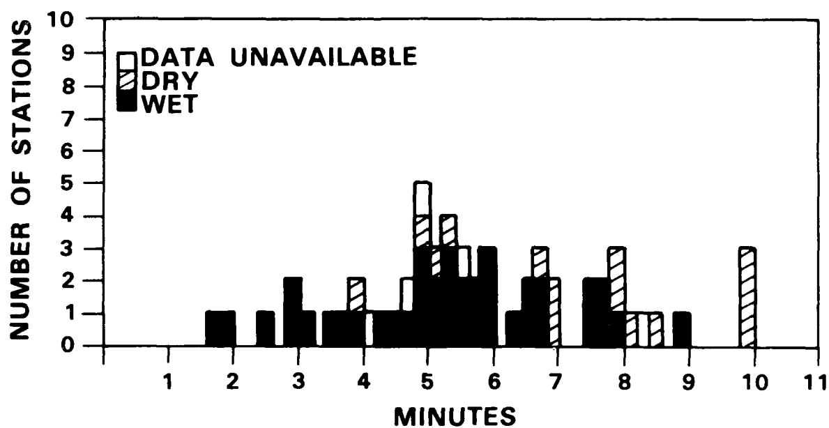
Figure 3.7 Duration of FLOWS 1984 microbursts.
