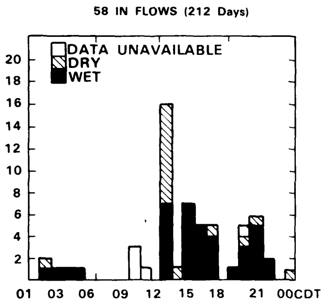
Figure 3.3 Diurnal variation of microbursts in (a) NIMROD, (b) JAWS, and (c) FLOWS. The FLOWS distribution shares some of the features of both the NIMROD and the JAWS distributions.
