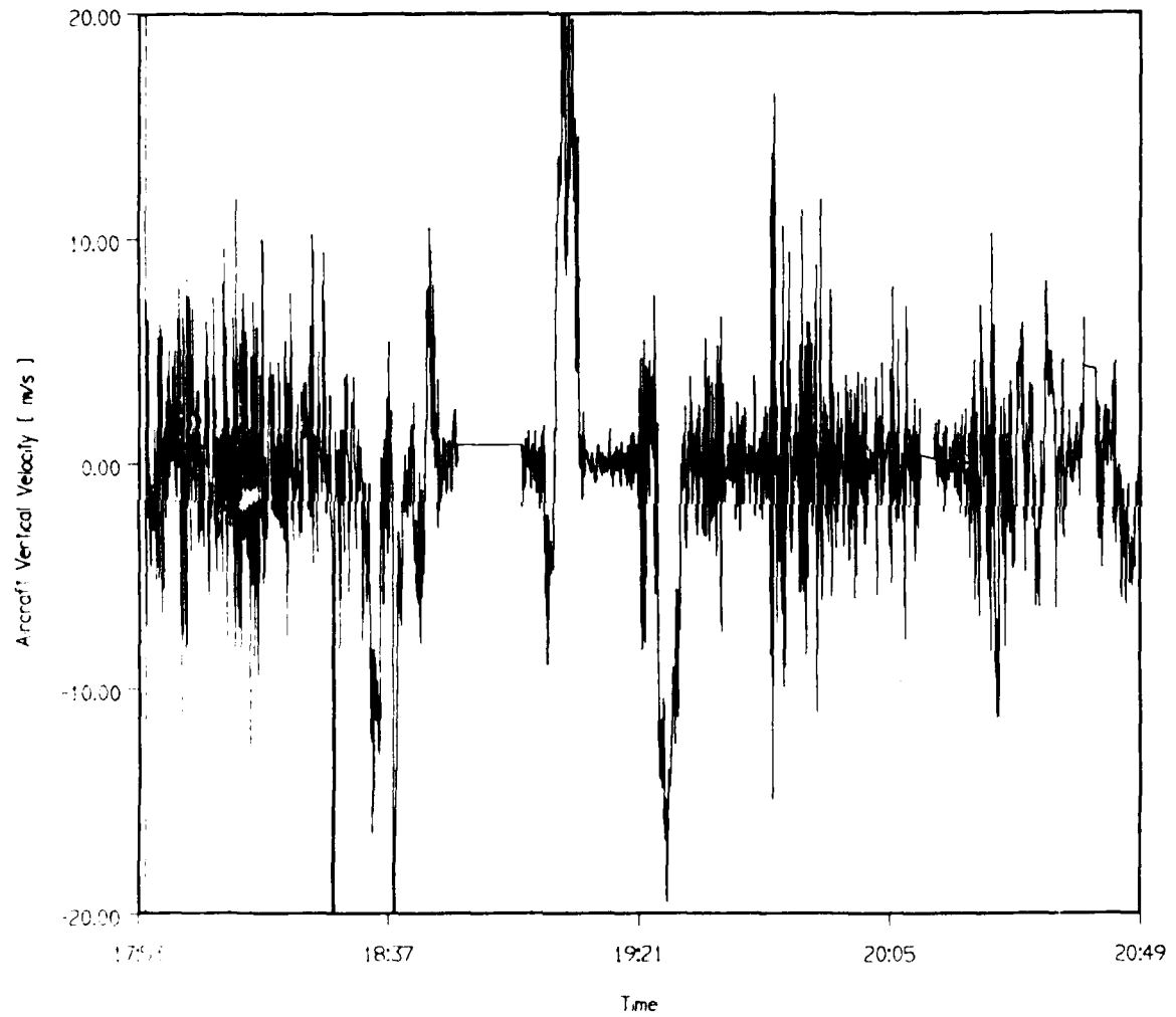
Figure 5.3 Vertical velocity of aircraft.
