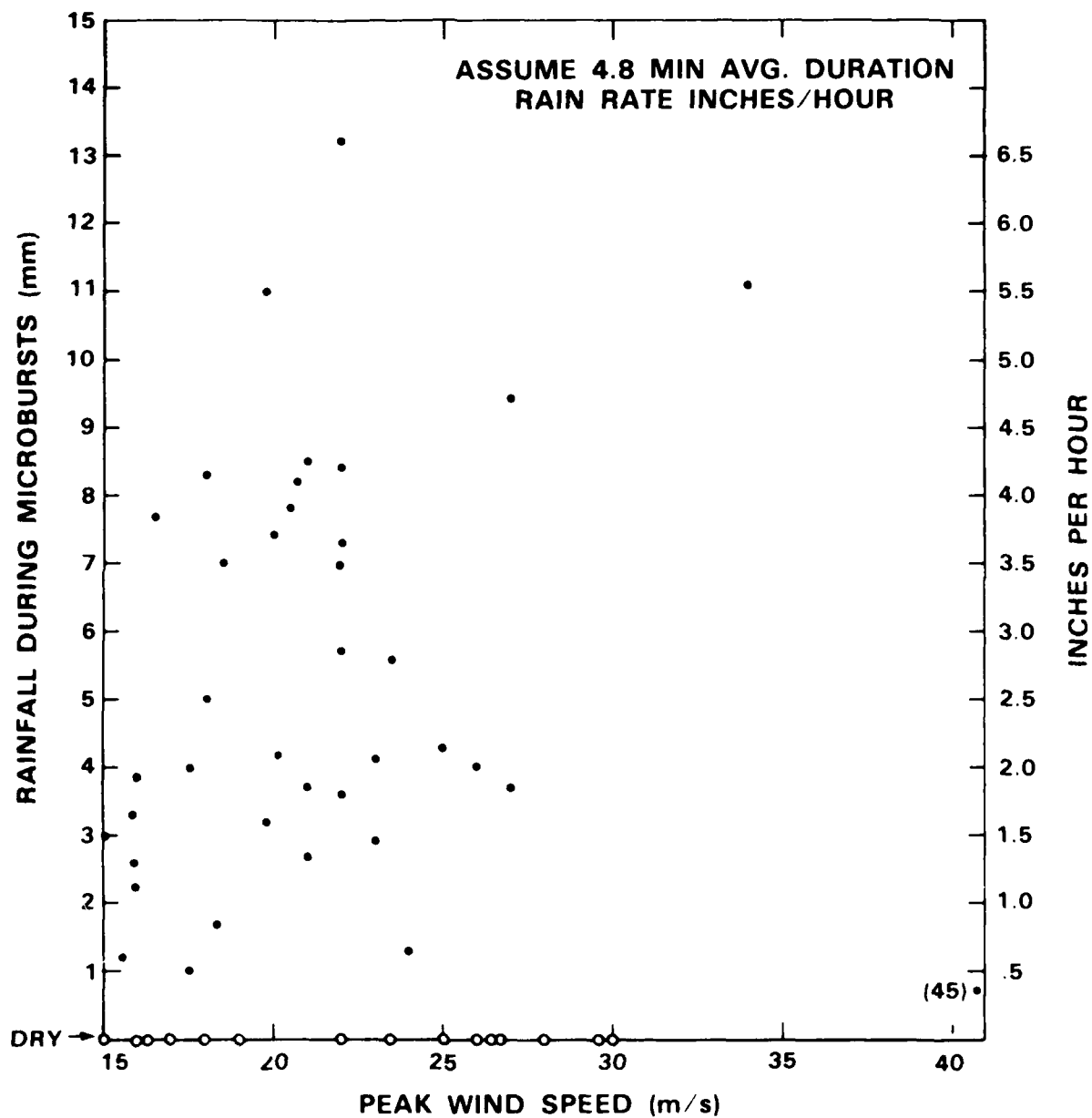
Figure 3.4 Total rainfall (or rainfall rate assuming 4.8-min microburst duration) versus maximum wind speed in 58 wet and dry microbursts during FLOWS 1984.
