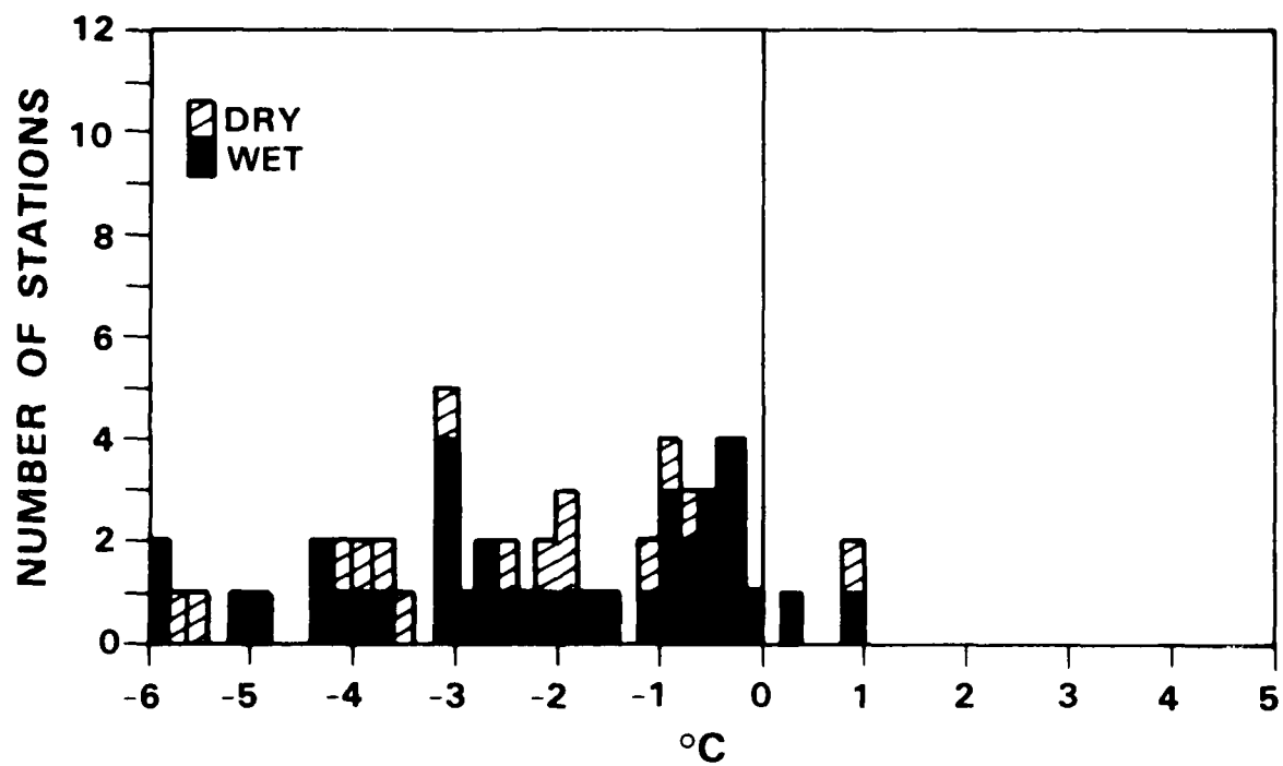
Figure 3.8 Temperature change in FLOWS 1984 microbursts.
