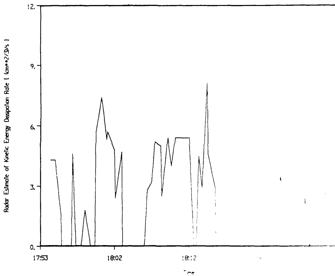
Figure 5.6(c) Time series of radar estimate of kinetic energy dissipation rate along aircraft track. Flight height 3.5 km, range 10 km.
