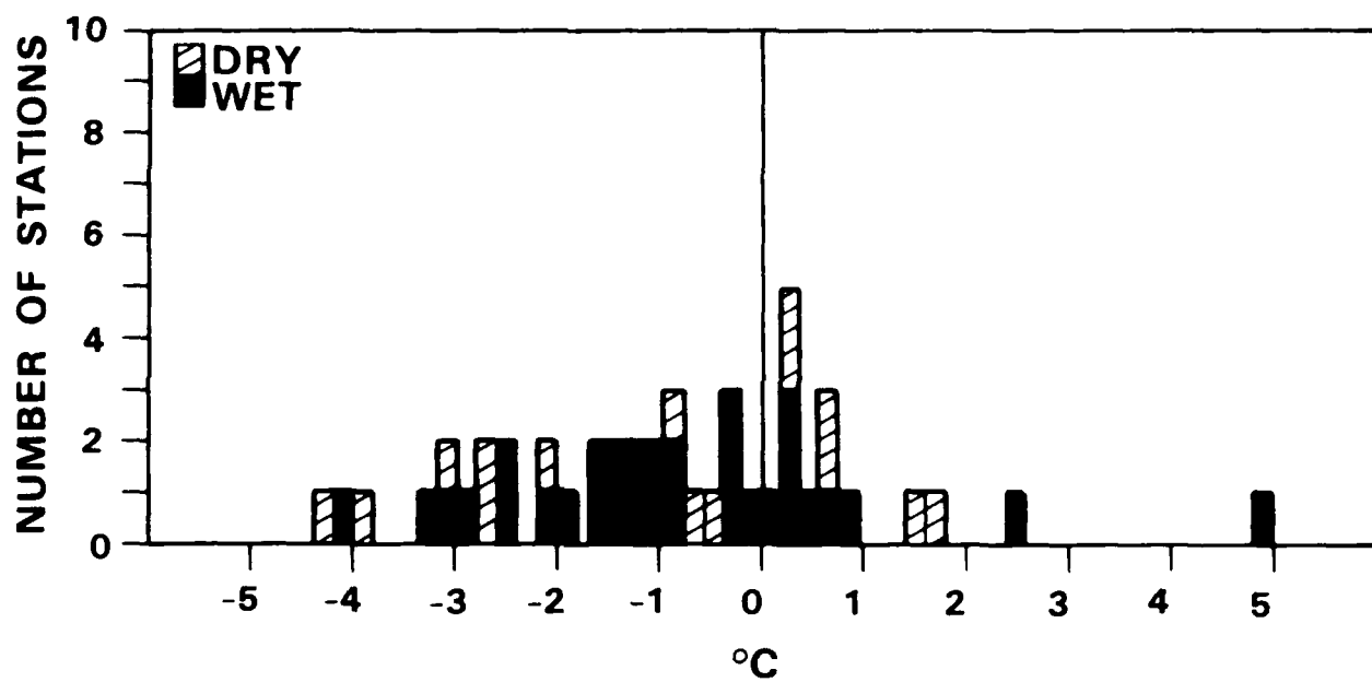
Figure 3.9 Dew point temperature change in FLOWS 1984 microbursts.
