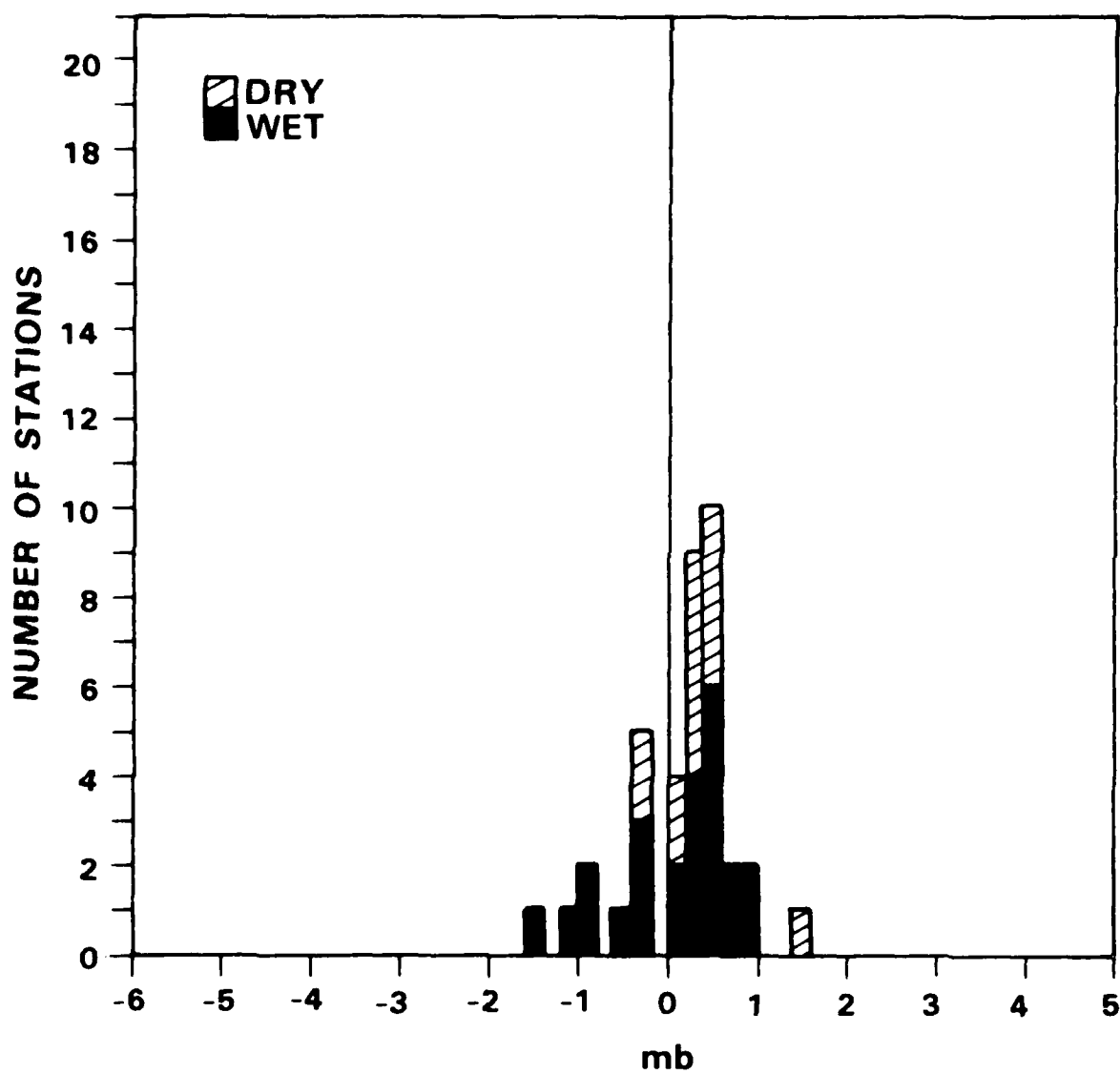
Figure 3.10 Pressure change in FLOWS 1984 microbursts.
