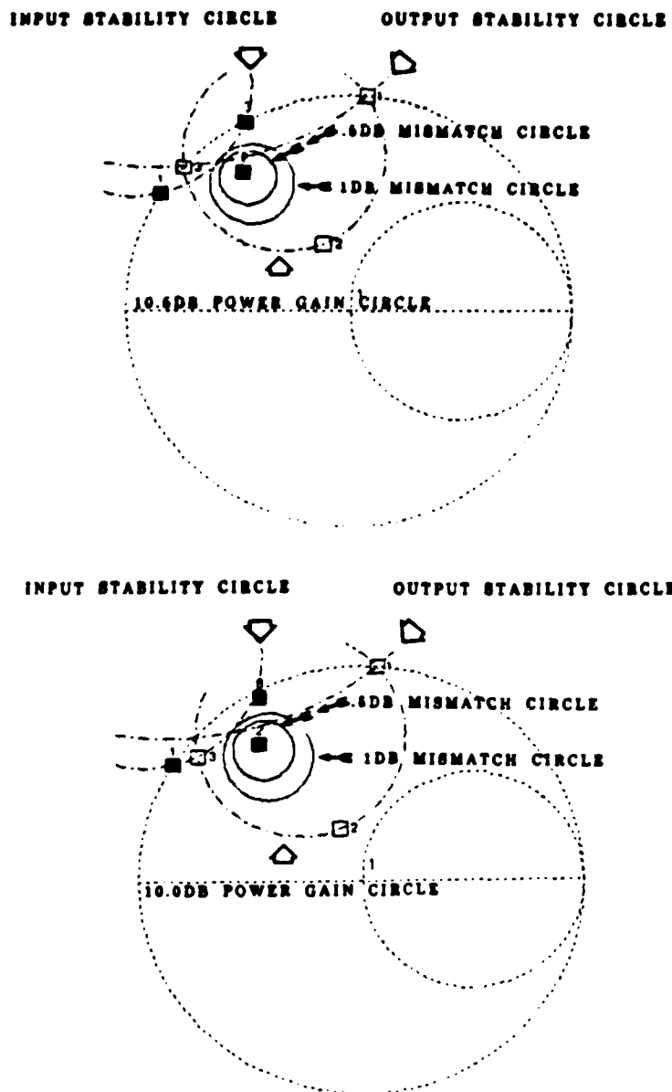
Figure 43b. 10.5 dB and 10.0 dB Power Gain Circles, 10 GHz Input and Output Stability Circles, and 1 dB and 0.5 dB Mismatch Circles Used for 10 GHz Amplifier Design
