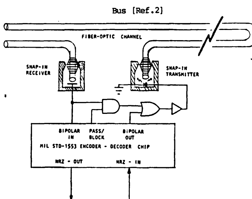
Figure 3b. Fiber Optic Implementation of Mil Std-1553
