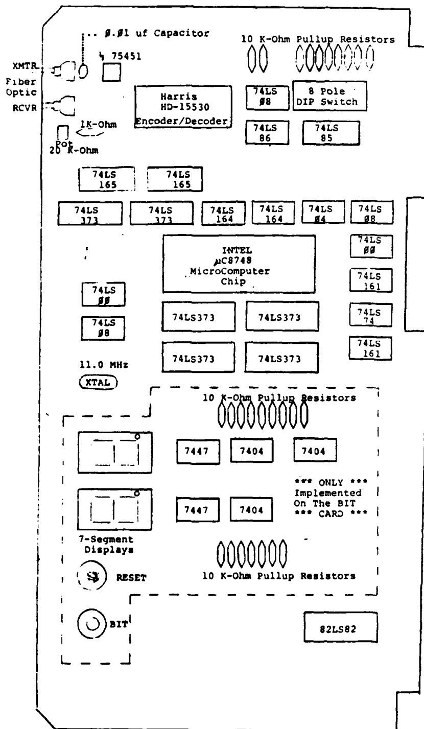
Figure A1. Mil Std-1553 Card Chip Placement
