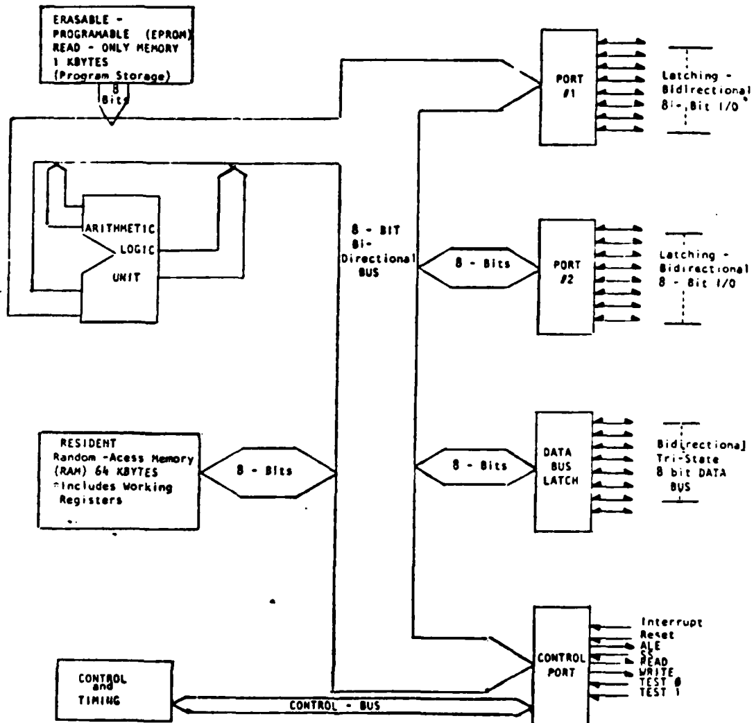
Figure 7. Block Diagram of the MC8748 (Ref. 4)
