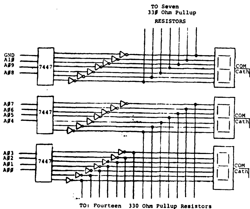
Figure C1. Single Step and Display Card Schematic
