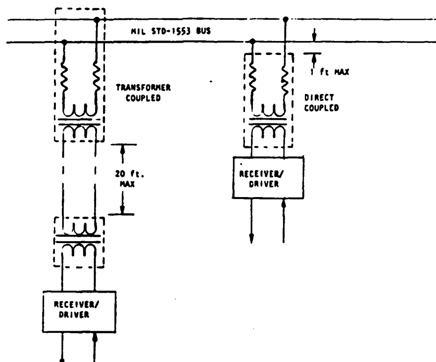
Figure 3a. Mil Std-1553 Transformer Coupled Coaxial Cable for Serial
