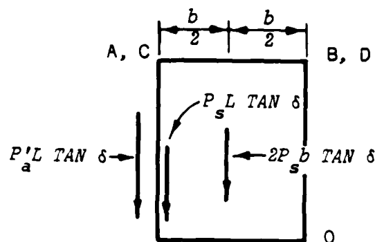
c. Friction forces producing resisting moment about 0
