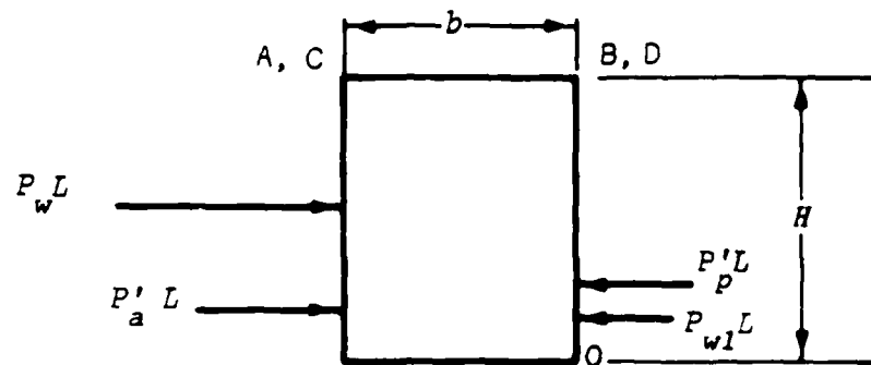
a. Driving force producing overturning moment about 0
