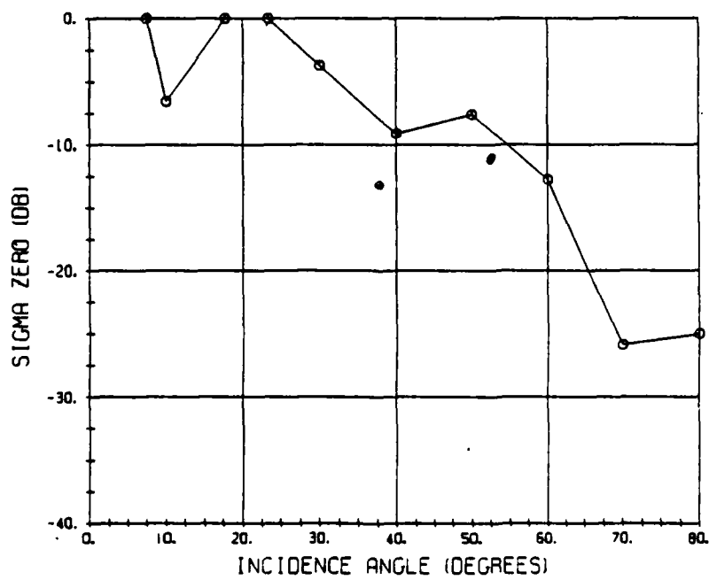
Figure 22 (b). Site H - Corn Stubble
