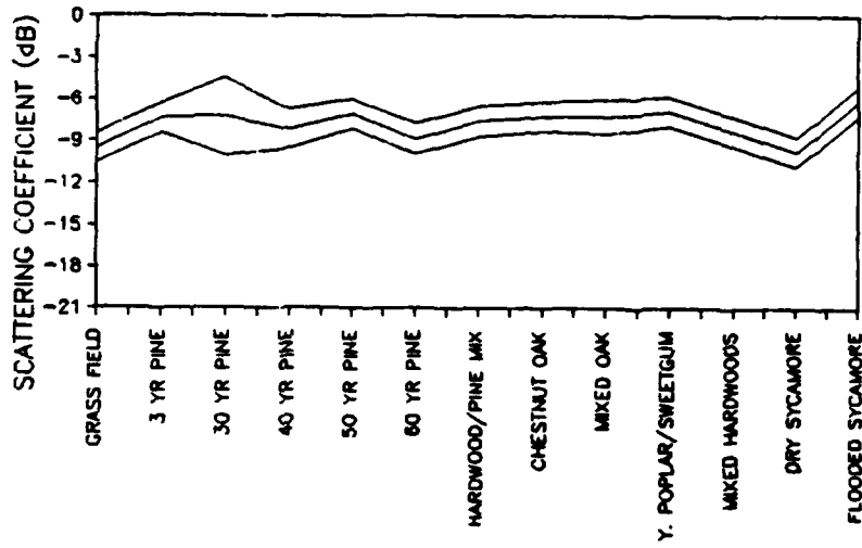
(b) C-band Data
