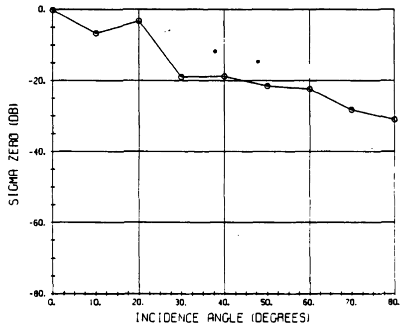
Figure 22 (c). Site K - Grass Field
