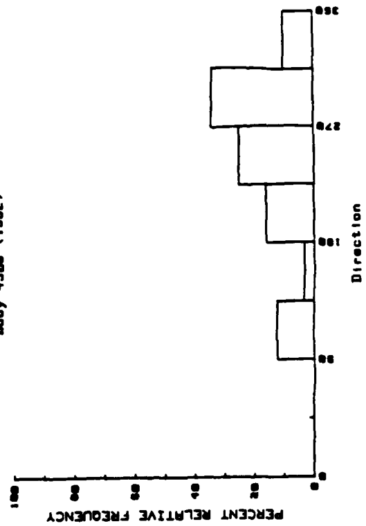
Buoy 4508 (1982)
