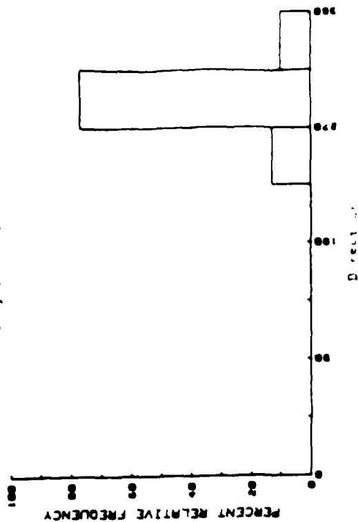
Buoy 261 (1979)
