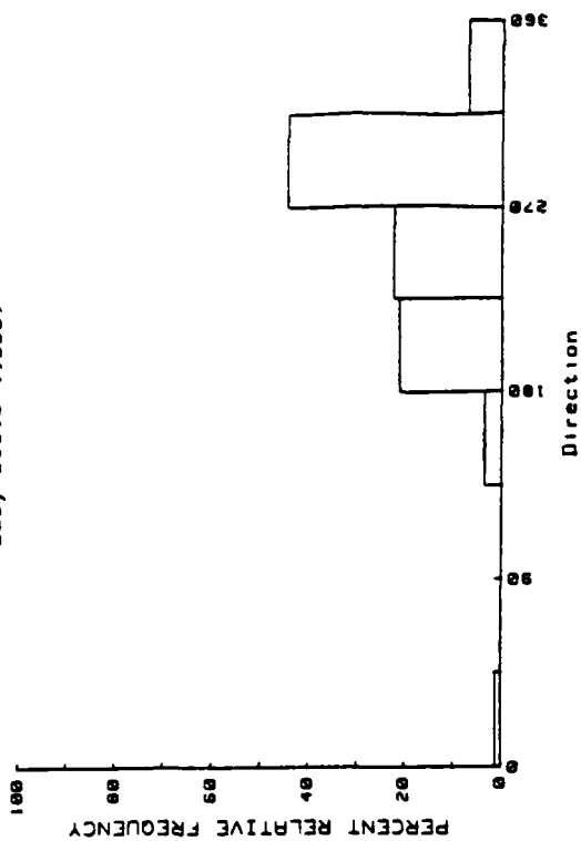
Buoy 2581b (1985)
