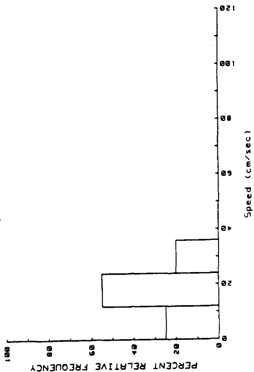
Buoy 4539 (1985)
