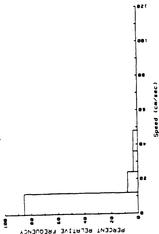
Buoy 4538 (1985)
