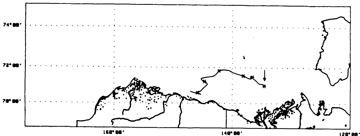
FIGURES 4-4c and 4-4d. TRAJECTORIES OF BUOYS 4507 AND 4508 (1982), RESPECTIVELY. EACH ASTERISK REPRESENTS 7 DAYS OF DRIFT.
