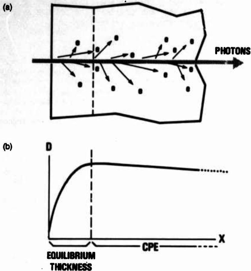
Figure 5. Charged particle equilibrium (CPE): (a) CPE is established at a depth approximately equal to range of secondary electrons; and (b) graph of dose as a function of material thickness.
