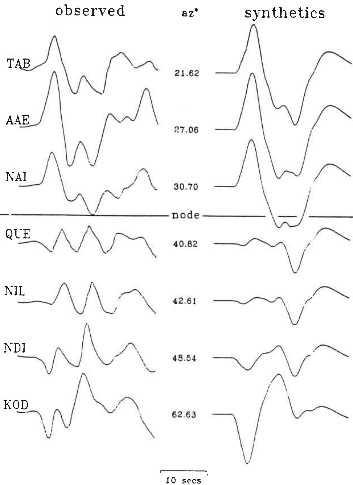
figure 15 - Observed P wave data from the September 29, 1969 South Africa event plotted adjacent to synthetics computed assuming a seaward thinning crust (dipping moho).
