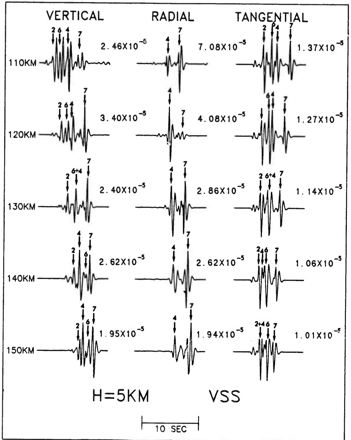
Figure 6 Generalized ray synthetics illustrating the complex interaction of rays #4 and #6 as a function of distance. Note the similarities to the wavenumber synthetics and the real events even though only seven ray paths, as shown in Figure 3, are specified.
