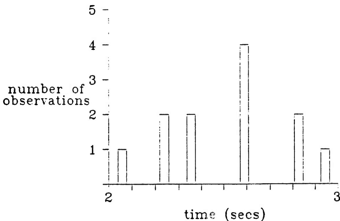
figure 10 - Histogram representing the number of short period records with a given sP-P time for the September 29, 1969 South Africa event. The short-period P wave recorded at ARE (WSSN station) shows sP-P separation. Measurement error is estimated to be \pm 0.1 seconds.
