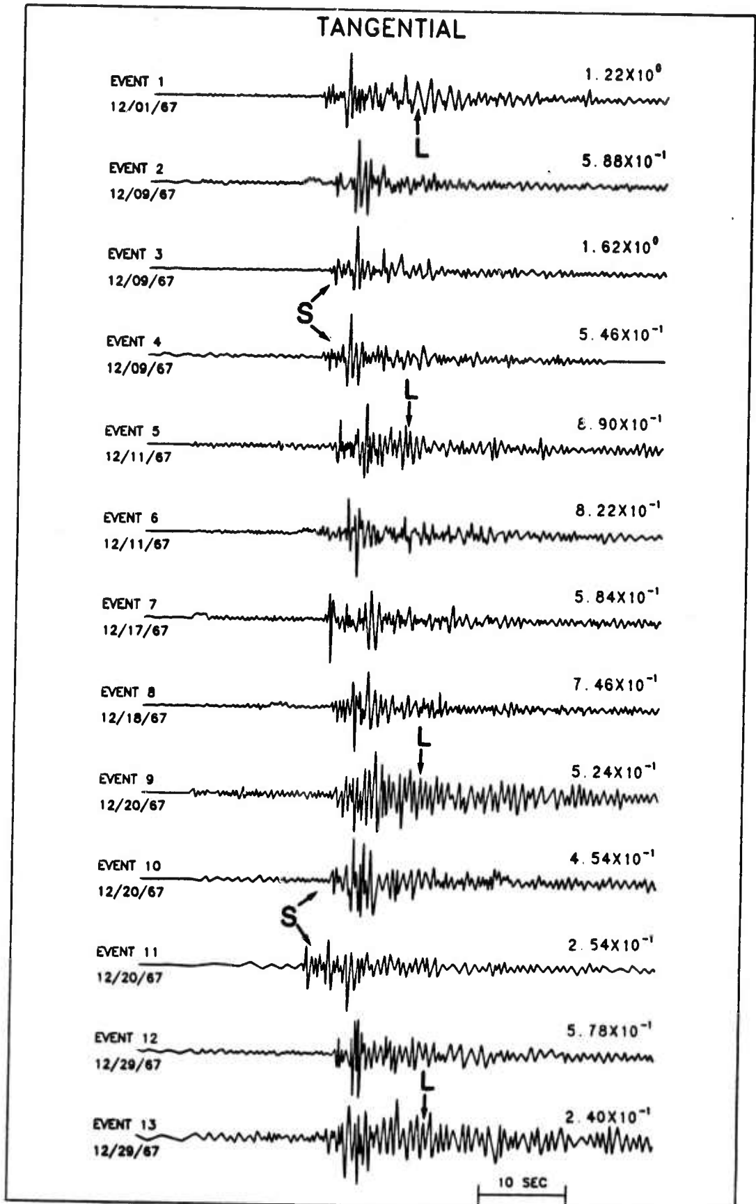
Figure 2.3 Tangential component of the thirteen digitized Koyna events of December 1967 recorded at P00. Major phases are denoted by S and L (Love). Amplitudes are normalized and given in microns.
