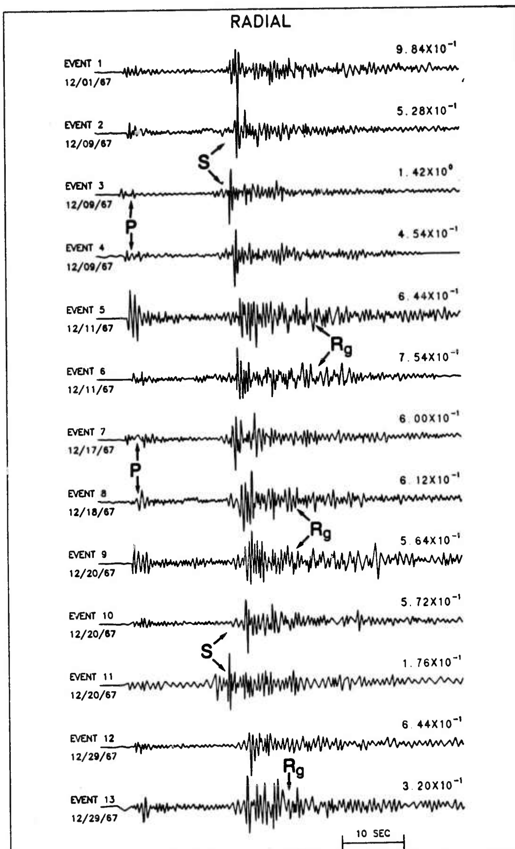
Figure 2.2 Radial component of the thirteen digitized Koyna events of December 1967 recorded at POO. Major phases are denoted by P, S and Rg. Amplitudes are normalized and given in microns.
