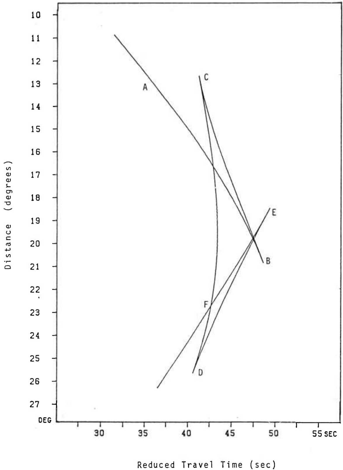
Figure 3b. Reduced travel-time curve for the E19 upper mantle velocity model. Travel times are reduced by 10.3 km/sec.
