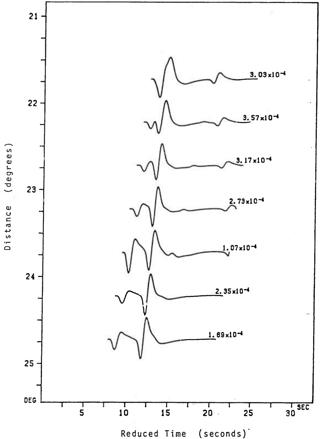
Figure 11. Intermediate-period synthetic seismograms calculated for S8. Absolute travel times are reduced by 10.3 km/sec and advanced by 30 seconds. Note that the SCP observation (figure 9) resembles the S8 synthetic at 22.25°
