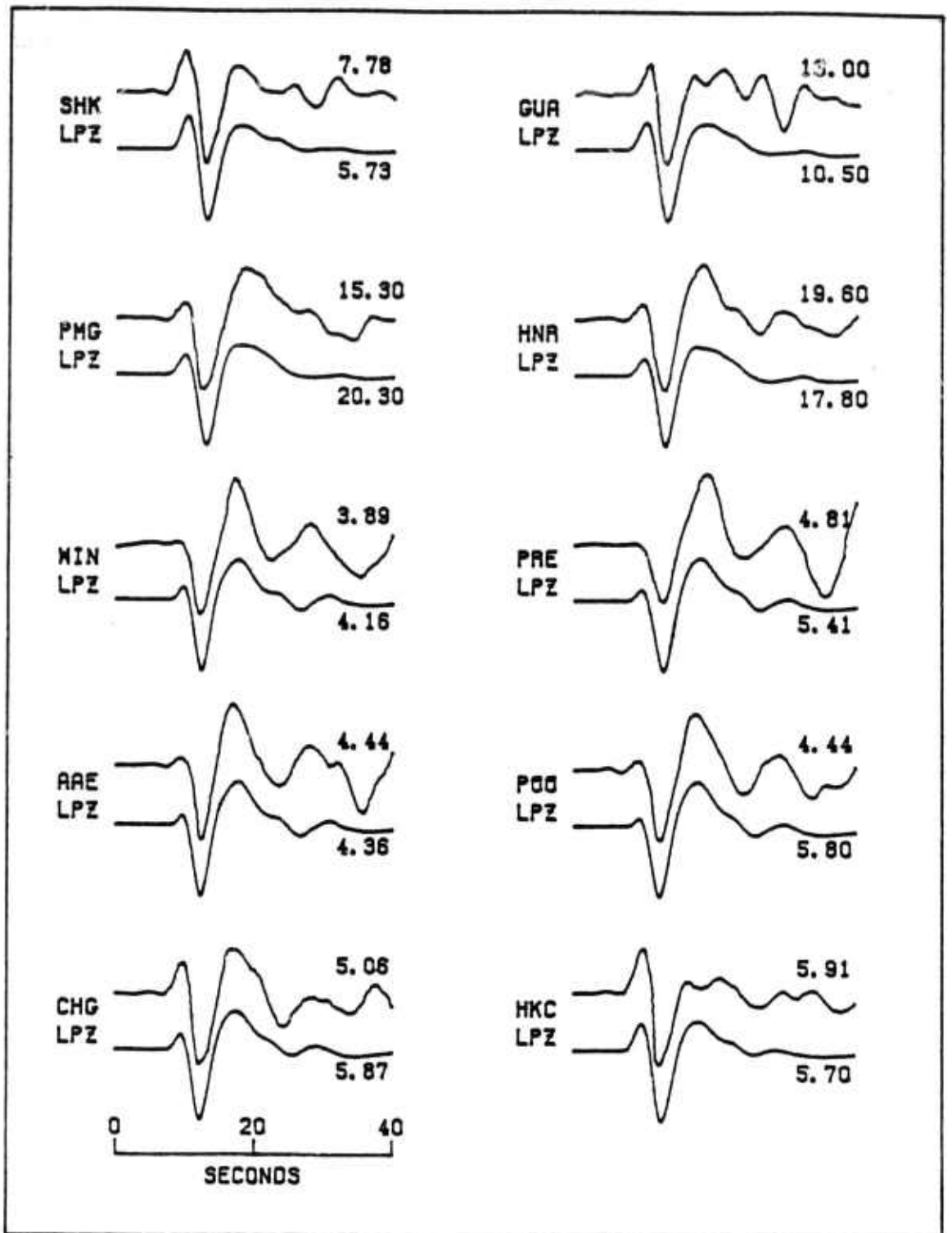
Figure 14. Observed (above) and synthetic (below) long period P waveforms for model 2.
