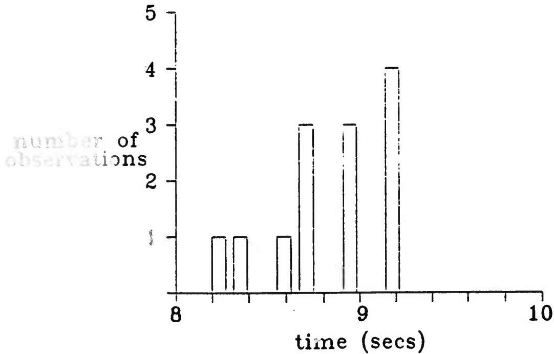
figure 6 - Histogram representing the number of short period records with a given pP-P time for the May 15, 1968 Zambia event. The short-period P wave recorded at P00 (WSSN station) shows pP-P separation.
