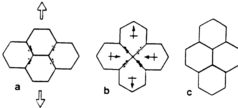
Figure 2.1 Ashby-Verrall Grain Boundary Sliding Model.
