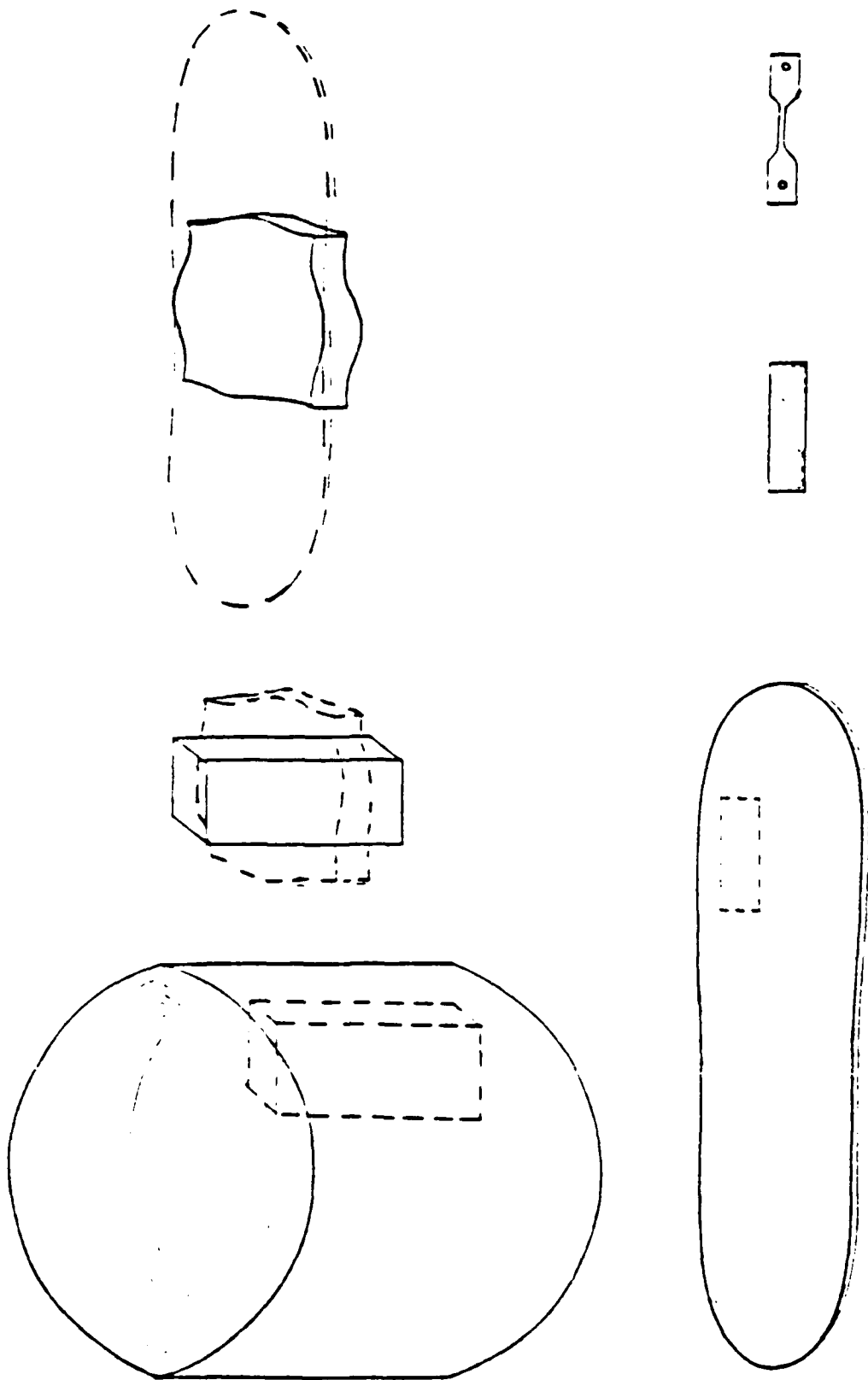
Figure 3.4 Evolution of Tensile Test Specimens.
