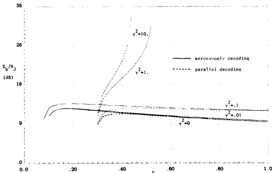
Fig. 1 — Minimum E_b/N_J required for P_e = 10^{-3} vs \rho for asynchronous FH/SSMA communications using RS(64,32) codes with error-only and parallel erasure/error decoding ( q = 100 , N_b = 12 , M = 8 , m = 2 , E_b/N_0 = 12 dB, K = 5 ); Rician fading channel with varying \gamma^2 .
