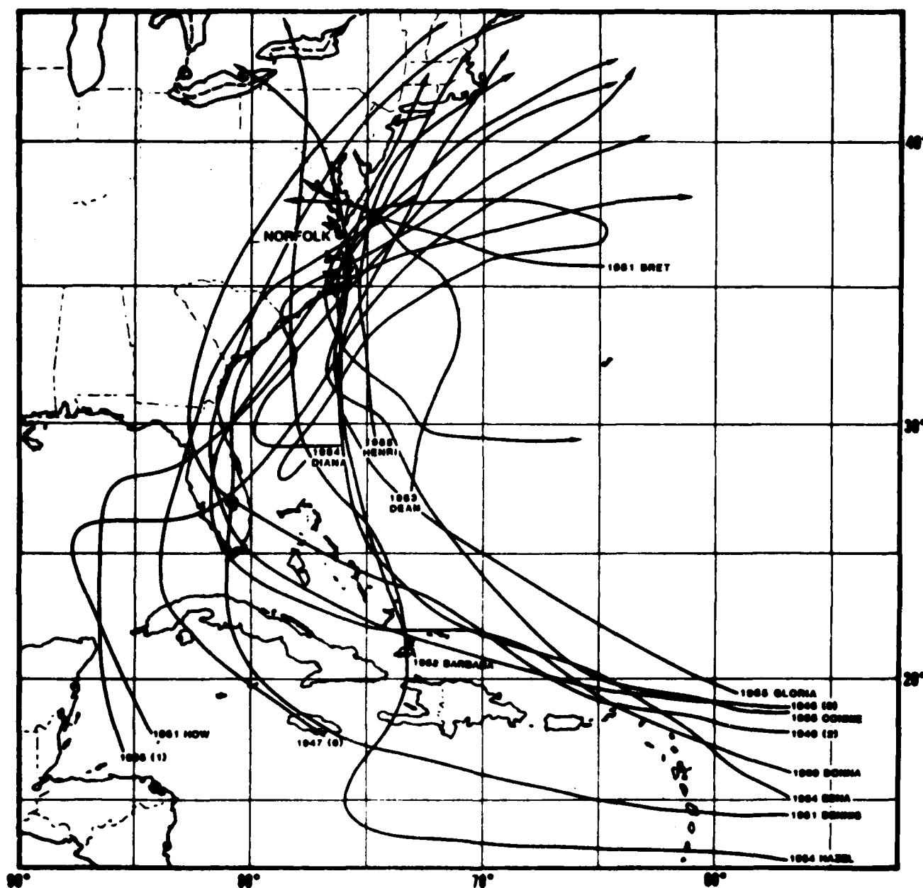
Figure II-12. Tracks of 17 tropical cyclones that produced winds of 34 kt or greater at NAS Norfolk (based on data from 1945-85).
