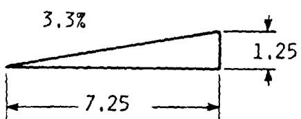
Fig. 8. Force model fences. Dimensions in inches. (Continued).
