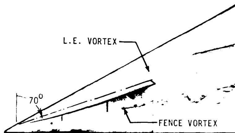
FENCE SWEPT 70°
