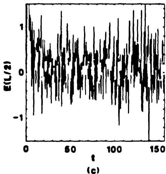
Fig. 12. Time histories of electric field in center of simulation region for four different runs. (a) and (b) are quiet injection runs with (b) having four times as many particles as (a), and (c) and (d) are noisy injection runs with (d) having four times as many particles as (c). RMS value of E in (b) should be 1/4 that of (a), and RMS value of E in (d) should be half that of (c).
