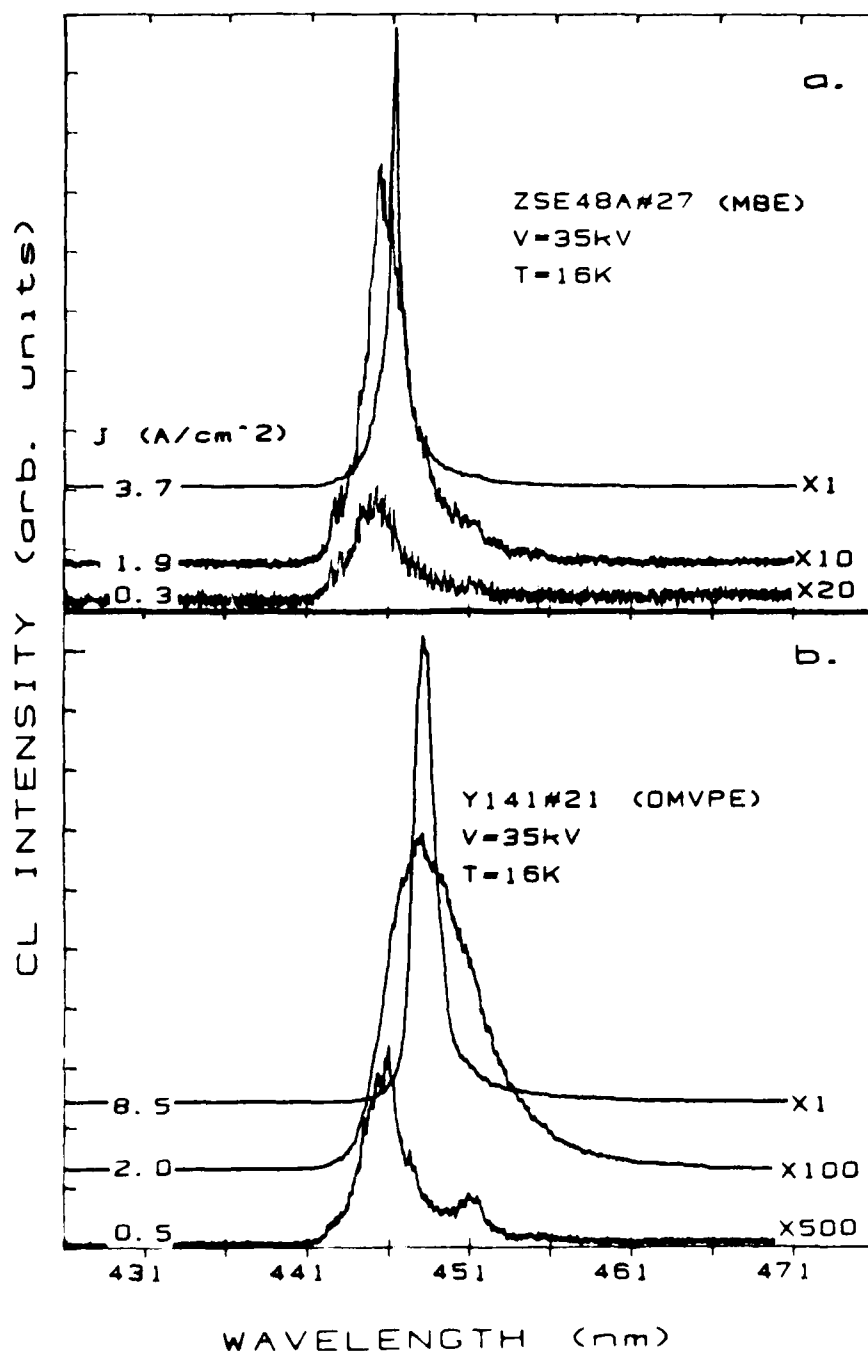
Figure 2-29. Spectral output of ZnSe films prepared by (a) MBE, and (b) OMVPE for differing incident electron beam current densities as indicated. Measurements were made by a gated OMA at T = 16K with an accelerating voltage of 35 kV.
