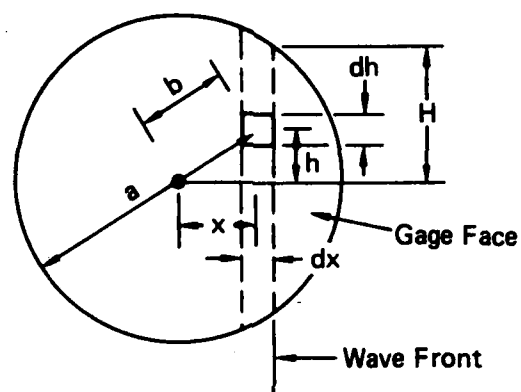
FIGURE B.1 NOMENCLATURE FOR ANALYSIS OF THE RESPONSE OF THE SE DIAPHRAGM GAGE TO A SWEEPING WAVE
