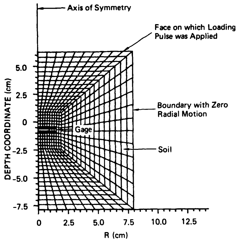
(a) Configuration for the Embedded Gage Computation after 500 \mu s
