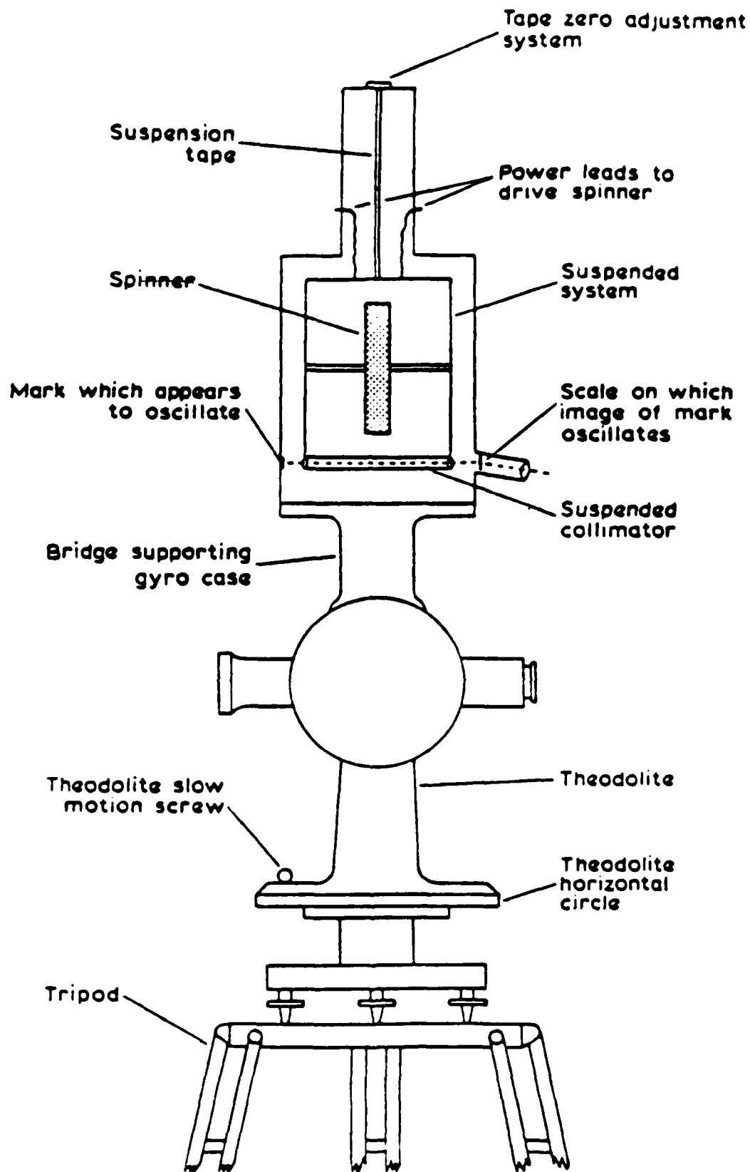
Figure 1. Suspended gyro.
