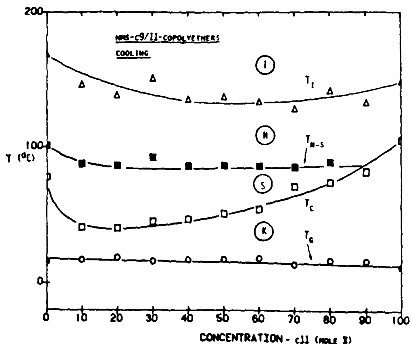
Figure 6: Thermal transitions ( T_g , T_c , T_{N-S} , and T_i ) for the HMS-C9/11 copolyethers as a function of copolymer composition on the cooling scan.
