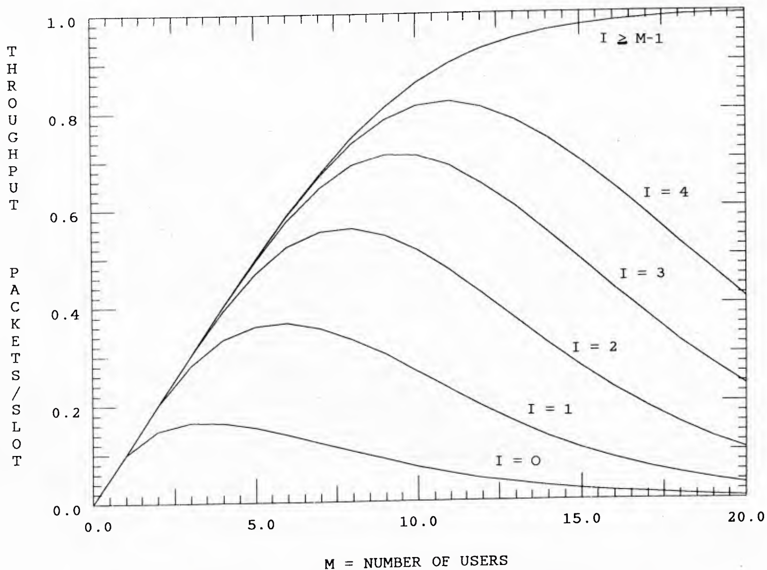
Fig. 10 Throughput performance of distributed reservation scheme; threshold model for effects of other-user interference: several values of I are shown; Q = 3 .
