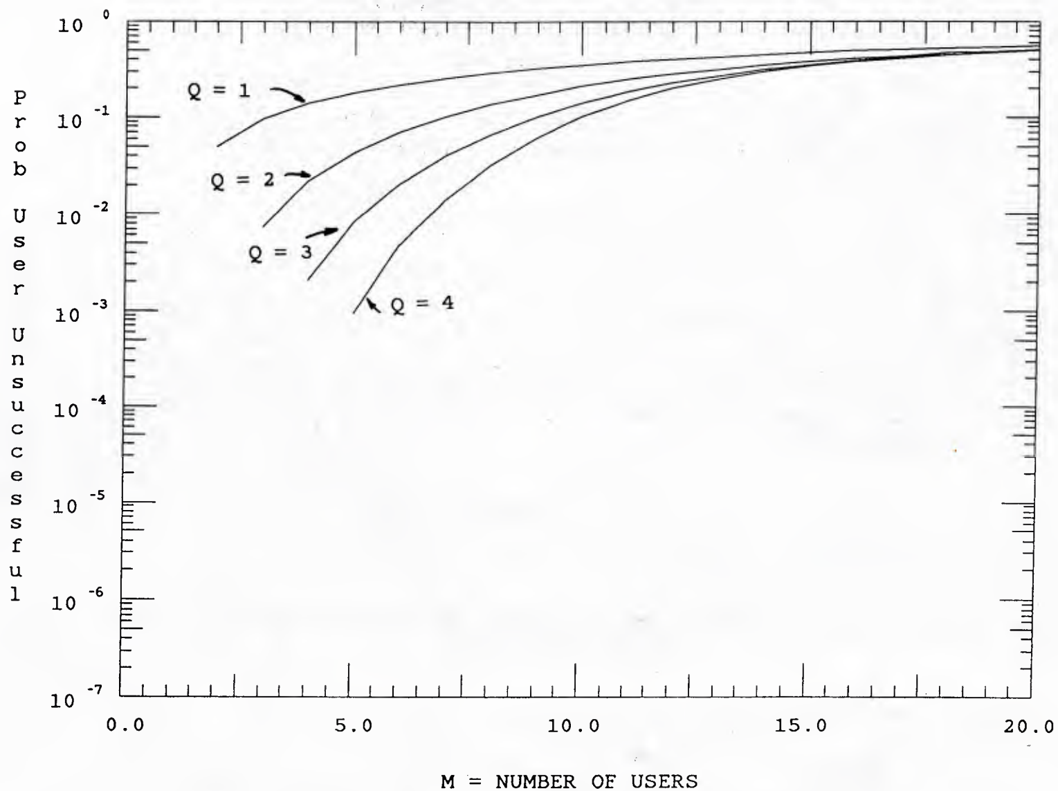
Fig. 6 Probability a user is unsuccessful under distributed reservation scheme; orthogonal CDMA codes.
