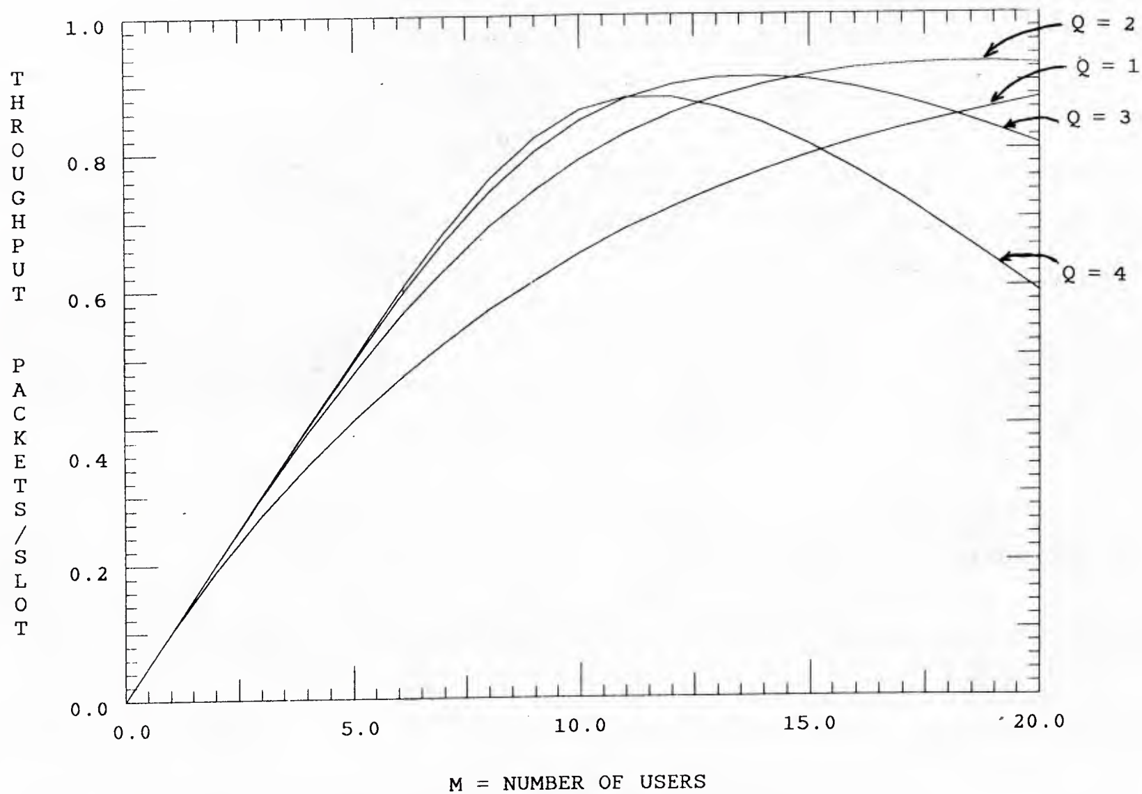
Fig. 12 Throughput performance of distributed reservation scheme; RS(32,16) coding; noiseless channel; q = 50 frequency bins; Q = 1, 2, 3, 4 .
