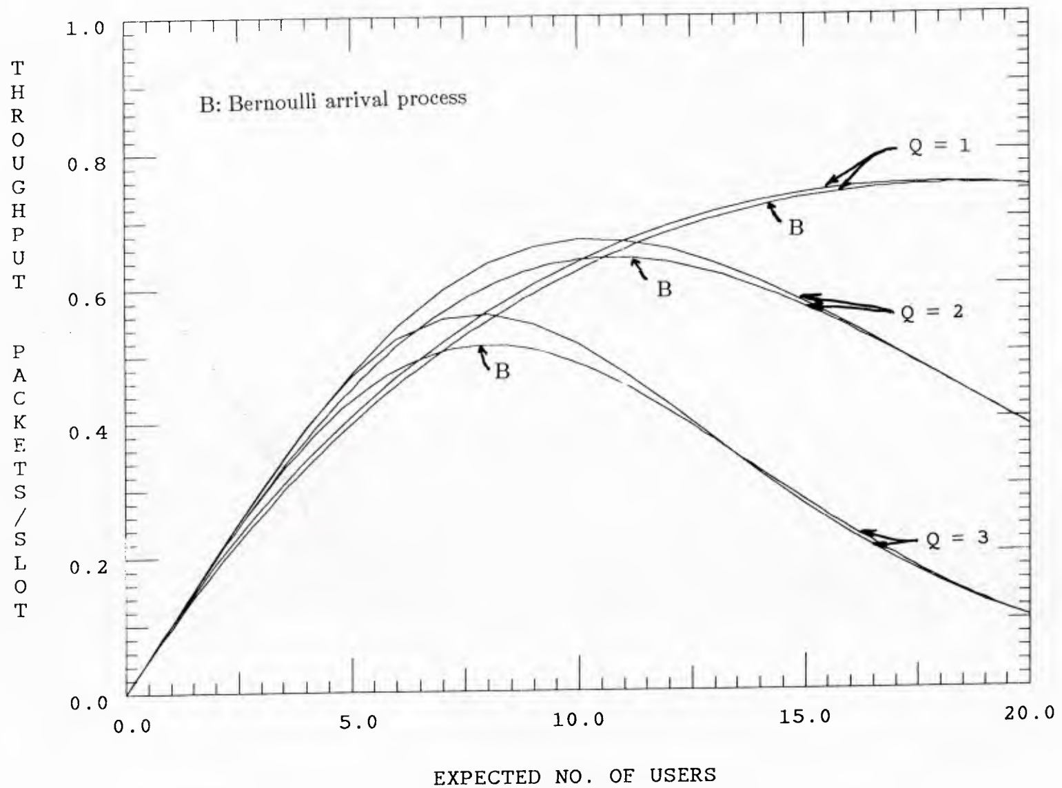
Fig. 15 Throughput performance of distributed reservation scheme; Bernoulli arrival process ( M = 20 users) compared with system in which all users transmit; threshold model for effects of other-user interference: 2 other users can be tolerated; Q = 1, 2, 3 .
