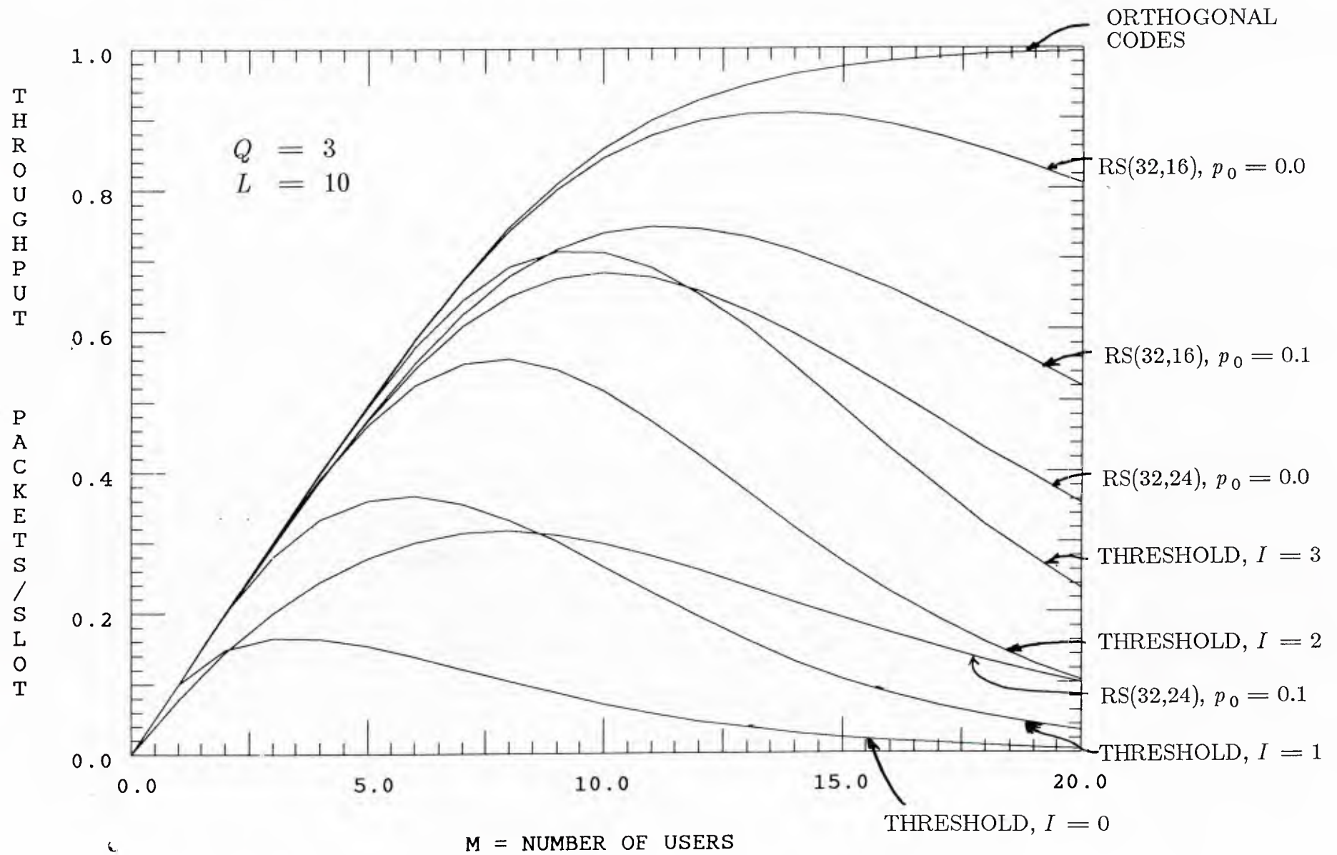
Fig. 11 Throughput performance of distributed reservation scheme; probabilistic (Reed-Solomon coding with q = 50 frequency bins) model for effects of other-user interference compared with threshold model.
