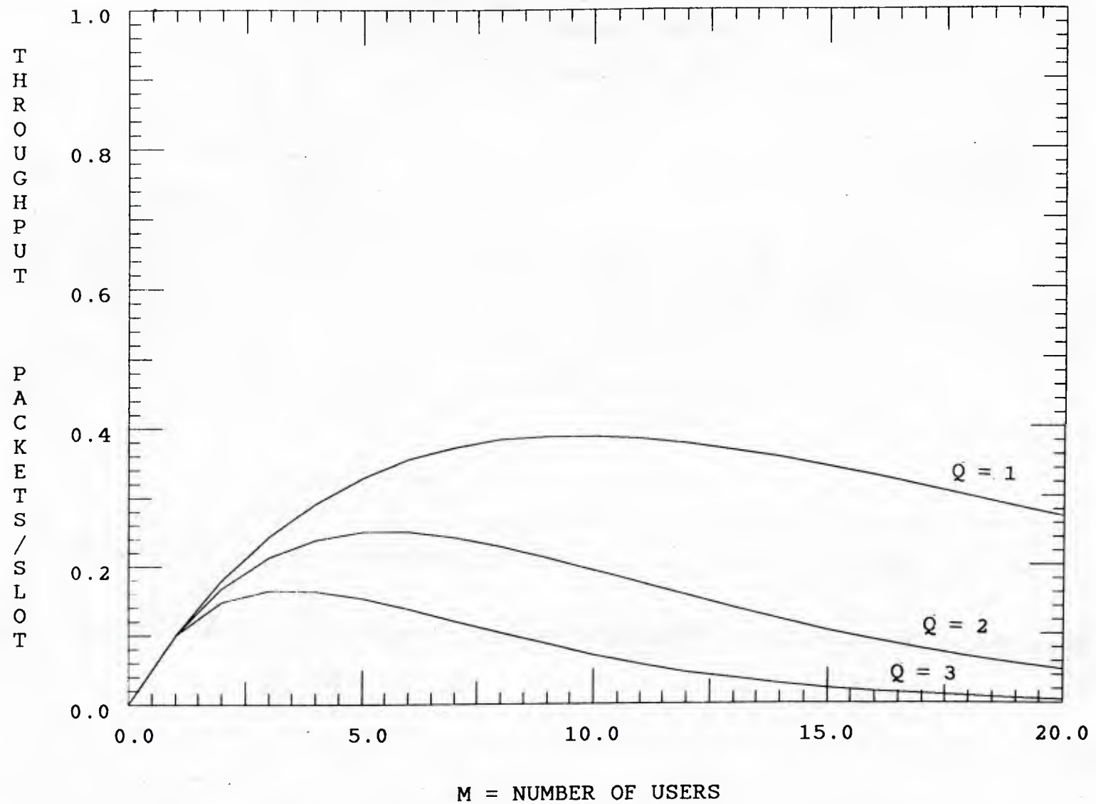
Fig. 8 Throughput performance of distributed reservation scheme; no other users can be tolerated in same slot.
