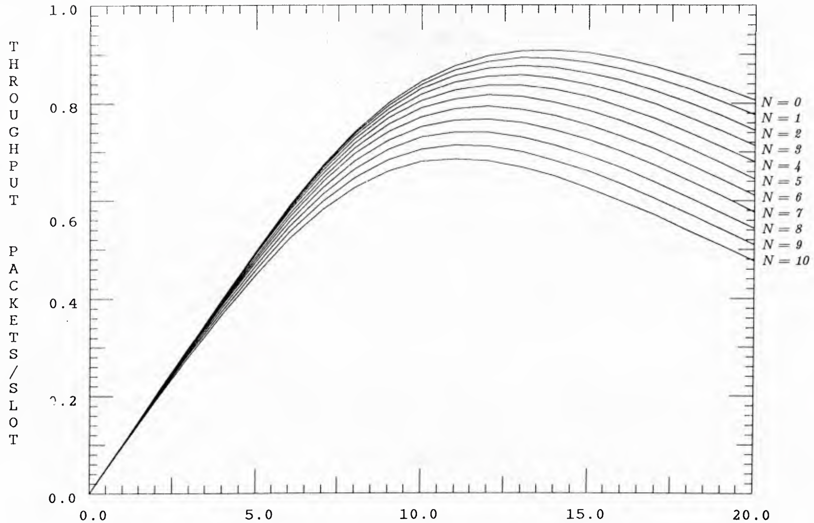
Fig. 16 Throughput performance of distributed reservation scheme; M is the number of users that make reservations successfully; N is the number of additional FH users that share channel; RS(32,16) coding; noiseless channel; q = 50 frequency bins; Q = 3
