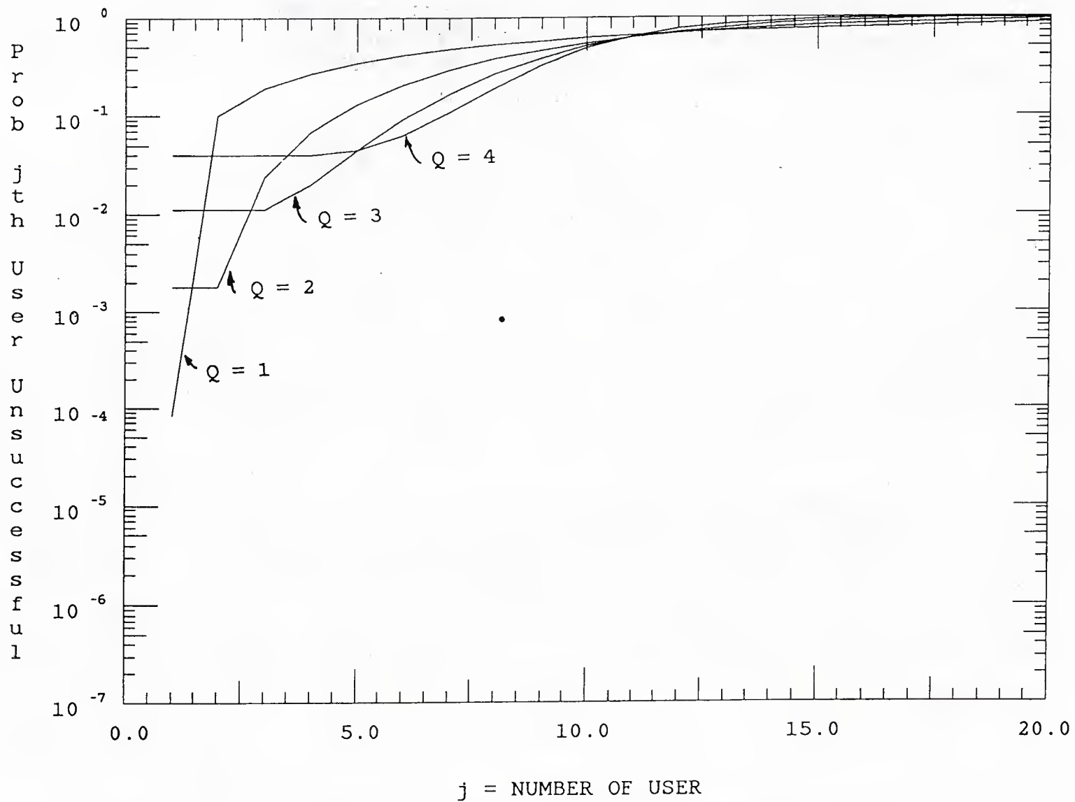
Fig. 14 Probability j^{\text{th}} user is unsuccessful for distributed reservation scheme; RS(32,16) coding; noiseless channel; M = 20 users; q = 100 frequency bins; Q = 1, 2, 3, 4 .
