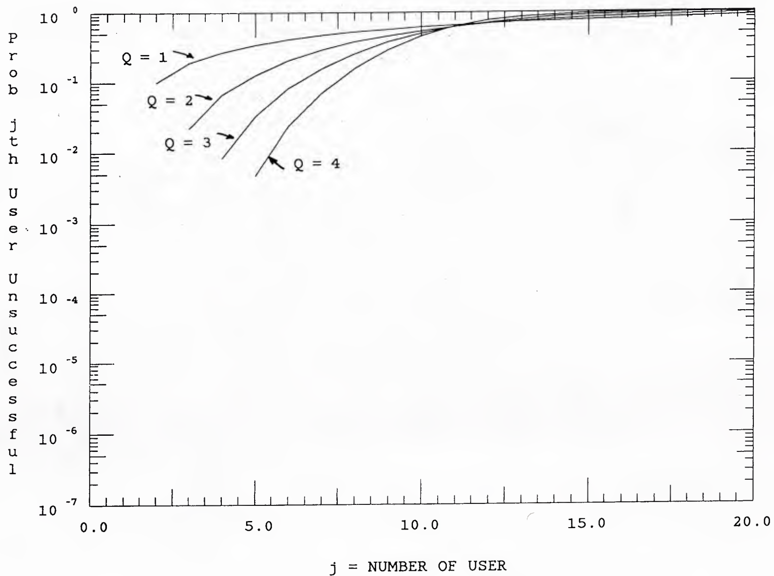
Fig. 7 Probability j^{th} user is unsuccessful under distributed reservation scheme; orthogonal CDMA codes.
