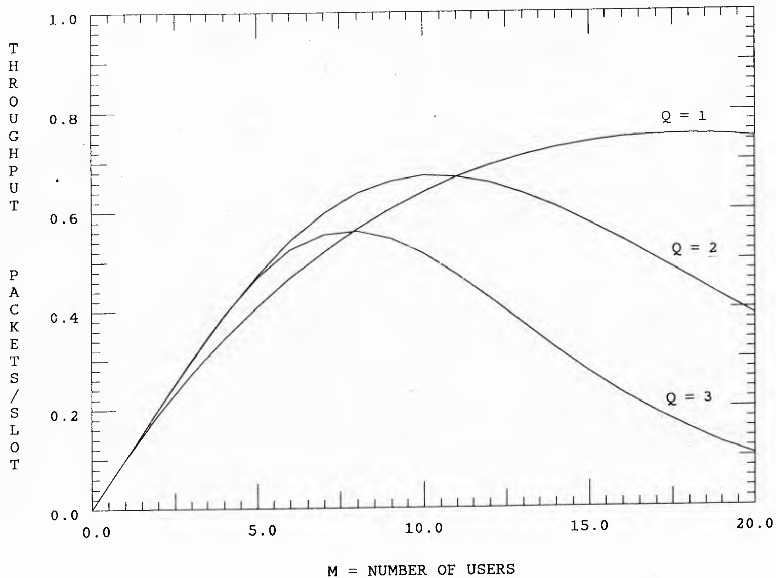
Fig. 9 Throughput performance of distributed reservation scheme; threshold model for effects of other-user interference: 2 other users can be tolerated in same slot.
