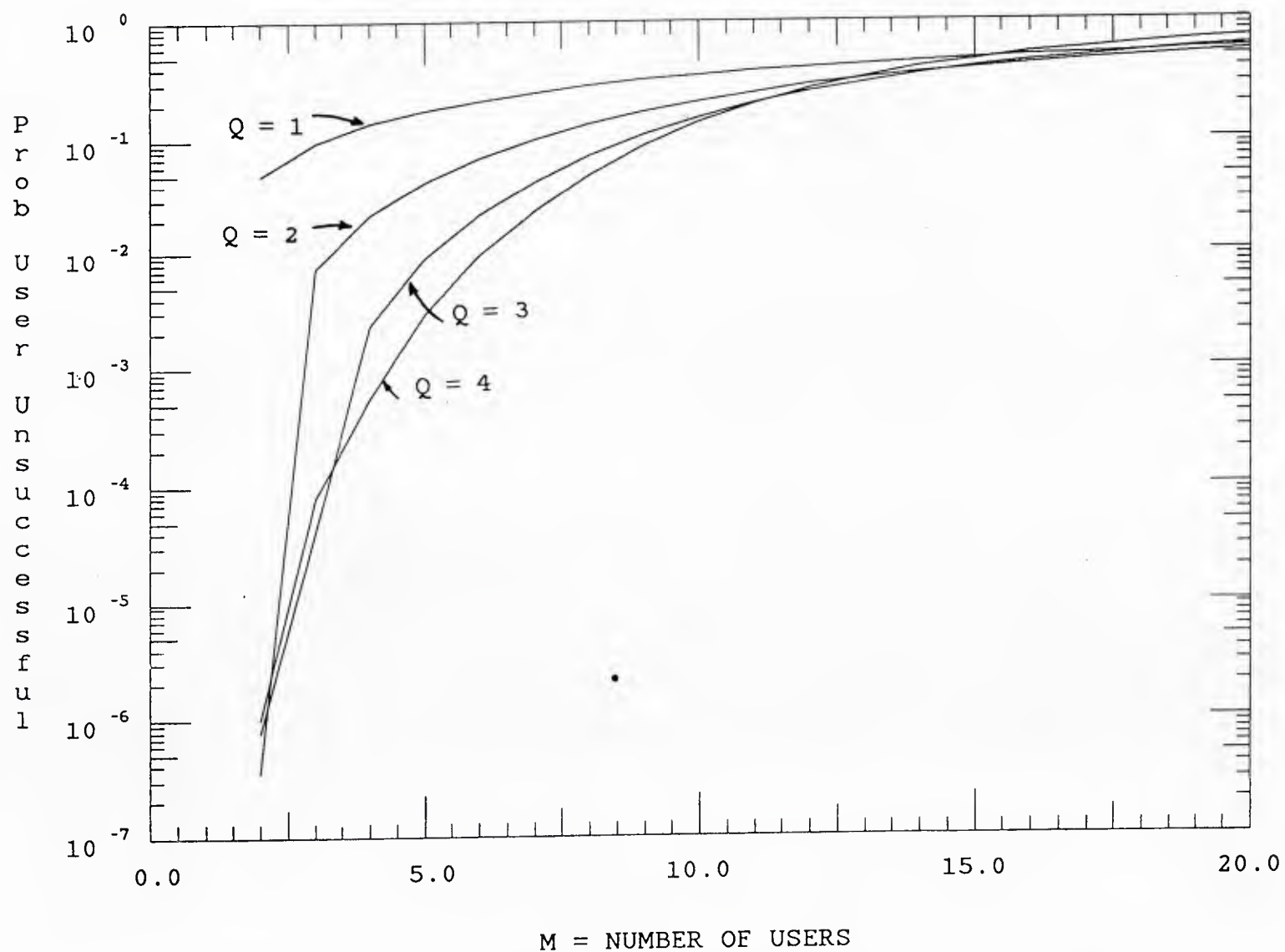
Fig. 13 Probability a user is unsuccessful for distributed reservation scheme; RS(32,16) coding; noiseless channel; q = 50 frequency bins; Q = 1, 2, 3, 4 .
