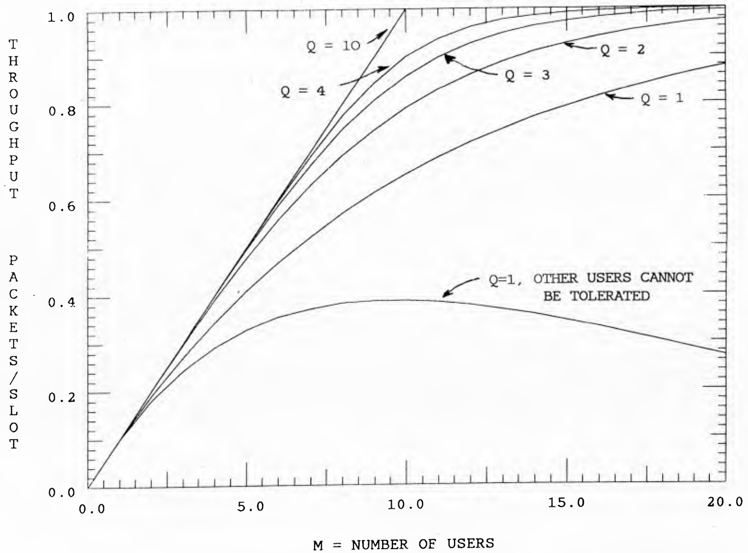
Fig. 5 Throughput performance of distributed reservation scheme; orthogonal CDMA codes.
