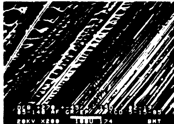
Figure 6-19. +45/-45 Plies at -65°F Dry, 70°F Dry, and 270°F Dry Conditions (SEM 200X)
