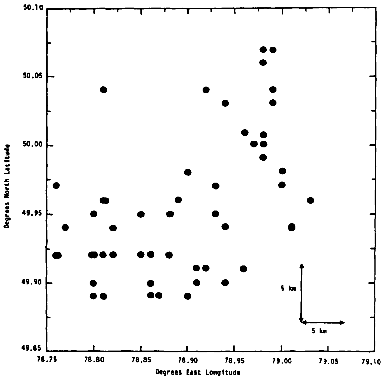
Figure 3. Map showing the JED relocations of Shagan River explosions used in this study.
